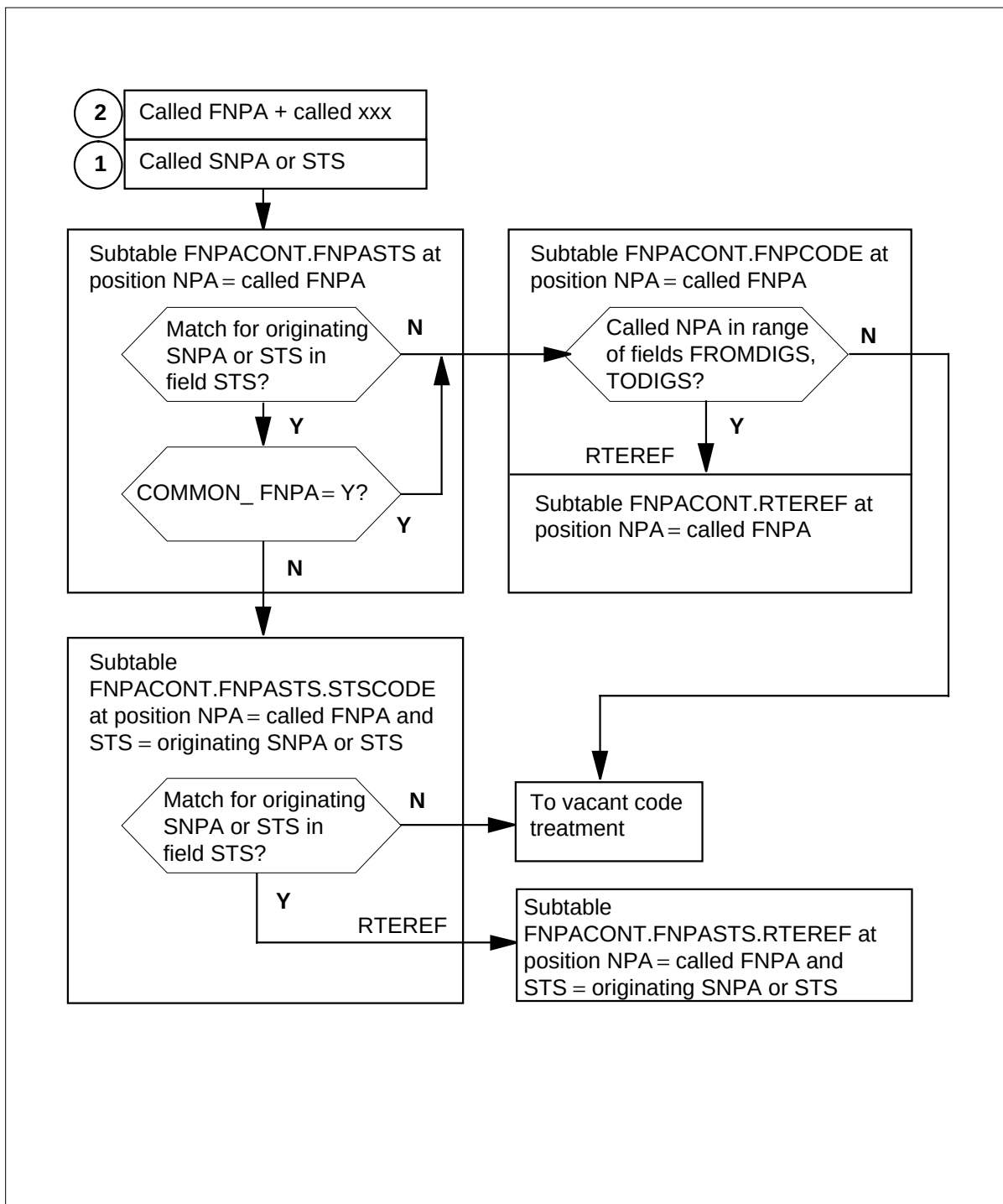
Six-digit translation flow diagram: tableFNPACONT and subtables for six-digitxx
