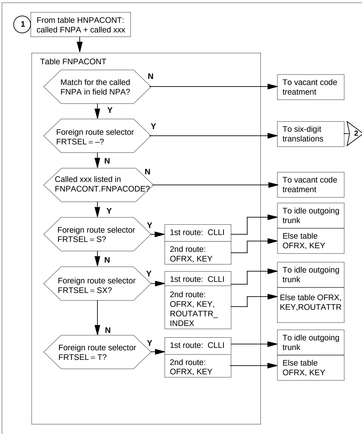
Six-digit translation flow diagram: table FNPACONT
