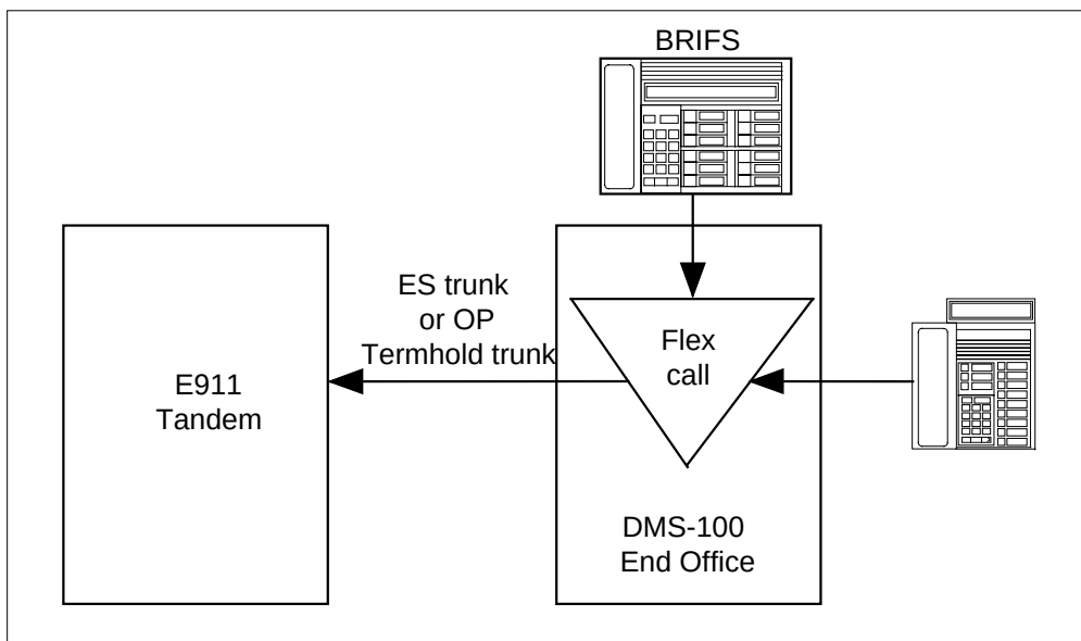
Flex Call interworking with E911 in end office
