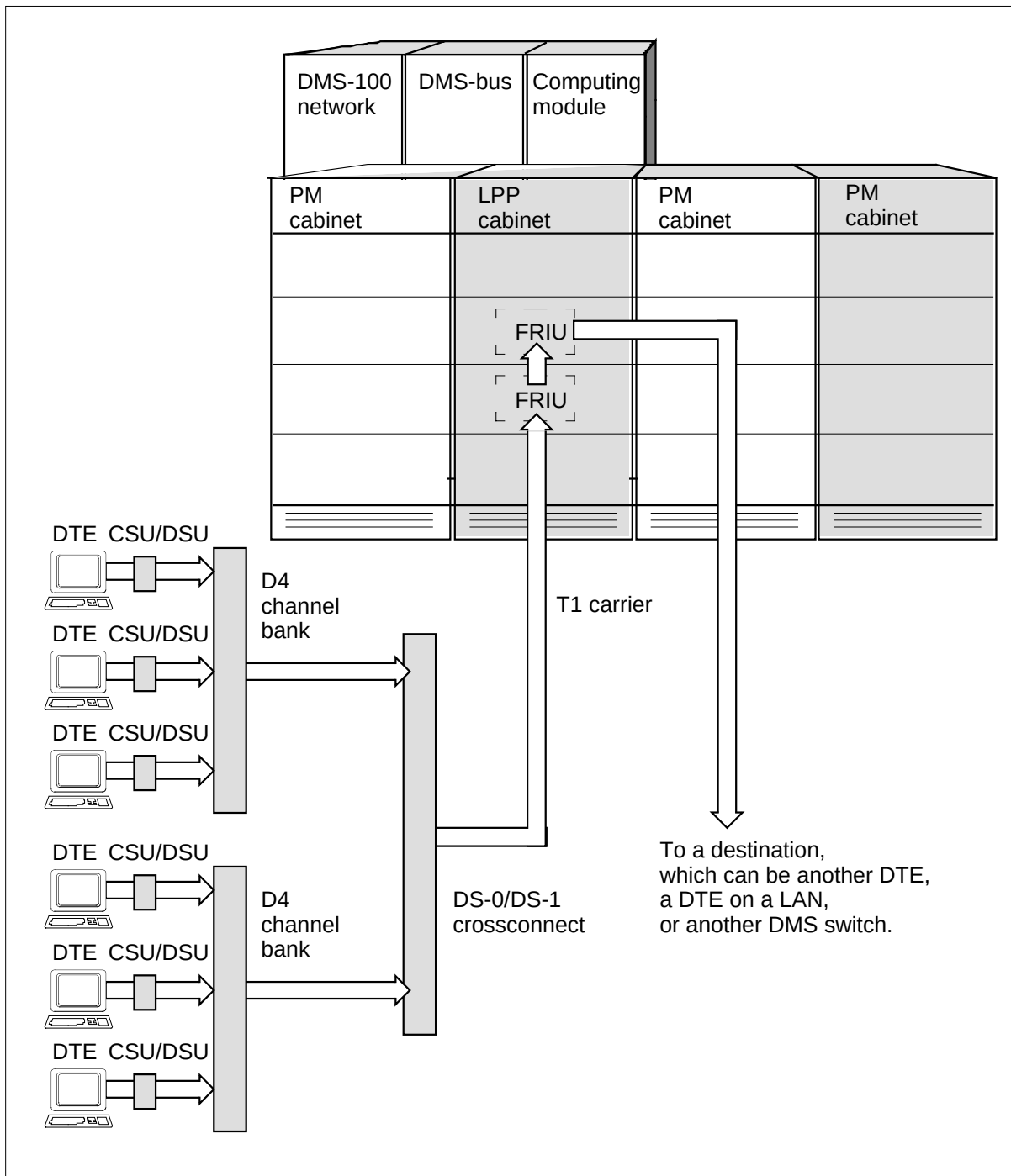
Transmission path for non-ISDN channelized access
