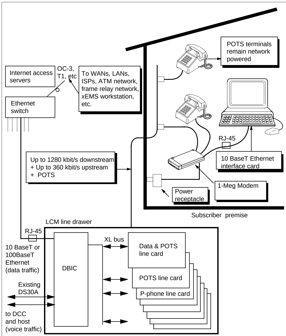
Figure 1-1 1-Meg Modem Service system overview
