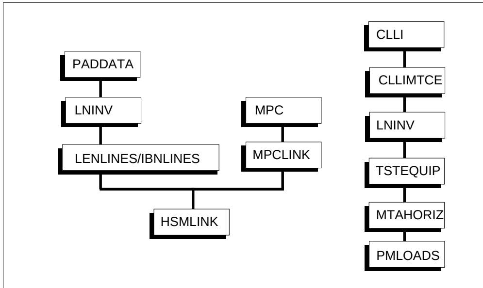
Datafill dependencies for ESTU - Enhanced Services Test Unit
