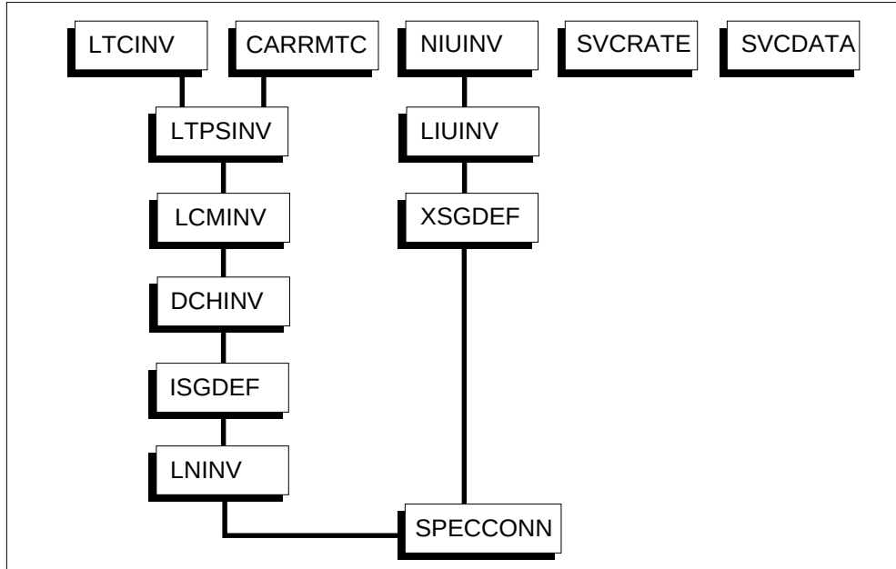
Datafill dependencies for ISDN BRI office configuration tables
