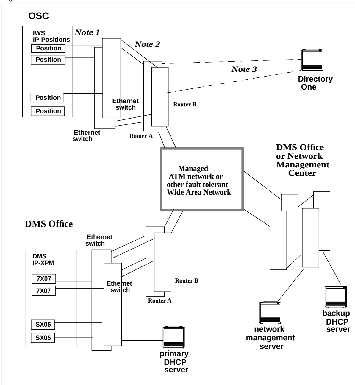
Figure 279 TOPS-IP network: OSC connected to DMS office via WAN
