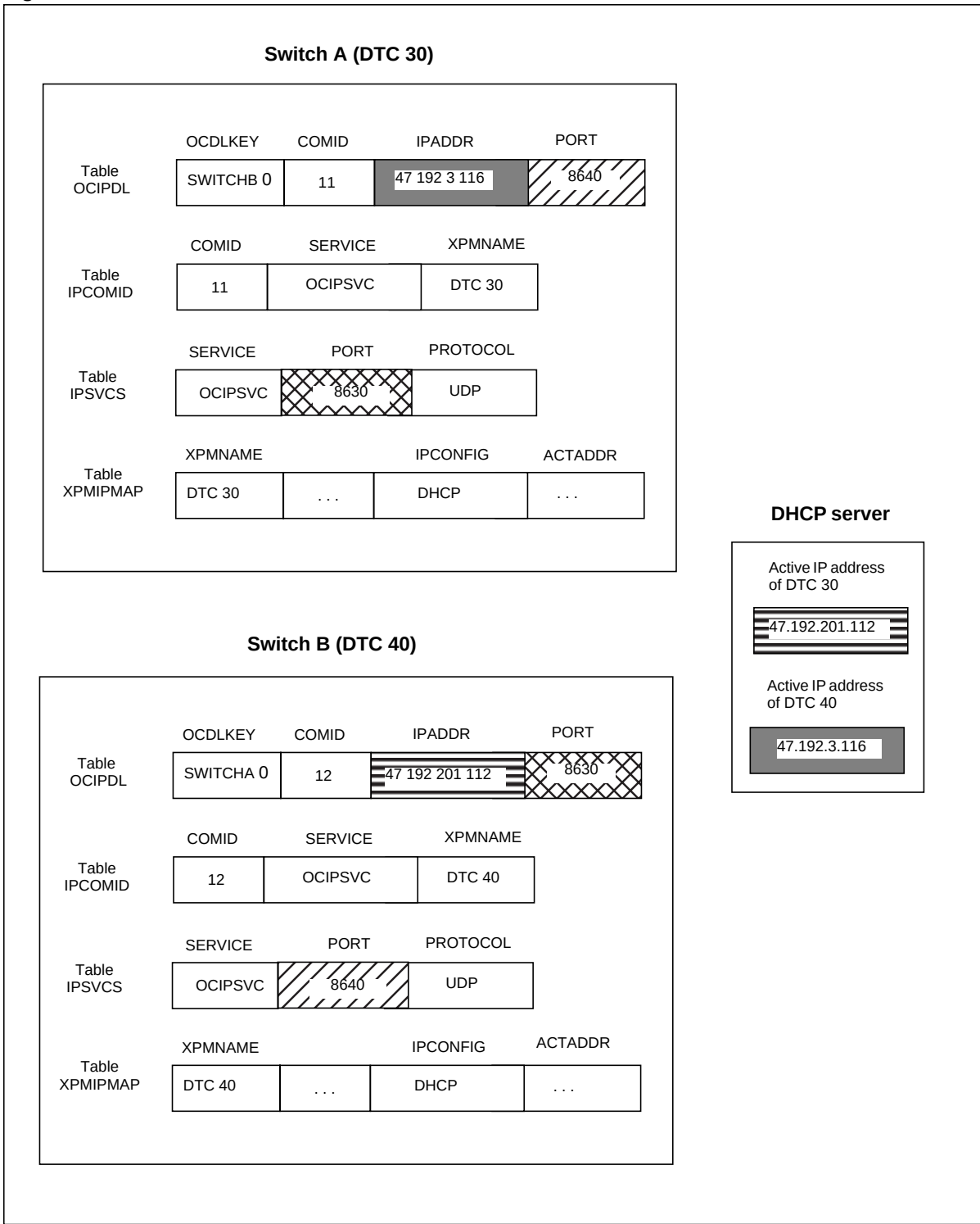
Figure 47 Parallel datafill for OC-IP data links—network method
