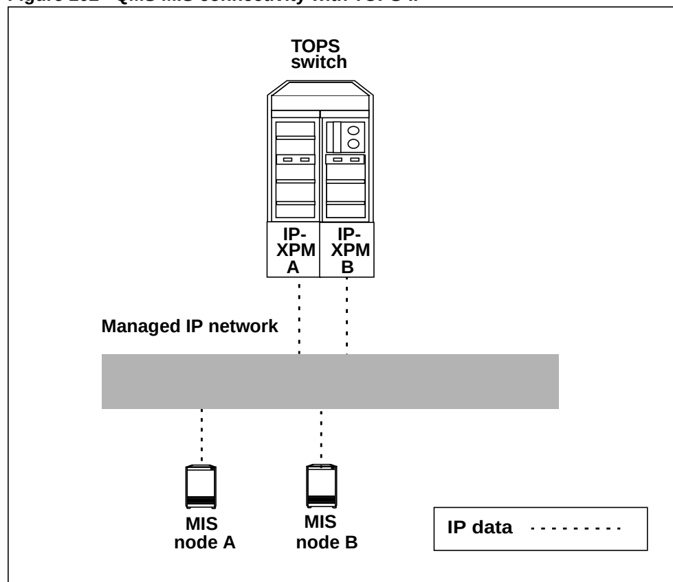
Figure 102 QMS MIS connectivity with TOPS-IP
