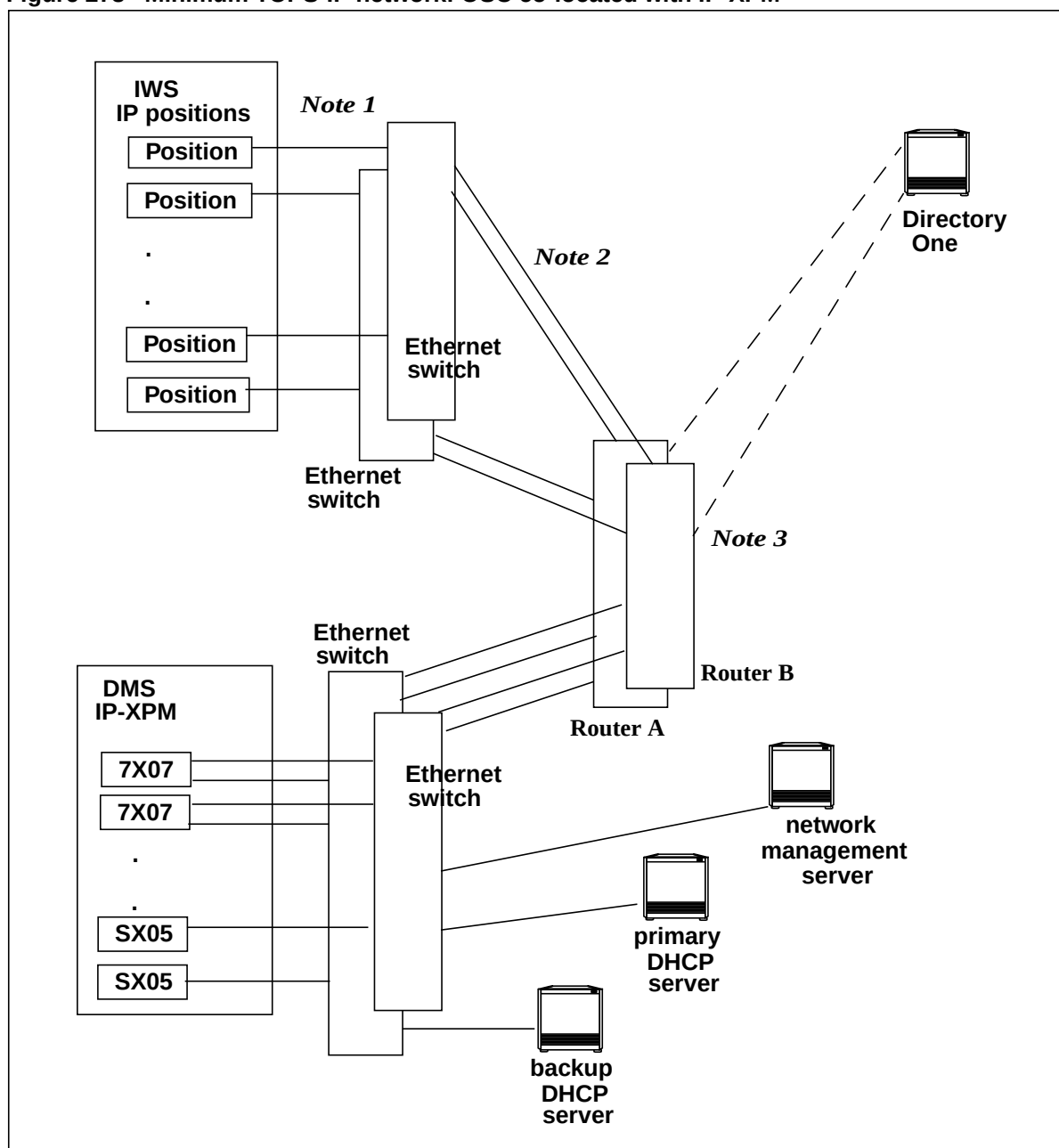
Figure 278 Minimum TOPS-IP network: OSC co-located with IP-XPM
