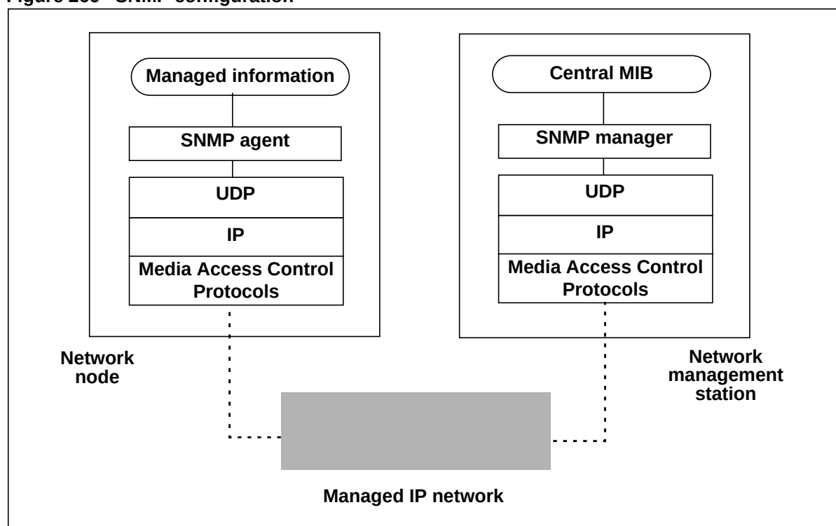
Figure 266 SNMP configuration
