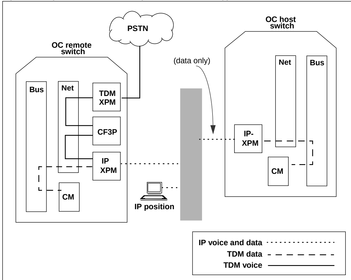
Figure 71 IP position voice and data paths for host voice bypass call
