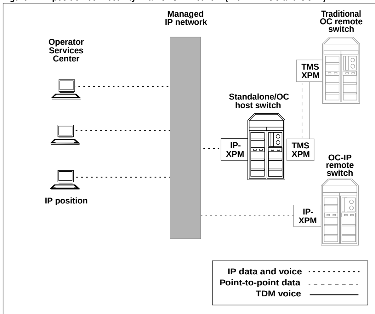
Figure 7 IP position connectivity in a TOPS-IP network (with TDM OC and OC-IP)
