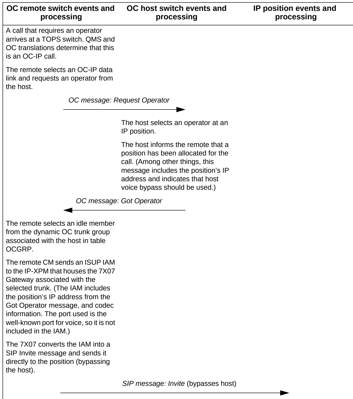
Figure 100 Example of IP position call flow with OC-IP call flow
