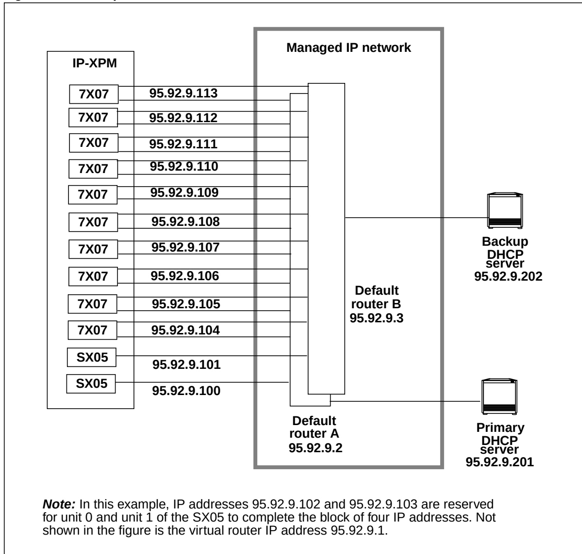
Figure 265 Example IP addresses for one subnet
