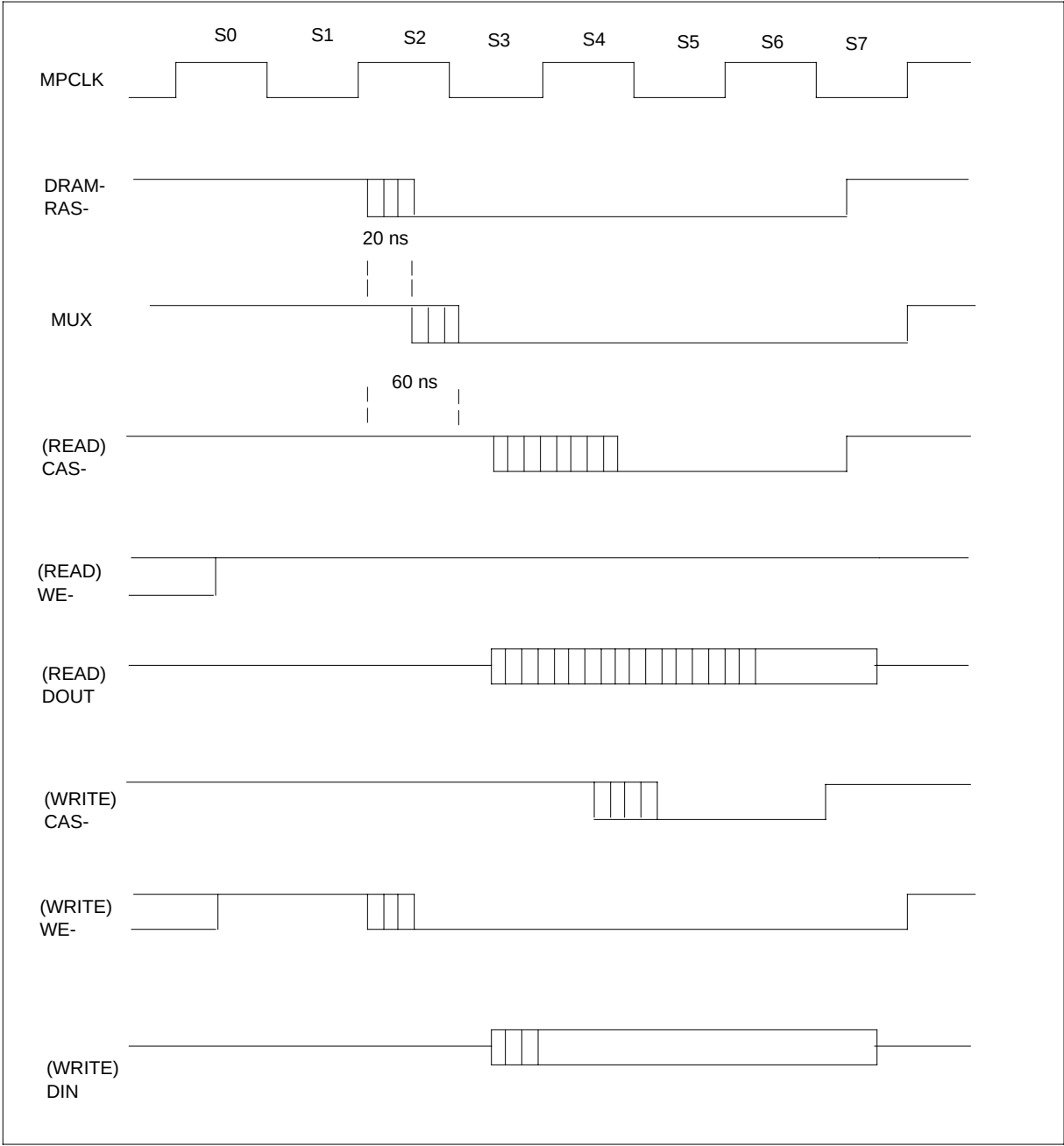
NTIX80BA DRAM access control timing
