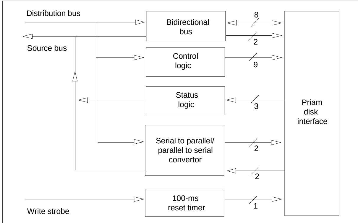
NT1X55FA functional blocks for the disk interface
