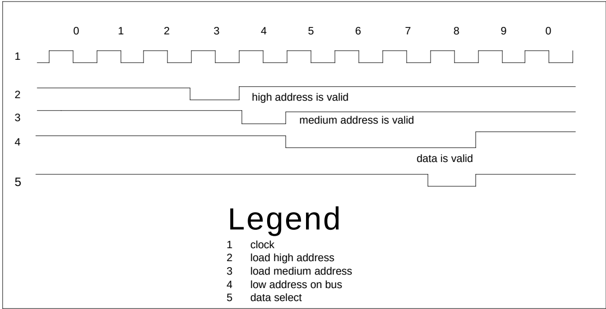
NT1X76AB timing
