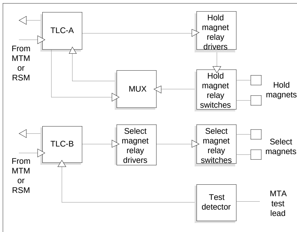
NT2X50AB functional blocks
