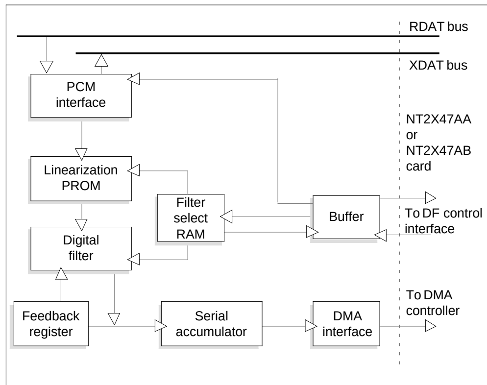
NT2X56AA functional blocks
