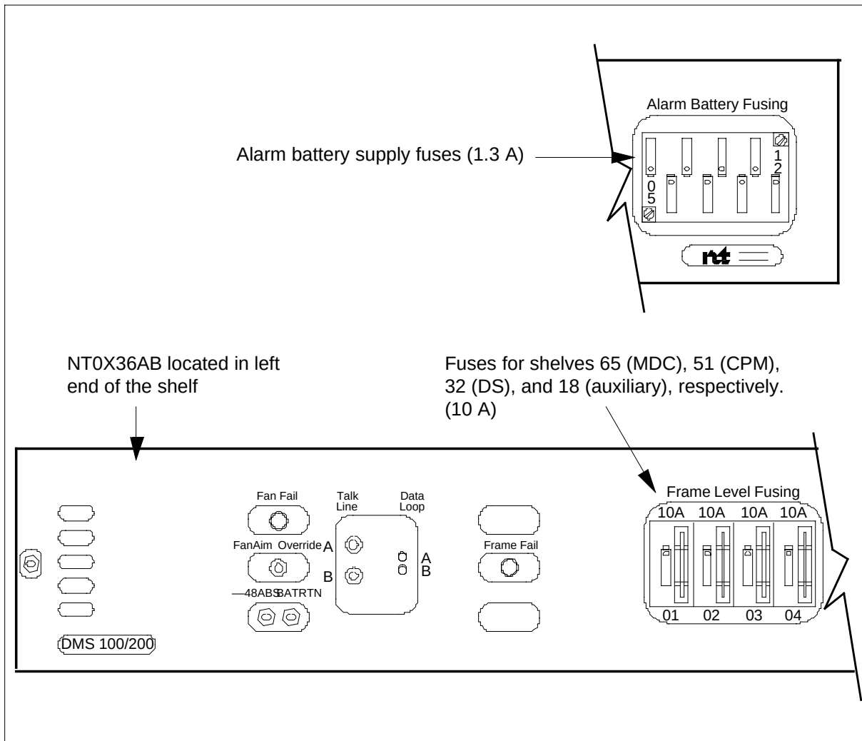
NT0X28AF front view
