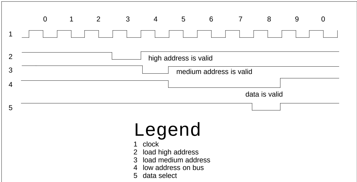
NT1X76AE timing
