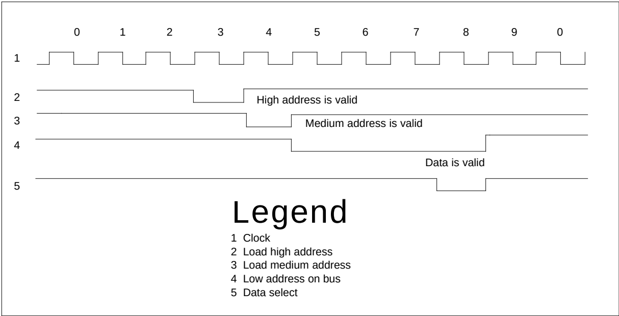
NT1X76JB timing
