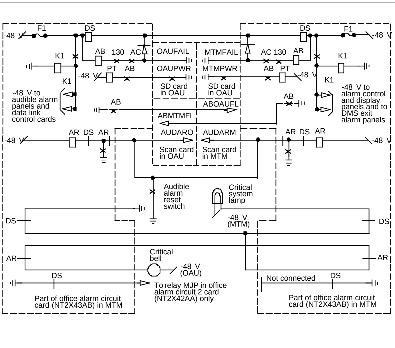
NT2X43 functional blocks for part of office alarm circuit 3 card (OAU and MTM)
