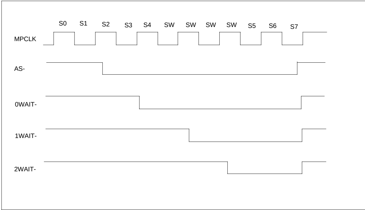
NTIX80BA WAIT clock timing
