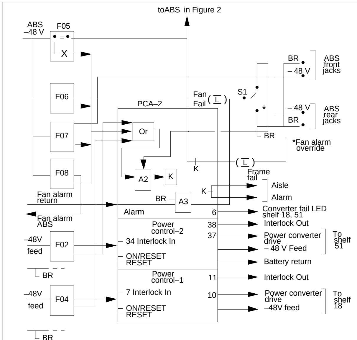
NT0X28AF simplified block diagram
