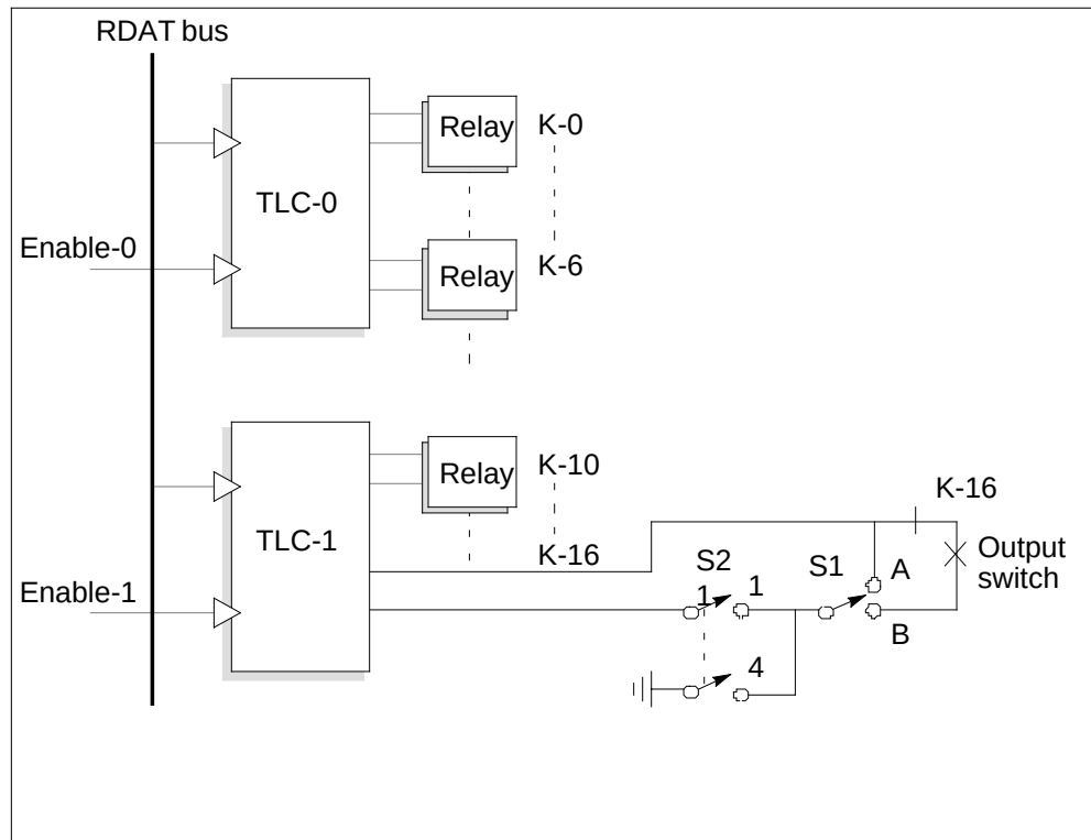
Figure NT2X57AB functional blocks
