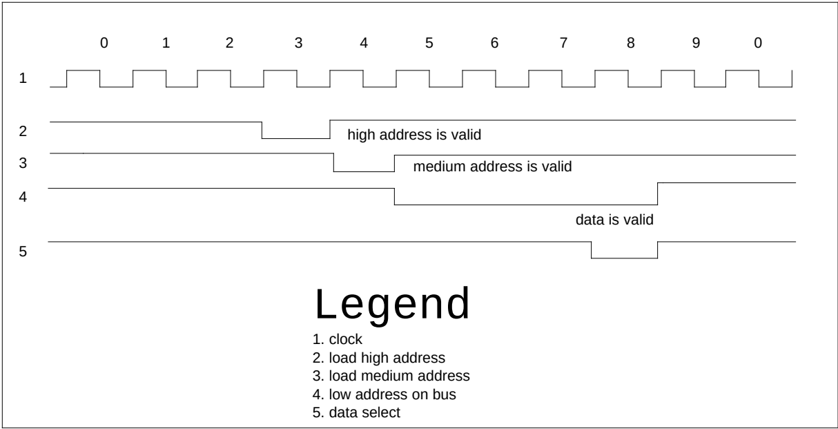
NT1X76BW timing
