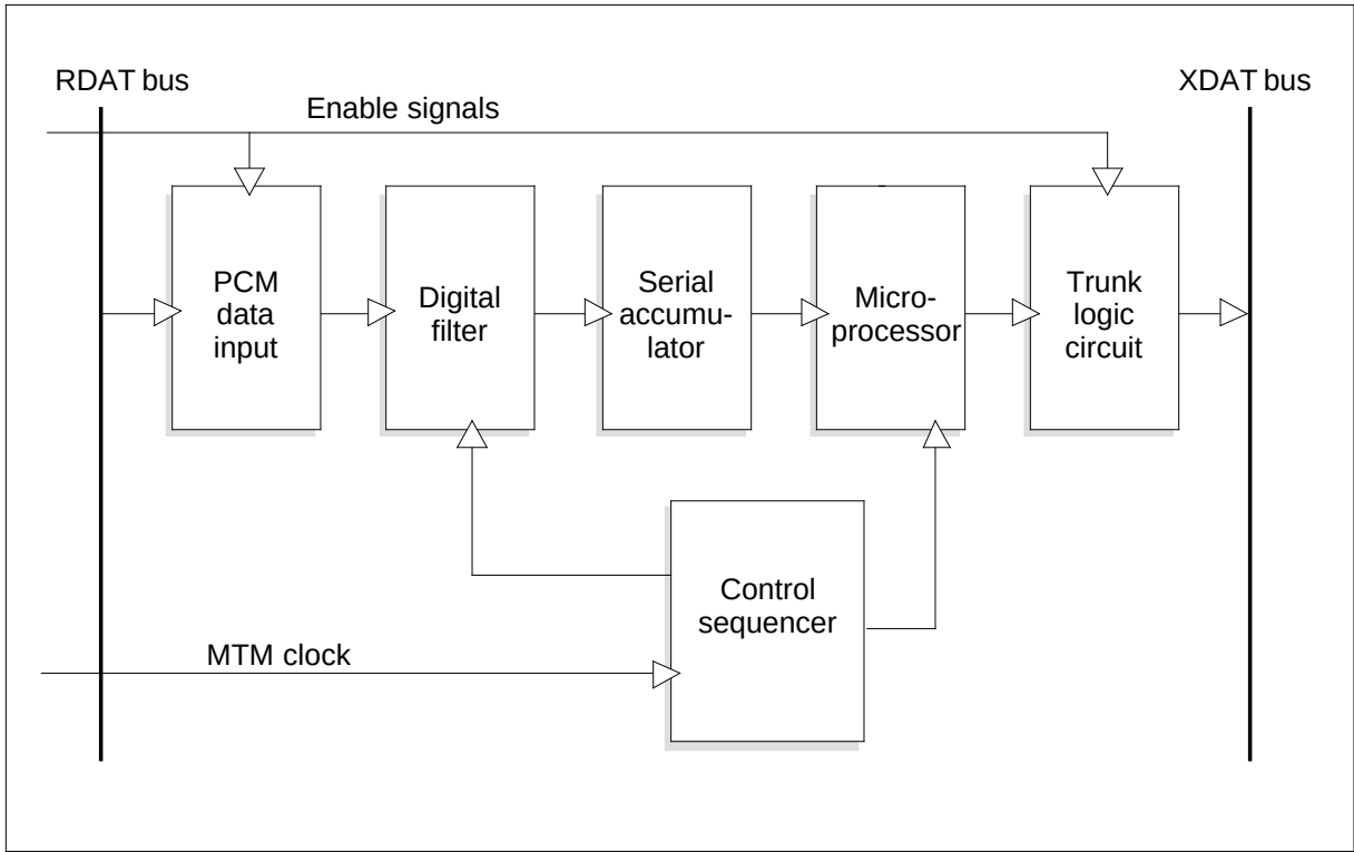
NT2X48BA functional blocks
