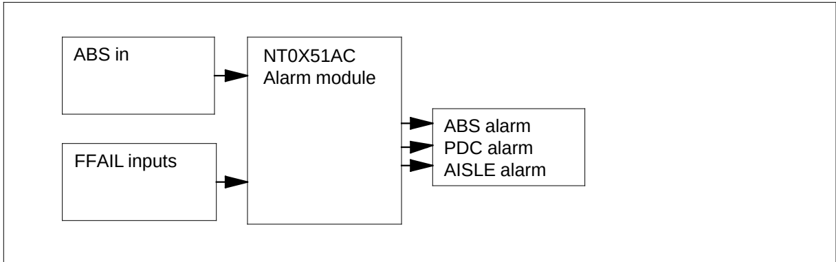
NT0X51AC functional blocks
