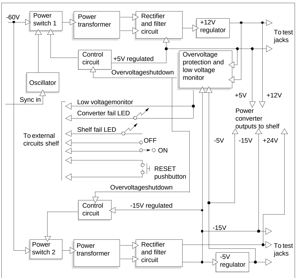
NT2X09KA functional blocks
