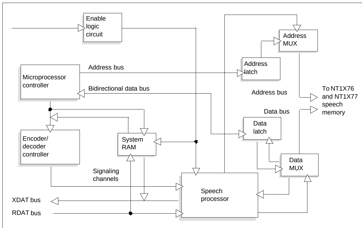
NT1X75AA functional blocks
