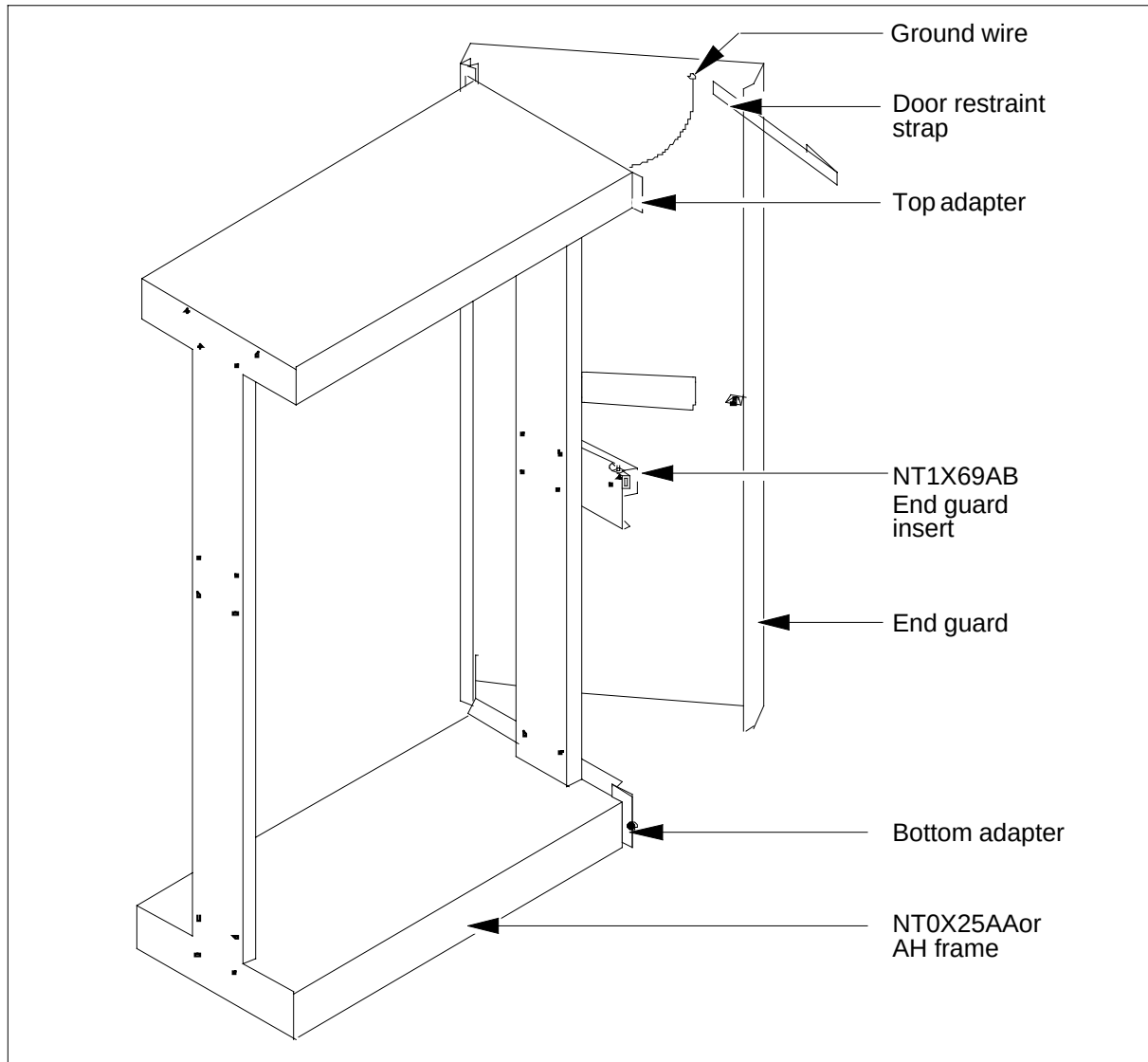
Typical diagonal view of NT0X73AJ end guard kit (installed)
