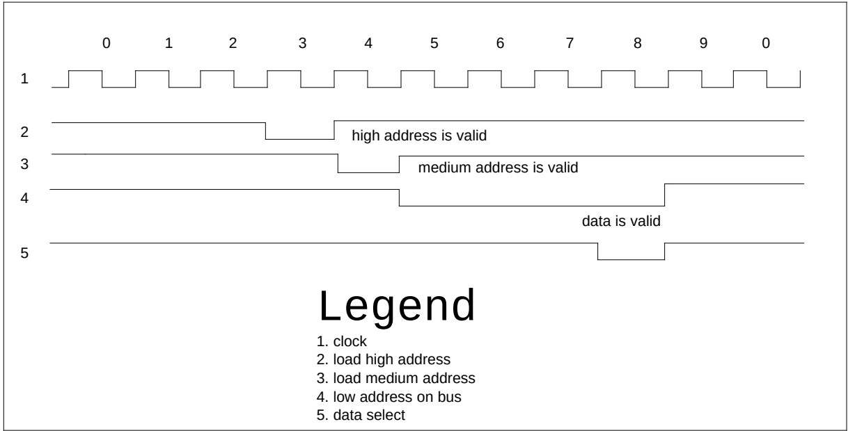
NT1X76BU timing
