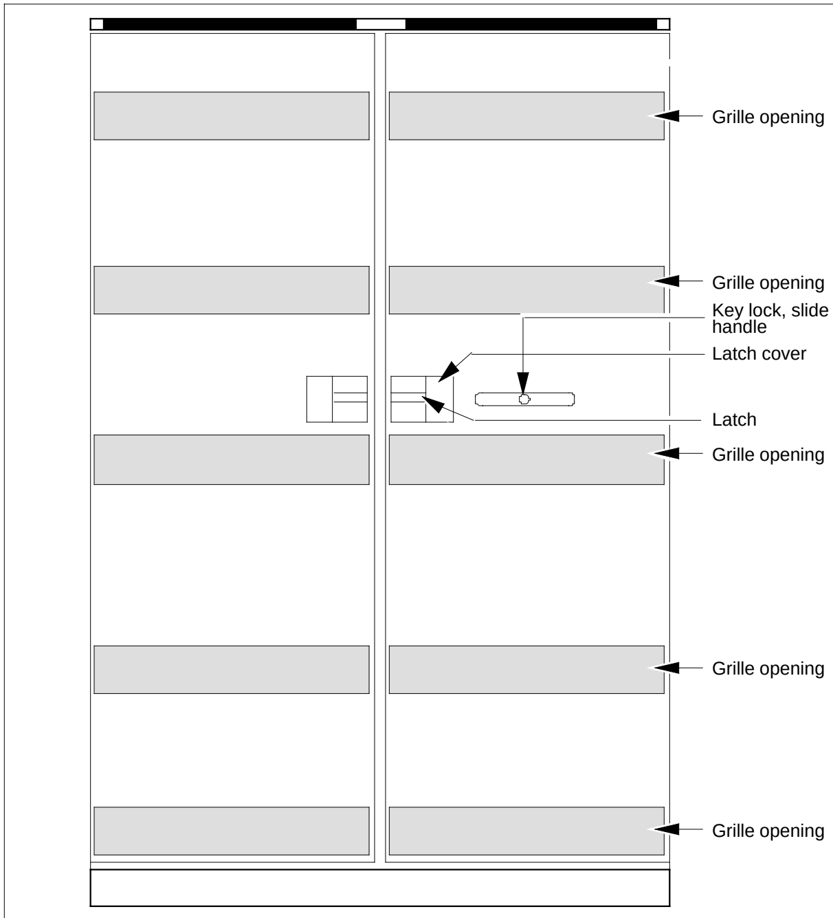
Normal rear view of NT0X71CA door kit
