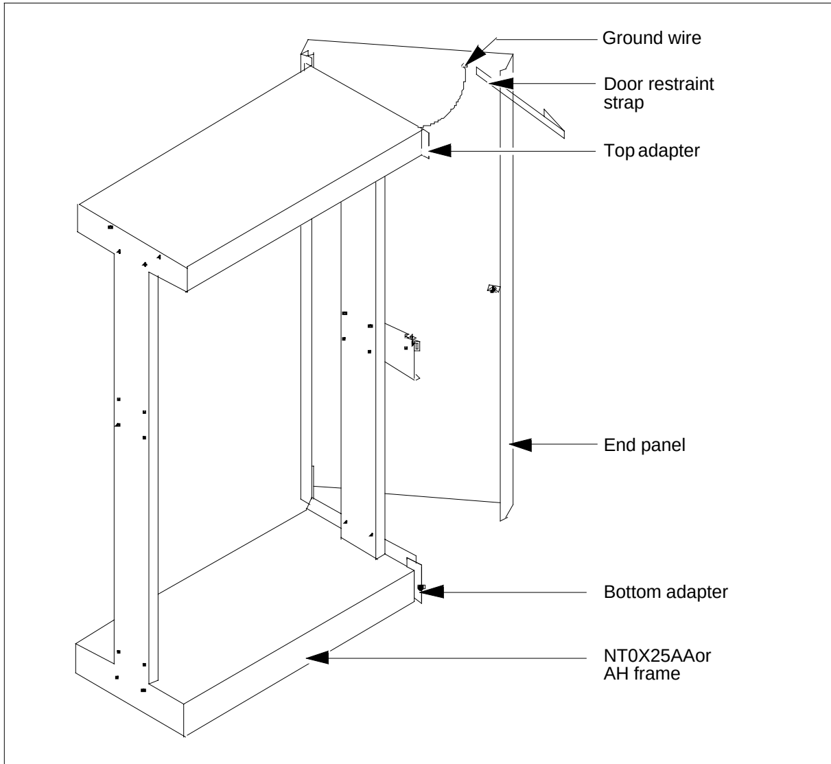
Typical diagonal view of NT0X73AK end panel kit (installed)
