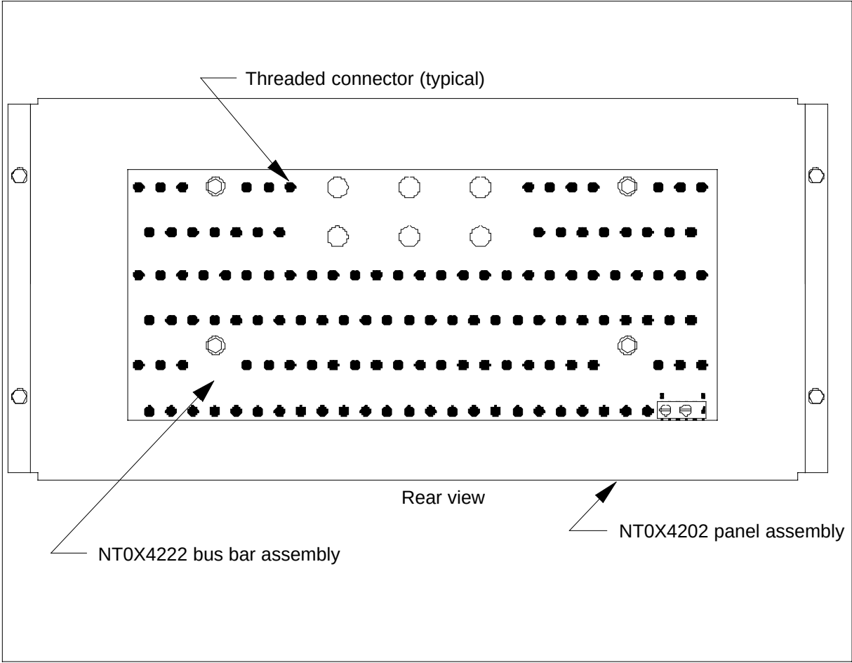
NT0X42AE rear view
