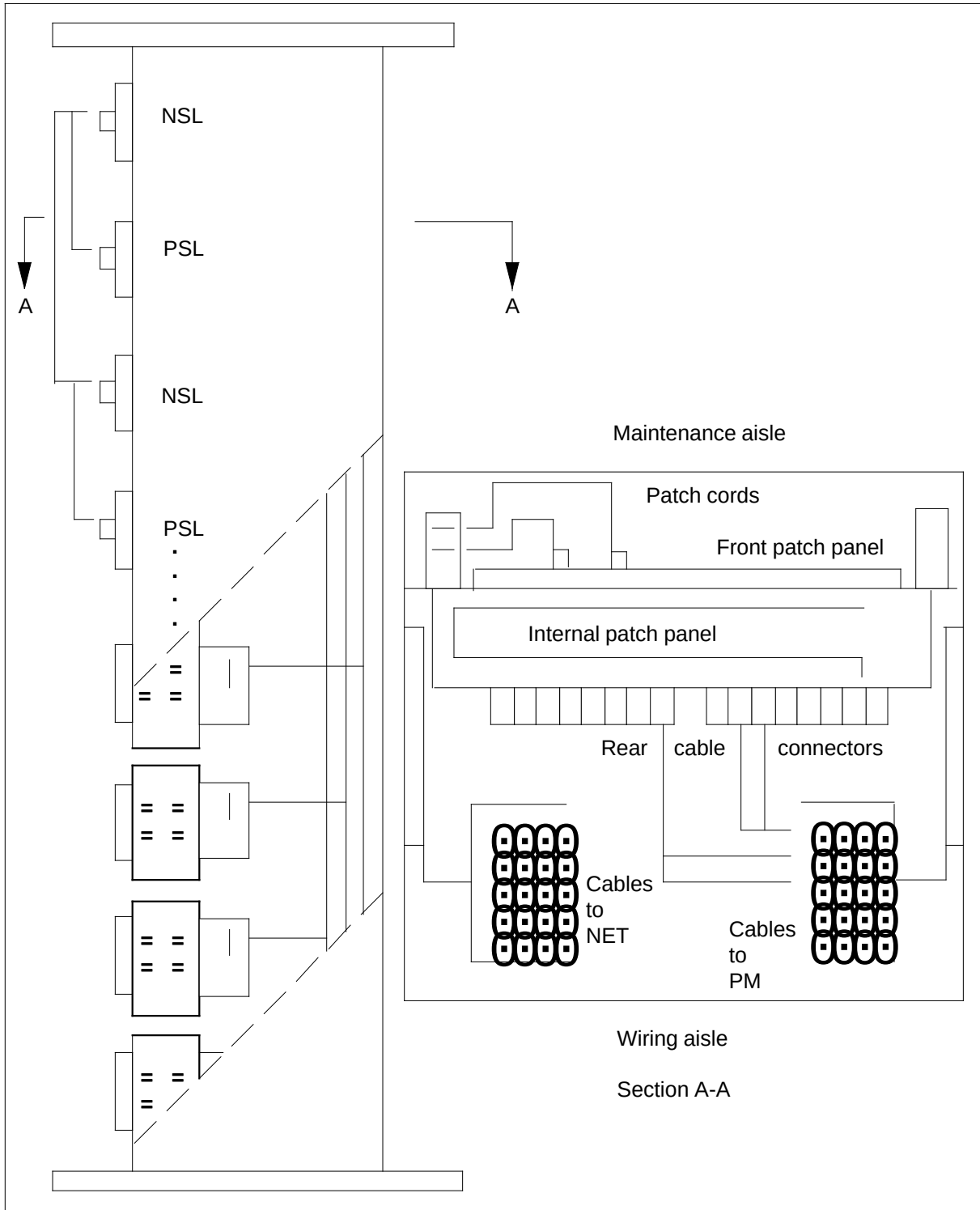
NT0X56 typical SLC frame, side view
