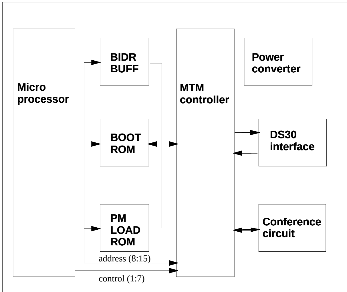
NT1X81BA functional blocks
