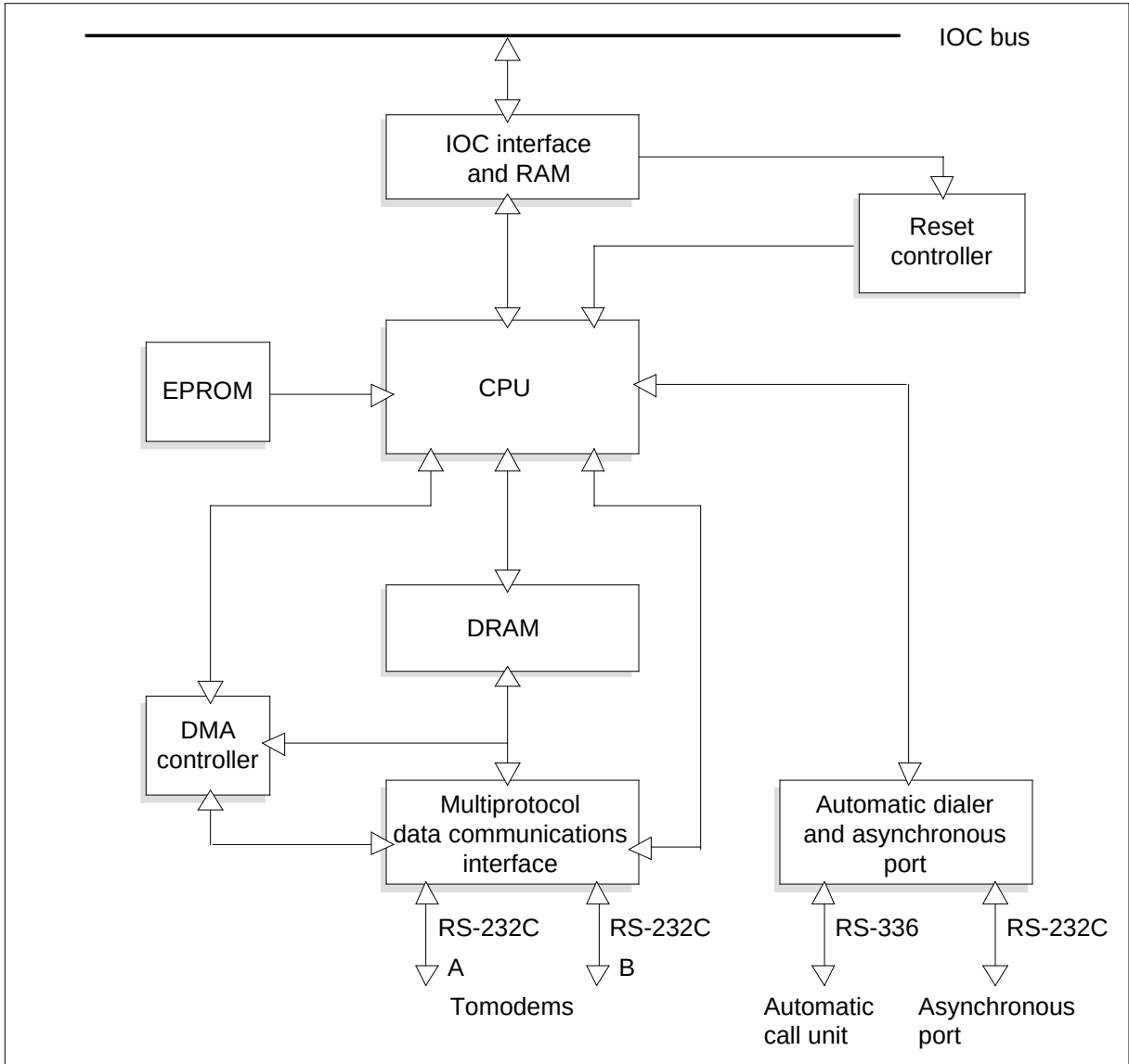
NT1X89AA functional blocks
