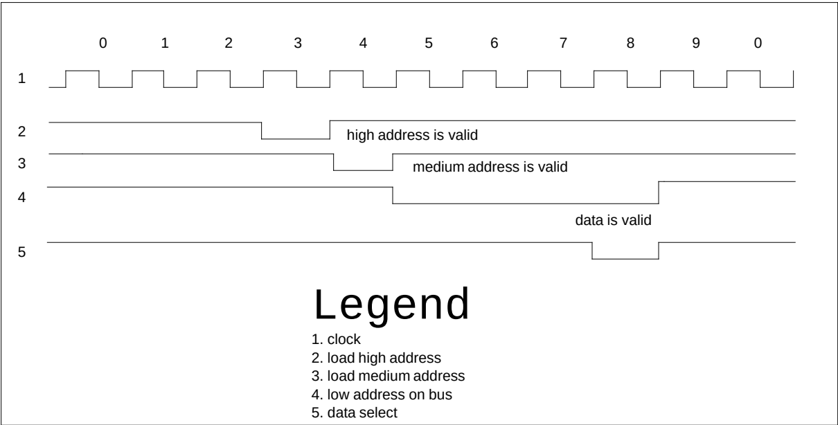
NT1X76GH timing
