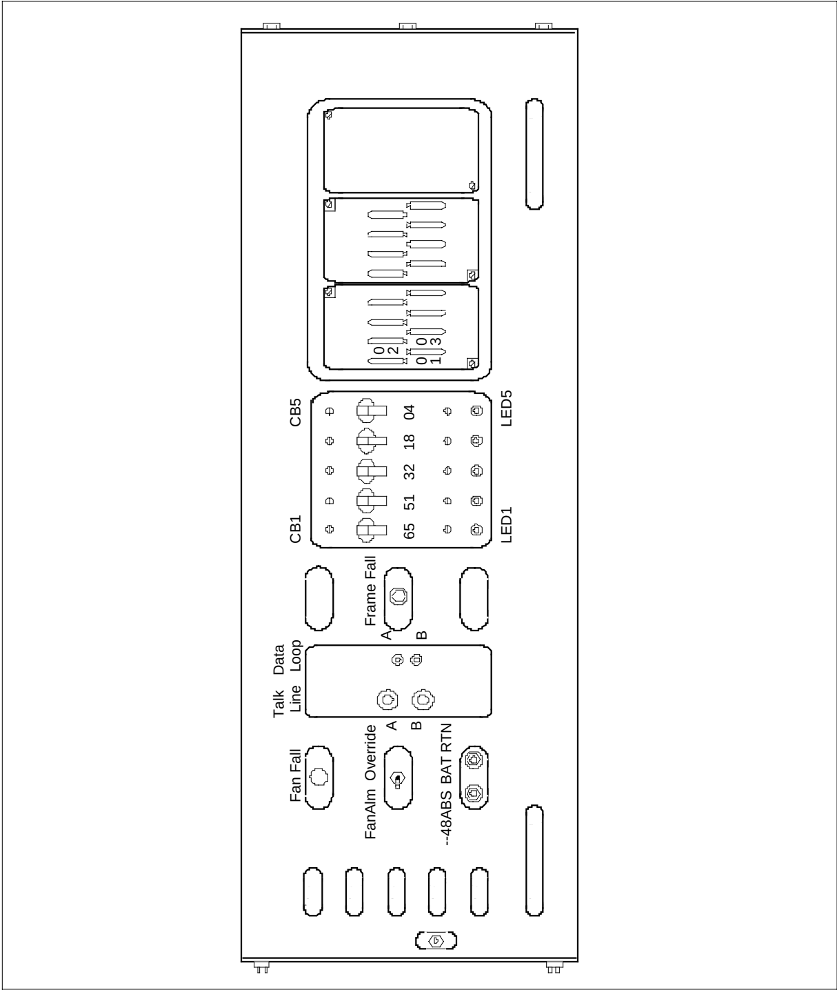
NT0X28AM front view
