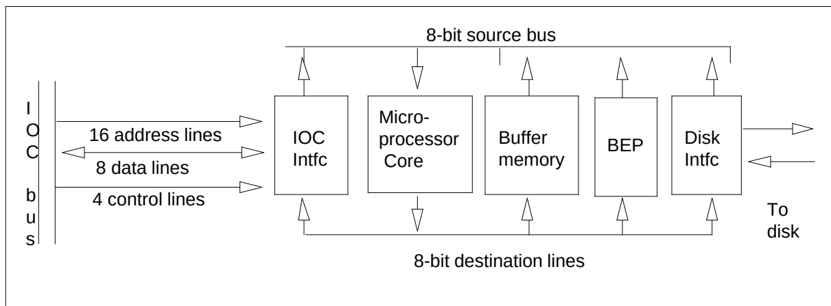
NT1X55 functional blocks for the disk controller
