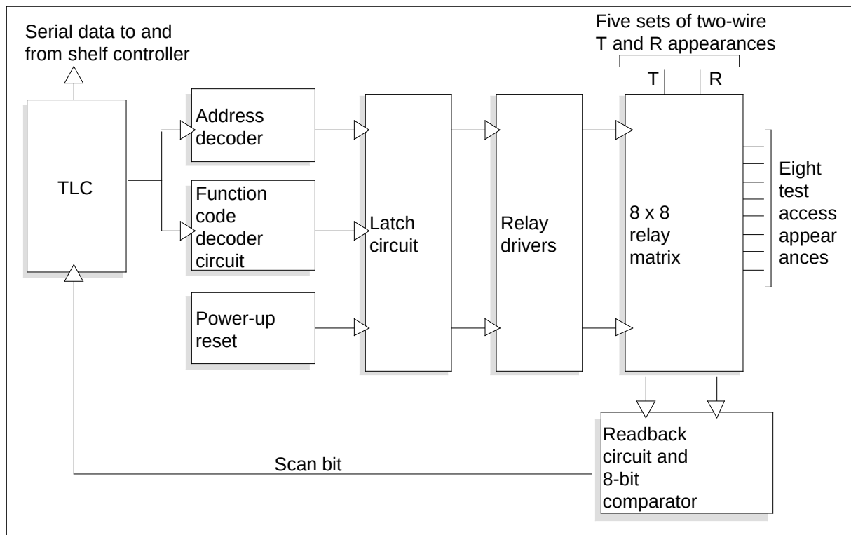
NT3X09BA functional blocks
