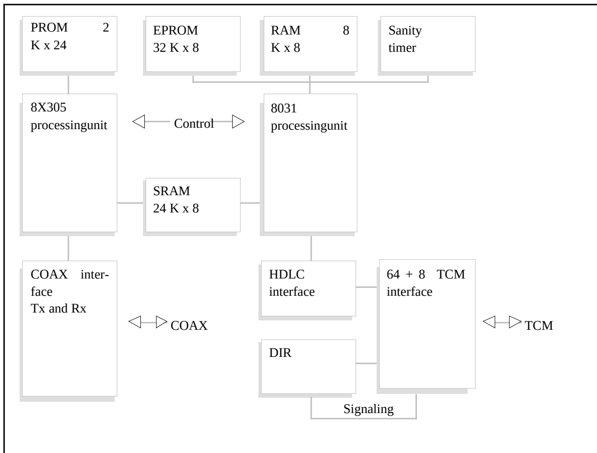
NT4X25DA functional blocks
