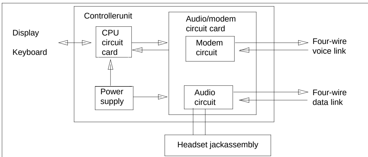
NT4X70 functional blocks
