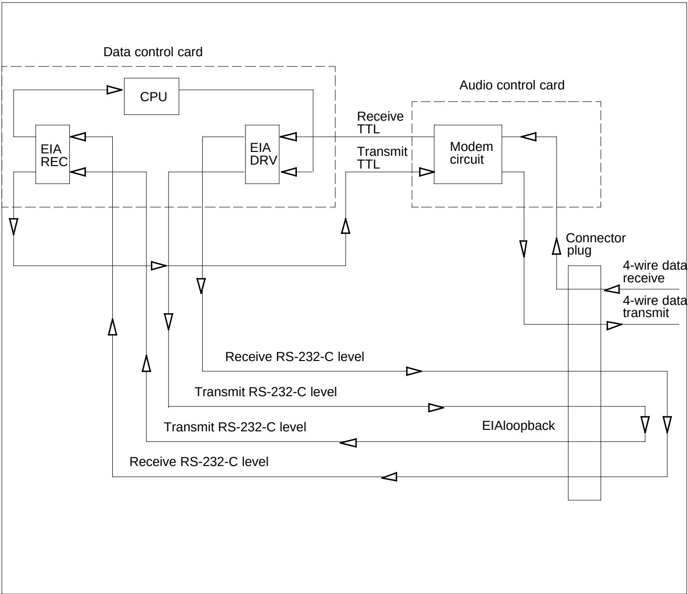
NT4X71 Data path between audio and data control cards
