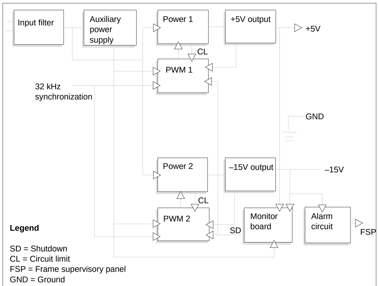
NT6X53EA functional blocks
