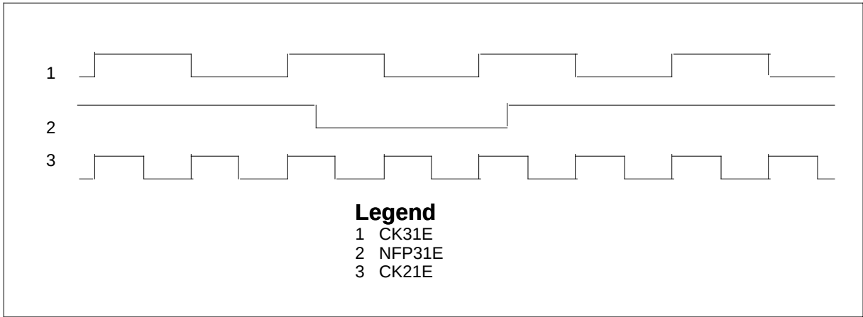
NT6X35BA frame pulse timing
