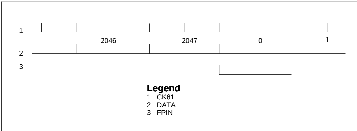
NT6X35BA V-bus timing
