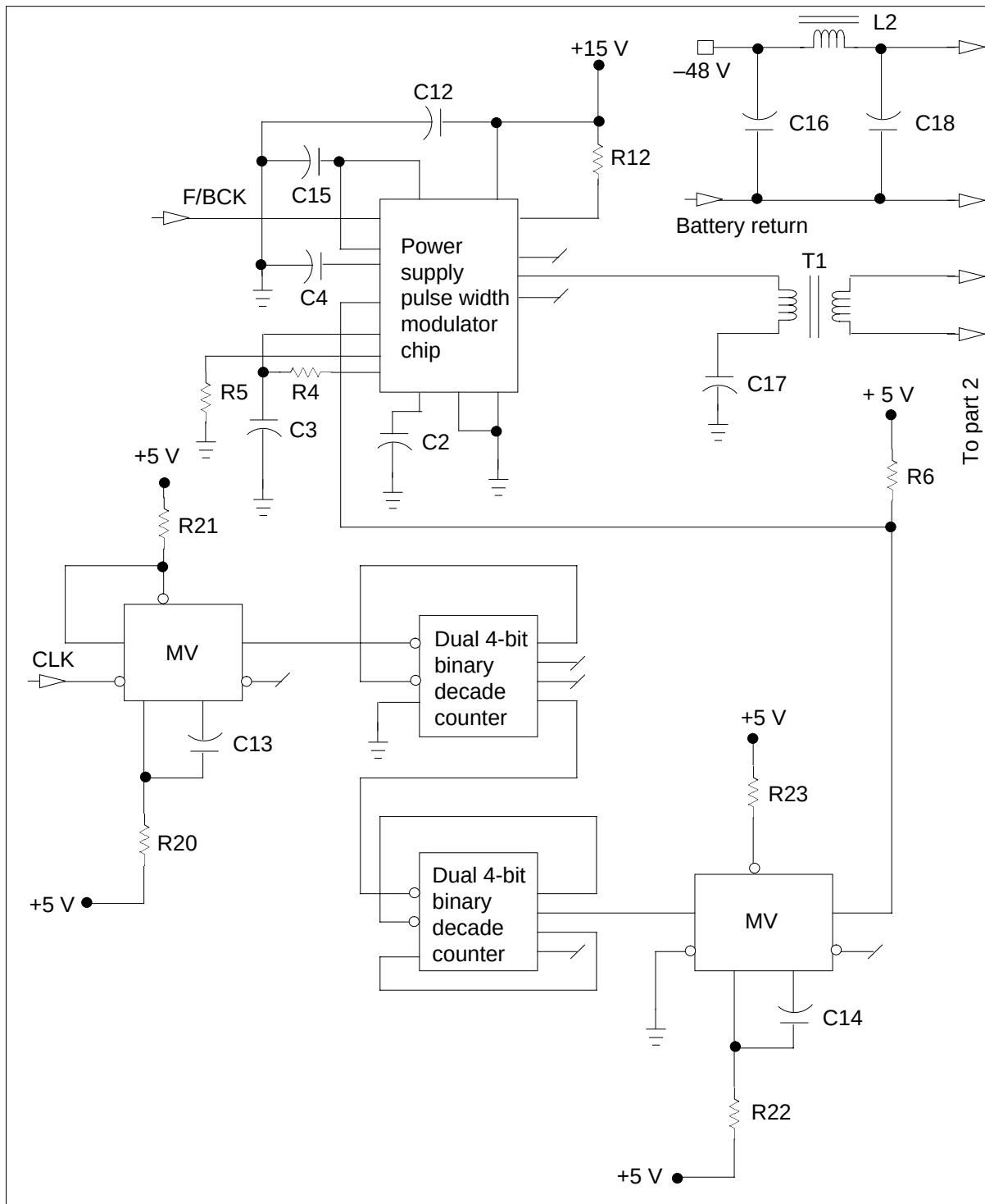
NT6X20AA circuit diagram (Part 1)
