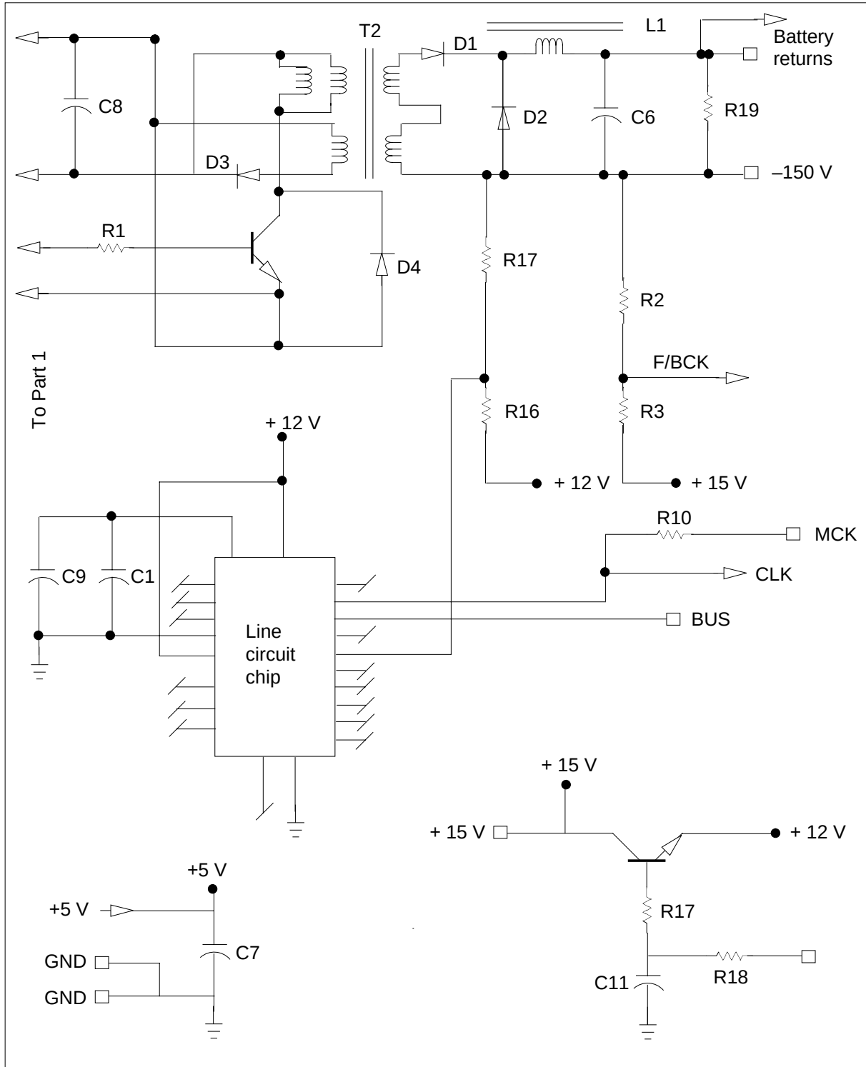
NT6X20AA circuit diagram (Part 2)
