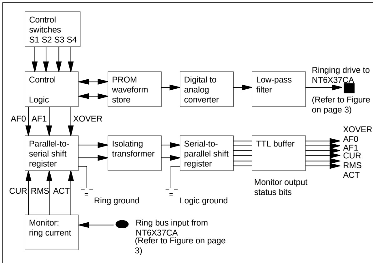
NT6X38BA Ringing control block diagram
