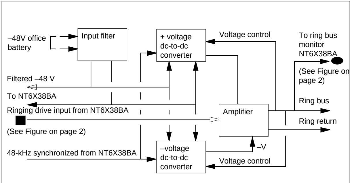
NT6X37CA Ringing amplifier block diagram
