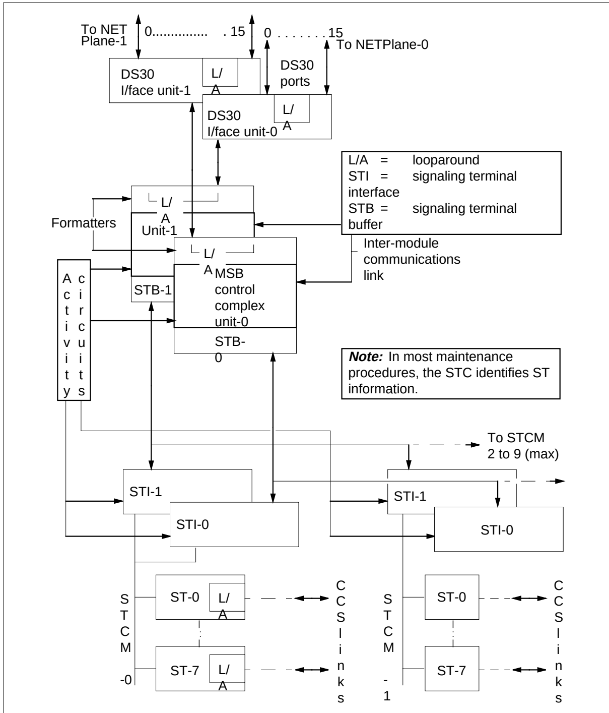
NT6X07AC simplified block diagram
