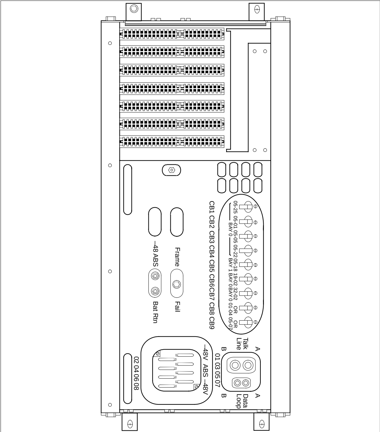
NT6X25BA front view
