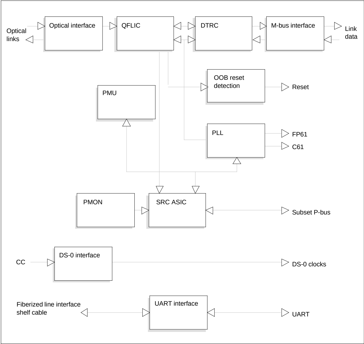
NT9X98AA functional blocks
