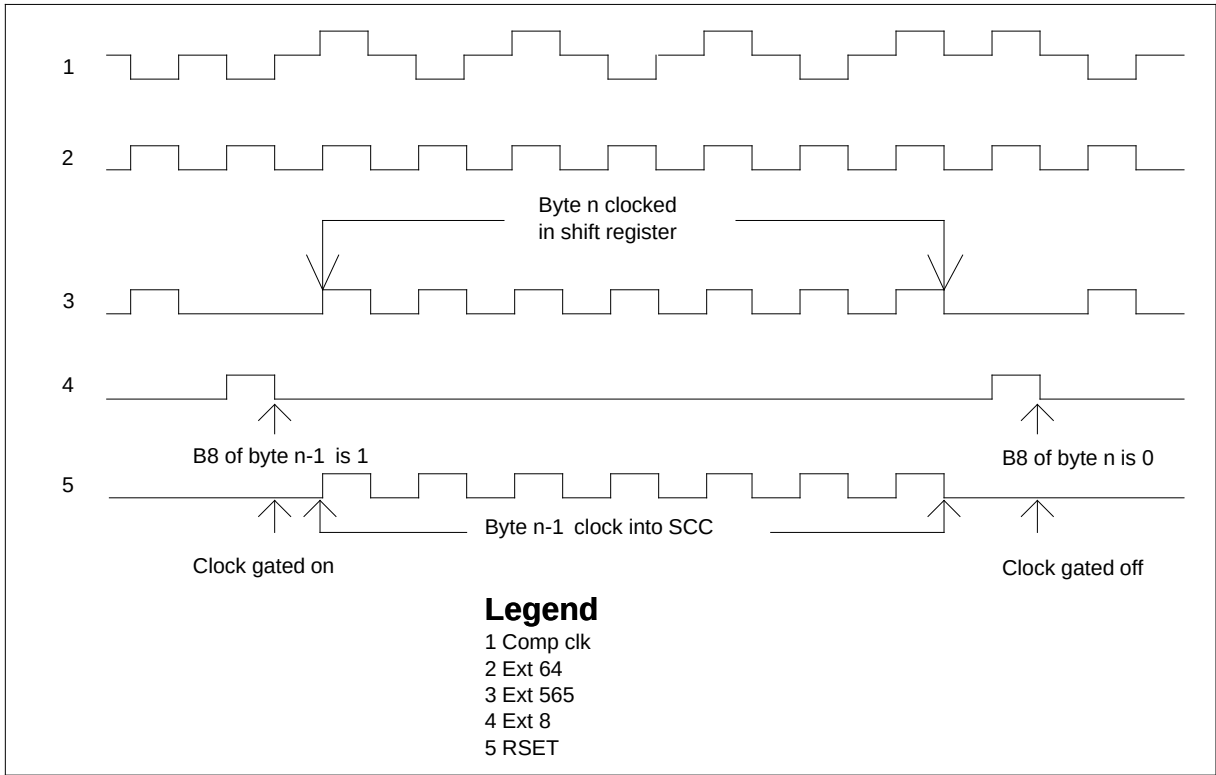
NT9X78CA timing
