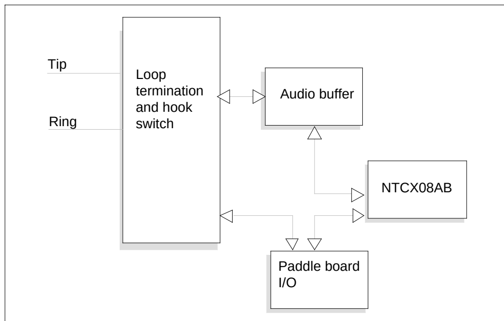
NTCX07AB functional blocks
