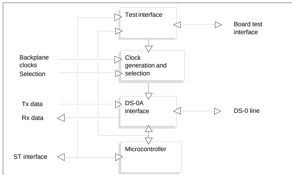
NT9X78CA functional blocks
