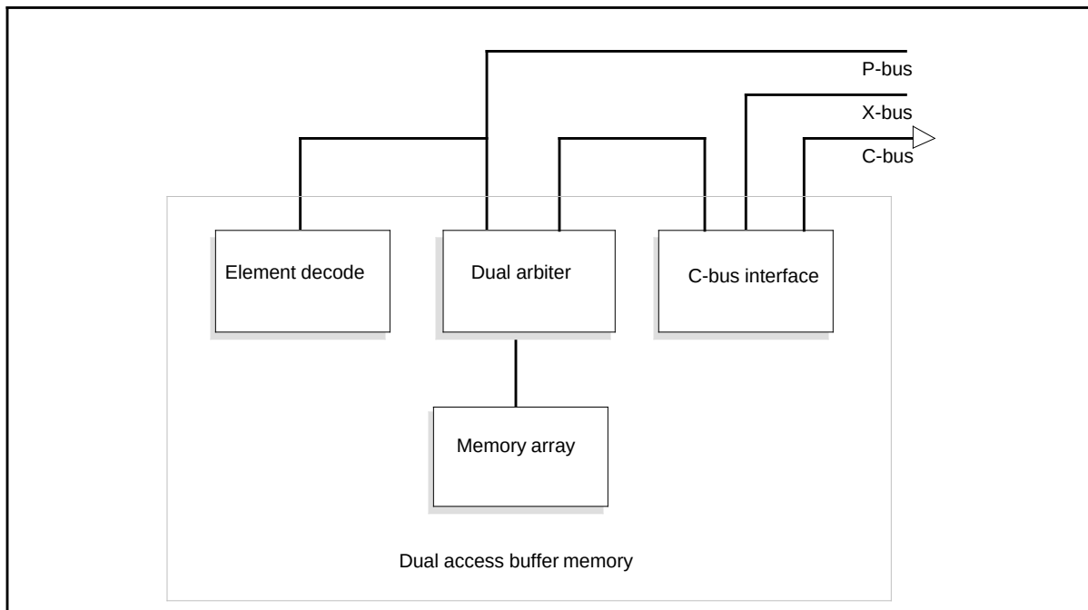
NT9X87AA functional blocks
