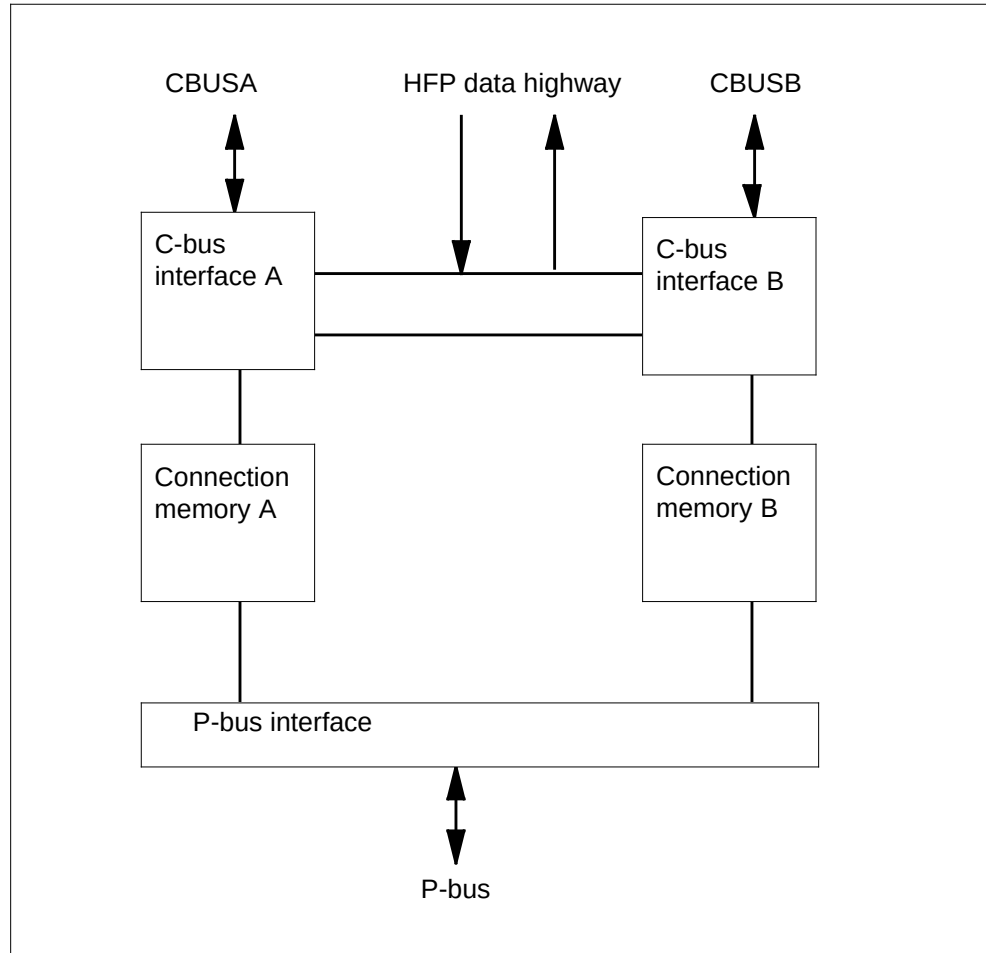
NTFX09AA functional blocks
