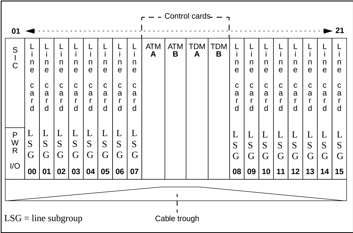
NTNP10BA: UE9000 DMS shelf assembly: front view
