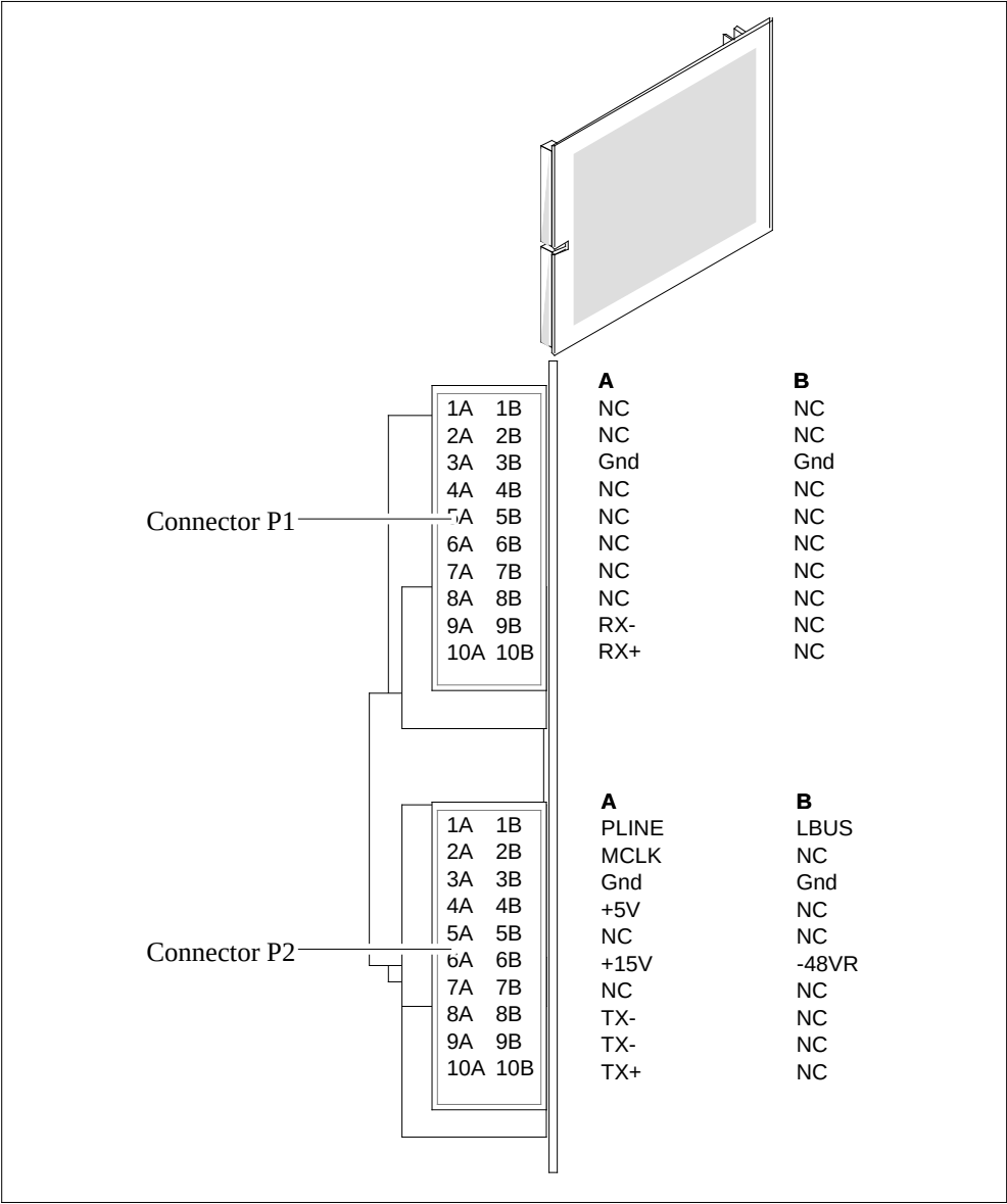
NTBX26AA pin numbers
