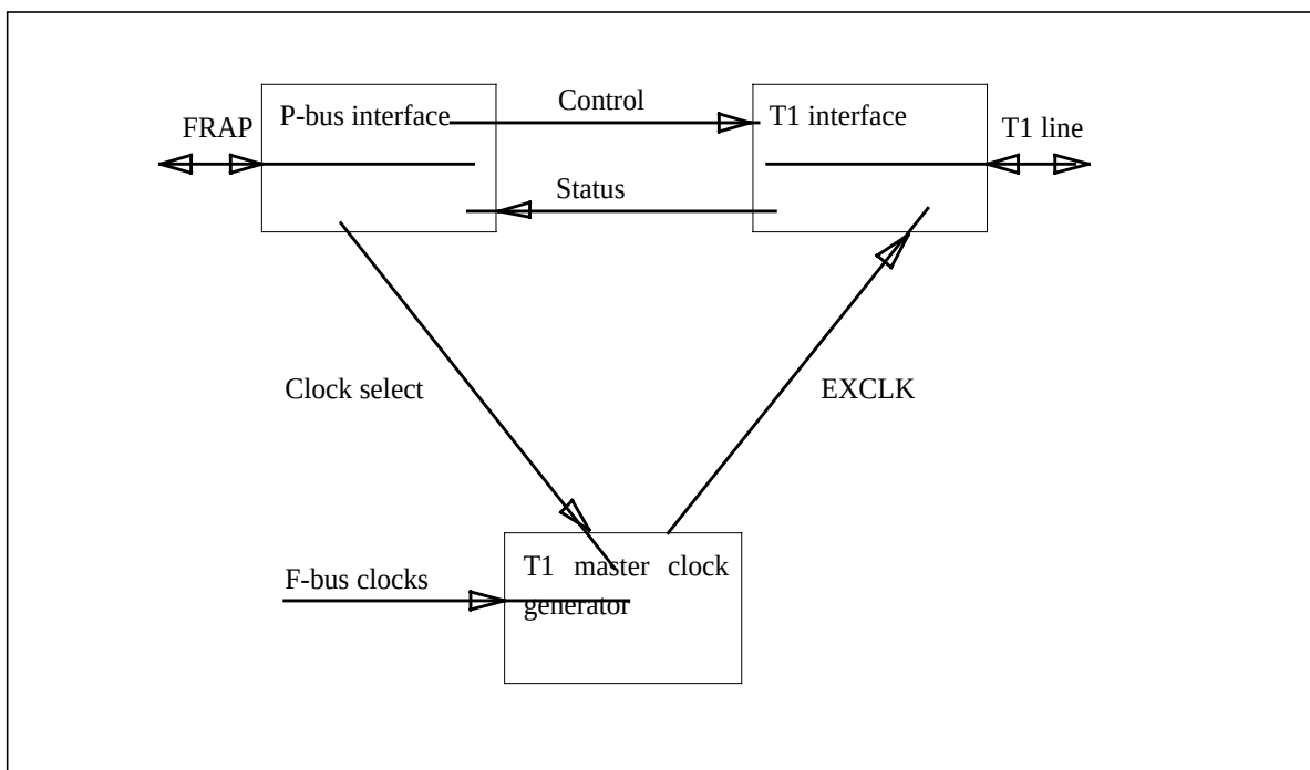
NTEX30AA functional blocks
