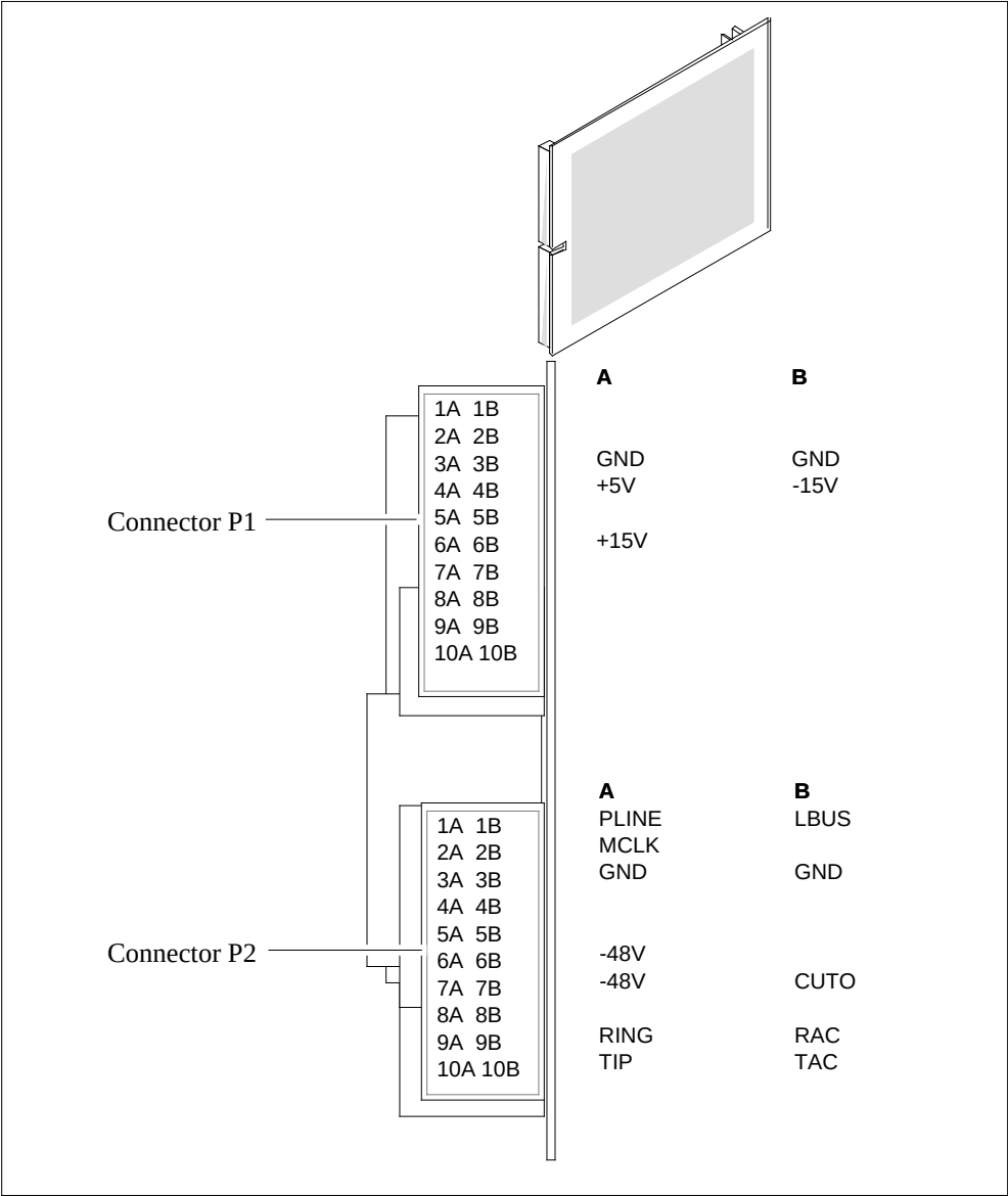
NTBX25AB pin numbers
