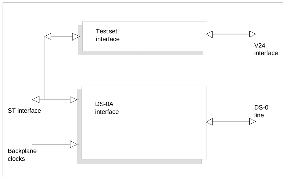
NT9X78AA functional blocks
