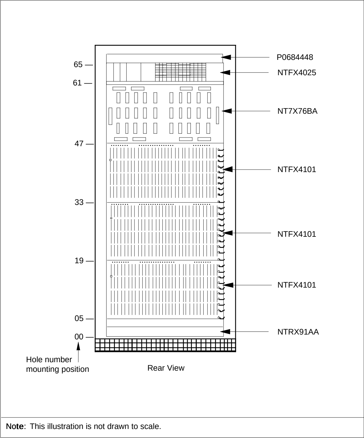
NTFX40EA CMTA rear view
