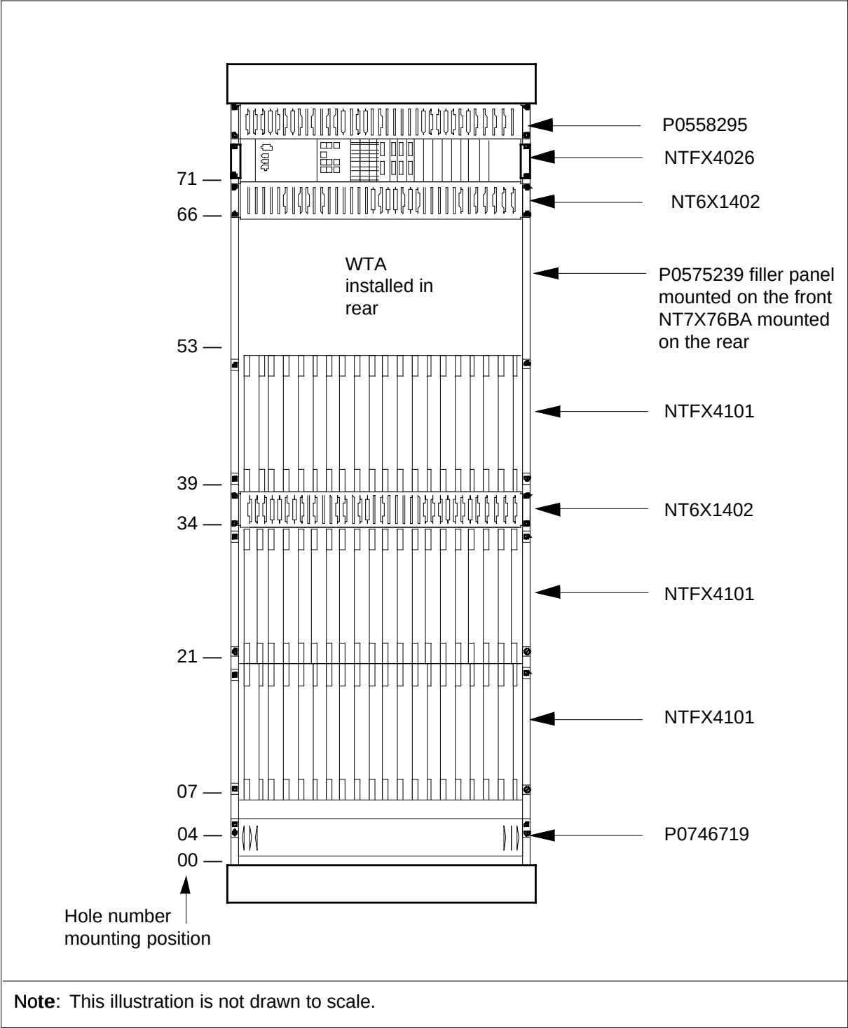
NTFX40FA MTAE front view
