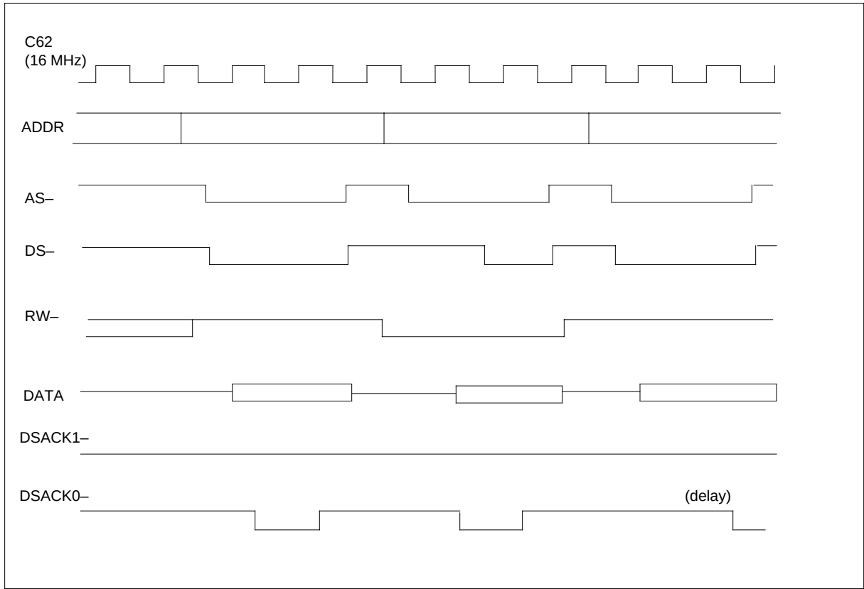
NTAX87AA CPU overall timing
