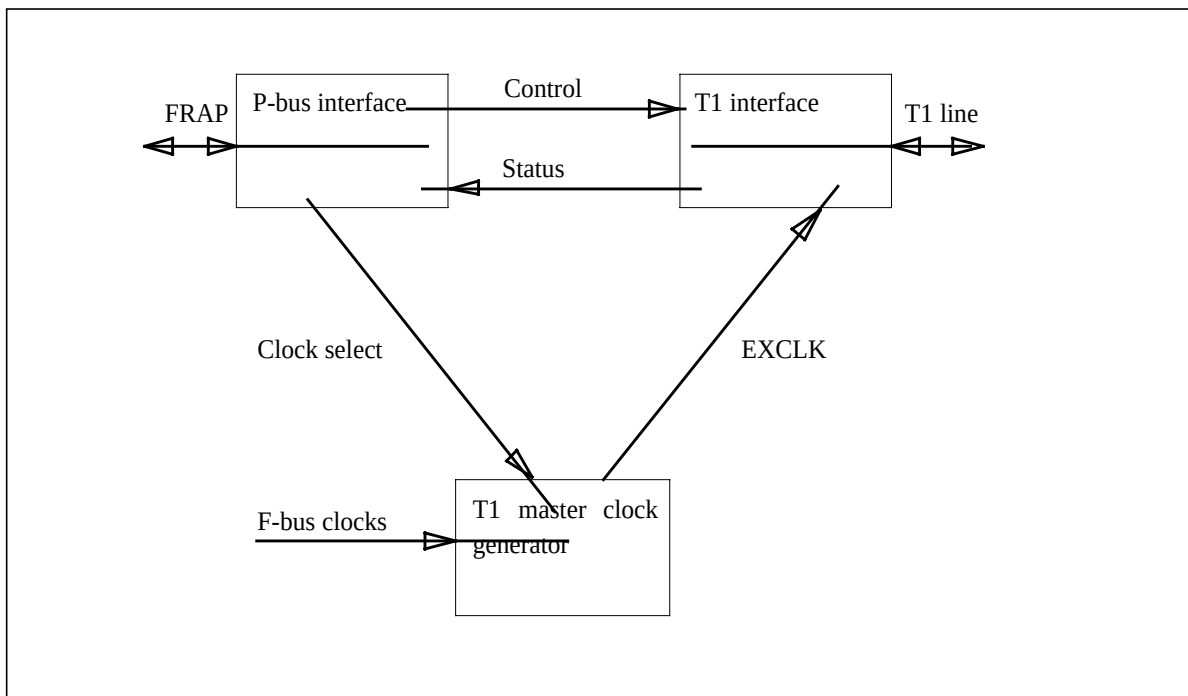
NTEX30AA functional blocks
