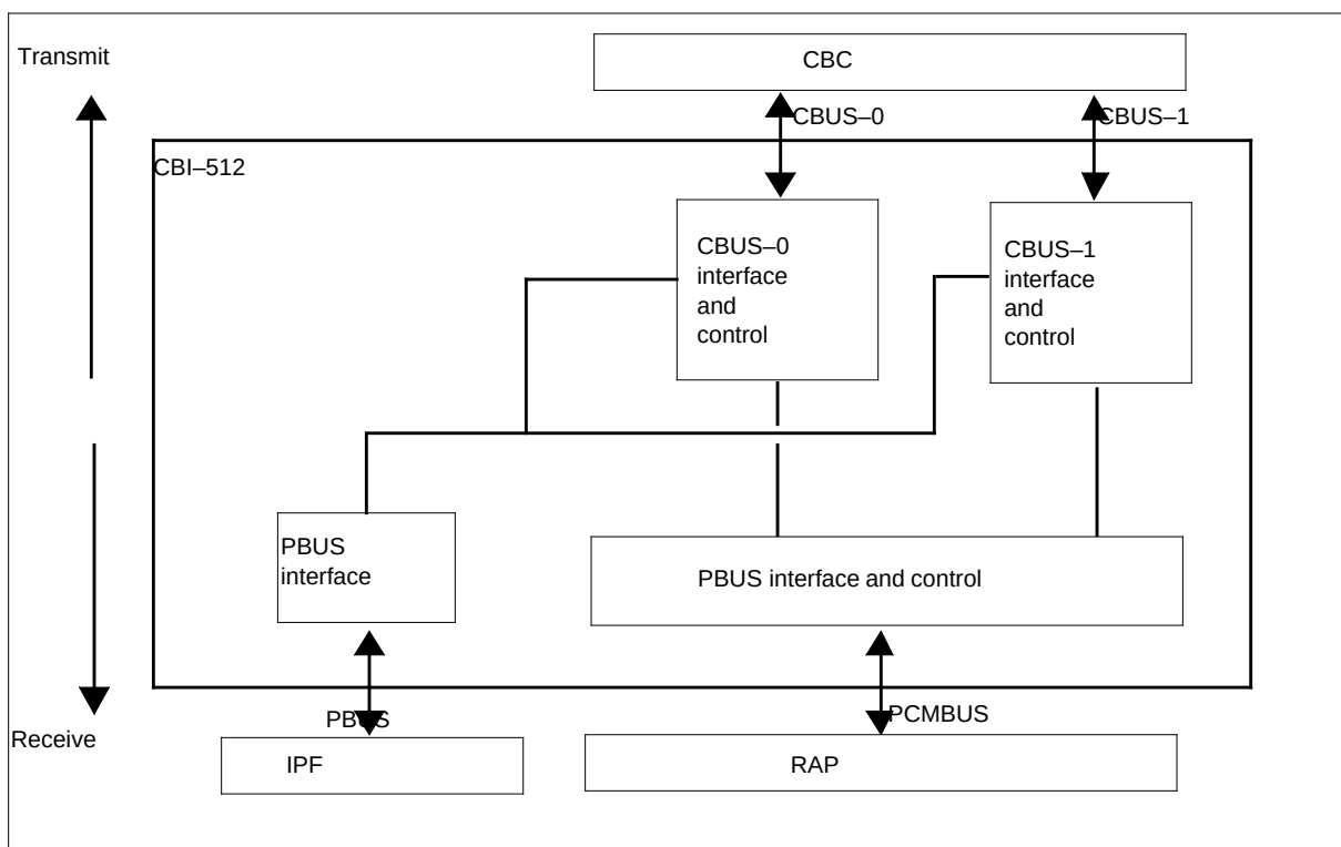
NTMX99AA functional blocks
