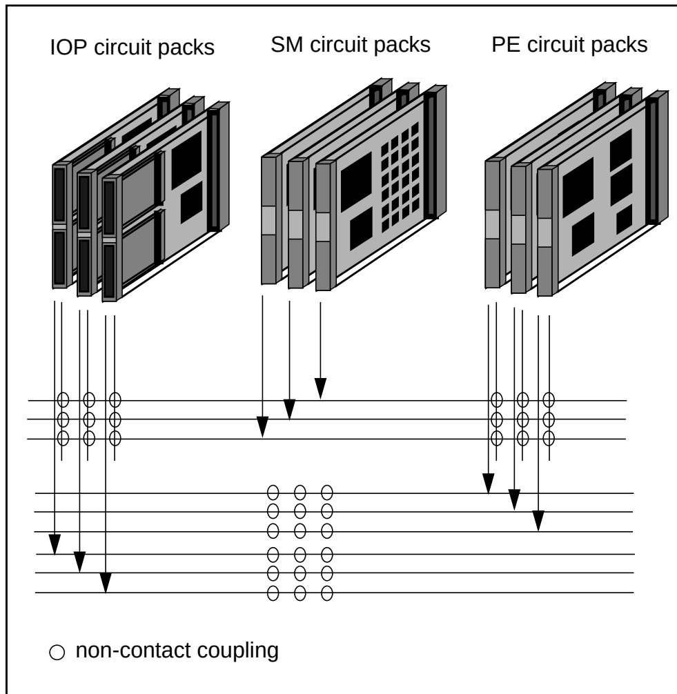
Figure 5-1 XA-Core multiprocessor architecture with XAI midplane
