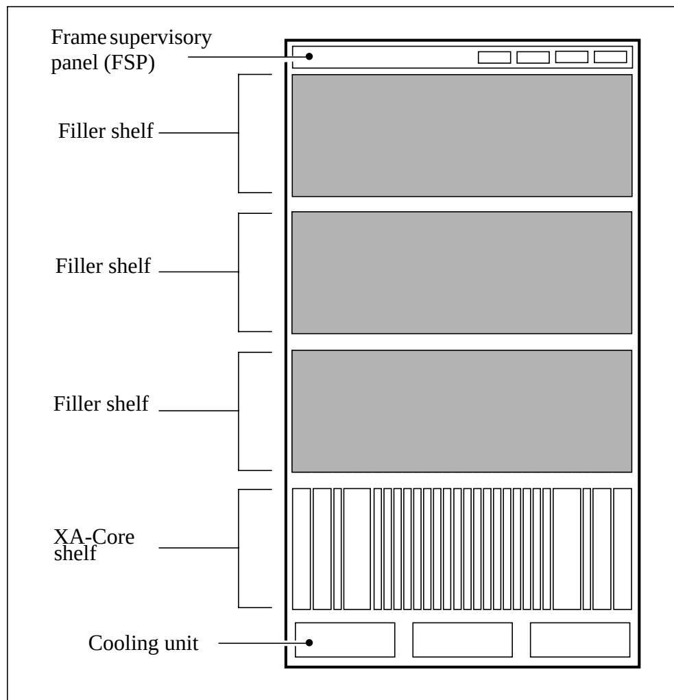
Figure 1-5 XA-Core in the extension cabinet layout
