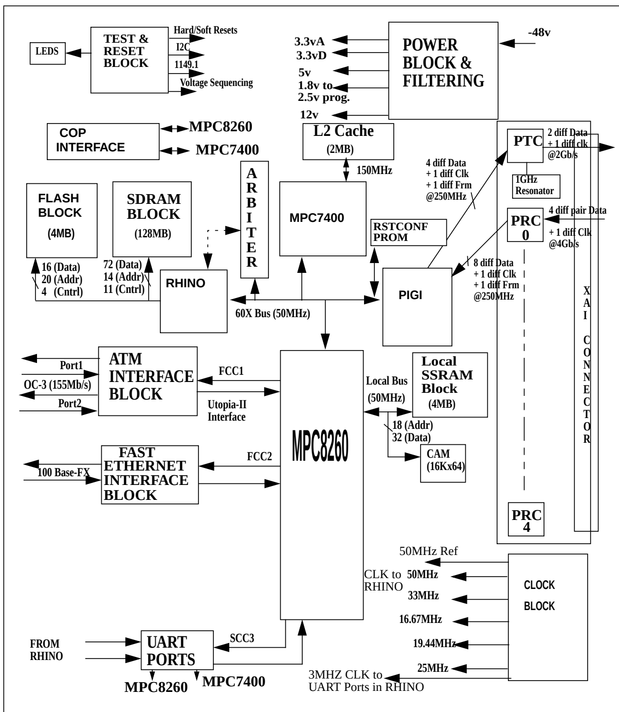
NTLX04 block diagram
