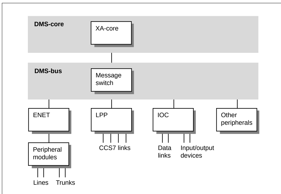
Figure 1-1 XA-Core in the architecture of the DMS SuperNode switch
