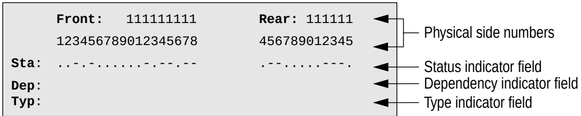
Figure 4-5 XA-Core MAP shelf layout area
