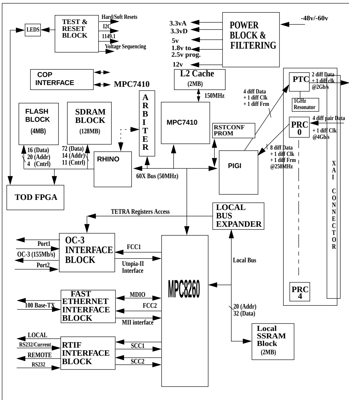
NTLX17 block diagram
