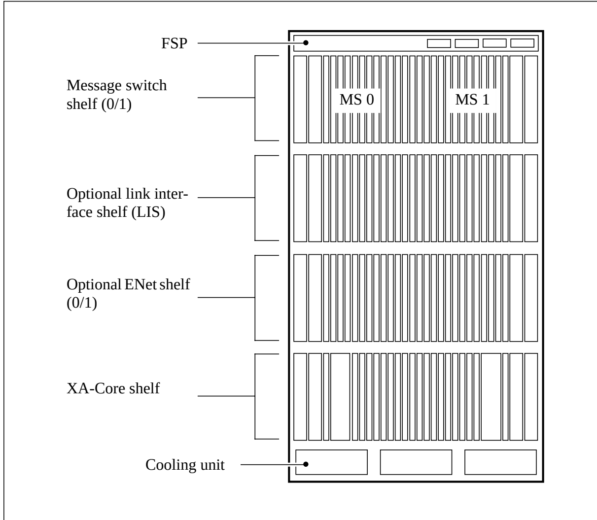
Figure 1-4 XA-Core in the SuperNode SE cabinet layout
