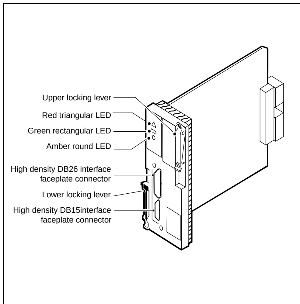
NTLX08 reset terminal interface
