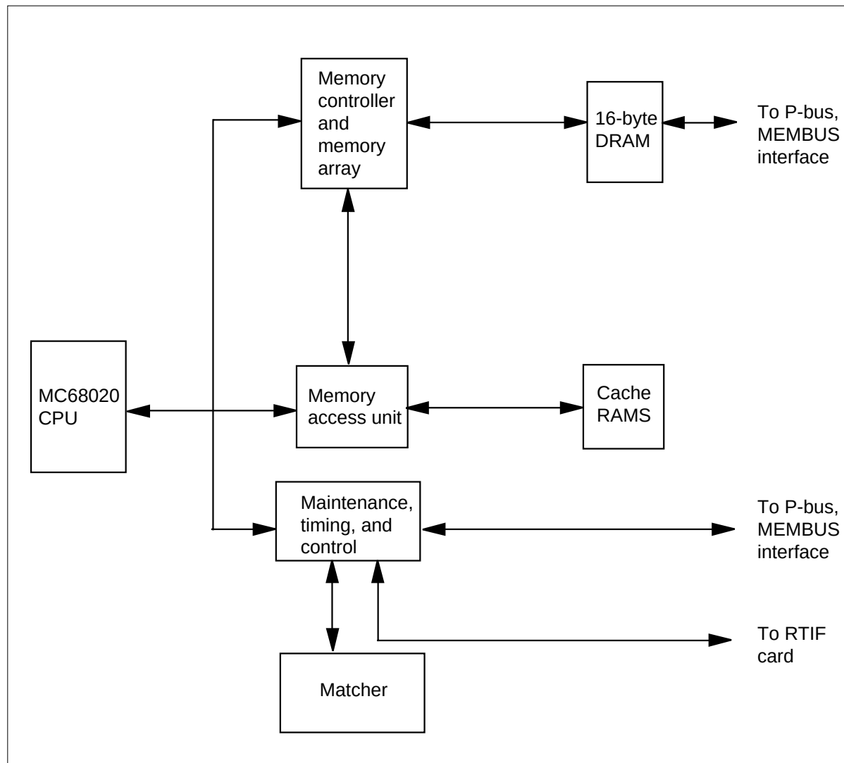
NT9X13NB functional blocks
