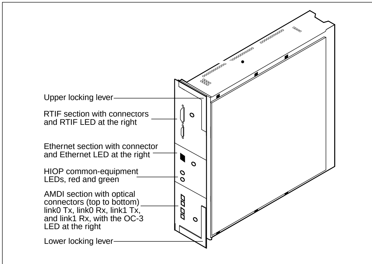
NTLX04 high performance input/output circuit pack front and side views
