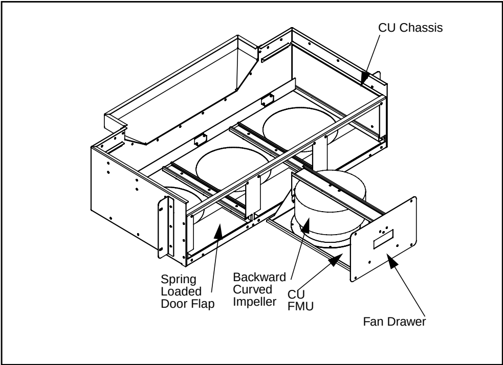
NTLX10AA XA-Core cooling unit assembly
