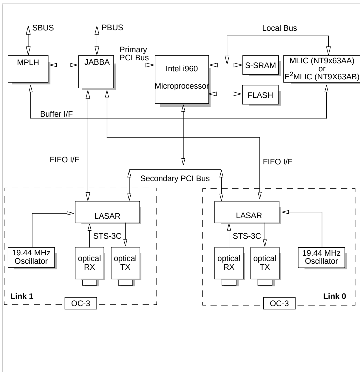
NT9X63AA/AB functional blocks
