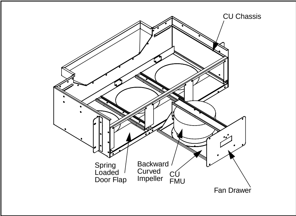
NTLX11AA XA-Core cooling unit fan drawer
