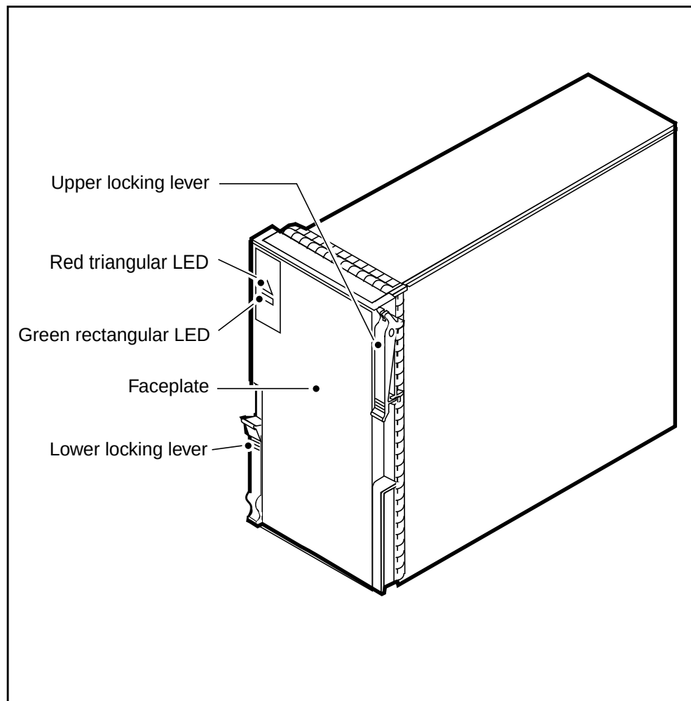
NTLX06 disk packlet
