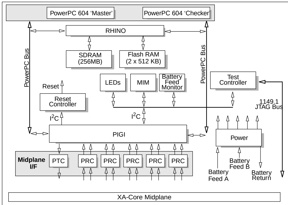
NTLX02CA functional blocks
