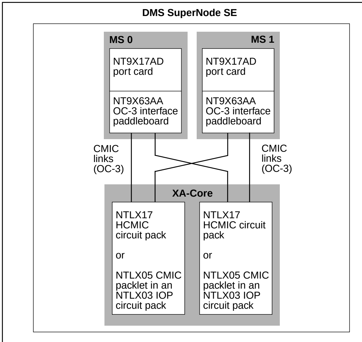
Figure 1-7 XA-Core to MS port connections for DMS SuperNode SE
