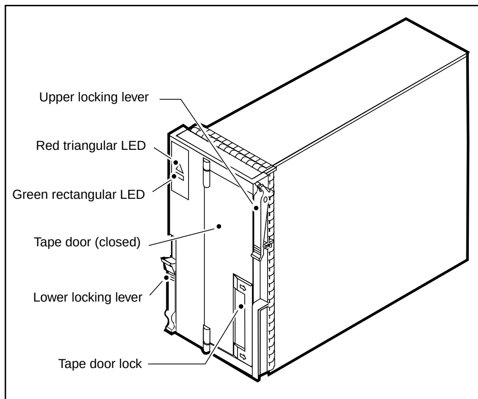
NTLX07 tape packlet
