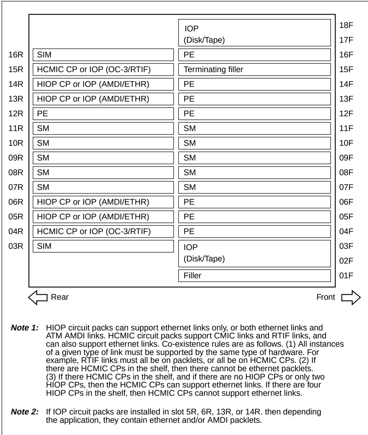
Figure 1-8 Example of XA-Core shelf layout
