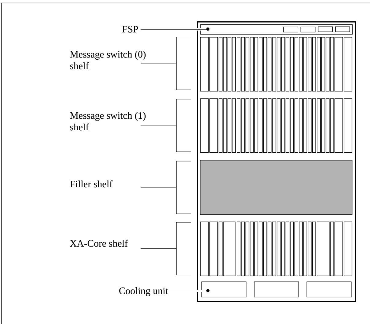
Figure 1-3 XA-Core in the SuperNode cabinet layout
