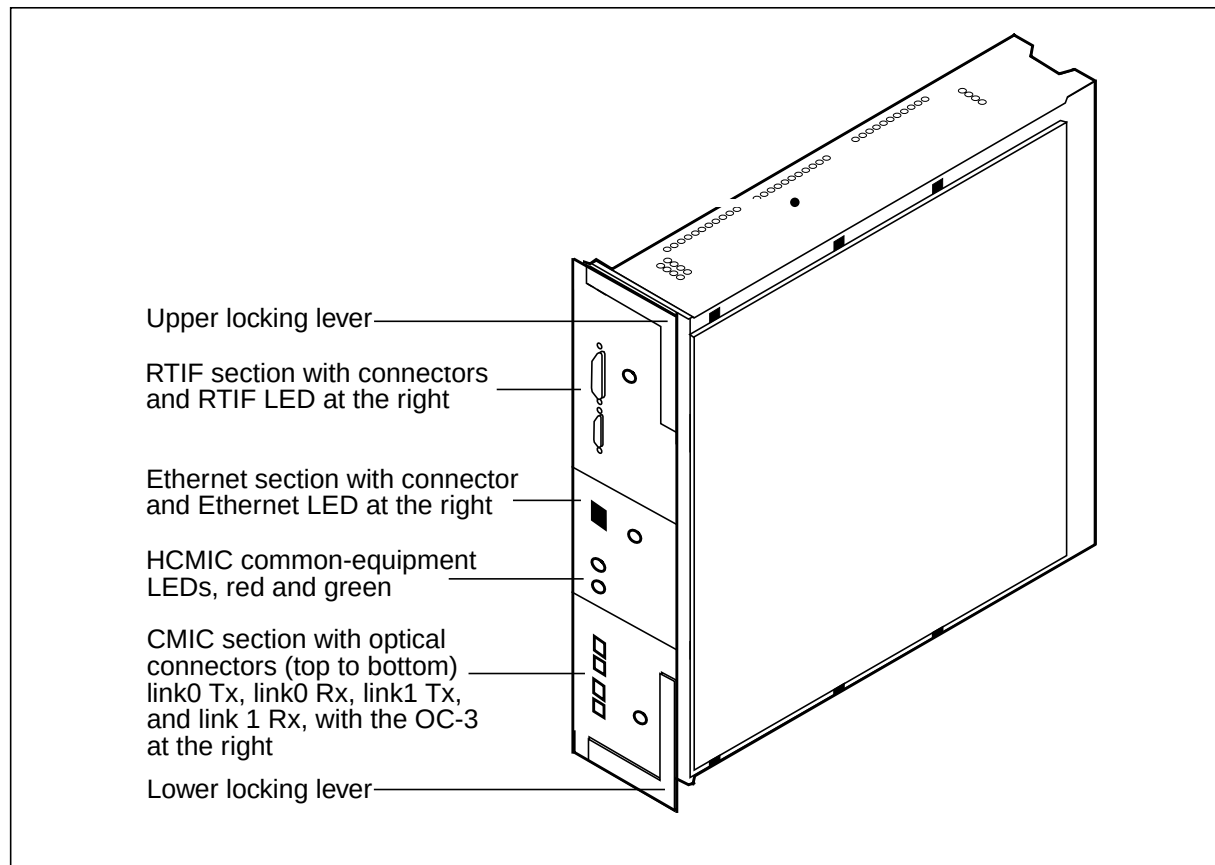
NTLX17 high performance CMIC circuit pack front and side views
