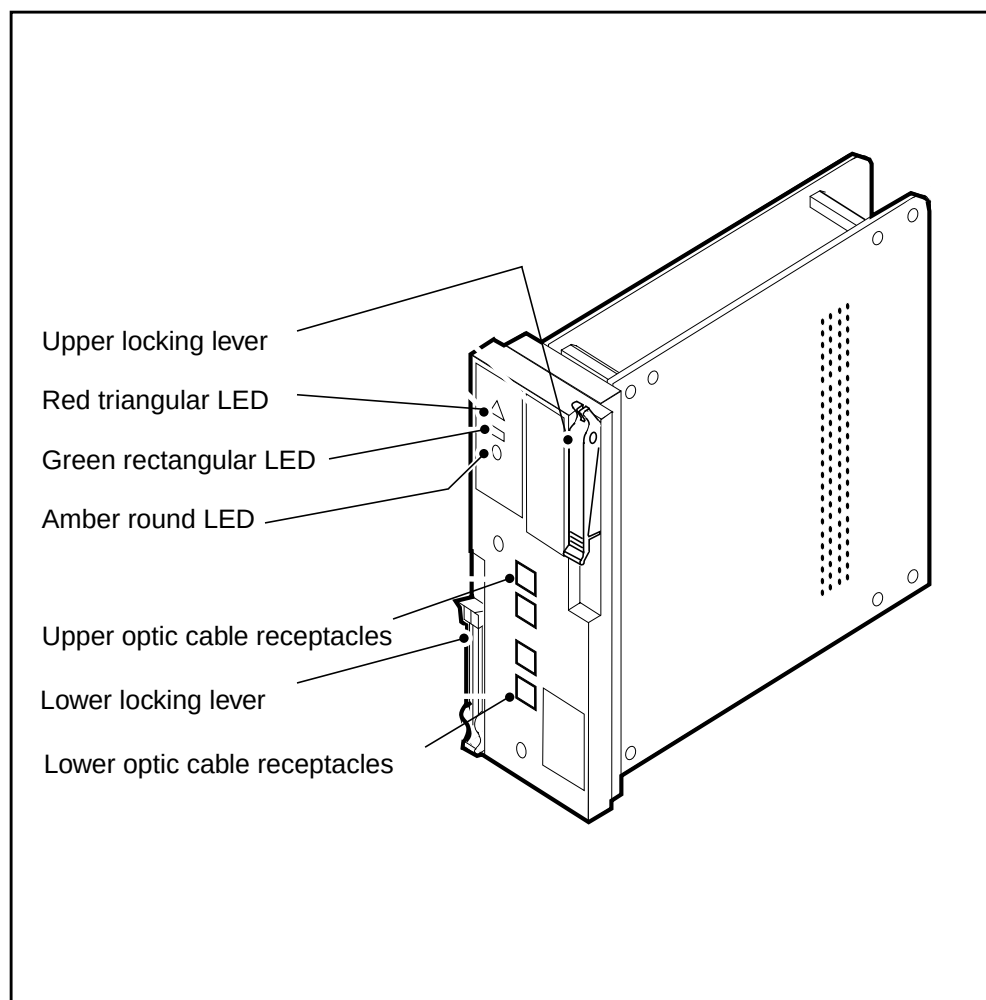
NTLX05BA OC-3 two-port interface packlet
