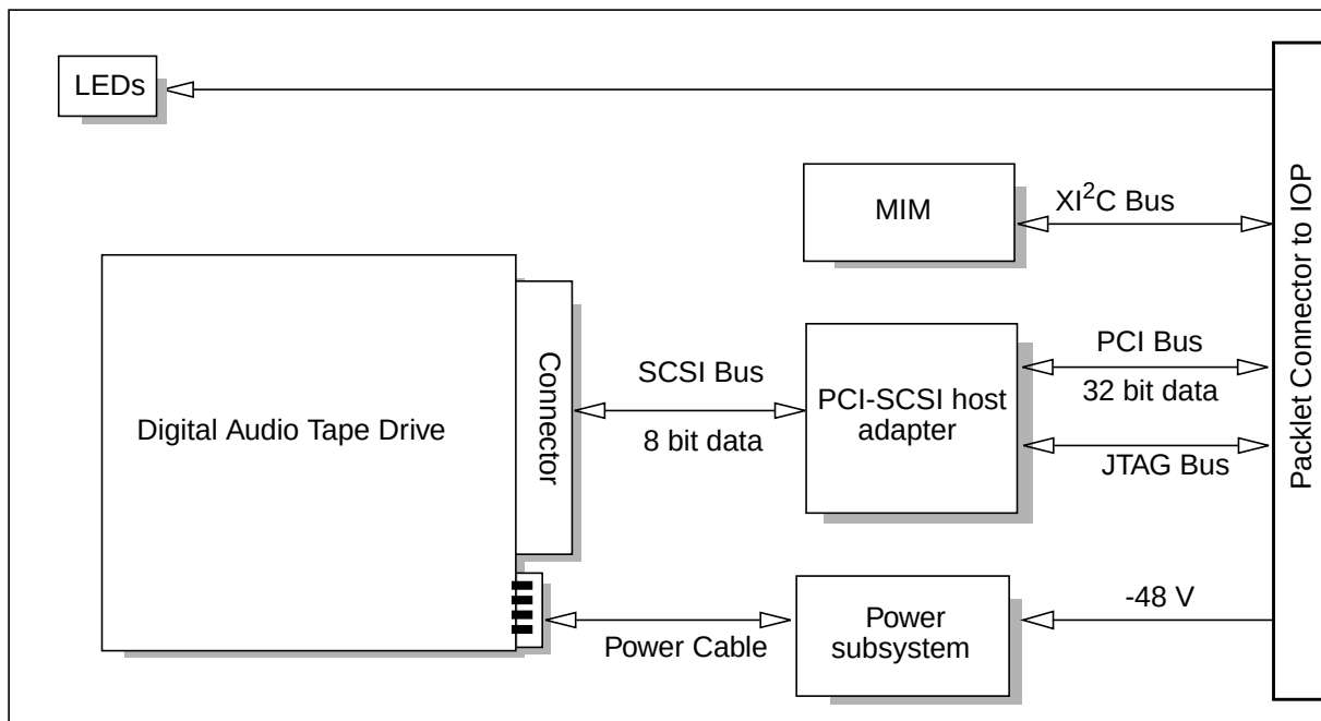
NTLX07 functional blocks
