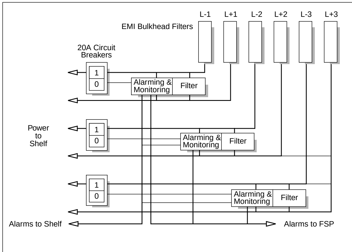
NTLX12AA functional blocks
