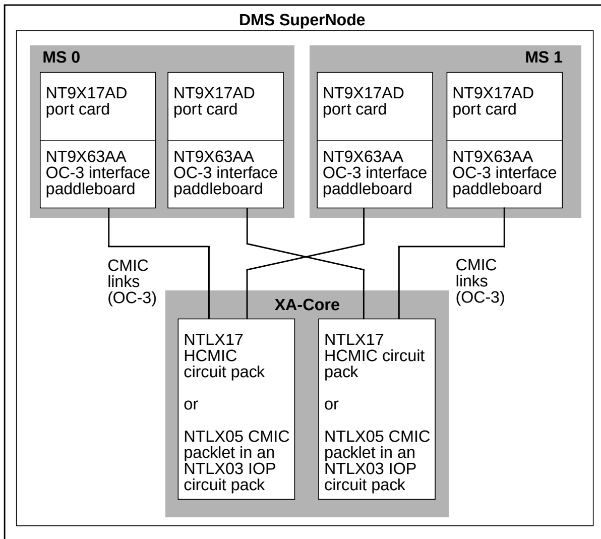
Figure 1-6 XA-Core to MS port connections for DMS SuperNode
