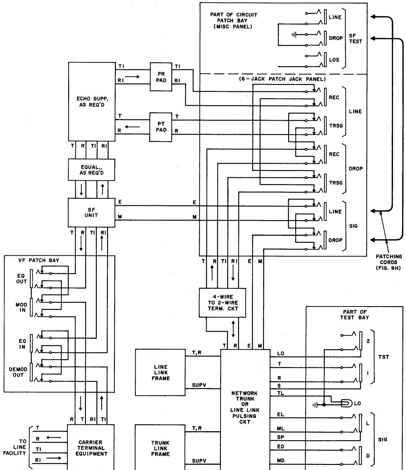
Fig. 11 — Typical Arrangement For Test and Patch Jacks (Patched For Single Frequency Testing)—17E Testboard
