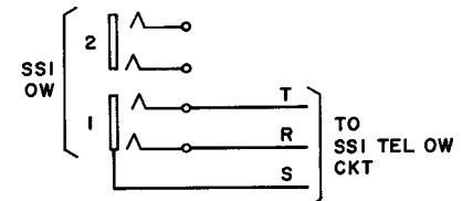
FIG. 8D SSI TELEPHONE ORDER WIRE JACKS SD-56540-01, FIG. 6
