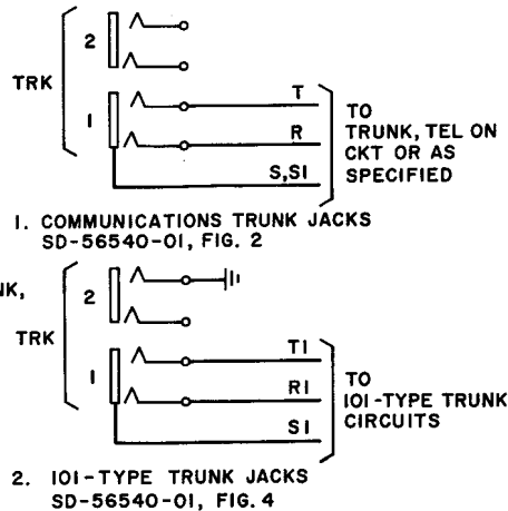
FIG. 8B TRUNK JACK CIRCUITS
