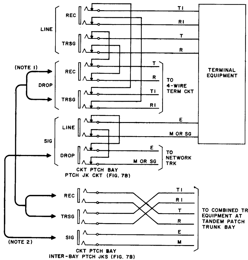
FIG. 12B TYPICAL DROP PATCH USING COMBINED SPARE EQUIPMENT AT TANDEM PATCH TRUNK BAY SD-68327-01, FIG. 111
