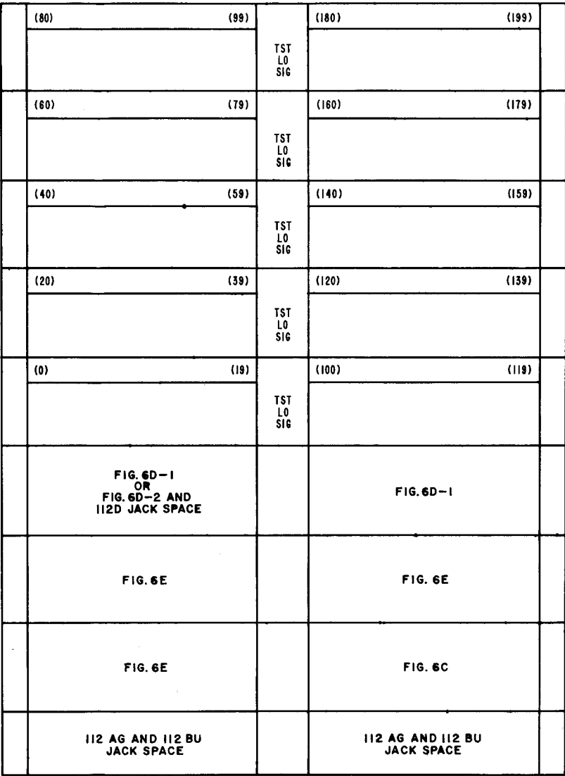
FIG. 6A-TEST BAY JACK FIELD
