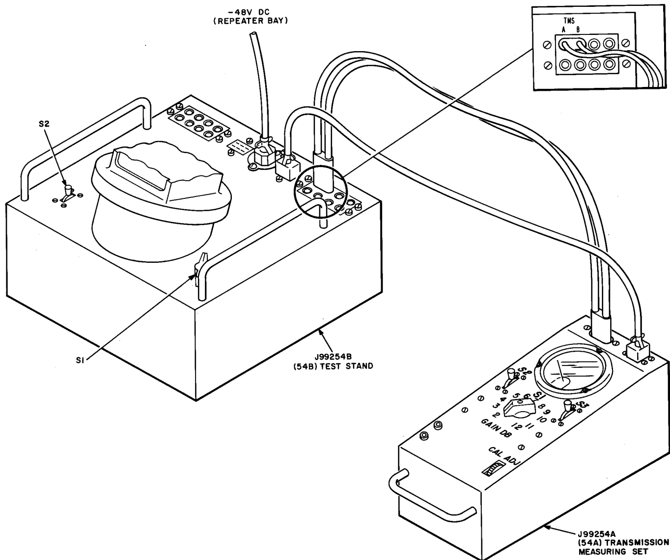
◆Fig. 1—Converter Gain—Test Equipment Connections◆
