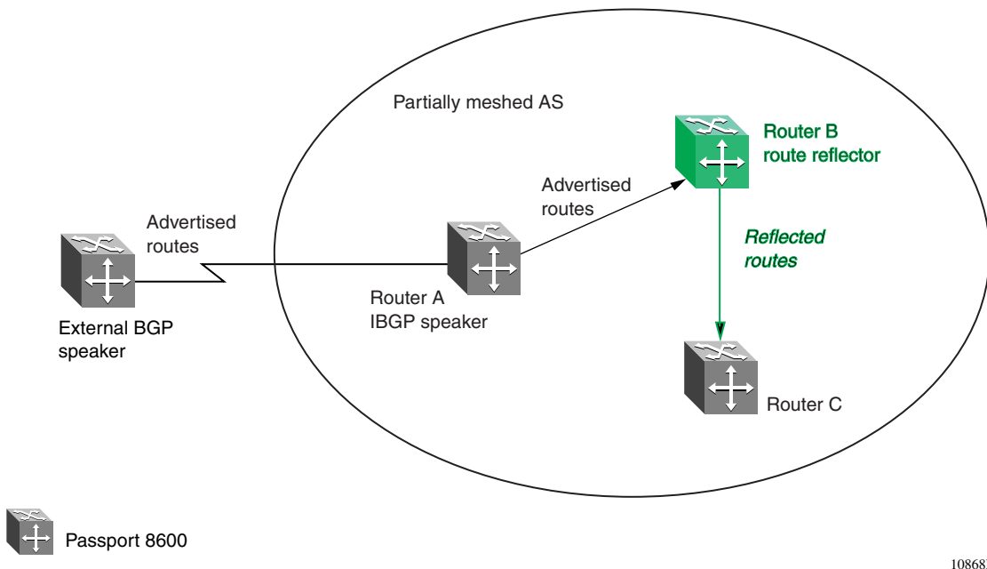
Figure 9 AS with route reflector
