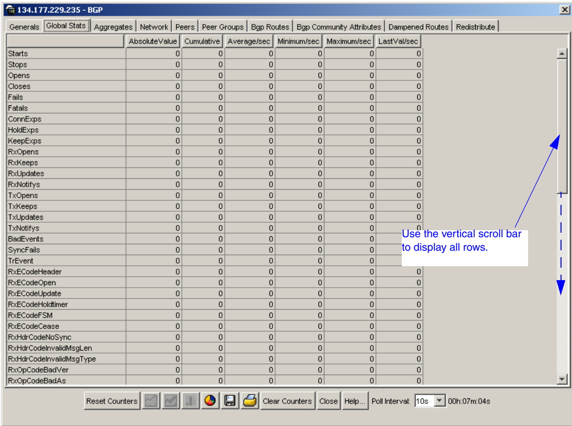
Figure 17 BGP dialog box—Global Stats tab
