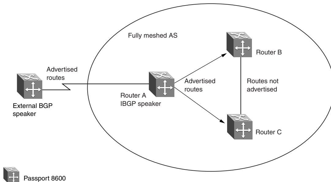
Figure 8 Fully meshed AS with IBGP speakers
