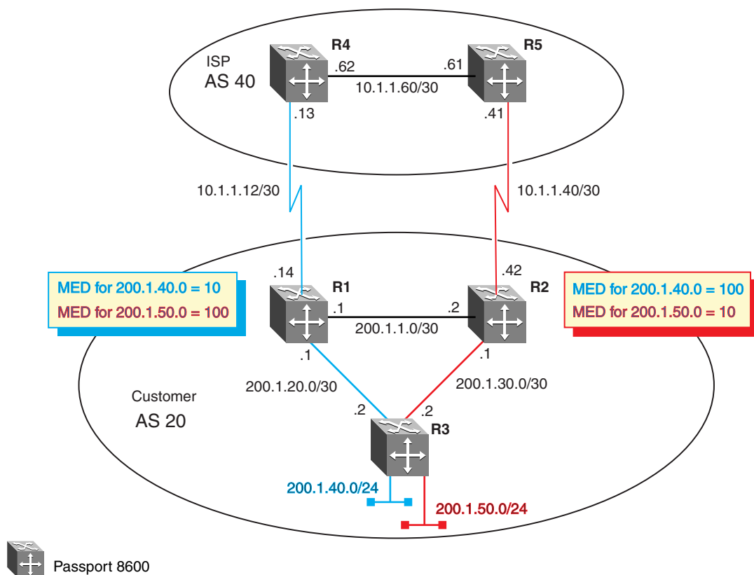
Figure 109 Using the MED attribute for load balancing routes
