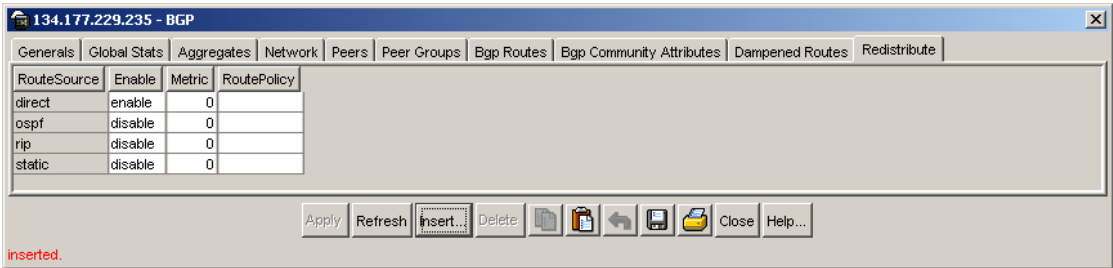
Figure 37 BGP dialog box—Redistribute tab
