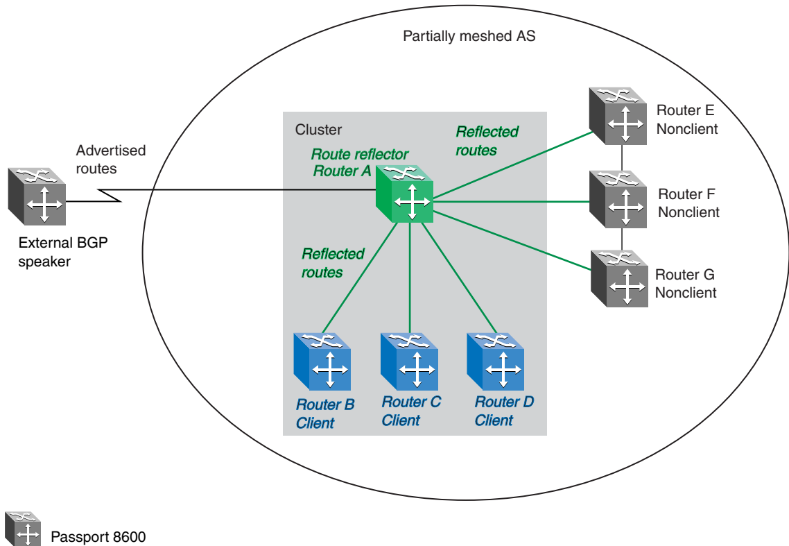
Figure 10 Route reflector with client and nonclient peers
