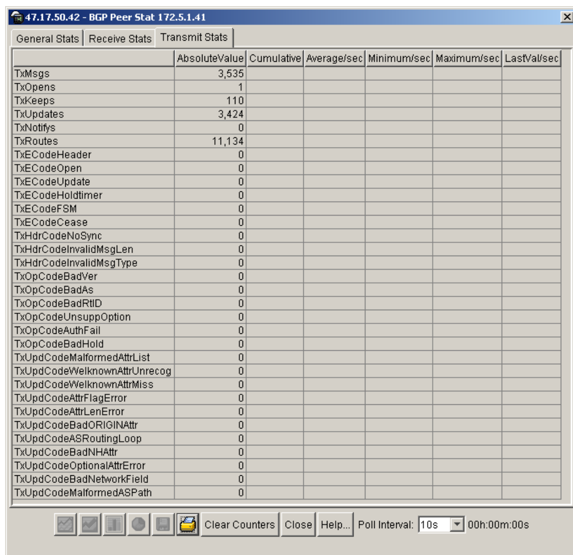
Figure 27 BGP Peer Stat dialog box—Transmit Stats tab
