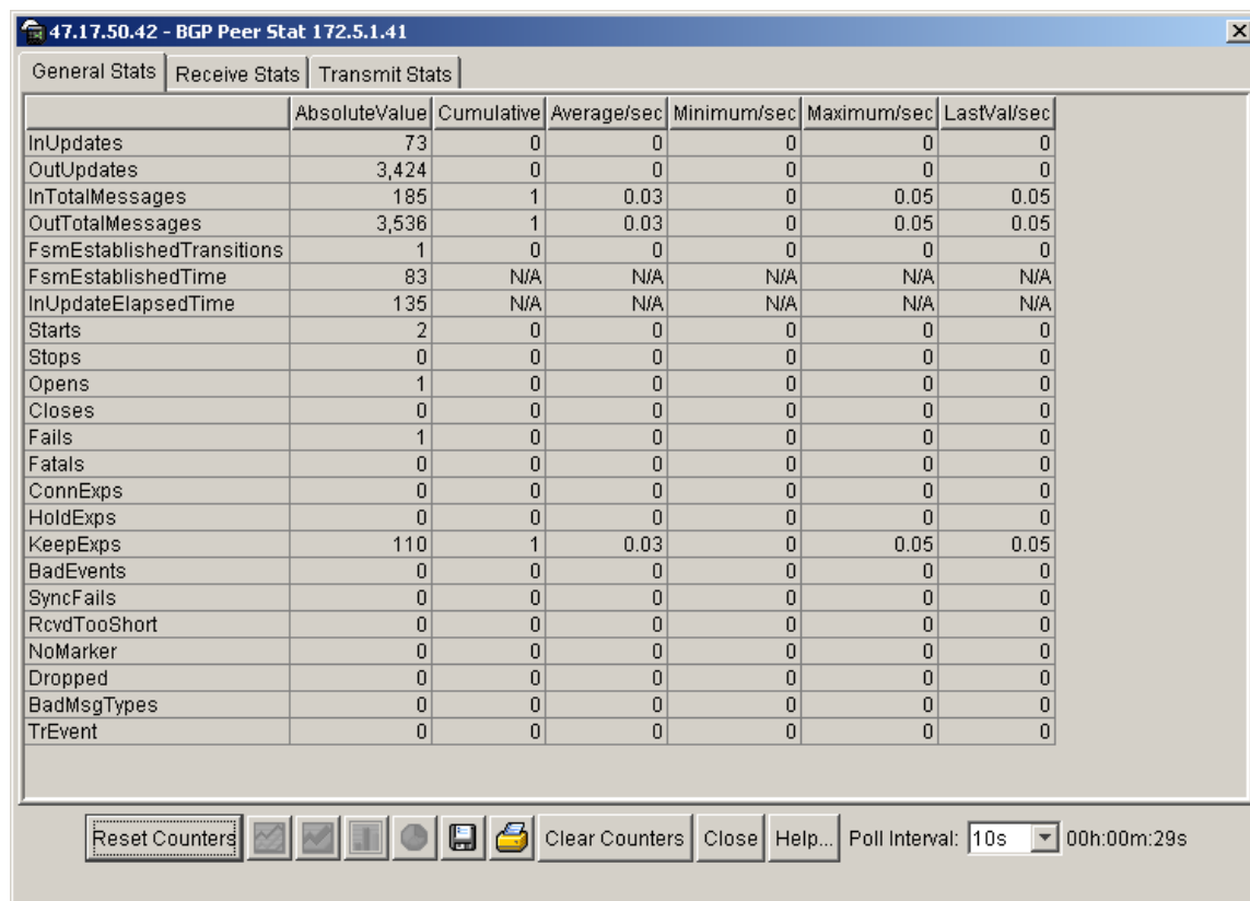
Figure 25 BGP Peer Stat dialog box—General Stats tab
