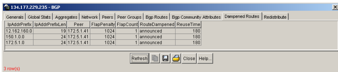
Figure 36 BGP dialog box—Dampened Routes tab
