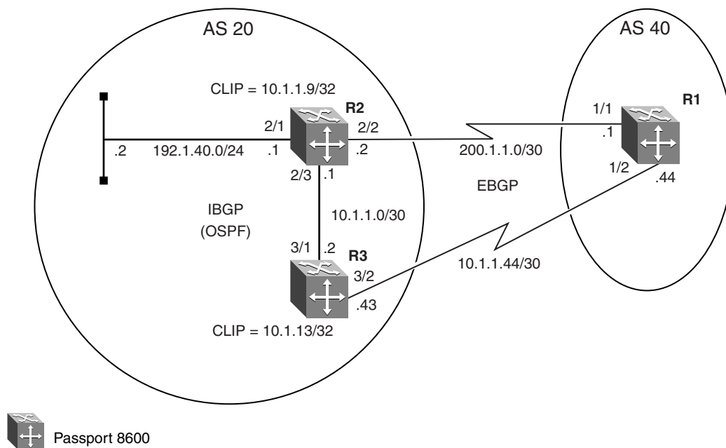
Figure 86 Basic BGP configuration
