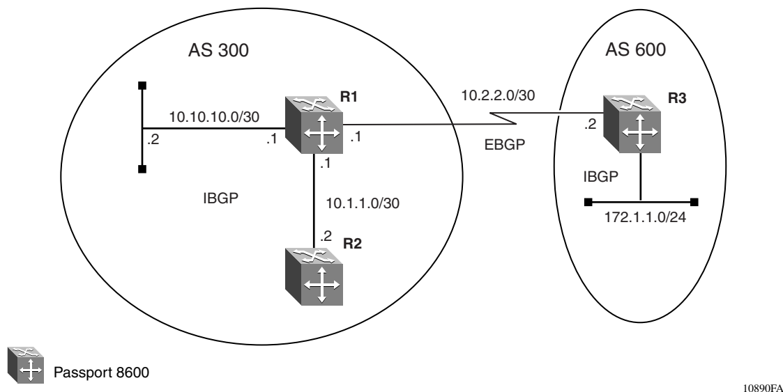
Figure 115 Route flap dampening example
