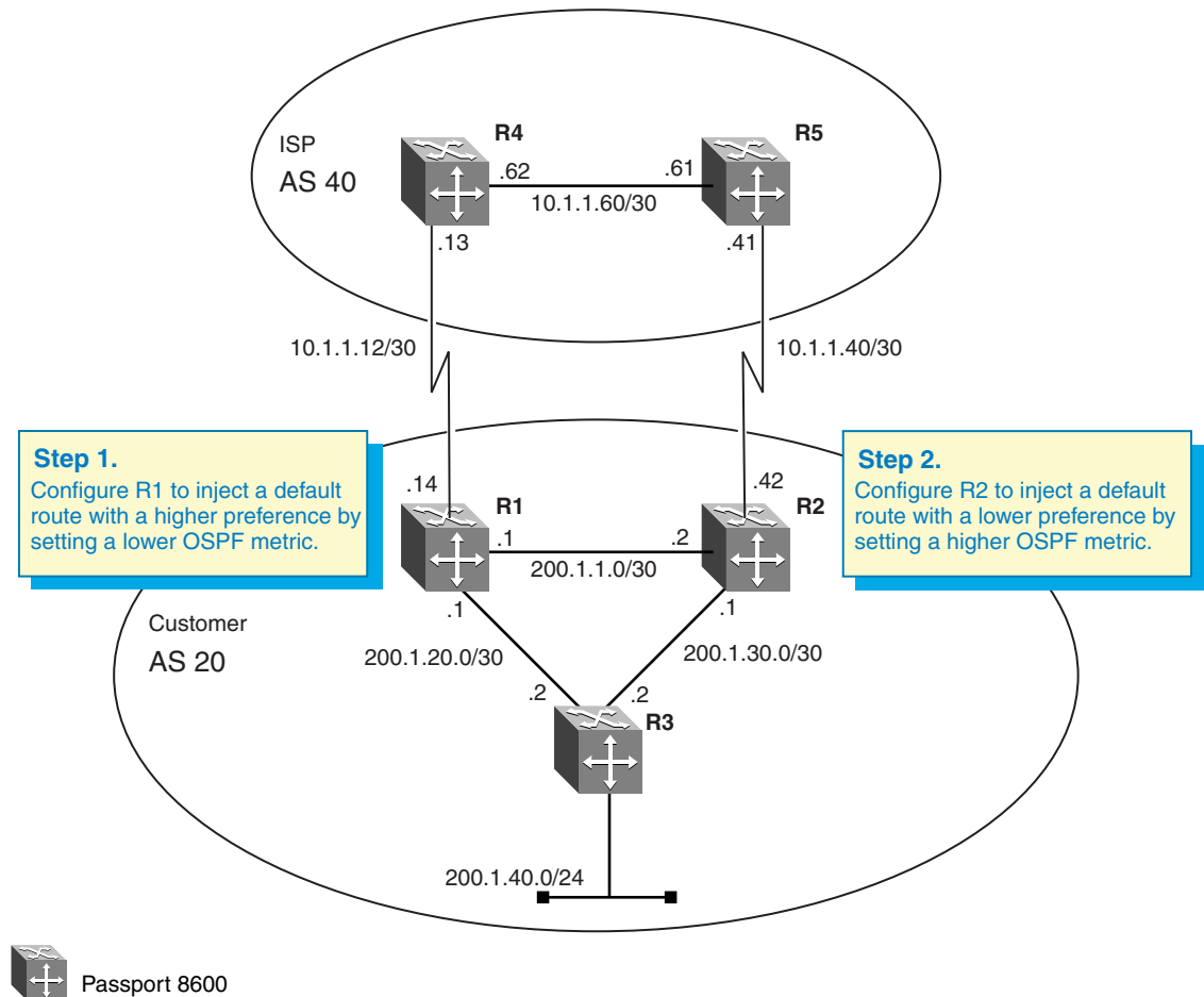
Figure 89 Injecting a default route example
