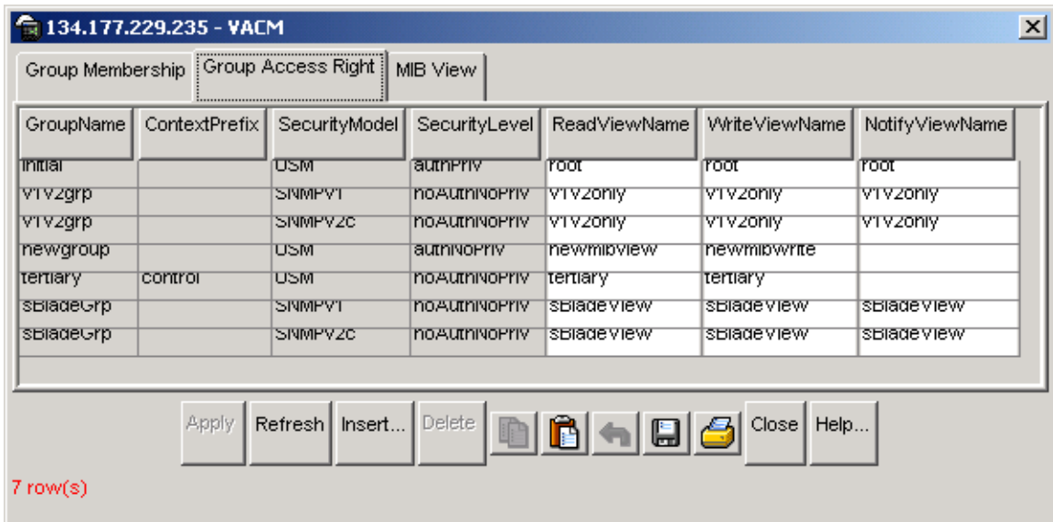
Figure 40 VACM dialog box—Group Access Right tab
