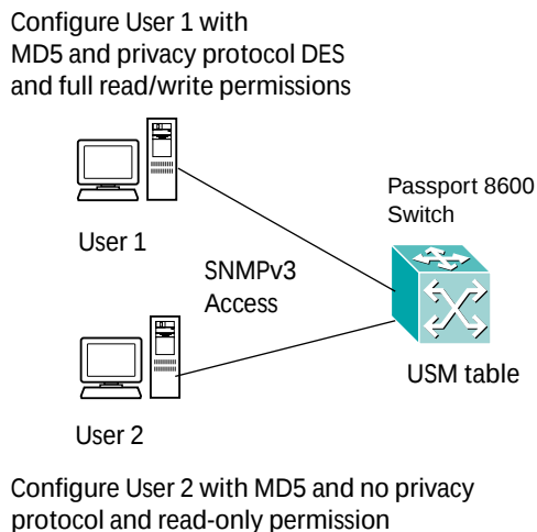
Figure 97 SNMPv3 for users with different permissions/privacy protocols
