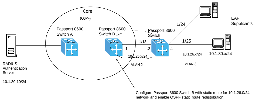
Figure 96 EAPoL via L3
