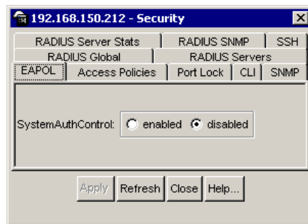
Figure 68 Security tab
