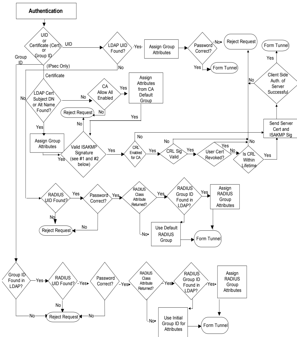
Figure 3 Authentication server validation flowchart
