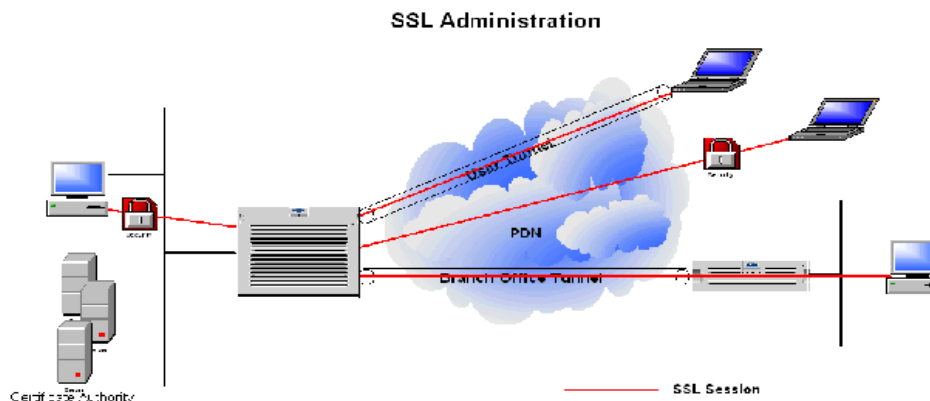
Figure 9 SSL administration
