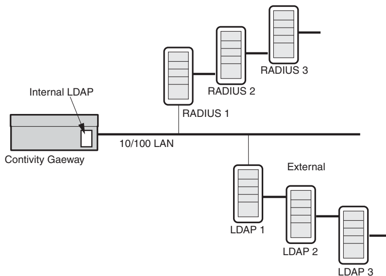
Figure 2 Authentication servers
