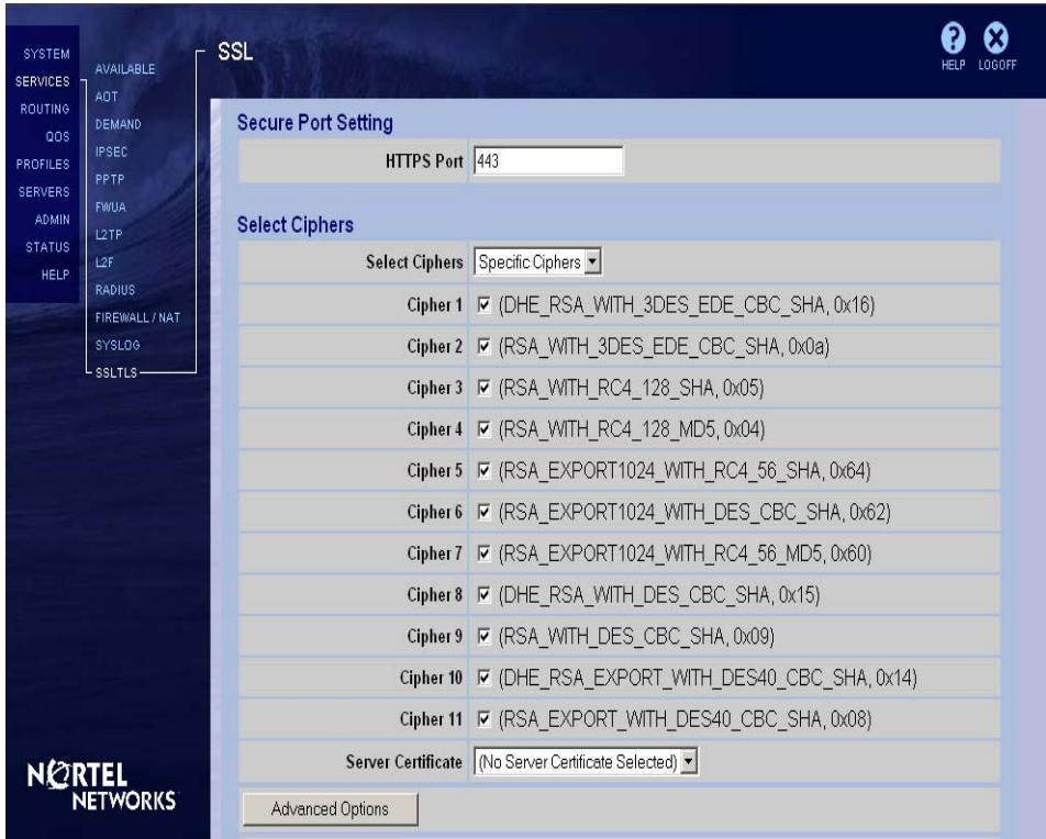
Figure 11 Select ciphers
