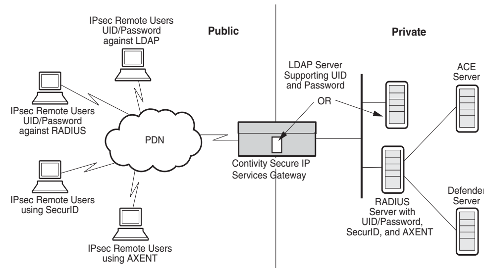
Figure 4 IPsec client authentication options
