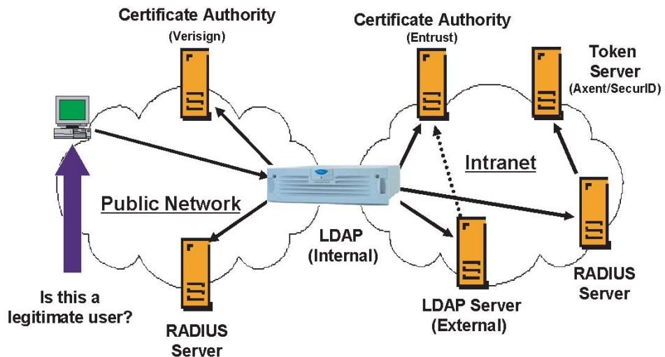
Figure 1 Authenticating users
