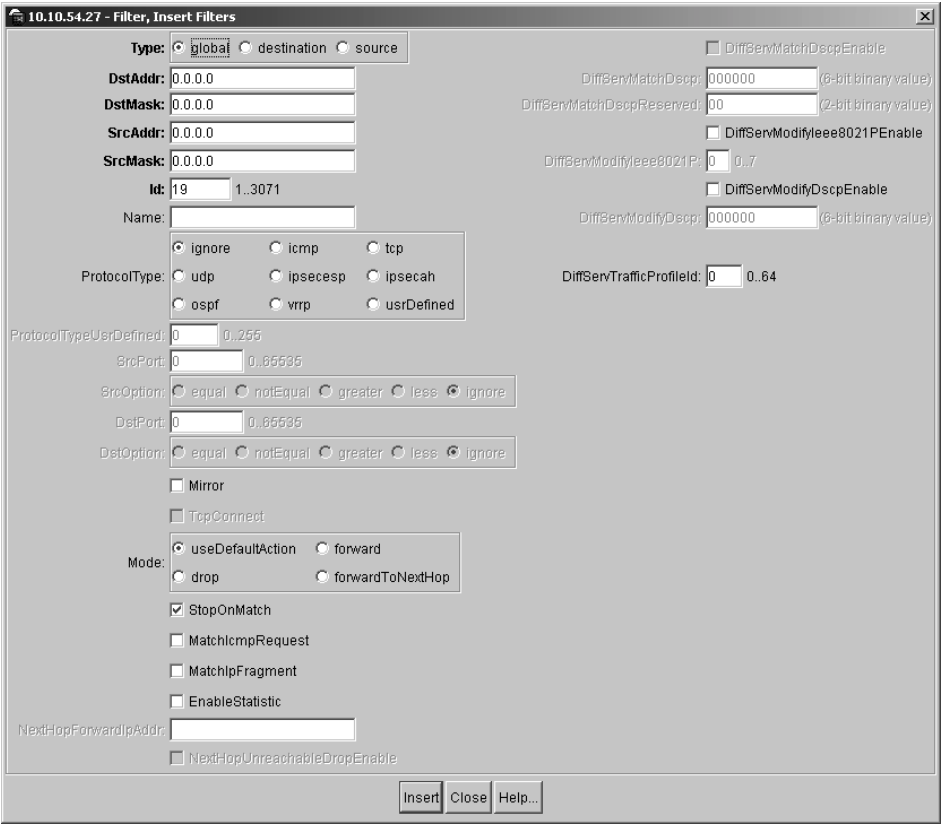
Figure 32 Filter, Insert Filters dialog box—global type selected
