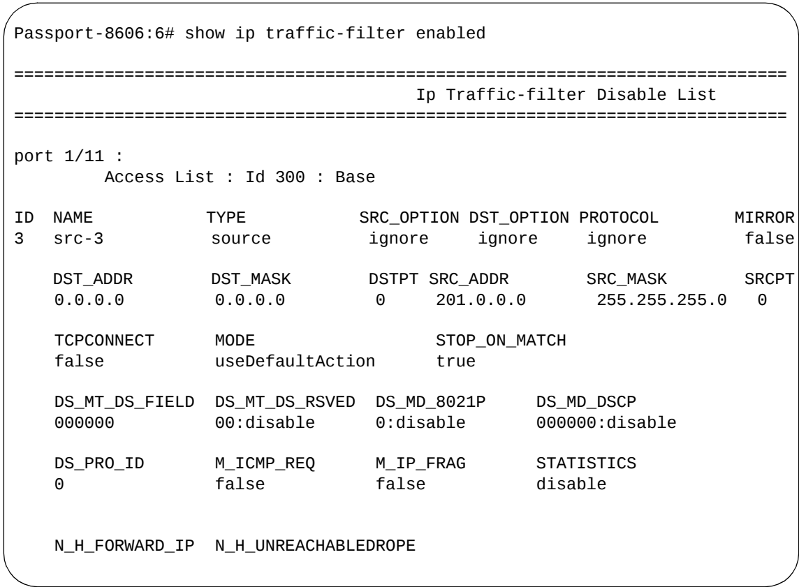
Figure 68 show ip traffic-filter enabled command output
