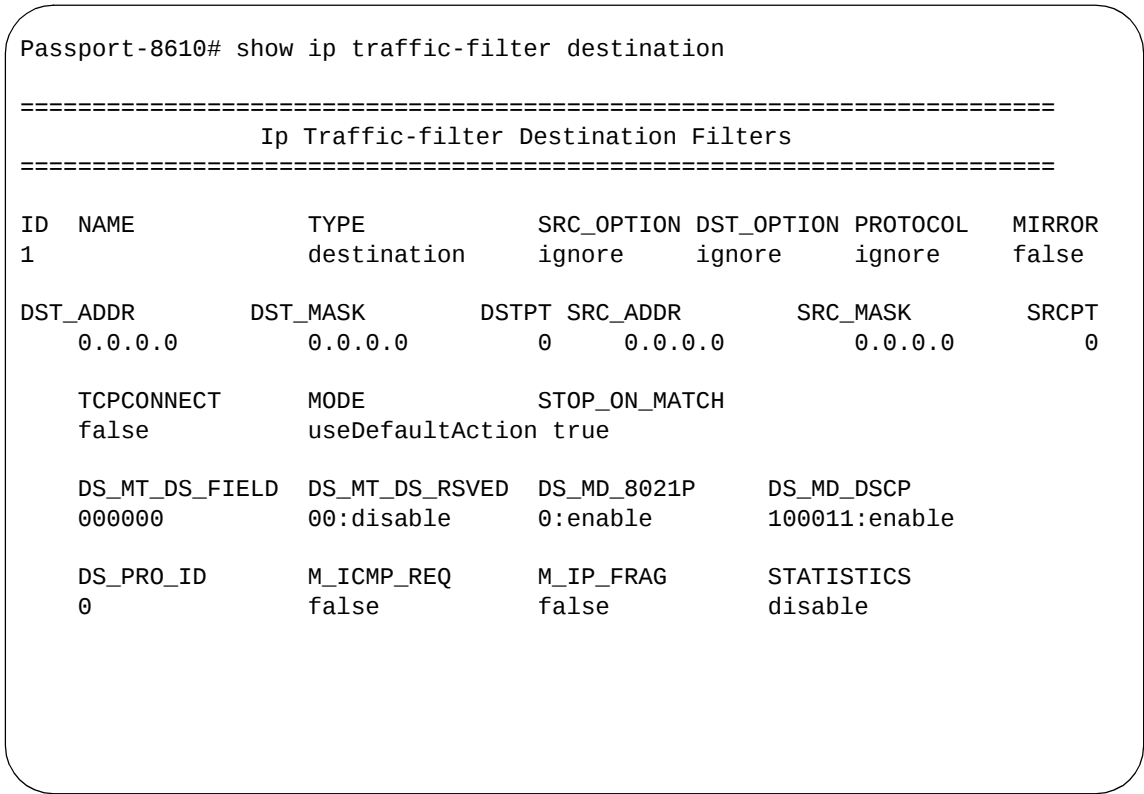
Figure 66 show ip traffic-filter destination command output
