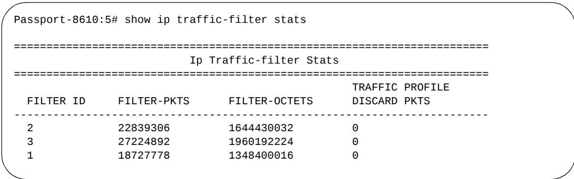
Figure 6 show ip traffic-filter stats
