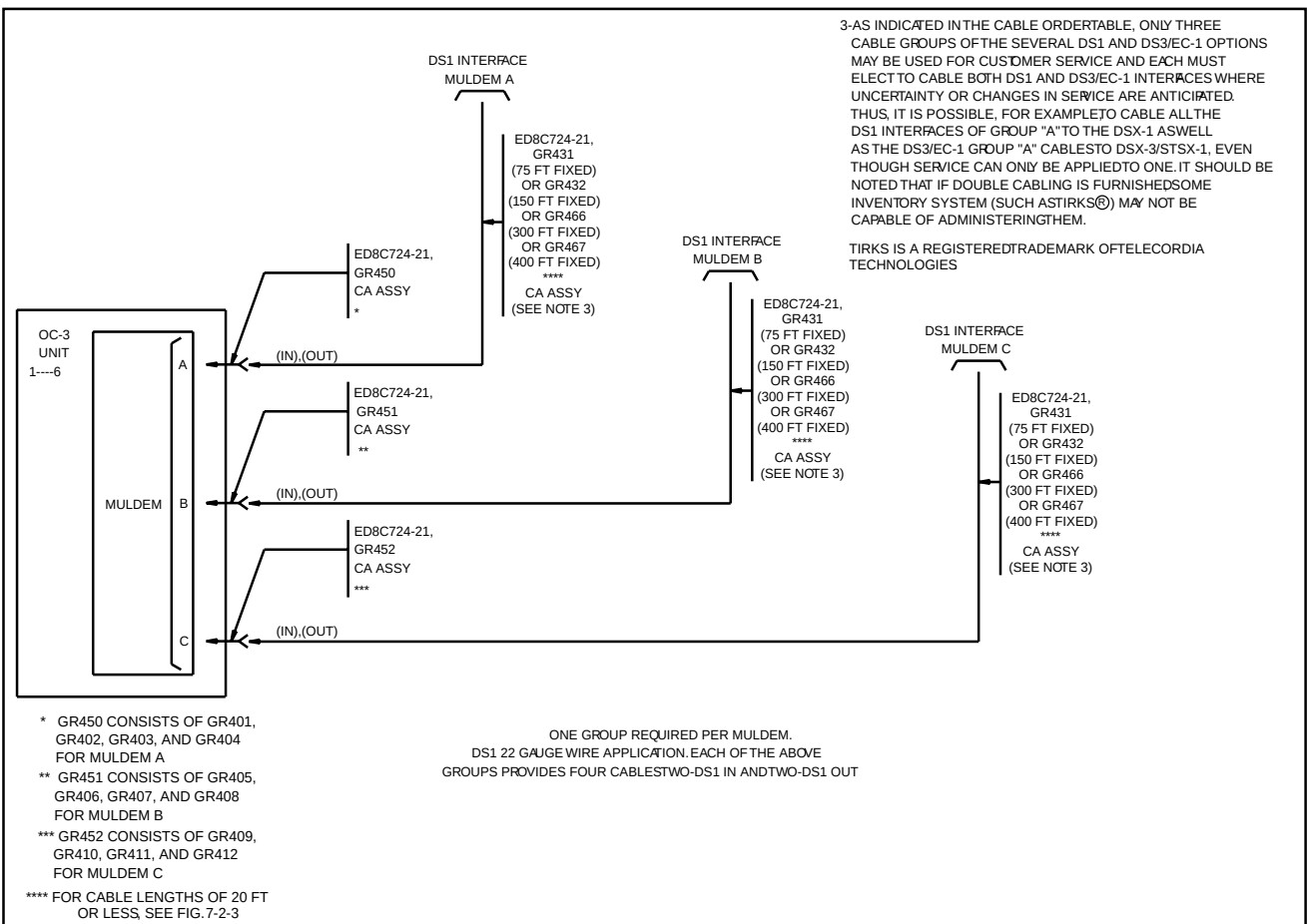
Figure 7-2-3 DS1 Transmission Cables — 22 Gauge
