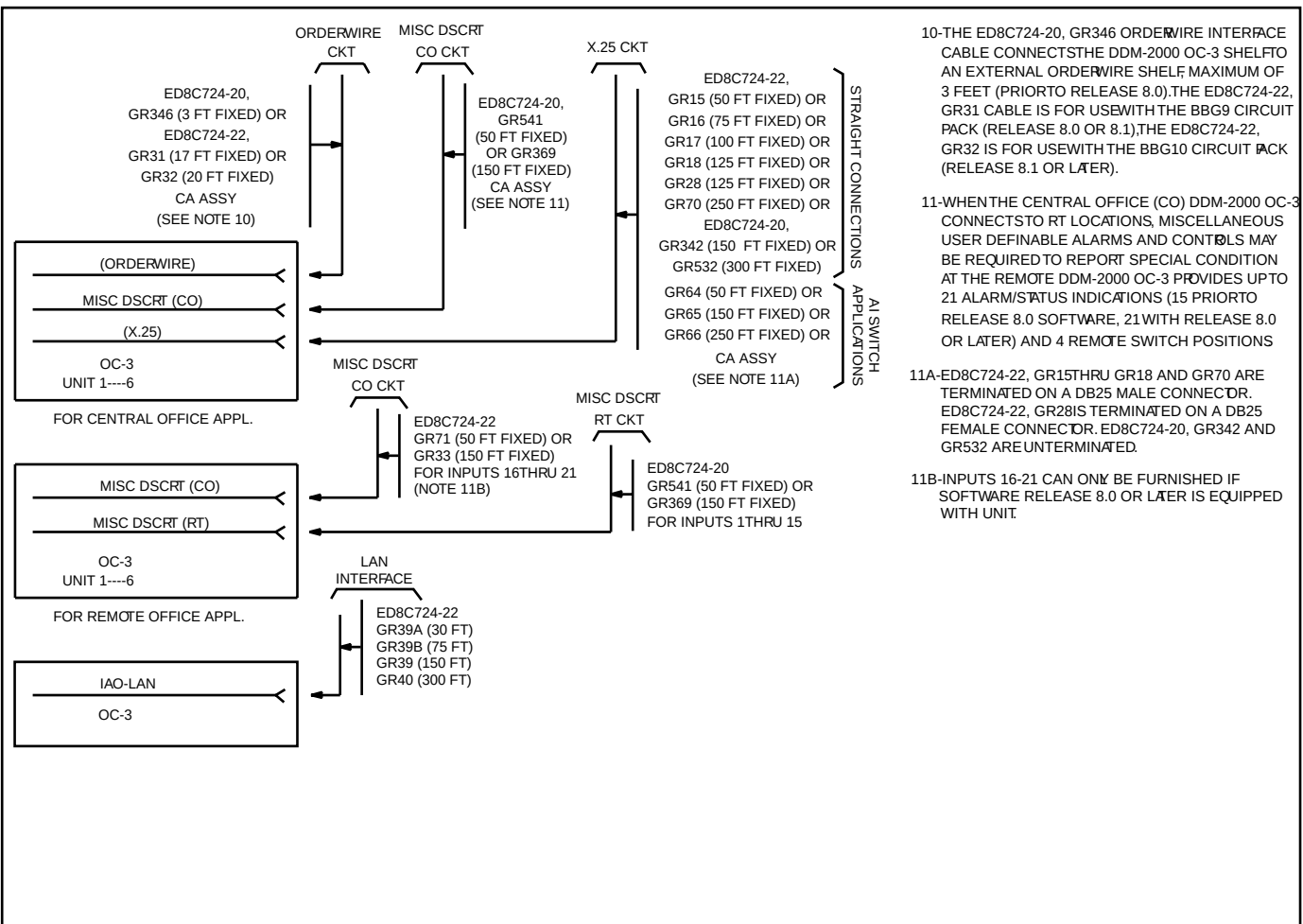
Figure 7-1-12 X.25 Interface, Miscellaneous Discretes, Orderwire, and LAN
