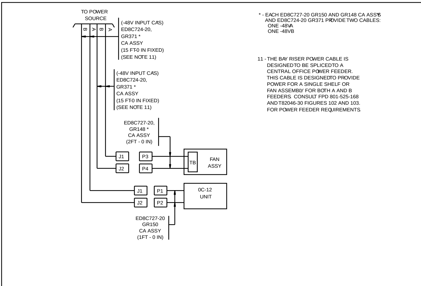
Figure 8-1-11 Power for Single OC-12 Unit and Fan Assembly
