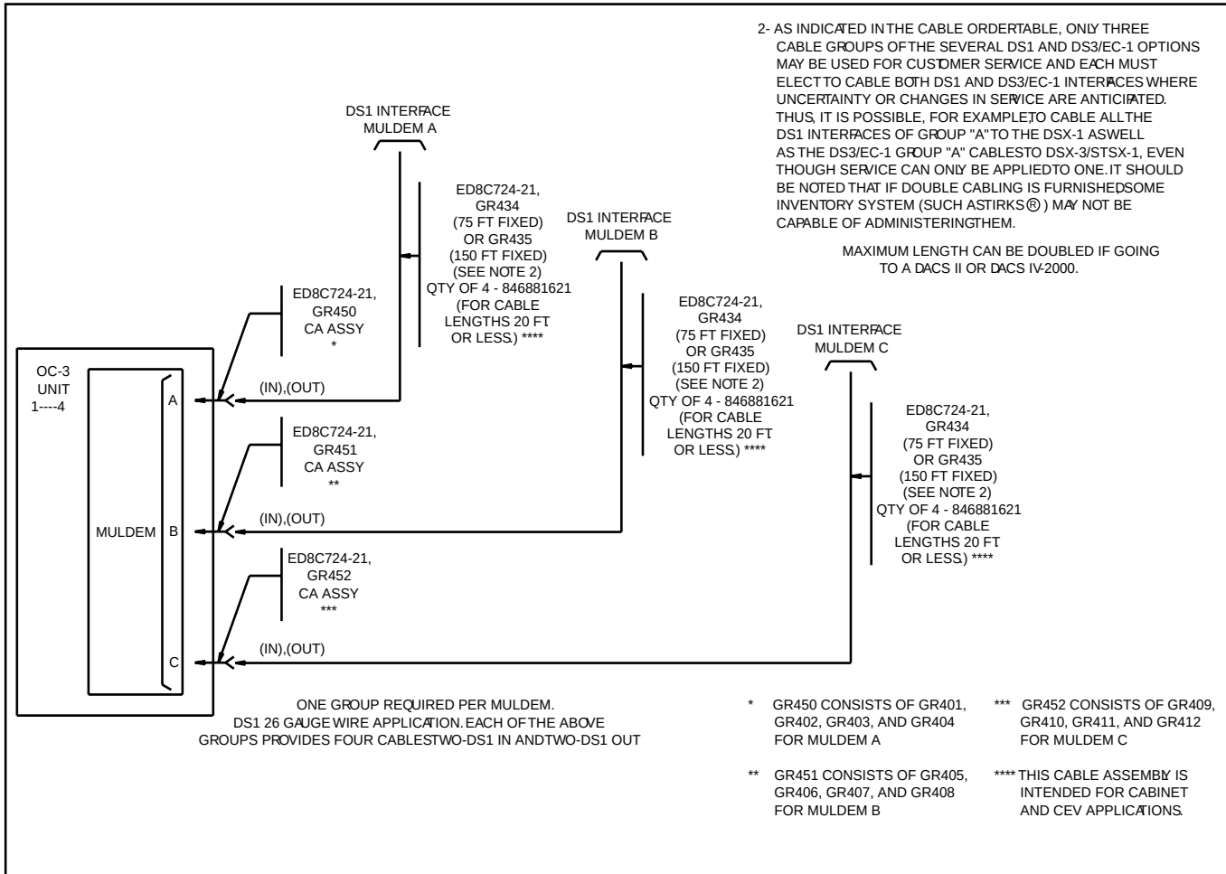
Figure 7-4-2 DS1 Transmission Cables — 26 Gauge
