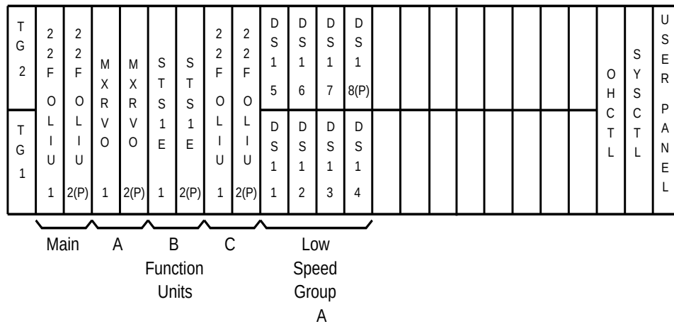
Figure 6-26. DDM-2000 OC-3 DS1 Add/Drop Shelf
