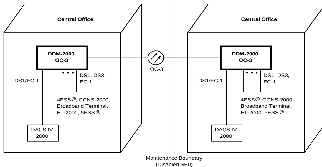
Figure 3-37. OC-3 Point-to-Point Interoffice Configuration
