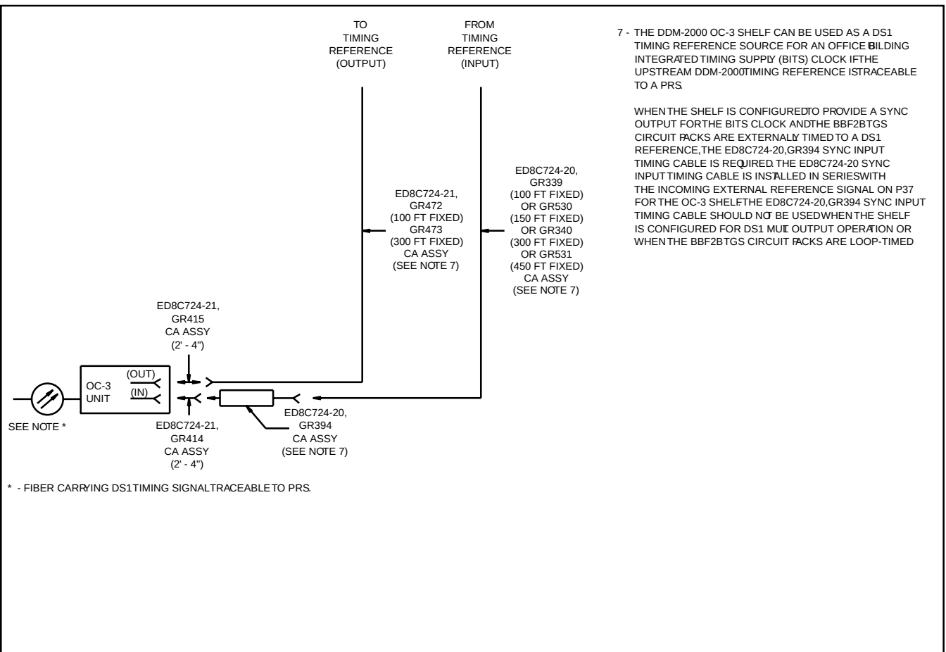
Figure 7-2-8 Synchronization for Timing Distribution Cable in a Single Shelf Assembly
