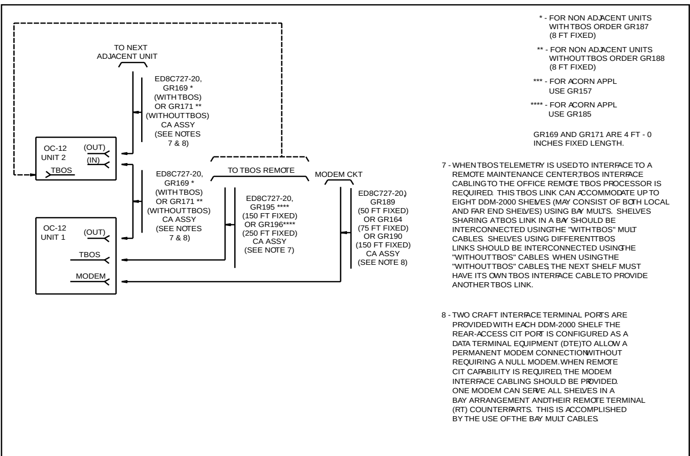
Figure 8-1-9 Modem, TBOS Interface, and Bay Mult Cable for TBOS, CIT, and Modem
