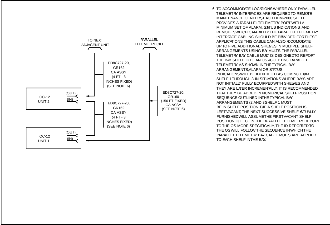
Figure 8-1-8 Parallel Telemetry Interface and Mult Cable
