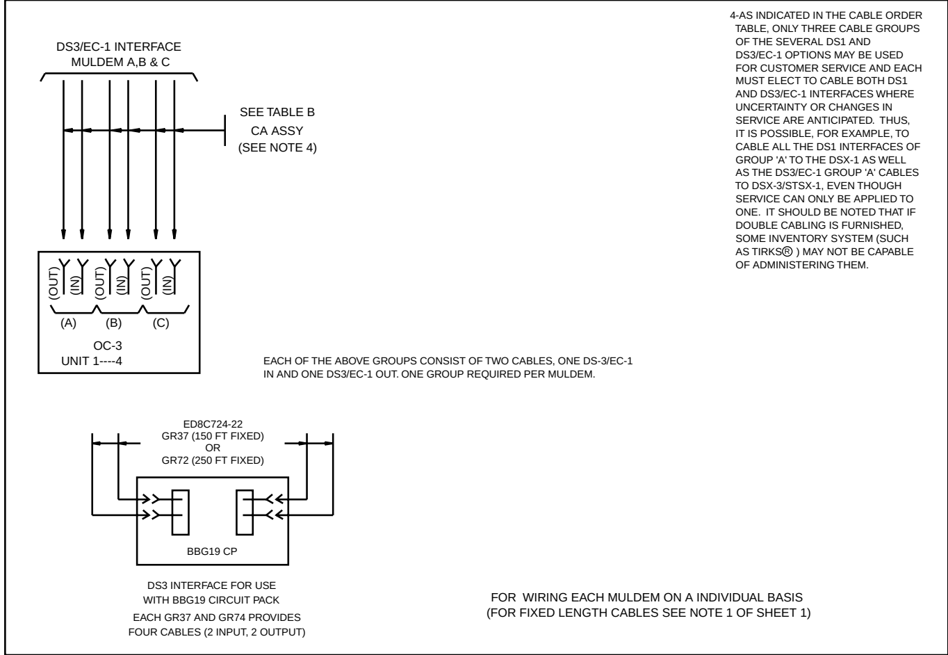
Figure 7-3-7 DS3/EC-1 TRANSMISSION CABLE
