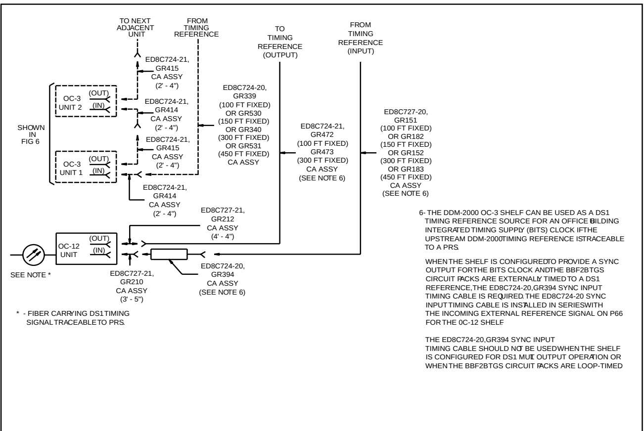
Figure 7-4-9 Synchronization for Timing Distribution Cable in a Bay Arrangement
