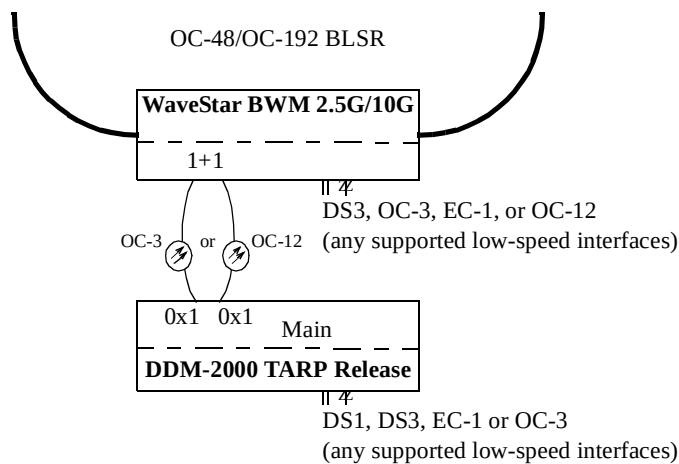
Figure 3-61. DDM-2000 to WaveStar Connectivity
