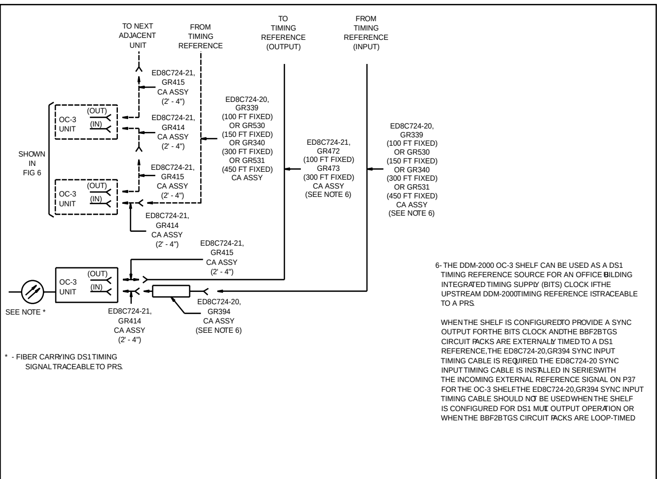
Figure 7-2-7 Synchronization for Timing Distribution Cable in a Bay Arrangement
