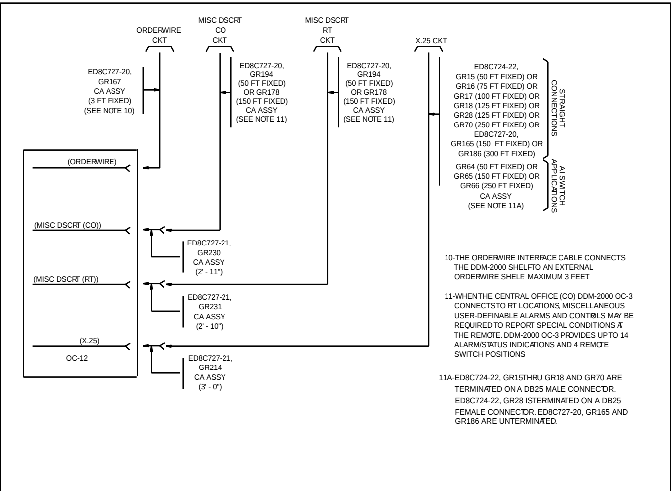
Figure 7-4-13 X.25 Interface, Miscellaneous Discretes, and Orderwire
