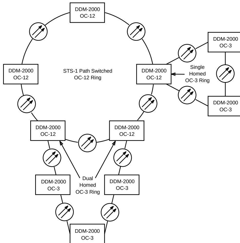
Figure 3-11. Multinode OC-3 Ring With OC-12 Ring Transport
