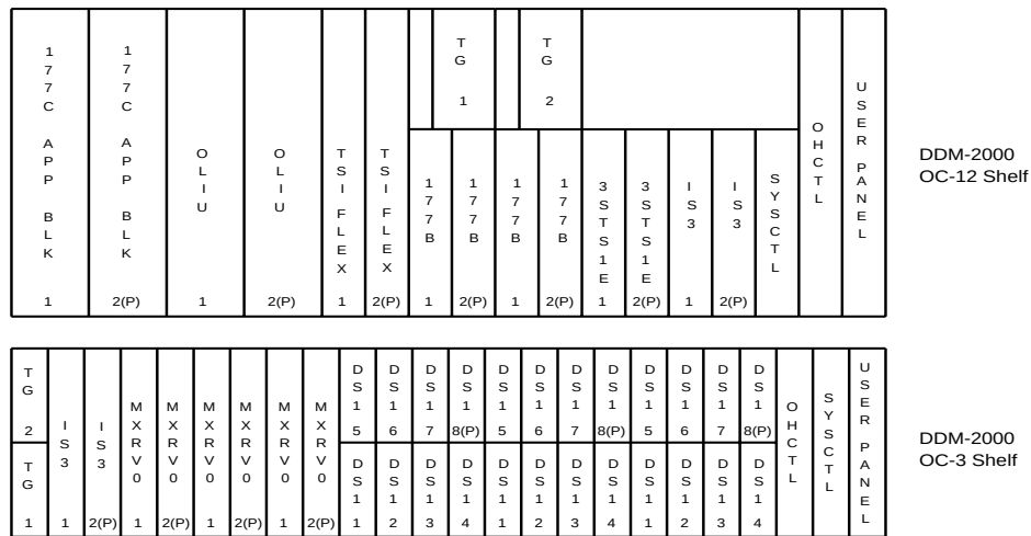
Figure 7-15. OC-3/12 Ring Shelf Equipped With 3 EC-1s and 84 DS1s
