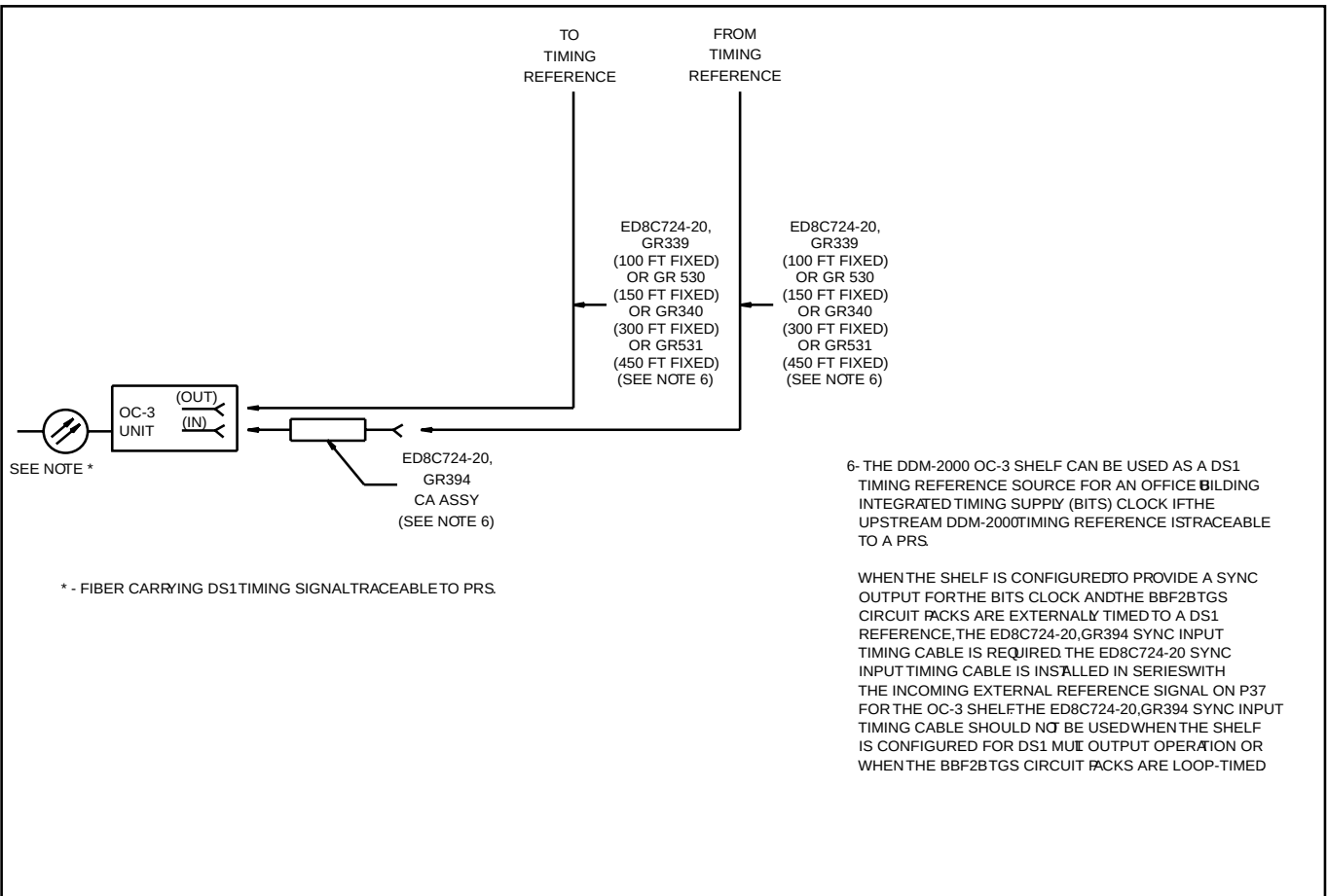
Figure 7-1-8 Synchronization for Timing Distribution Cable in a Single Shelf Assembly
