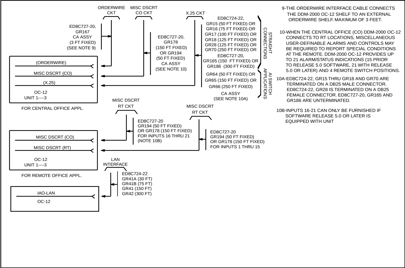
Figure 8-1-10 X.25 Interface, Miscellaneous Discretes, Order Wire, and LAN
