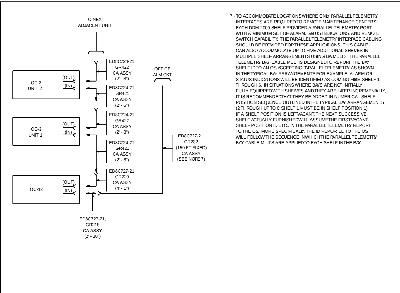
Figure 7-4-11 Parallel Telemetry Interface and Mult Cable
