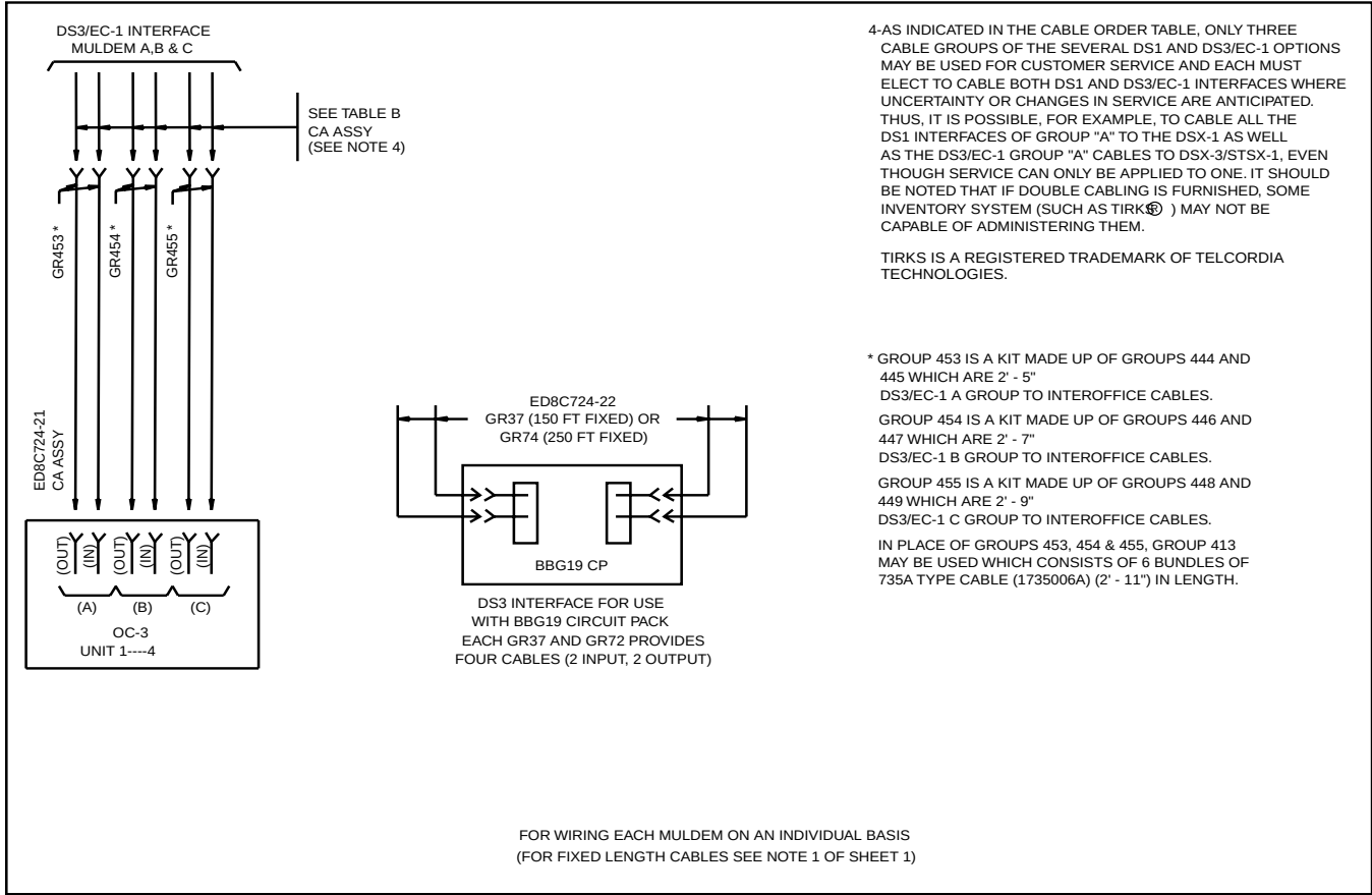
Figure 7-4-7 DS3/EC-1 TRANSMISSION CABLE
