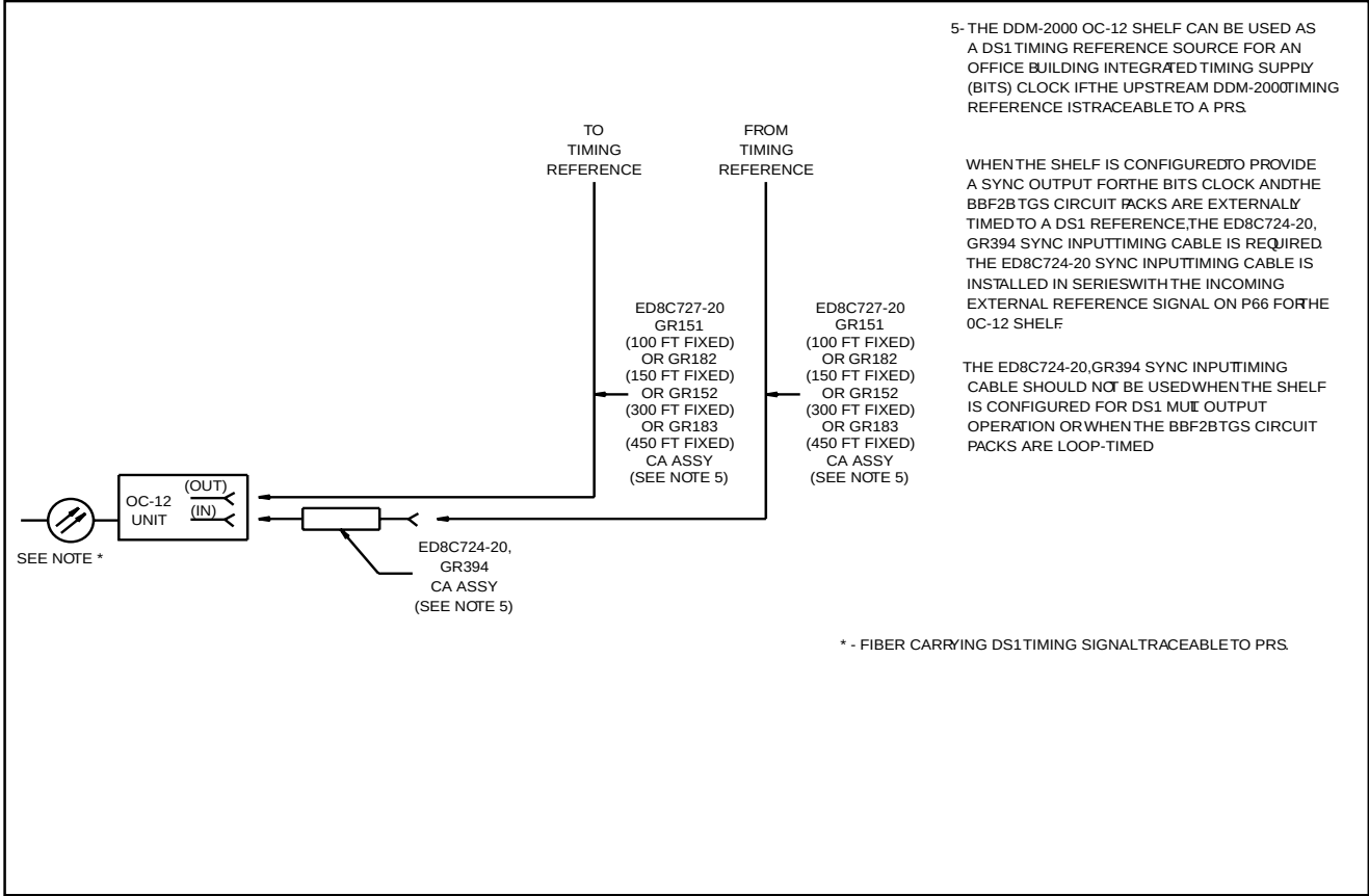
Figure 8-1-6 Synchronization for Timing Distribution Cable in a Single Shelf Assembly
