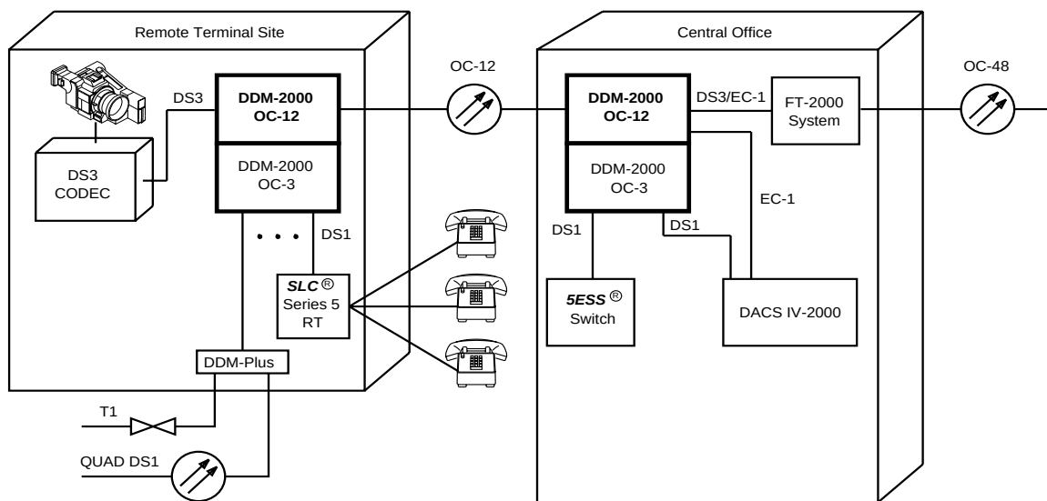
Figure 3-38. OC-12 Point-to-Point Loop Configuration
