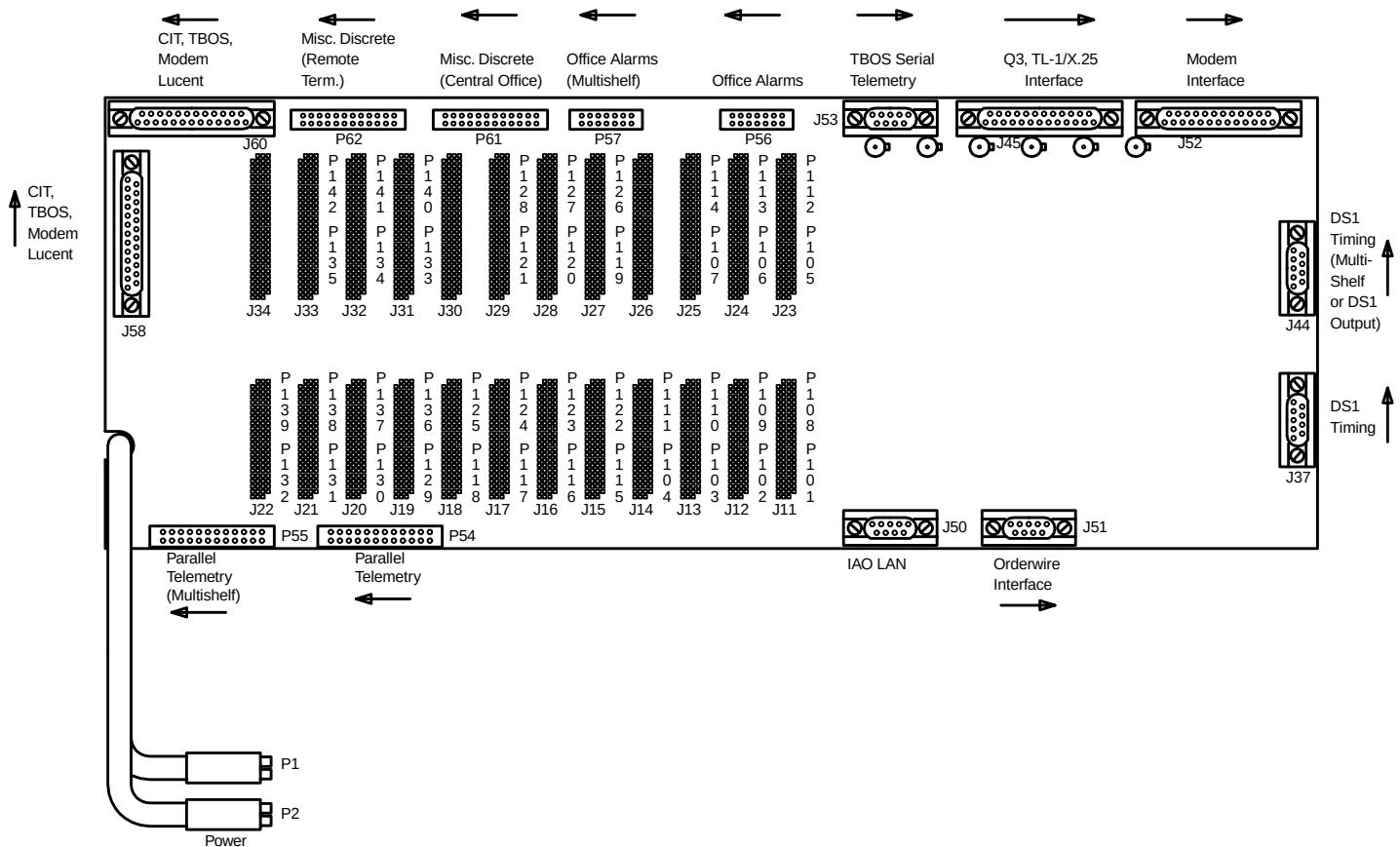
Figure 4-2. DDM-2000 OC-3 Group 4 Shelf — Rear View
