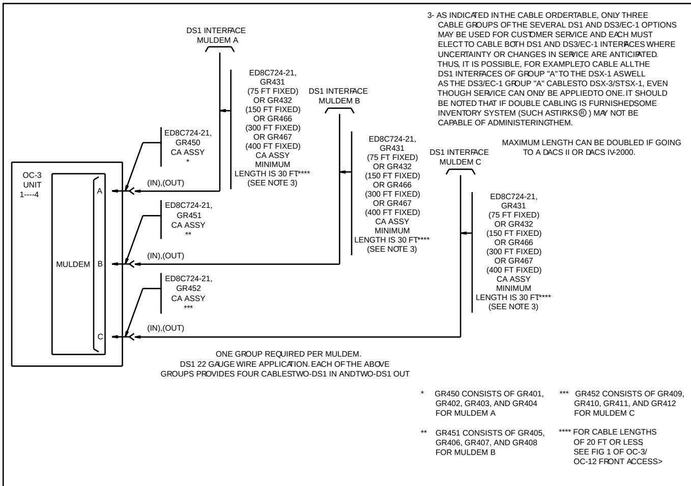
Figure 7-4-3 DS1 Transmission Cables — 22 Gauge
