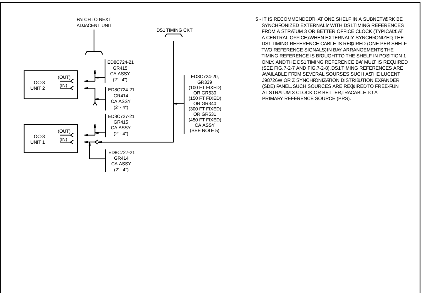
Figure 7-2-6 DS1 Timing Reference Interface and Mult Cable
