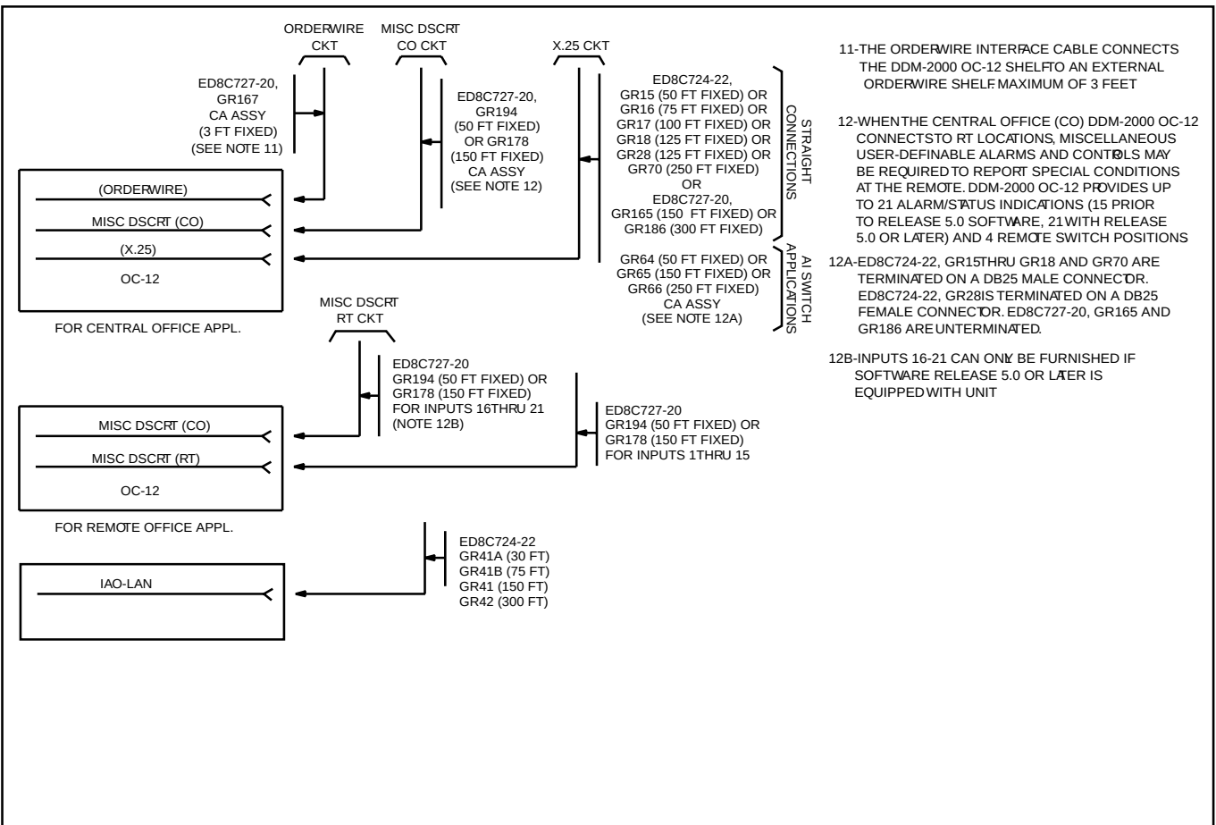
Figure 7-3-13 X.25 Interface, Miscellaneous Discretes, Orderwire, and LAN
