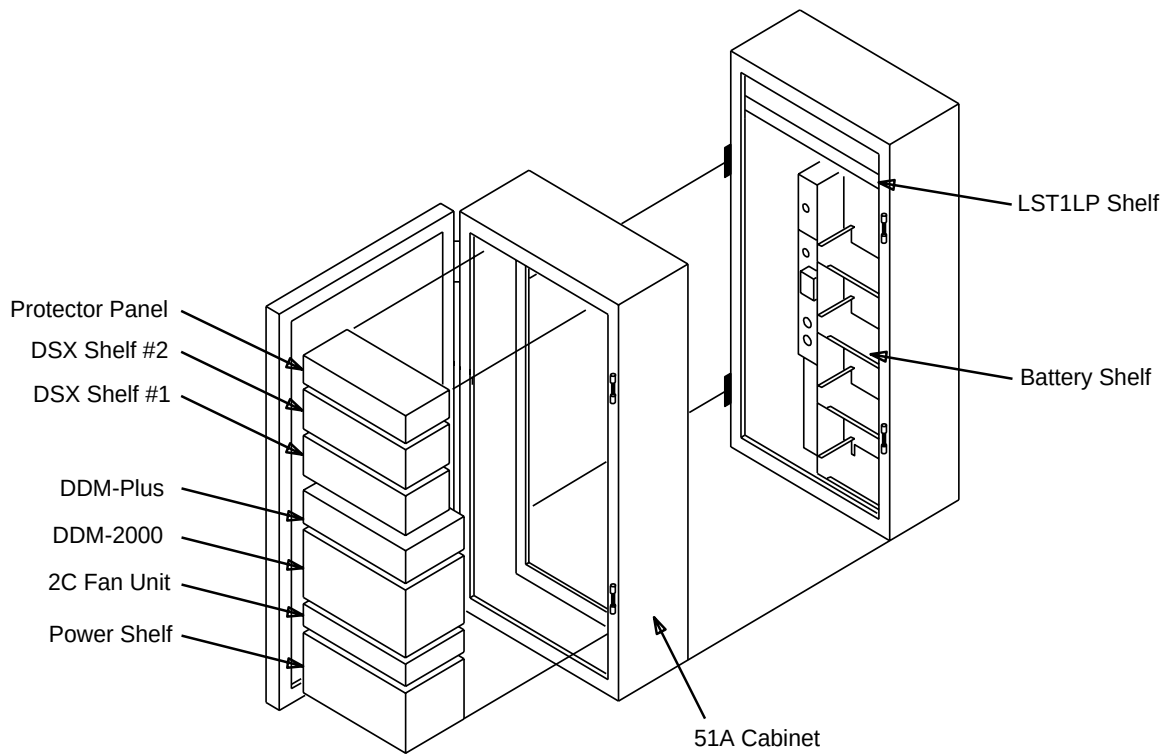
Figure 6-54. 51A Cabinet
