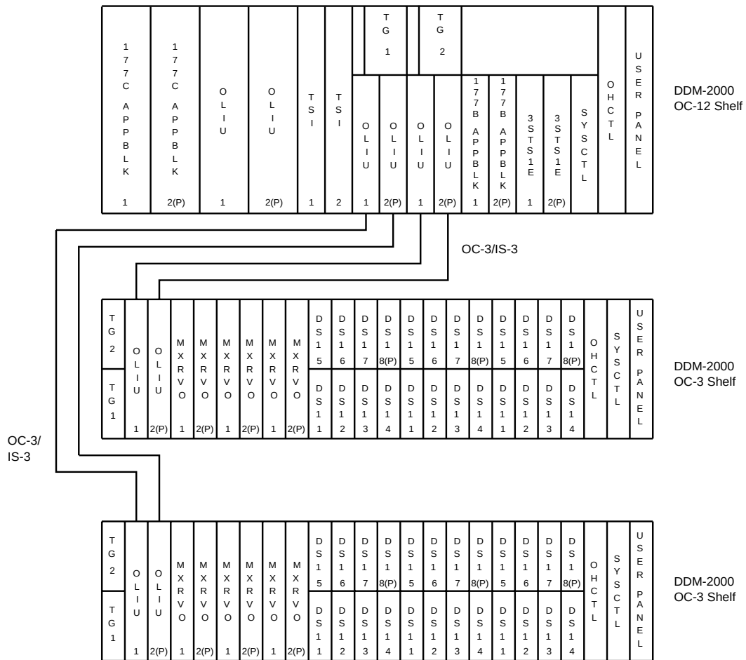
Figure 6-40. OC-12 Terminating Configuration (DS1/EC-1 Low-Speed Interfaces)
