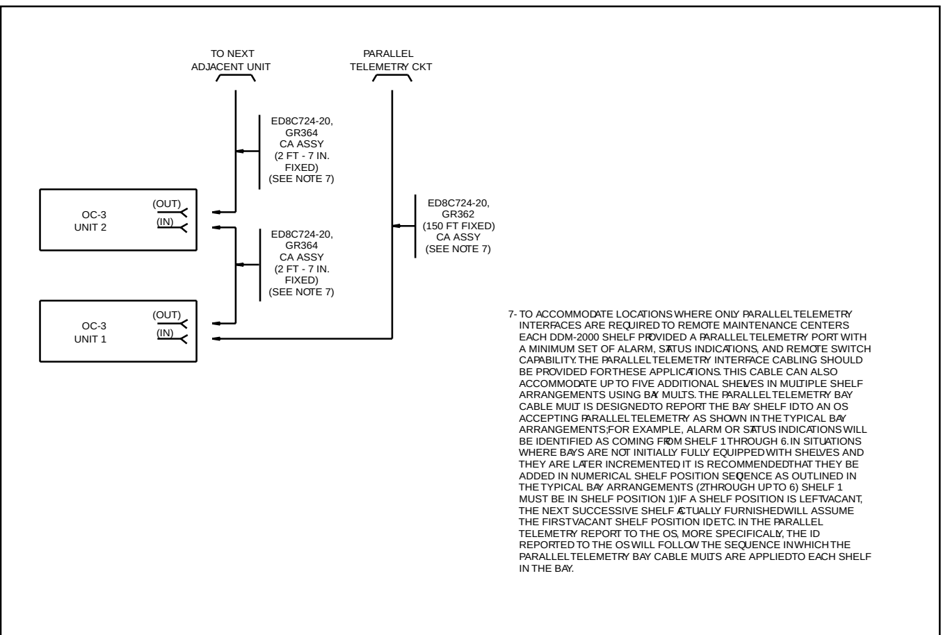
Figure 7-1-10 Parallel Telemetry Interface and Multi Cable
