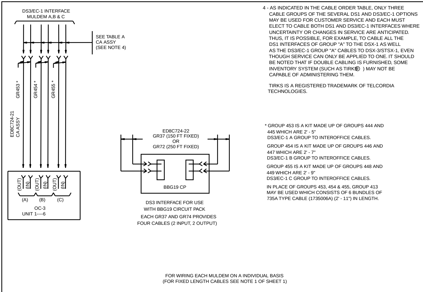
Figure 7-2-5 DS3/EC-1 TRANSMISSION CABLE
