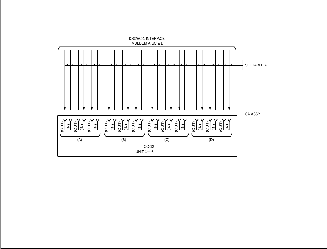
Figure 8-1-2 DS3/EC-1 Transmission Cable
