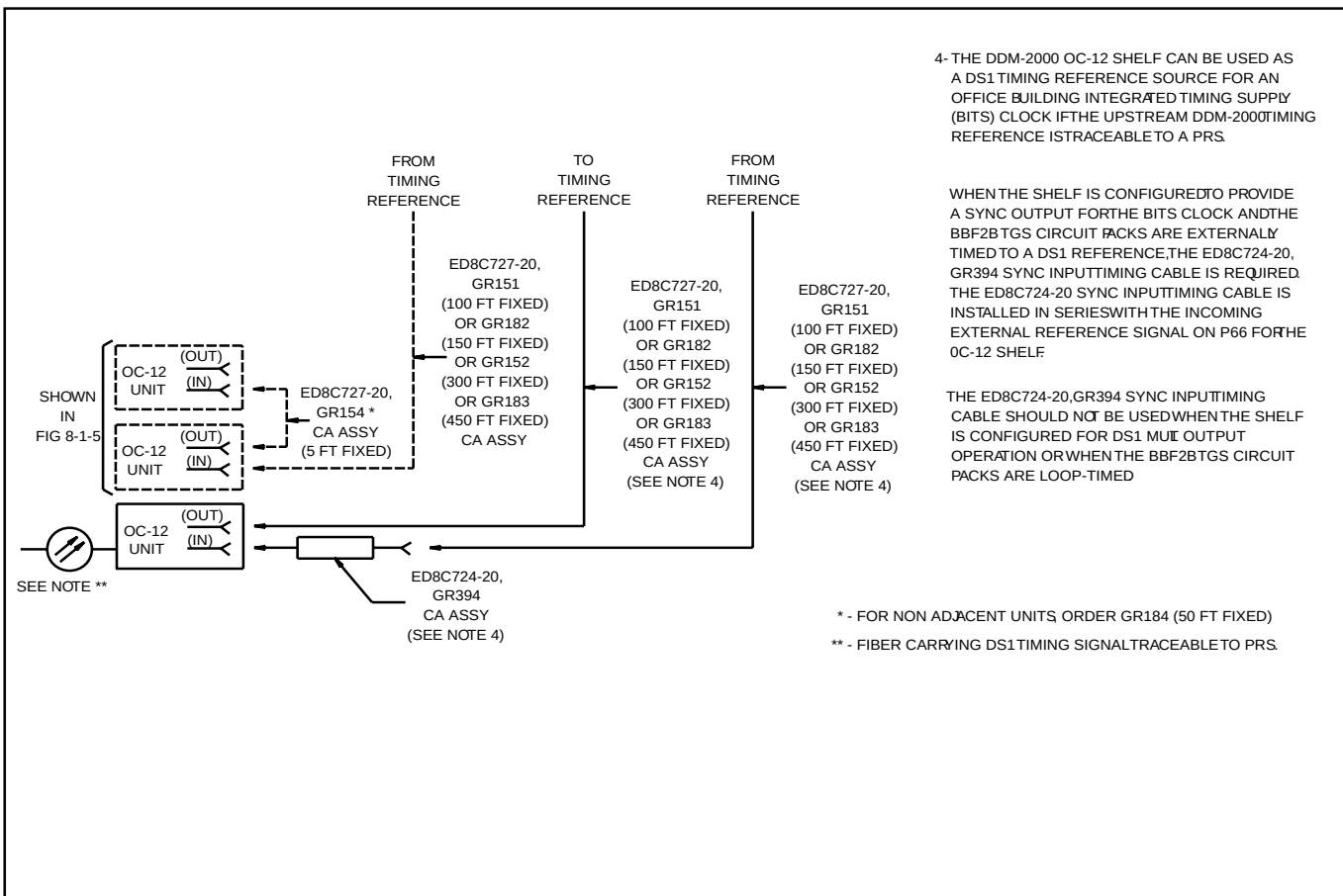
Figure 8-1-5 Synchronization for Timing Distribution Cable in a Bay Arrangement
