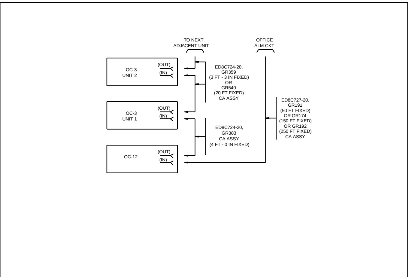
Figure 7-3-10 Office Alarm Interface and Mult Cable
