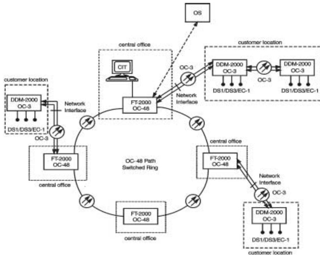
Figure 3-27. OC-3 Services Using Linear Optical Extensions From FT-2000 Ring
