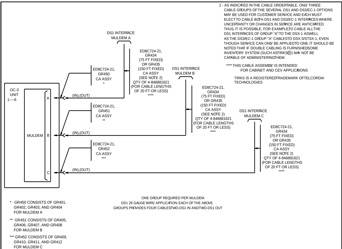
Figure 7-2-2 DS1 Transmission Cables — 26 Gauge
