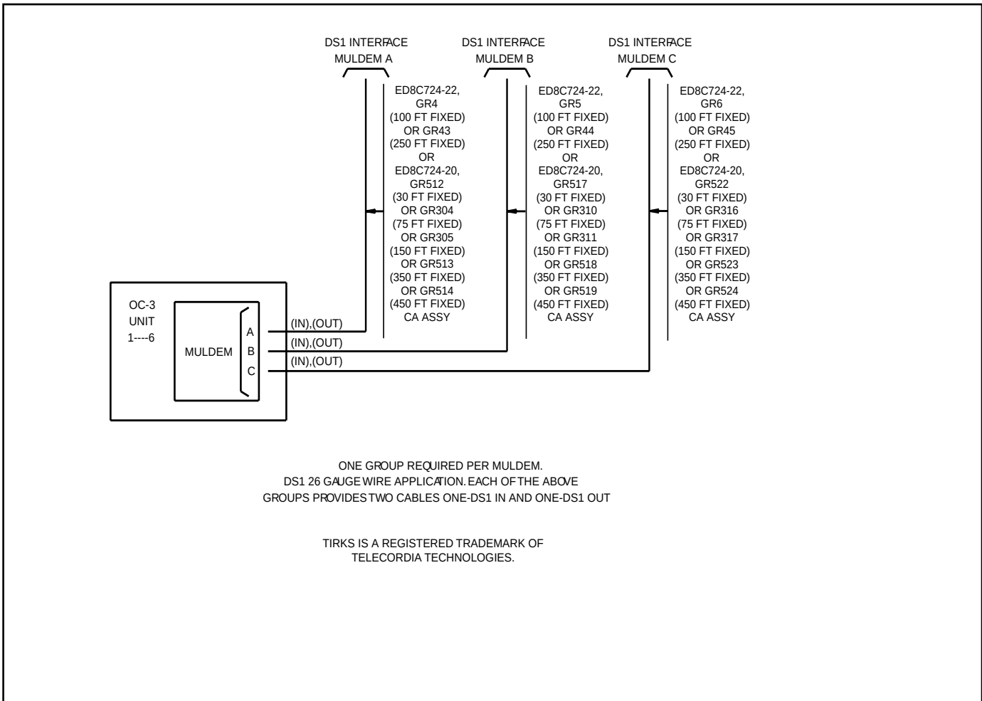
Figure 7-1-2 DS1 Transmission Cables — 26 Gauge
