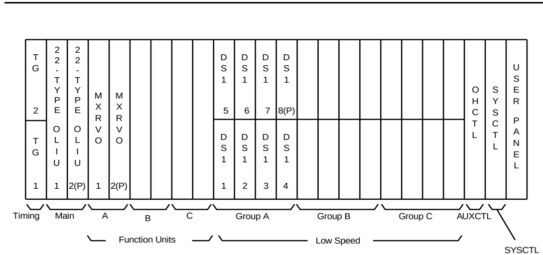
Figure 7-8. Ring Shelf Equipped With 28 DS1 Circuits
