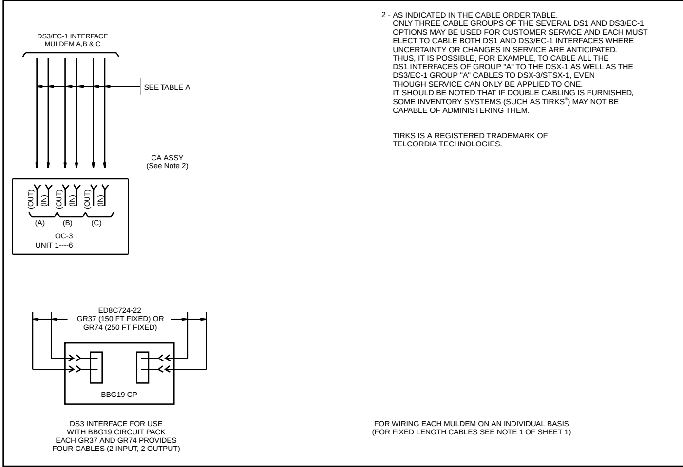
Figure 7-1-5 DS3/EC-1 TRANSMISSION CABLE
