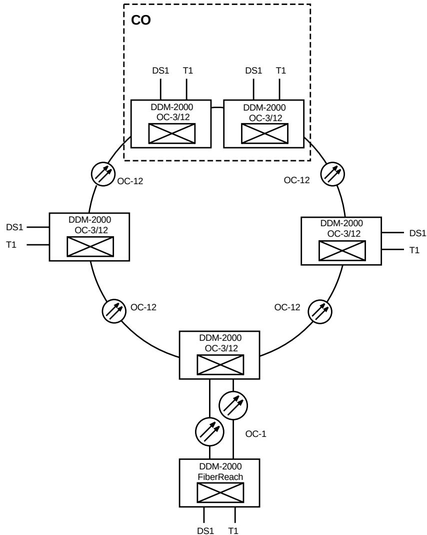
Figure 3-8. OC-12 VT Path Switched Ring Using DDM-2000 OC-3 Multiplexer With OC-12 Optics
