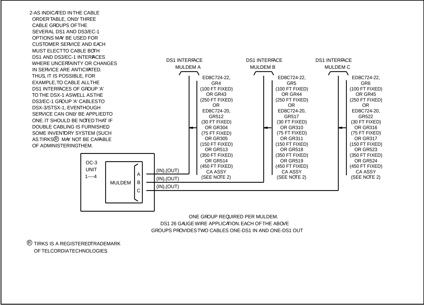
Figure 7-3-2 DS1 Transmission Cables — 26 Gauge
