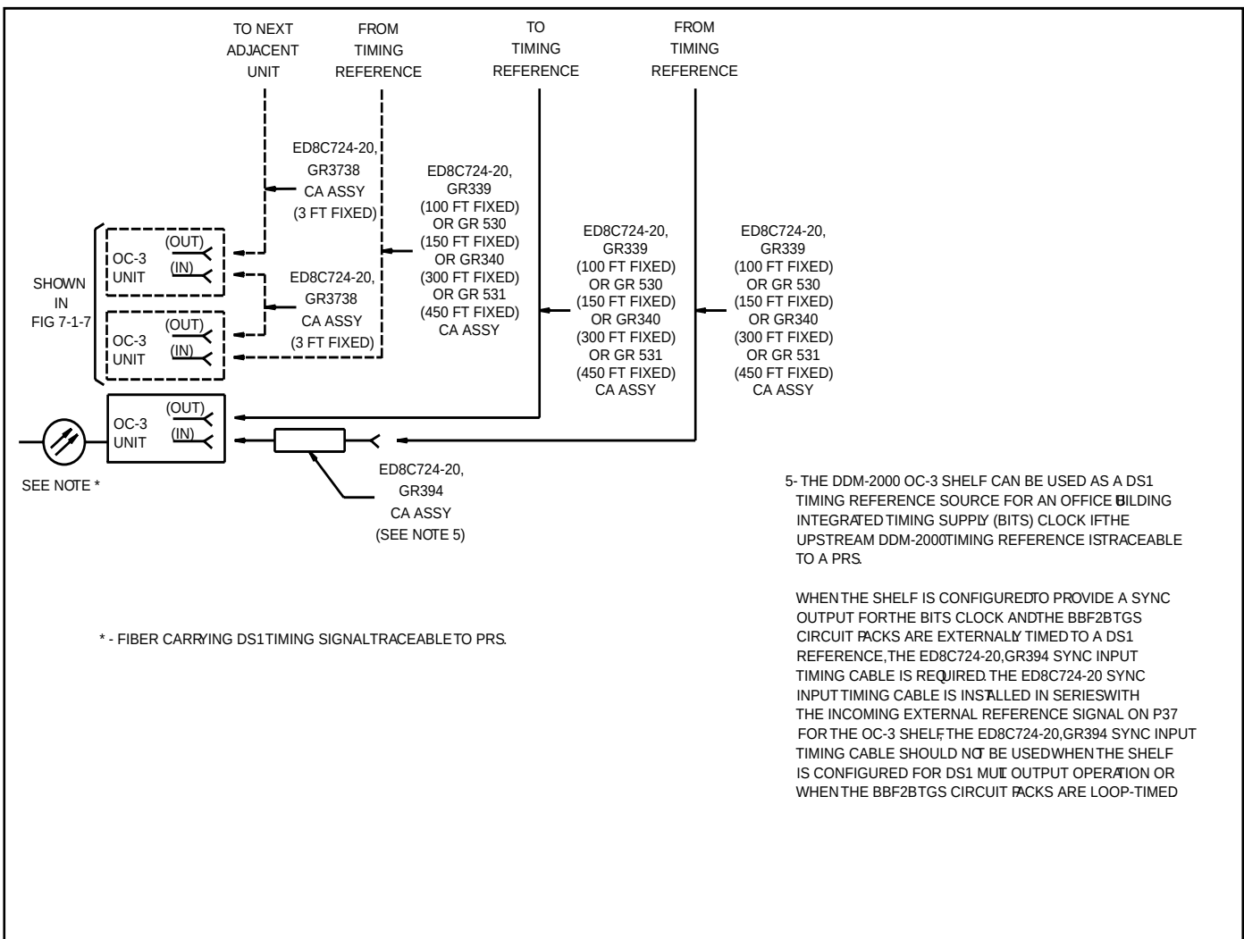
Figure 7-1-7 Synchronization for Timing Distribution Cable in a Bay Arrangement
