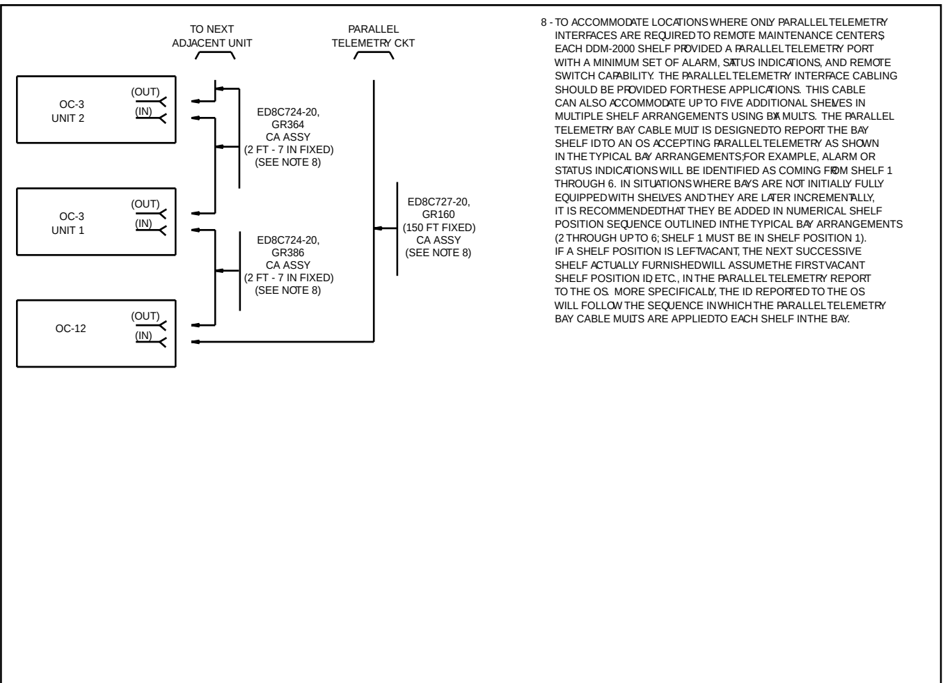
Figure 7-3-11 Parallel Telemetry Interface and Mult Cable
