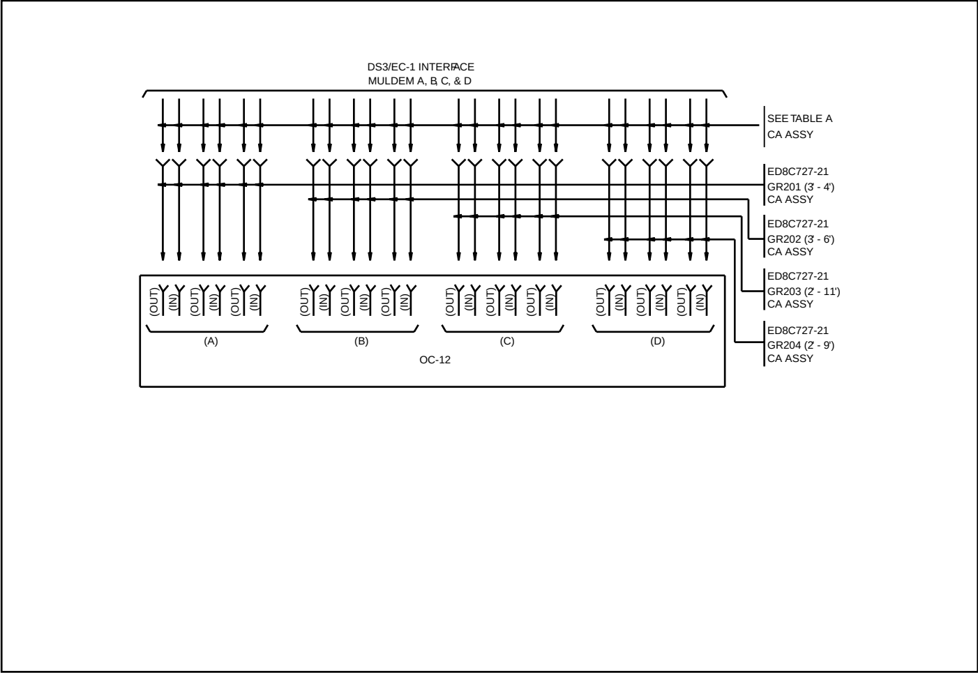
Figure 7-4-4 DS3/EC-1 Transmission Cable
