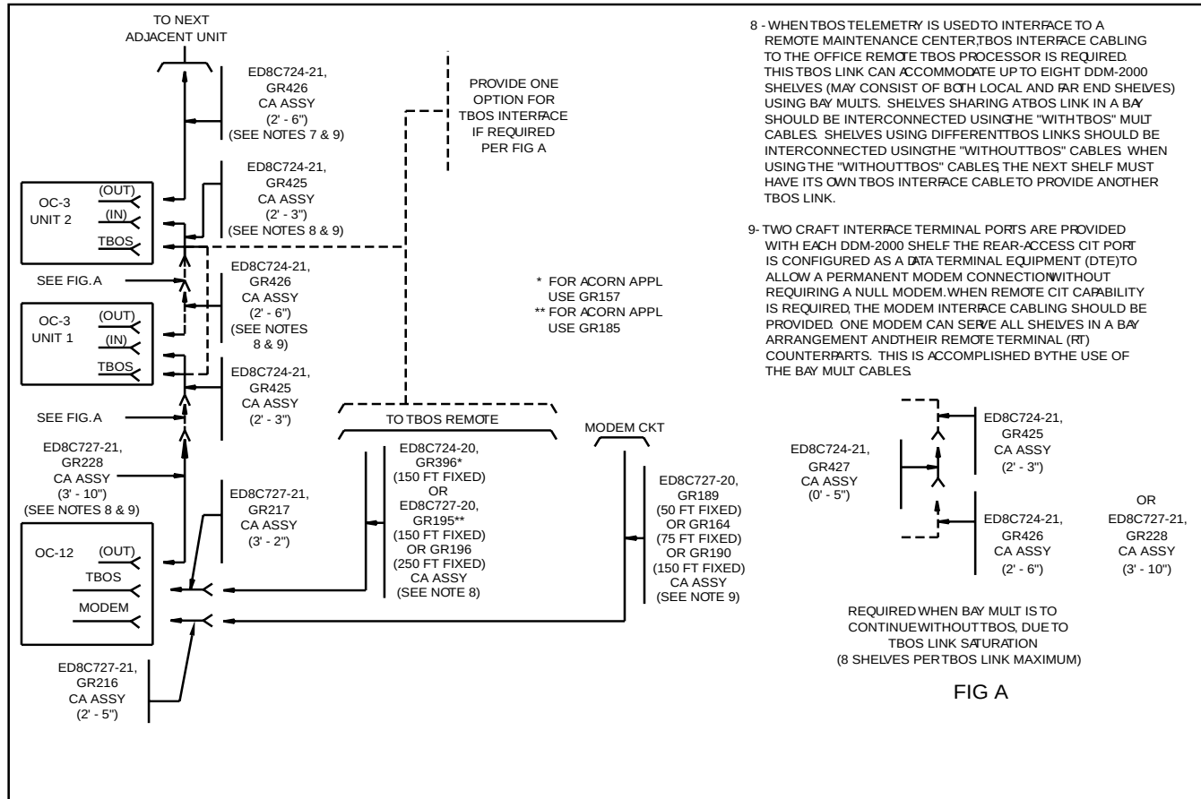
Figure 7-4-12 Modem, TBOS Interface, and Bay Mult Cable for TBOS, CIT, and Modem
