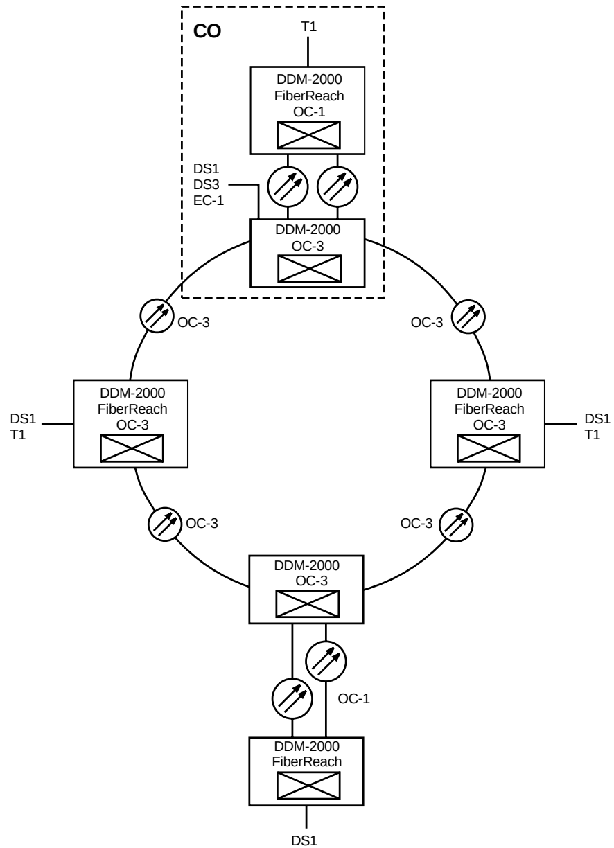
Figure 3-4. OC-3 Path Switched Ring Using OC-3 Multiplexer and FiberReach Multiplexer With OC-3 Optics
