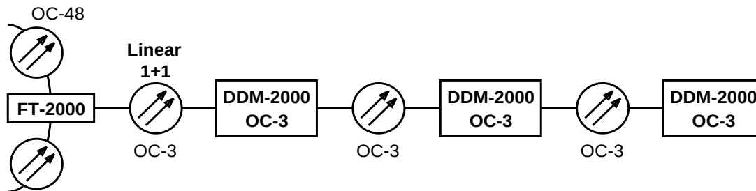
Figure 3-57. OC-3 Linear Interfaces with FT-2000 OC-48 Lightwave System
