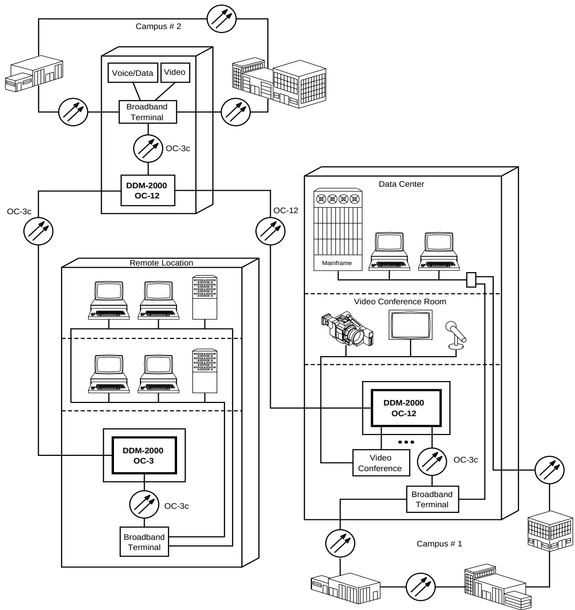
Figure 3-47. OC-3c Transport— Private Data/Video/ATM Network Application
