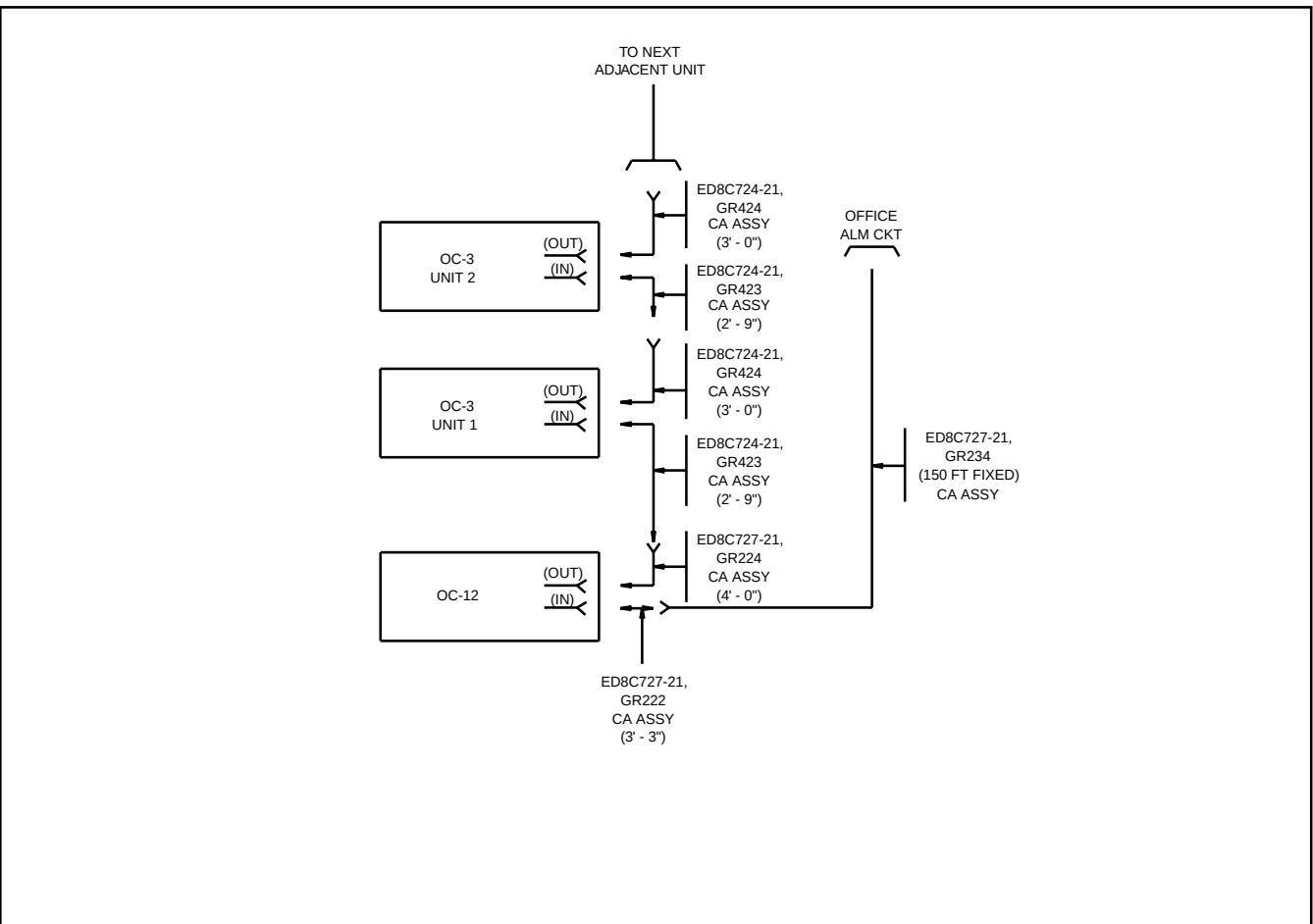
Figure 7-4-10 Office Alarm Interface and Mult Cable
