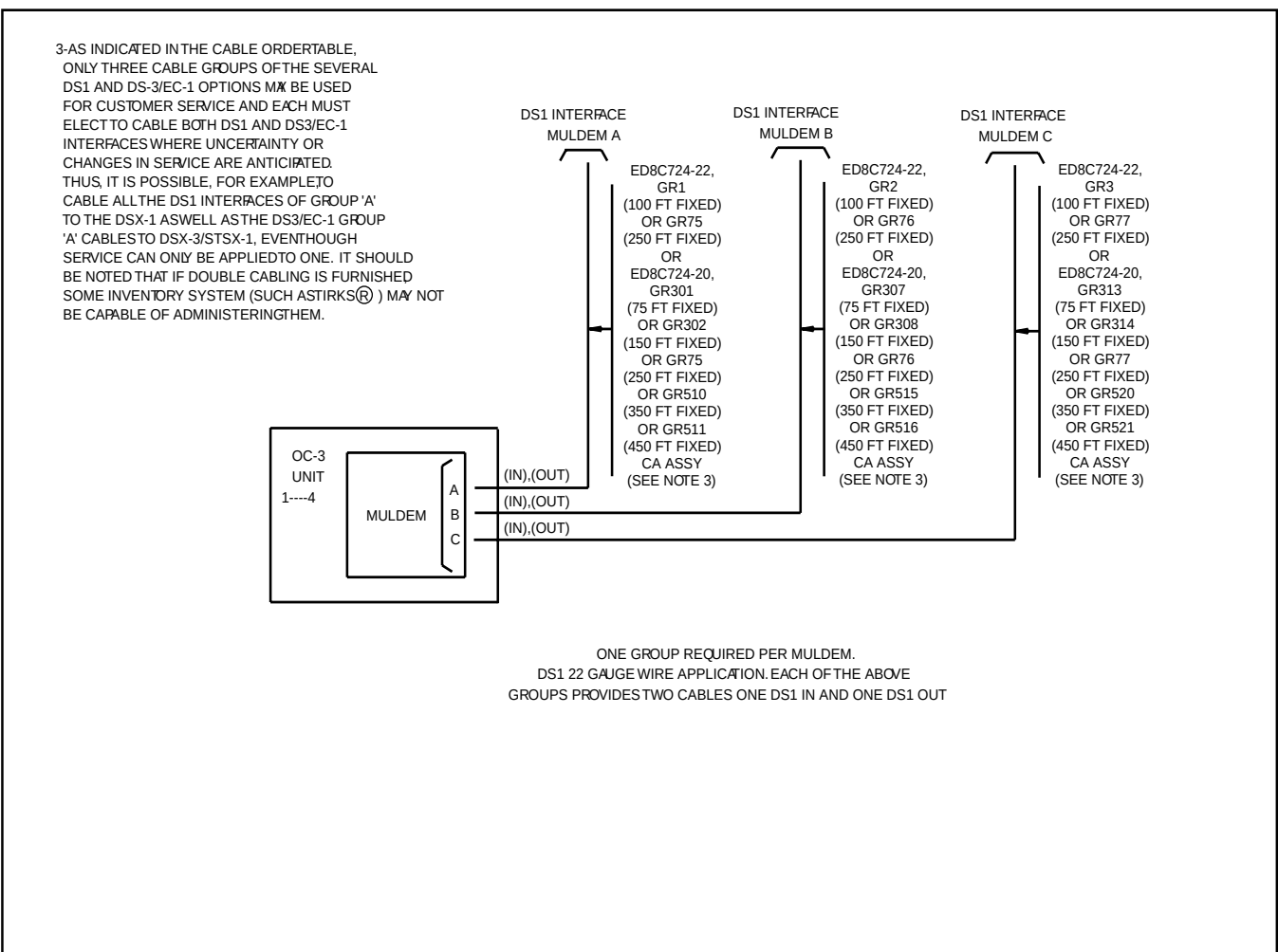
Figure 7-3-3 DS1 Transmission Cables — 22 Gauge
