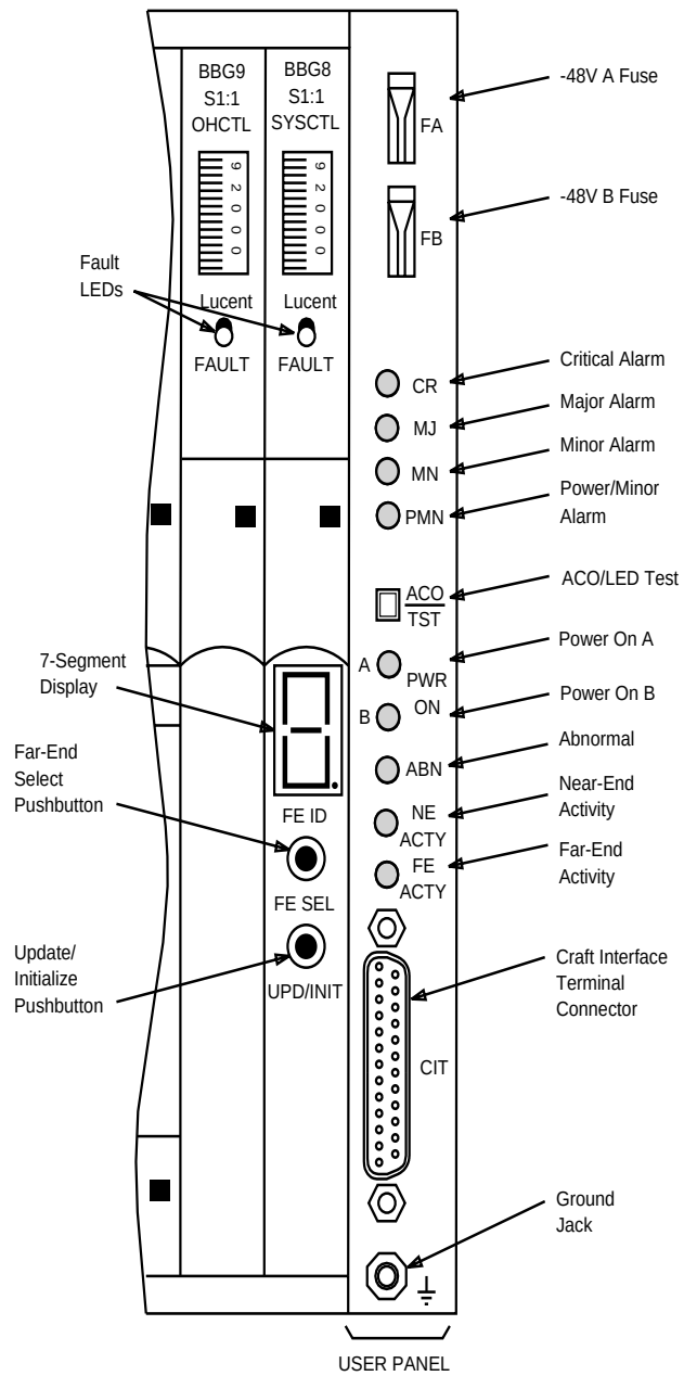
Figure 5-3. DDM-2000 OC-3 User Panel for Group 4 Shelves
