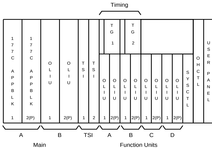
Figure 6-41. OC-12 Hub Shelf
