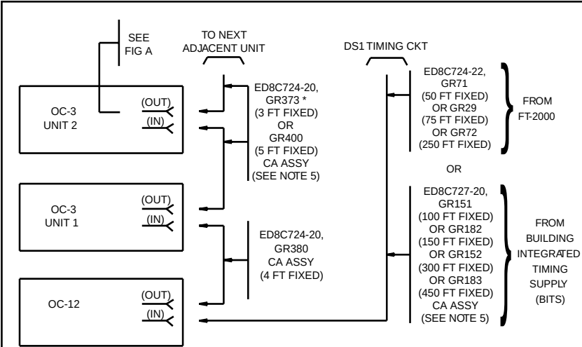
Figure 7-3-8 DS1 Timing Reference Interface and Mult Cable
