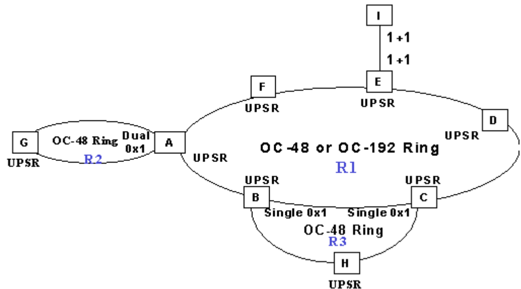
Figure 5-13 Dual homed subtending ring example
