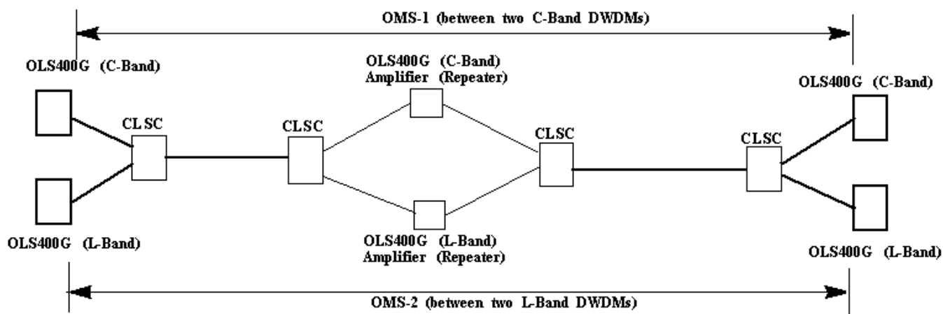
Figure 5-3 OMS provisioning between pairs of C-Band and L-Band DWDMs
