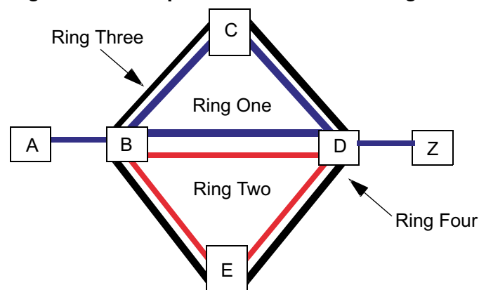
Figure 2-3 Sample formation of four rings
