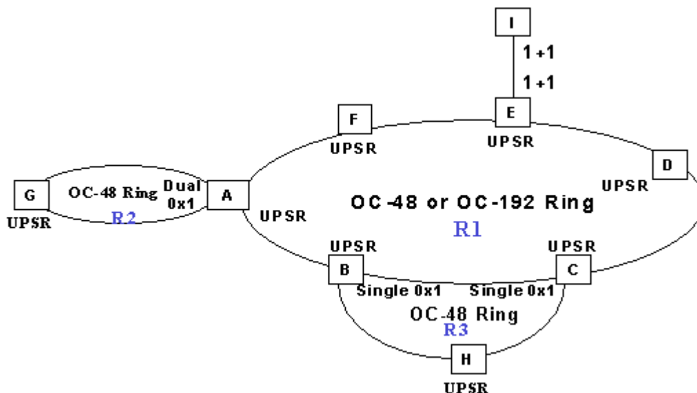
Figure 5-12 Single homed subtending ring example
