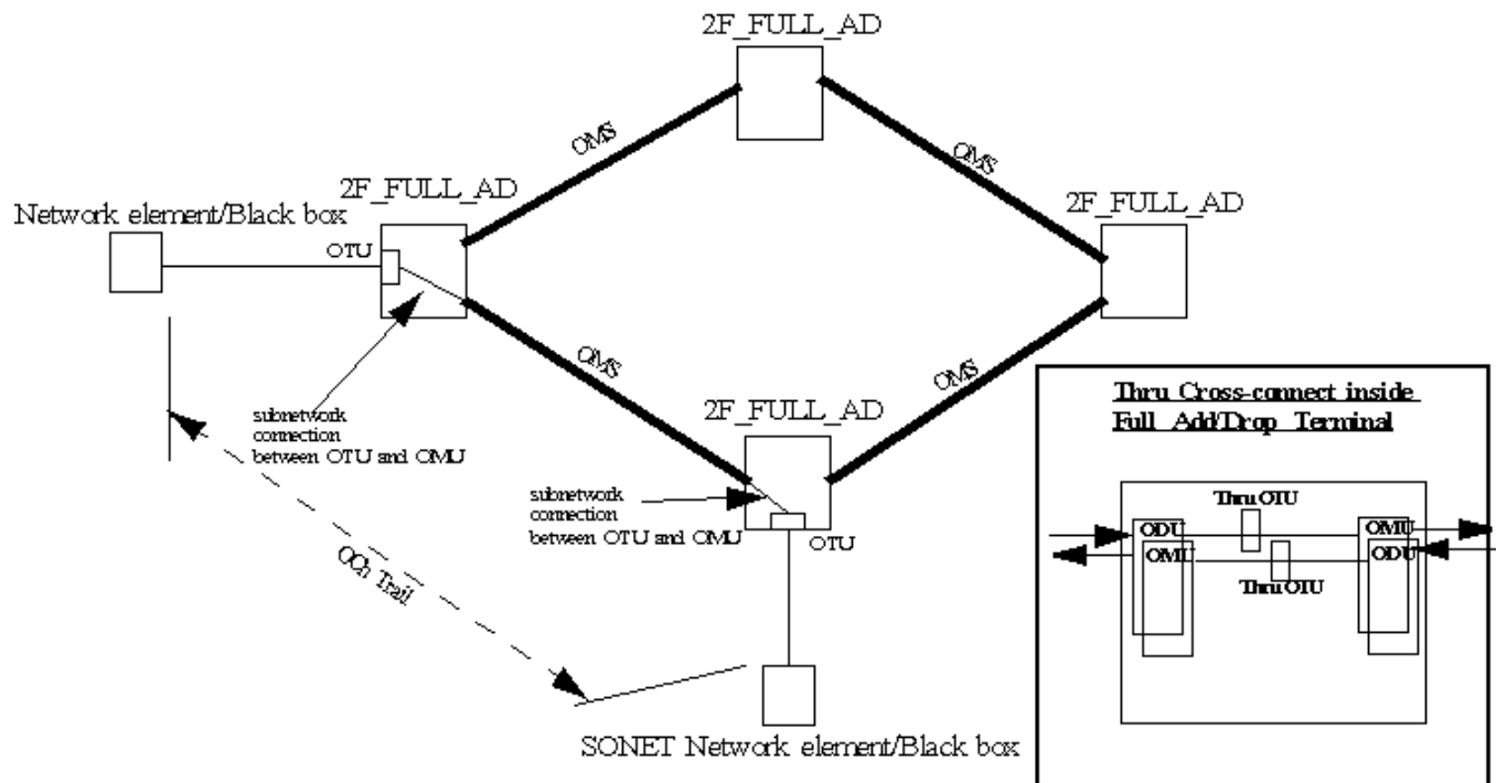
Figure 5-5 OCh trail terminating on the full add/drop (ring) terminal
