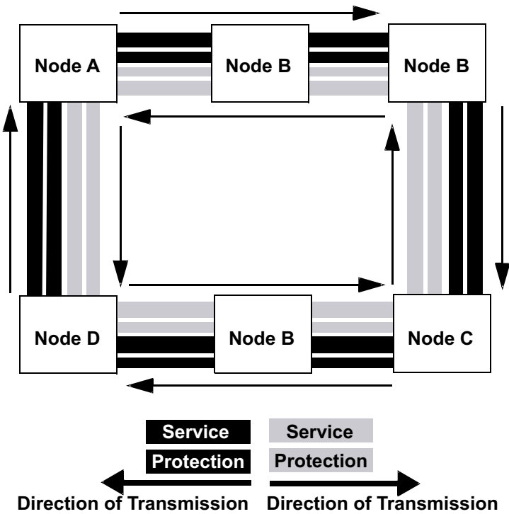
Figure 5-10 Four-Fiber BLSR
