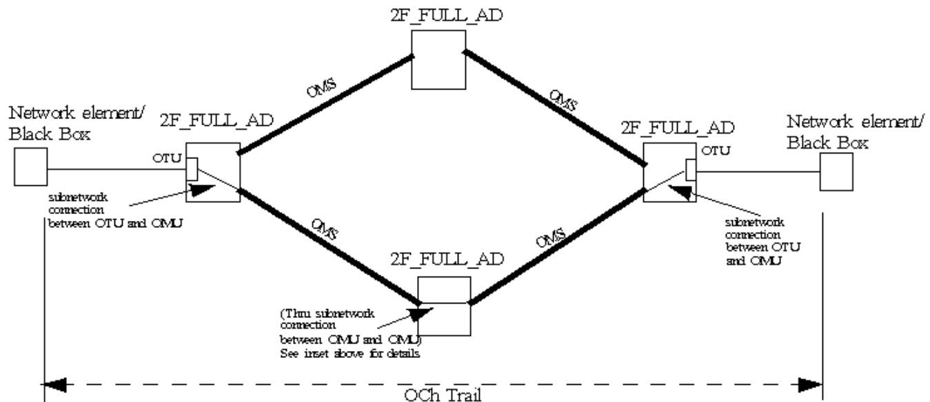
Figure 5-6 OCh trail passing the intermediate full add/drop (ring) terminal
