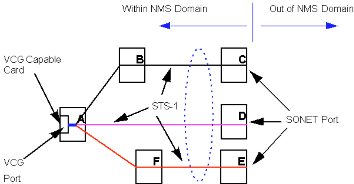
Figure 5-17 Members of a single-ended VCG
