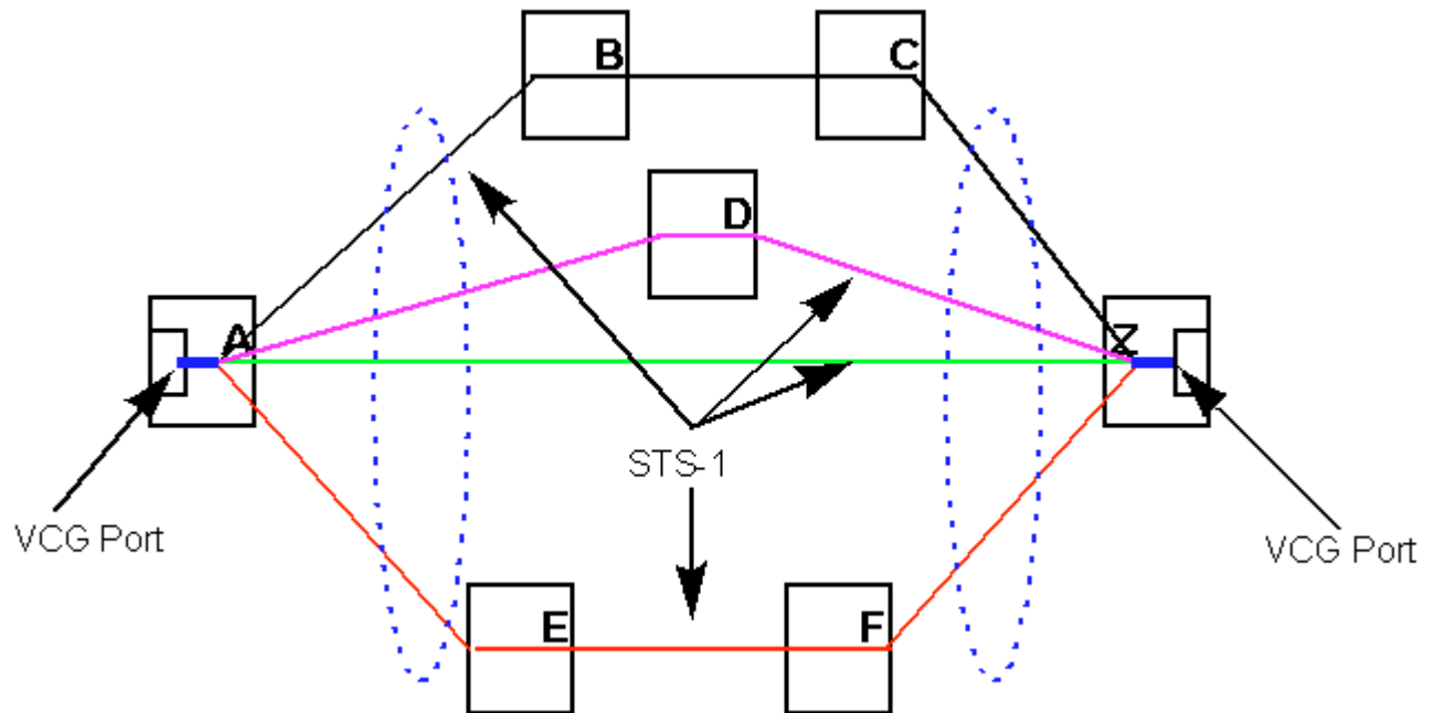
Figure 5-19 Members of a dual-ended VCG
