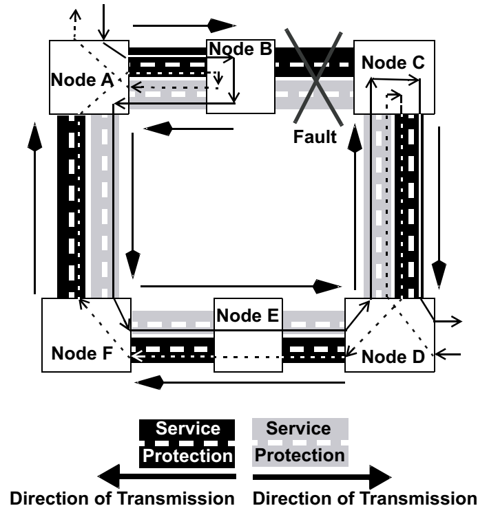
Figure 5-9 Two-Fiber BLSR with Fault
