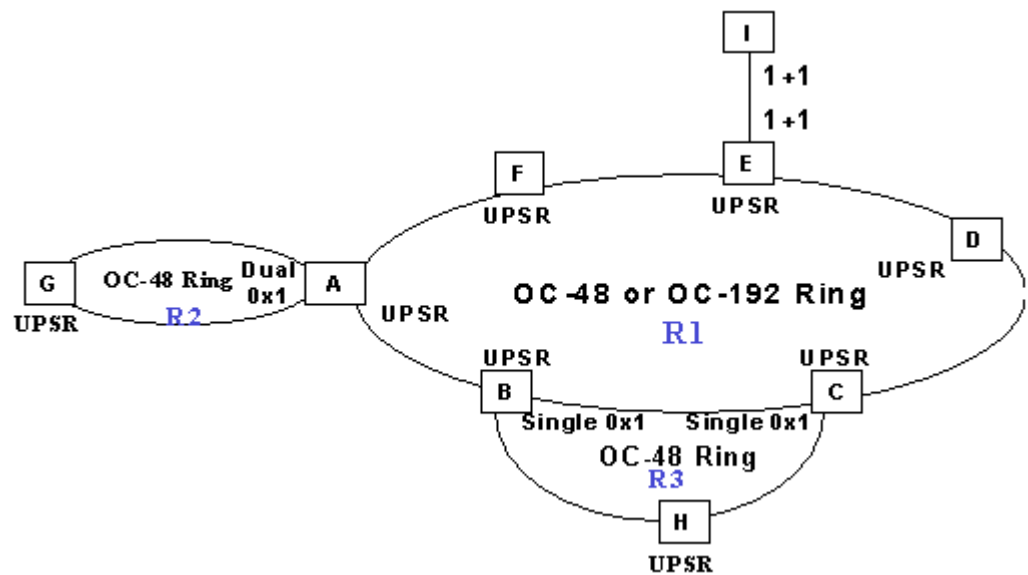
Figure 5-11 A typical Metropolis DMX and Metropolis DMXpress ring topology
