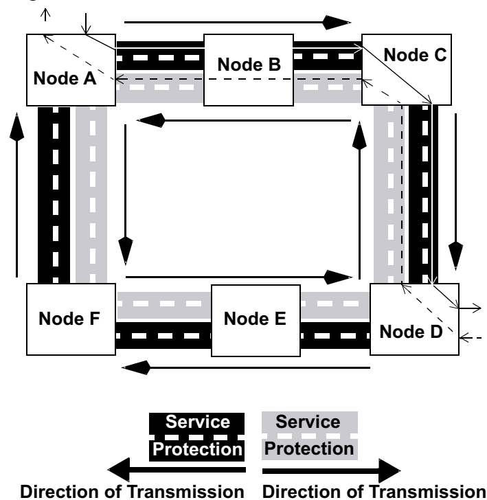
Figure 5-8 Two-Fiber BLSR
