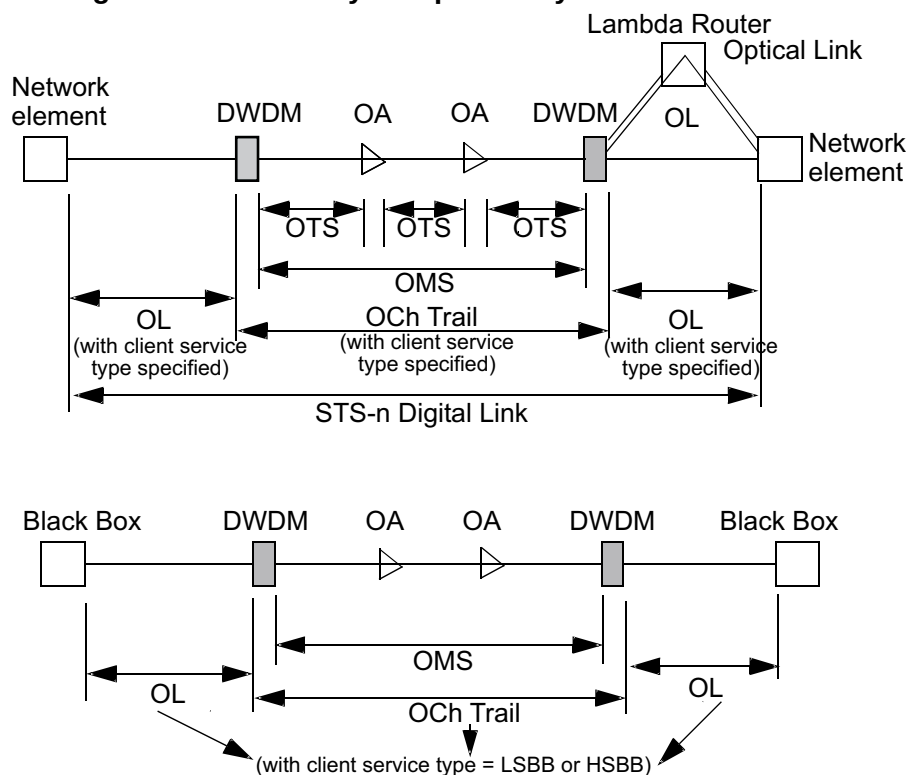
Figure 5-2 Hierarchy of Optical Layers
