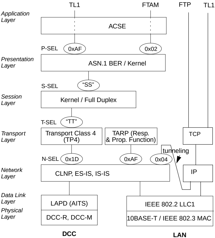
Figure 2-8 The network element stack profile
