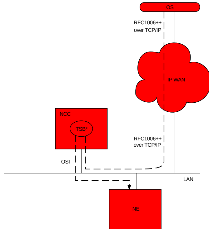
Figure 2-6 OS communication over RFC1006++ through the NCC to the NE
