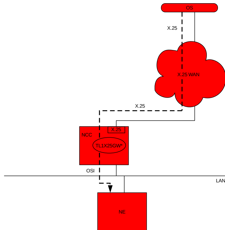
Figure 2-4 OS communication over X.25 through the NCC to the NE
