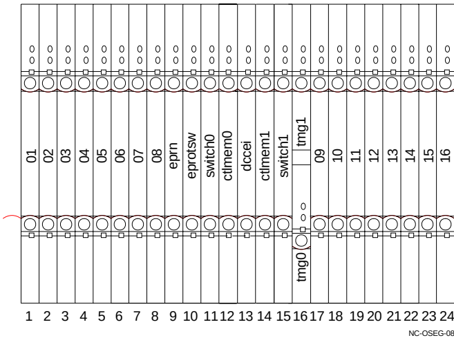
Figure A-1 Slot names in the WaveStar® TDM 2.5G (OC-48) Shelf
