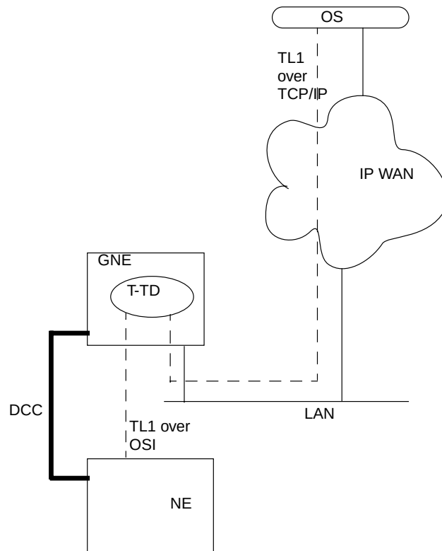
Figure 2-2 OS Communication (TL1) over IP through the GNE to the NE
