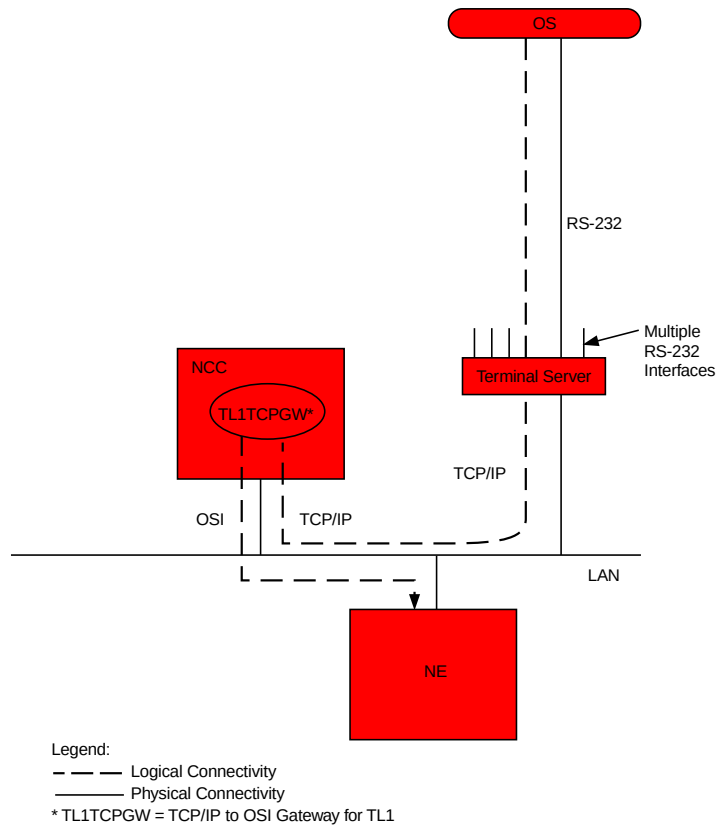
Figure 2-7 OS communication over RS-232 through the NCC to the NE
