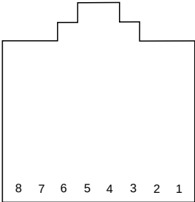
Figure 2-10 RJ45 connector
