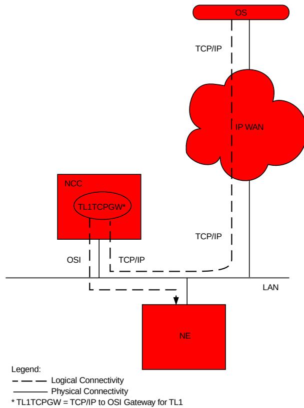
Figure 2-5 OS communication over TCP/IP through the NCC to the NE
