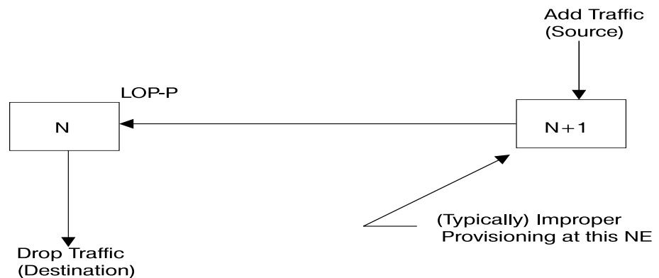
Figure 512-1 Example of a network that is indicating an LOP-P alarm
