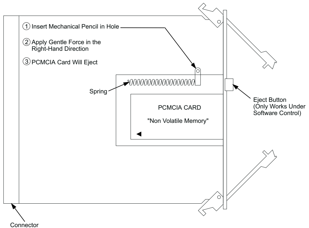
Figure 544-1 SYS50DM with PCMCIA Card Inserted
