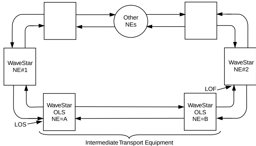
Figures Figure 545-2 Near-End and Far-End NEs with Intermediate Transport Equipment
