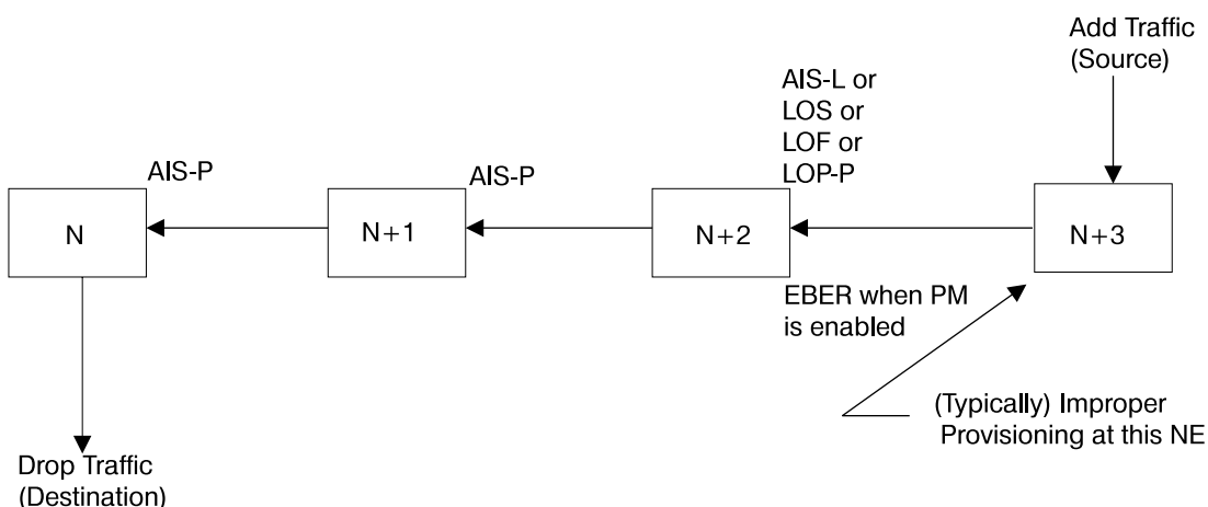
Figure 512-1 Example of a network that is indicating an AIS-P alarm
