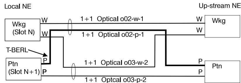
Example (a): 1+1 With OC-12 Circuit Pack
