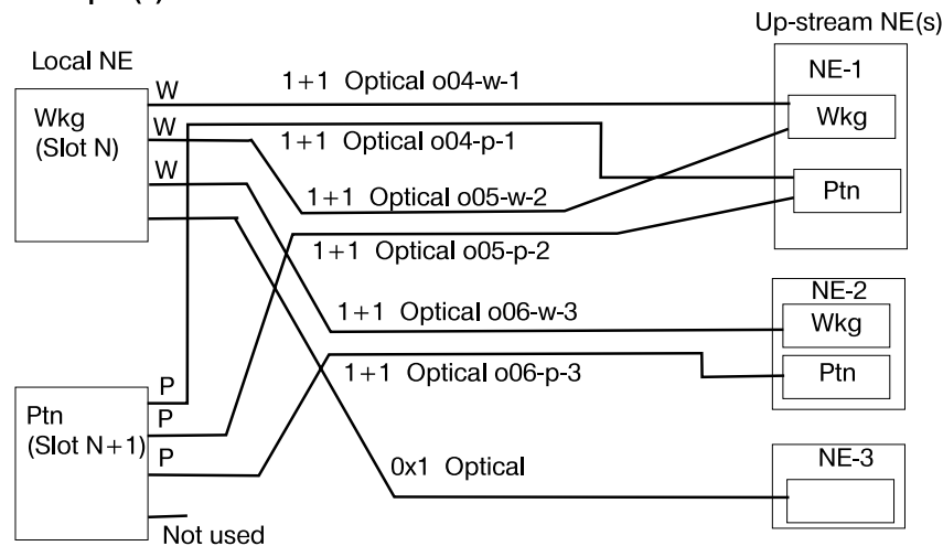
Example (a): 1+1 With OC-12 Circuit Pack
