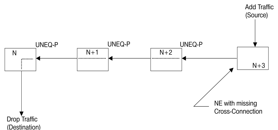
Figure 512-4 Currently no provisioned cross-connection
