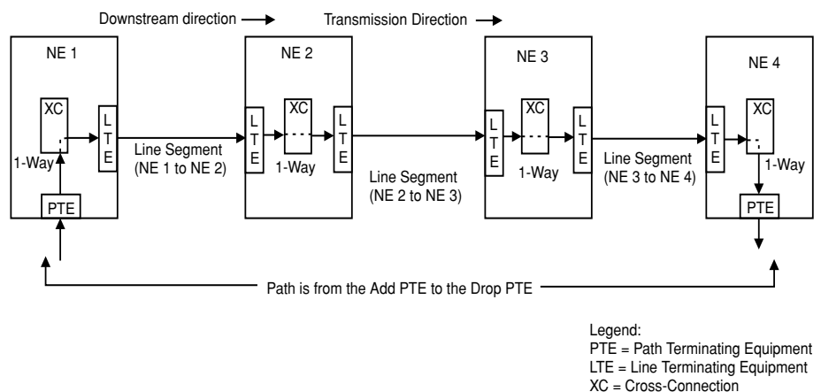
Figure 512-1 Path vs Line Differences
