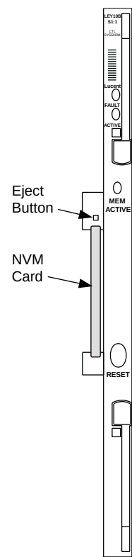
Figure 702-4 Front/Faceplate View of the SYS50DM Circuit Pack
