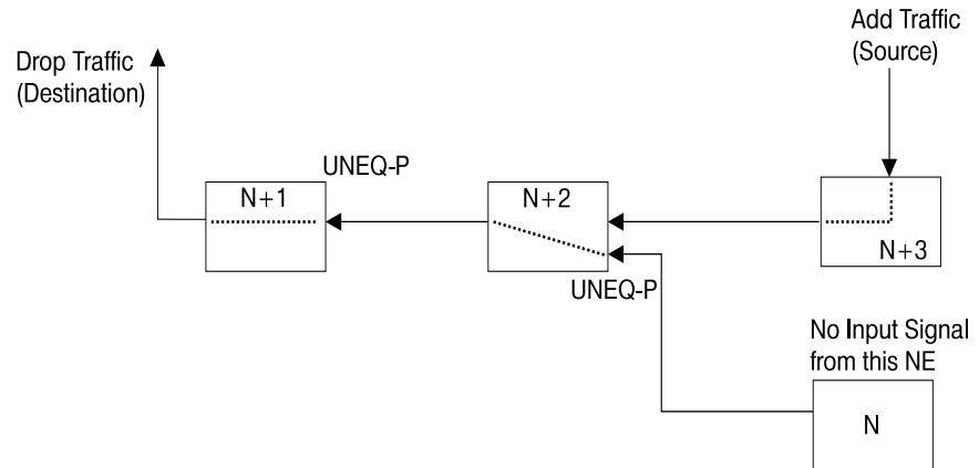
Figure 512-5 Improperly provisioned cross-connection
