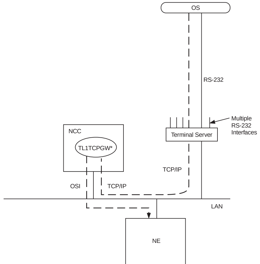
Figure 2-7 OS communication over RS-232 through the NCC to the NE
