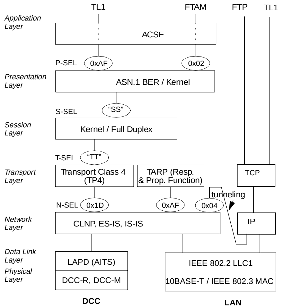
Figure 2-8 The network element stack profile
