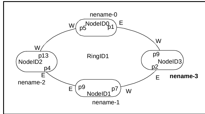
Figure 2. Ring Map for Closed Ring at nename-3
