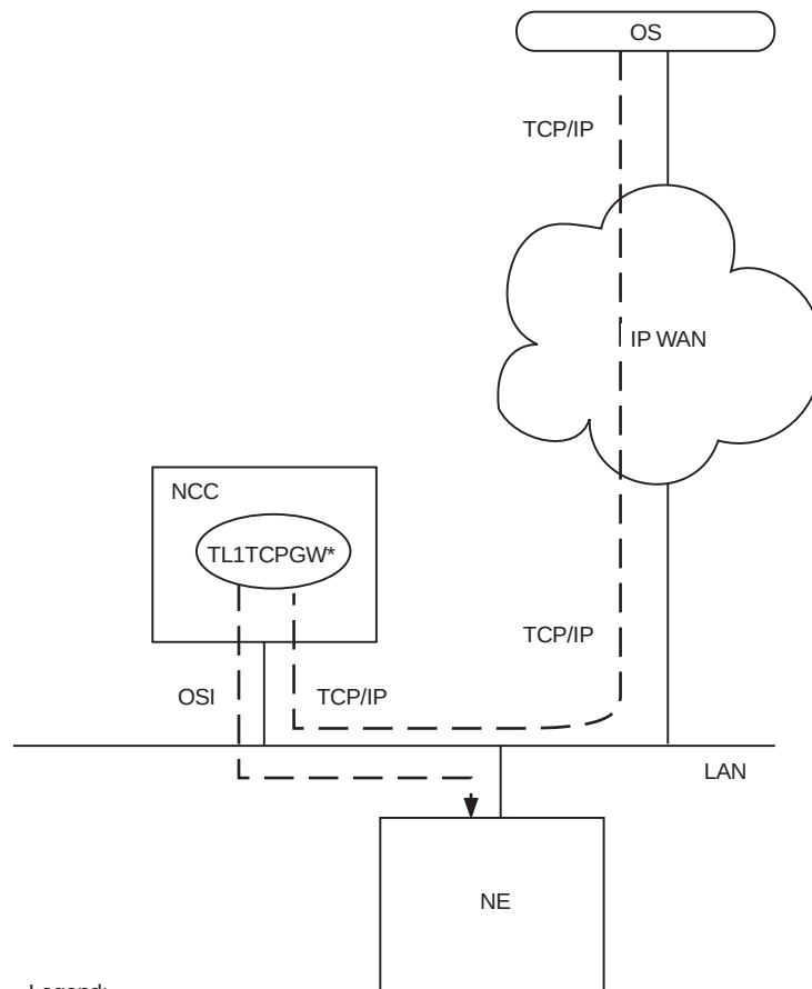
Figure 2-5 OS communication over TCP/IP through the NCC to the NE
