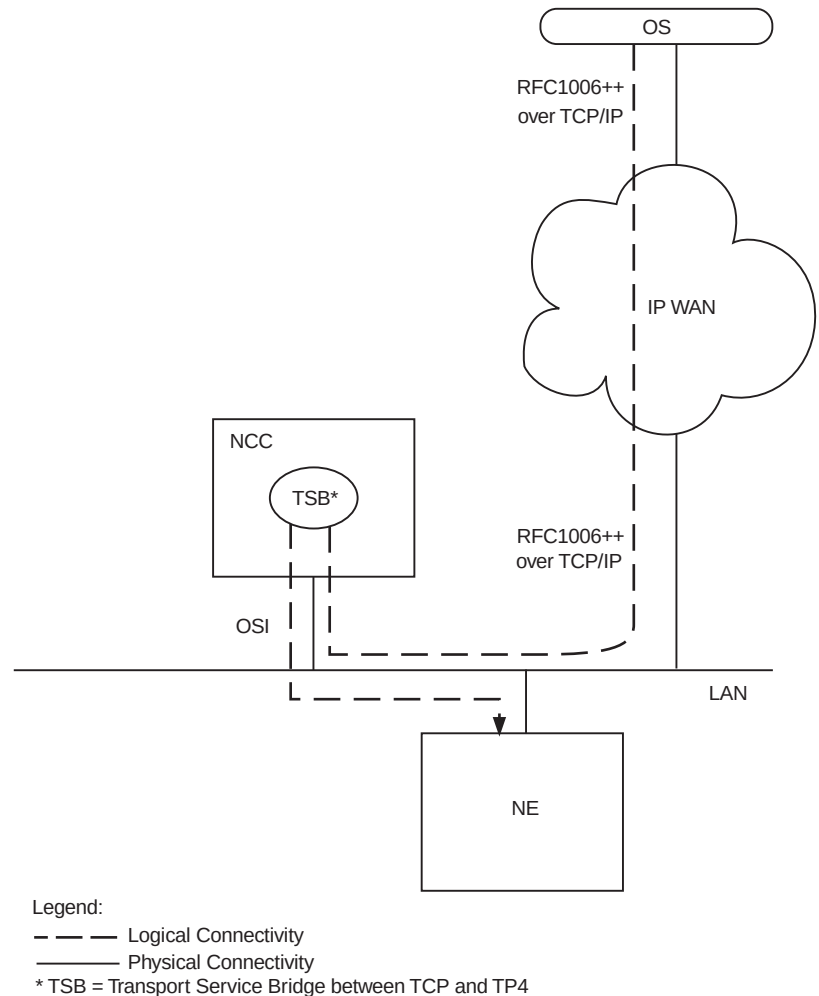
Figure 2-6 OS communication over RFC1006++ through the NCC to the NE
