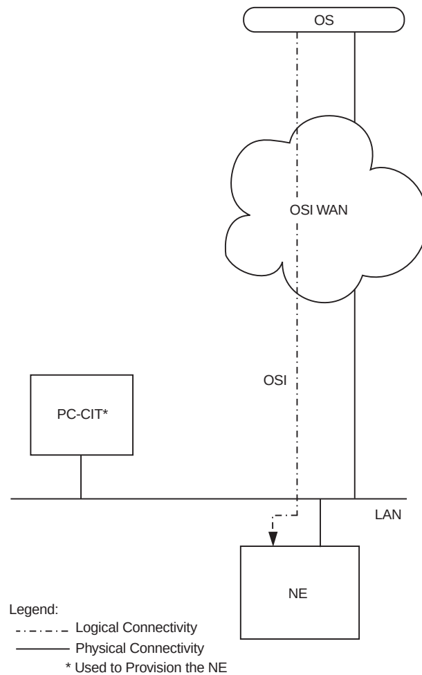
Figure 2-1 OS Communication over OSI Directly for OS Management of an NE
