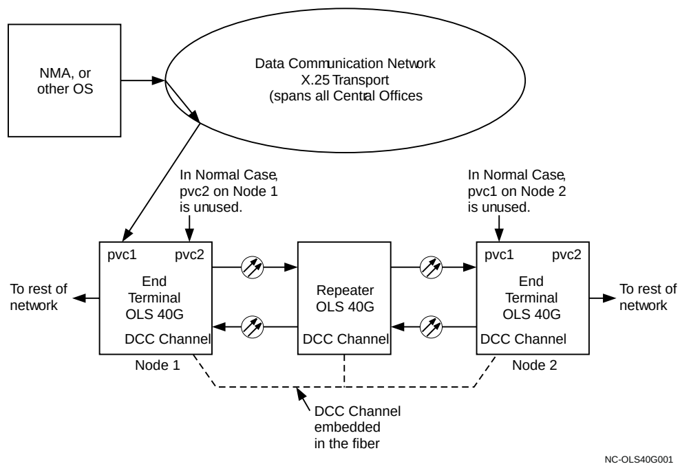
Figure 2-1. Normal Case - No Failure, No Redirect
