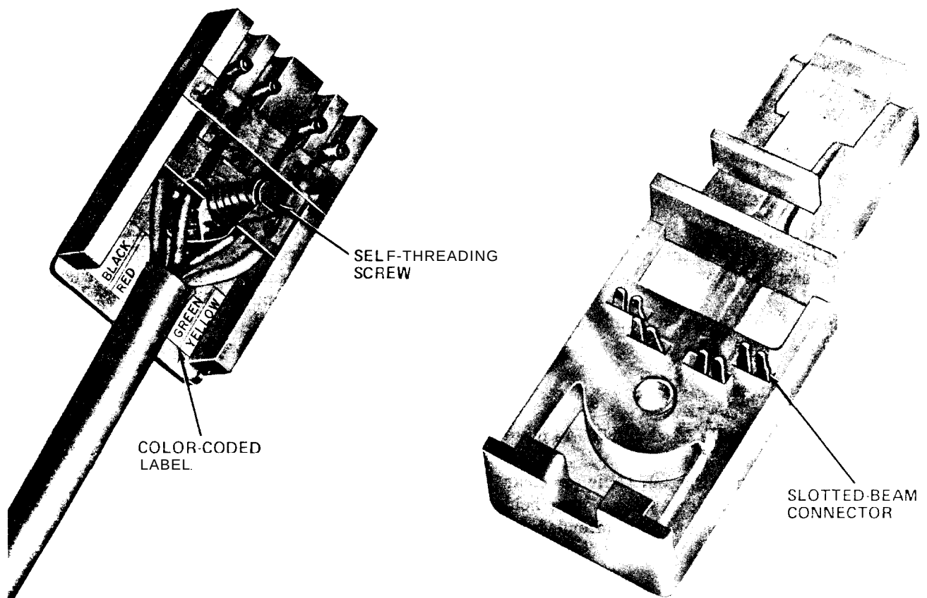
Fig. 27.1 — 700A4 Plug With Conductors Terminated
