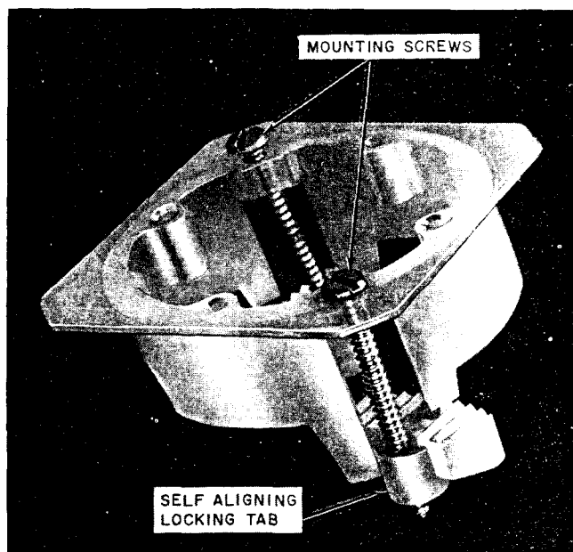
Fig. 1—KS-20502, List 2 Mounting Bracket
