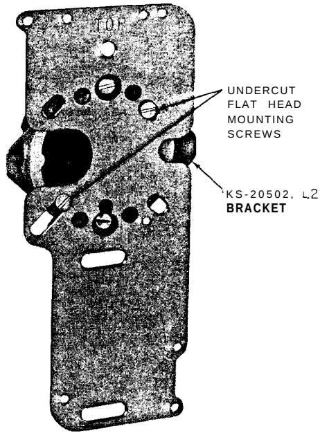
Fig. 4→155A Adapter Mounted on a KS-20502, list 2 Bracket
