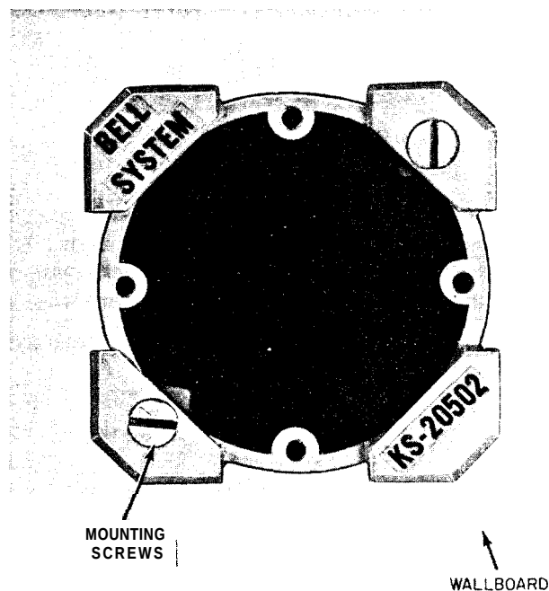
Fig. 2-KS-20502, list 1 (MD) Bracket, Mounted in a 2-1/4 Inch Hole (Front View)
