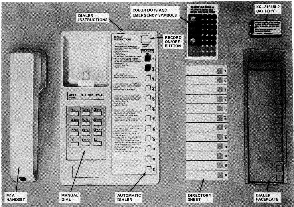
Fig. 2—5011T01A Telephone Set With Handset, Dialer Faceplate, Director Sheet, and Battery Removed
