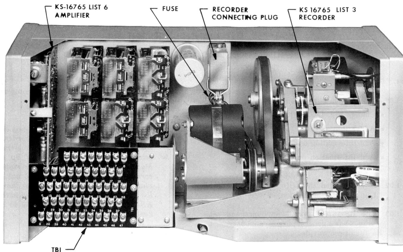
Fig. 2A — KS-16765, List Announcement Set (Front Cover Removed)
