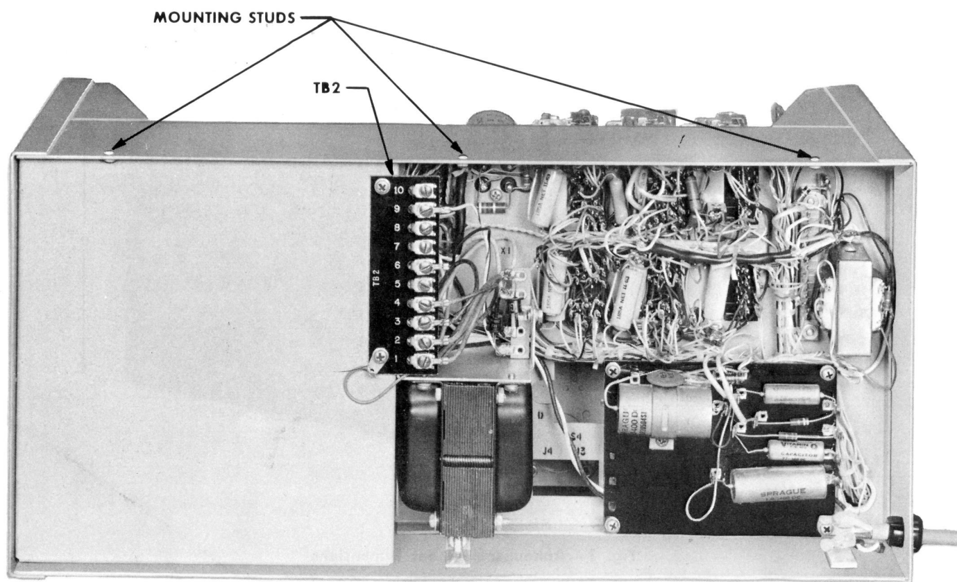
Fig. 2B — KS-16765, List 1 Announcement Set (Rear Cover Removed)
