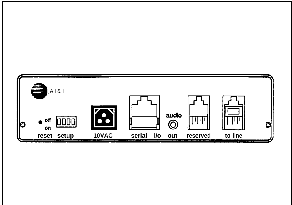
FIGURE 1-3 Back View of the SPIRIT Attendant.
