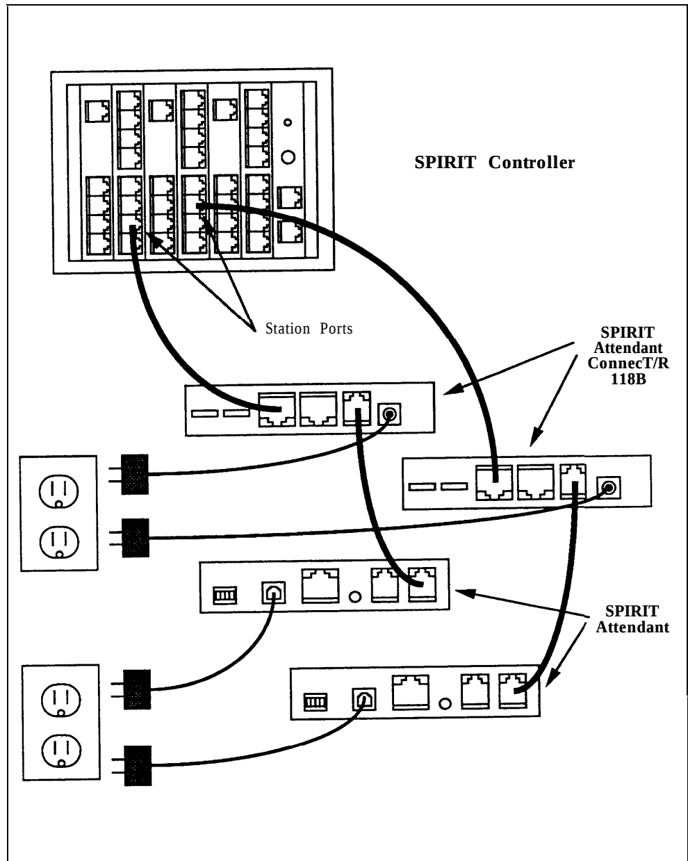
FIGURE 1-4. Connecting two SPIRIT Attendants.
