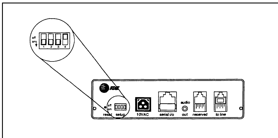
FIGURE 1-3. Setup Switch Positions for Installing Unit.
