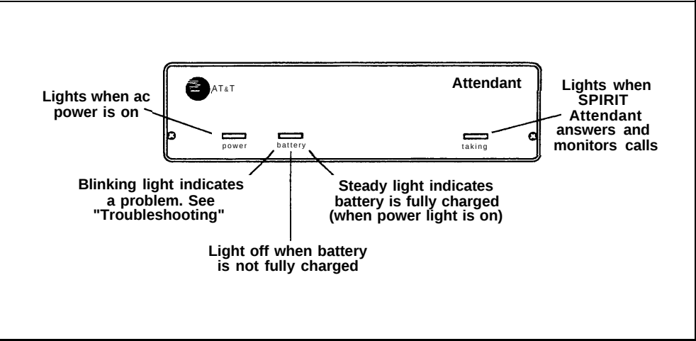
FIGURE 1-1. Front View of the SPIRIT Attendant.
