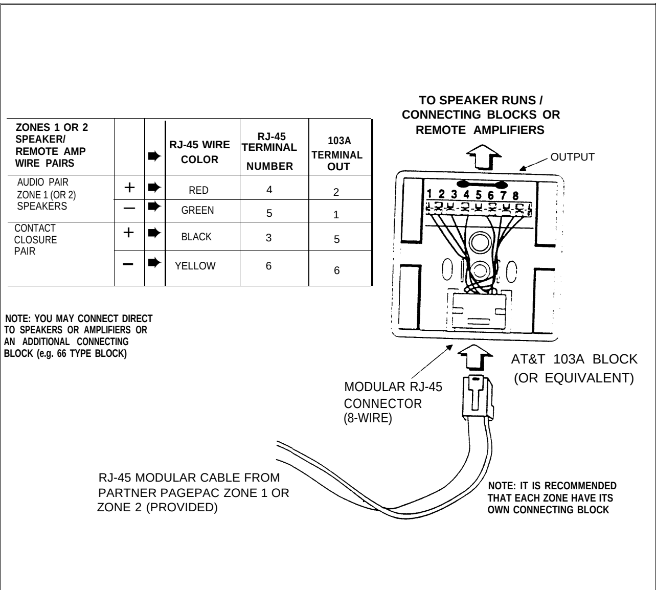
Figure 3-3 Example Speaker / Remote Amplifier Connection Block Wiring
