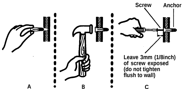
Figure 2. Inserting Anchors and Screws
