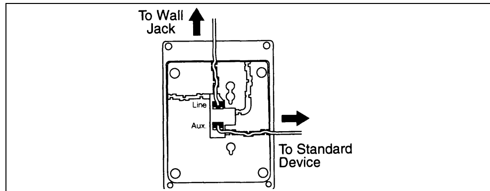
Figure 2. Combination Extension Using Direct Connection
