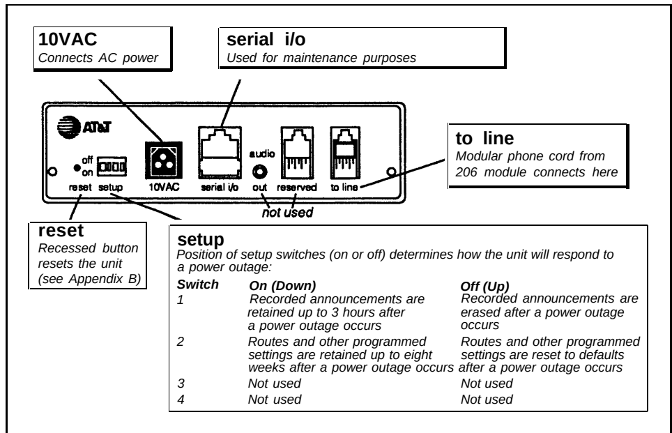
Figure 2-2 BackPanel
