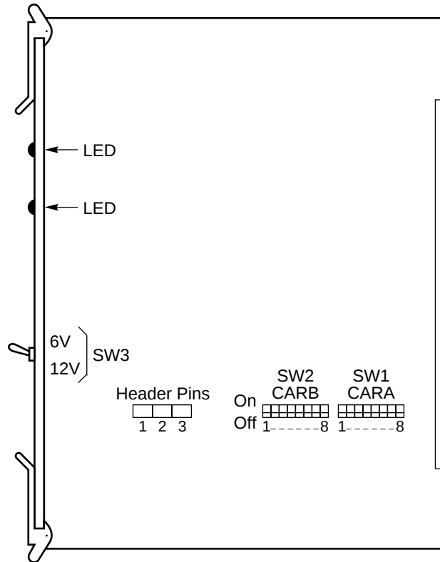
Figure 7 QPC62 1.5 Mbaud Converter Card option switches and header pins
