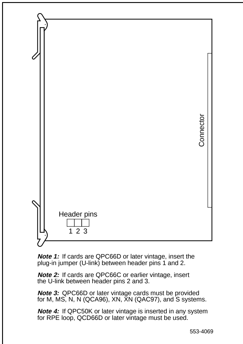
Figure 8 QPC66 2 Mbaud Converter Card header pins
