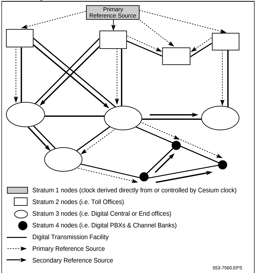
Figure 63 Hierarchical Synchronization
