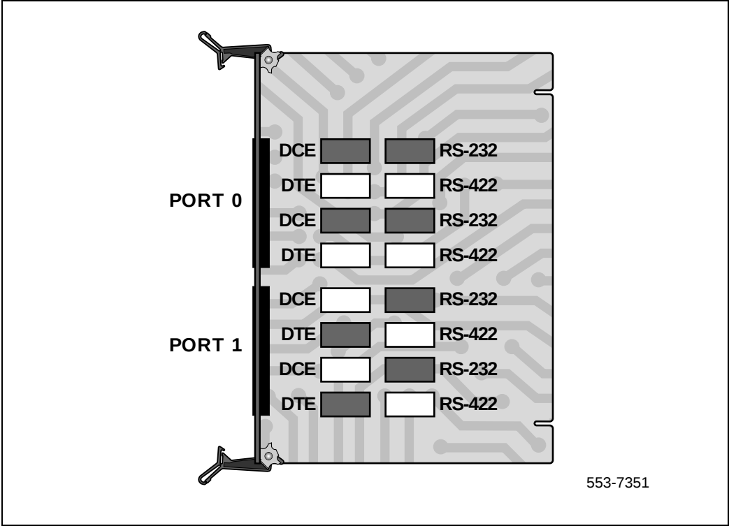
Figure 72 NT6D11AB, NT6D11AD DCHI with ISL low-speed programming jumper settings
