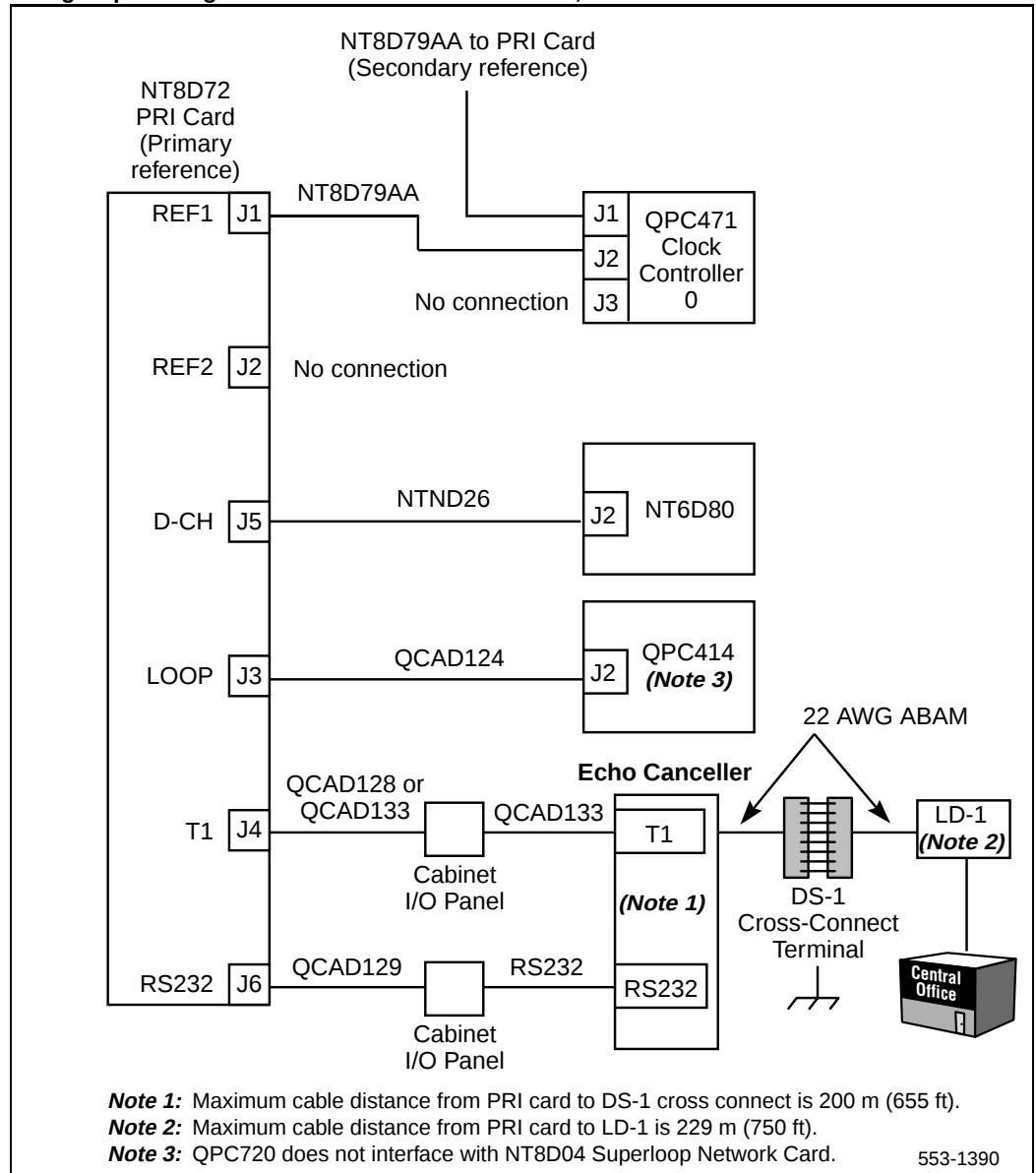
Figure 45 Half group cabling for the NT8D72 on 51C and 61C, with echo canceller
