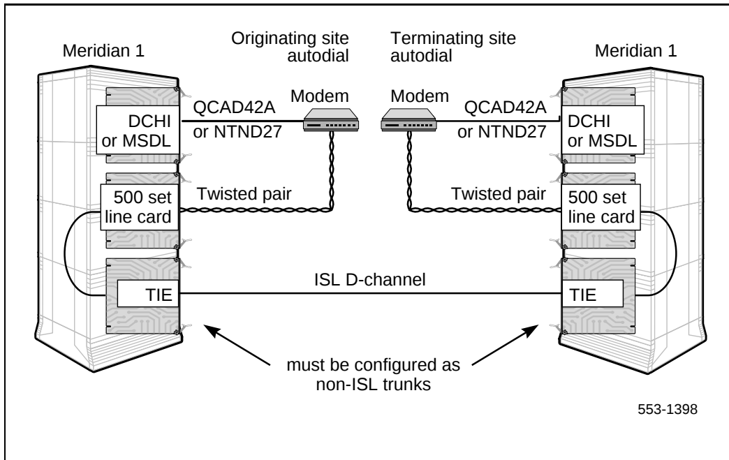
Figure 74 ISL in shared mode
