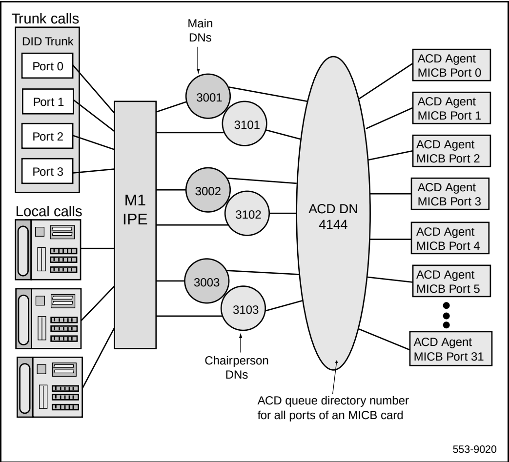
Figure 5 Call routing with chairperson access
