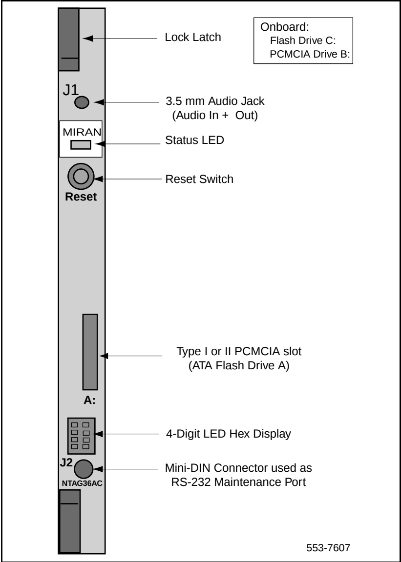
Figure 4 The NTAG36 MIRAN faceplate
