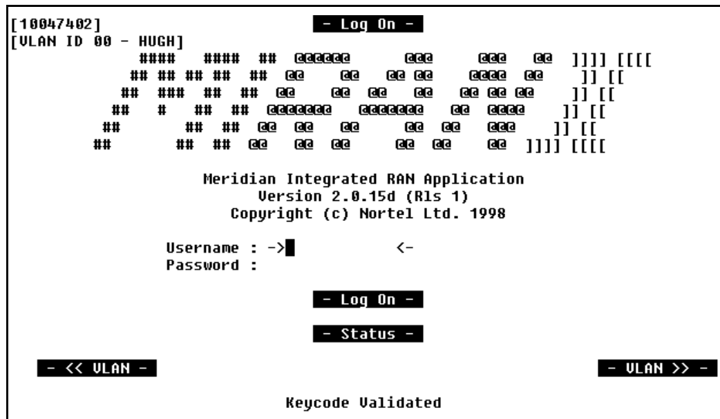
Figure 20 The Login screen
