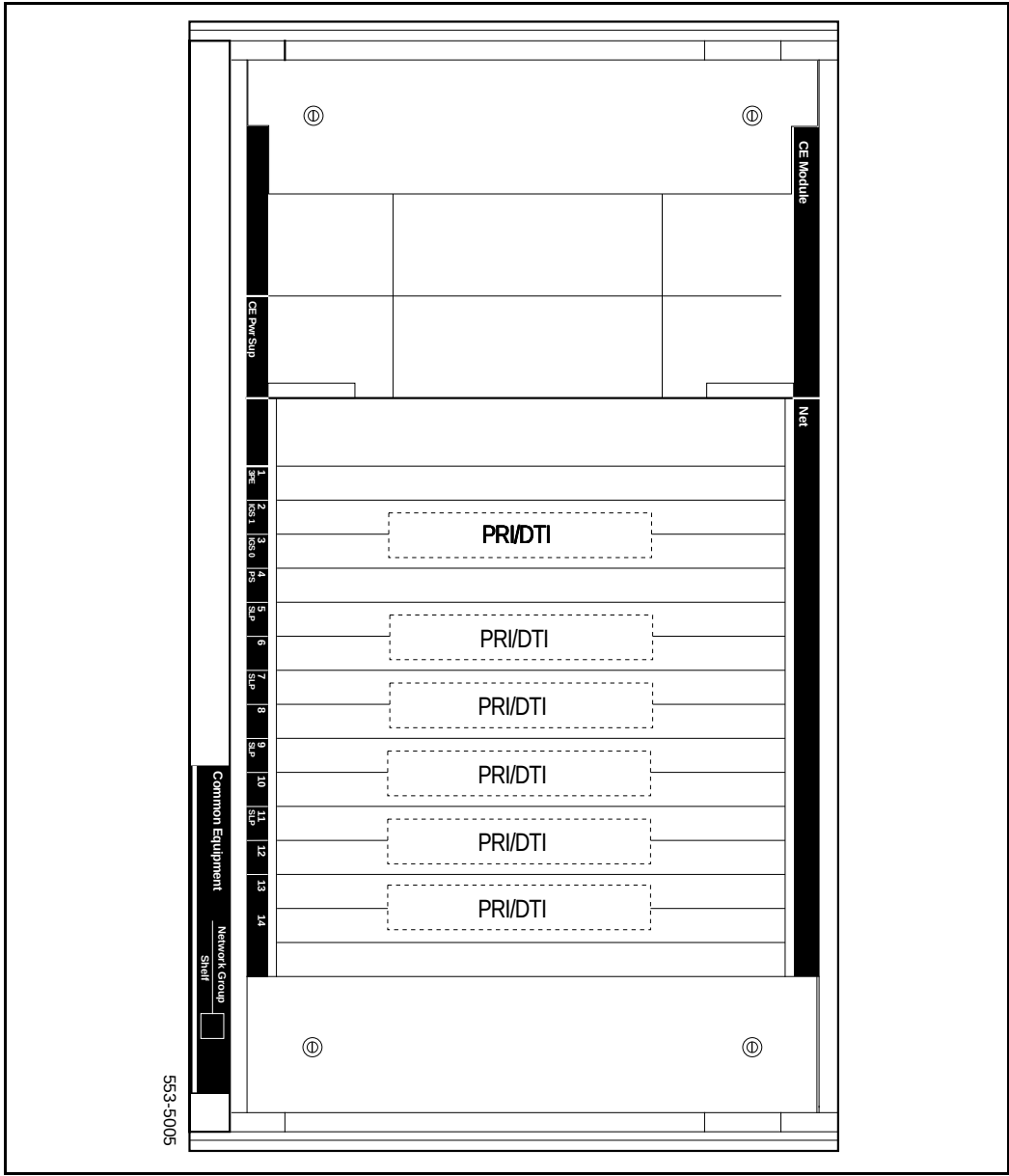
NT8D35 Network Module configured for PRI/DTI expansion
