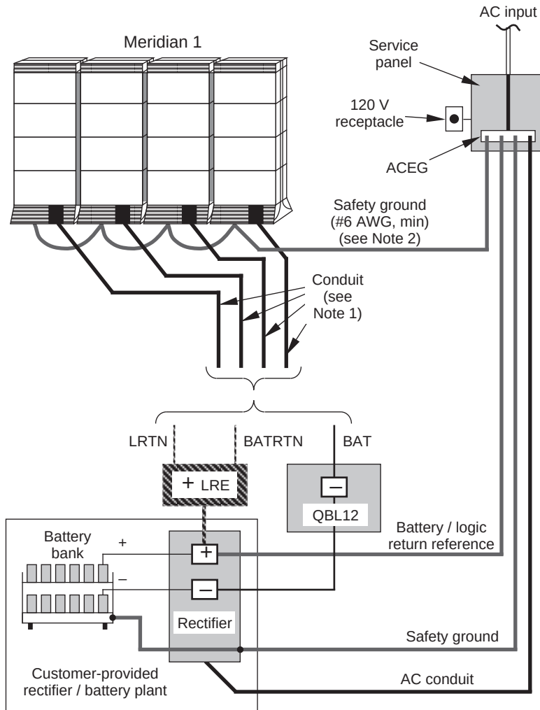
Figure 23 DC power—multiple-column distribution with QBL12 and customer power
