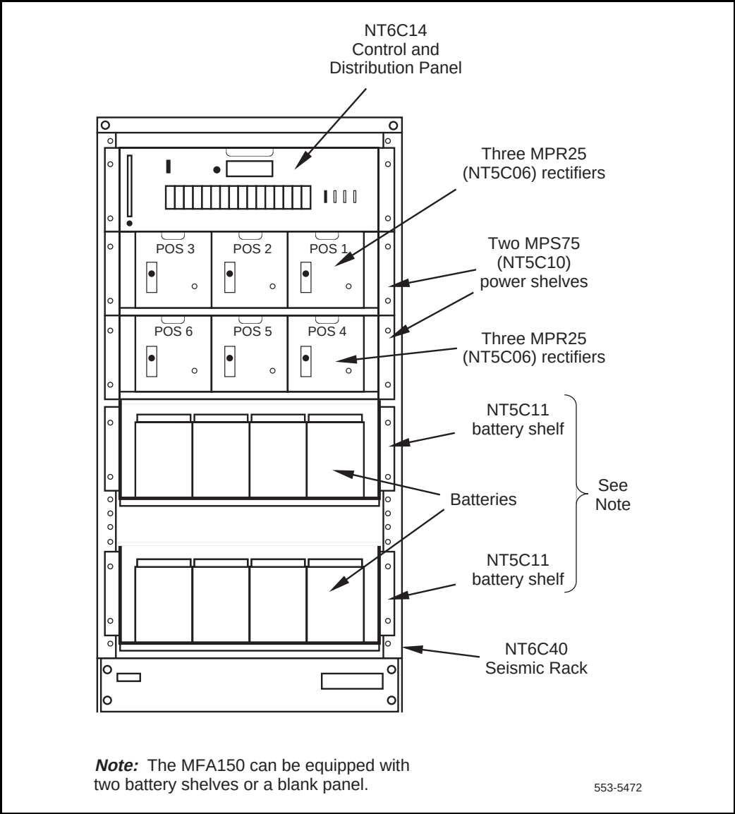
Figure 16 MFA150 Modular Power System with six MPR25 rectifiers
