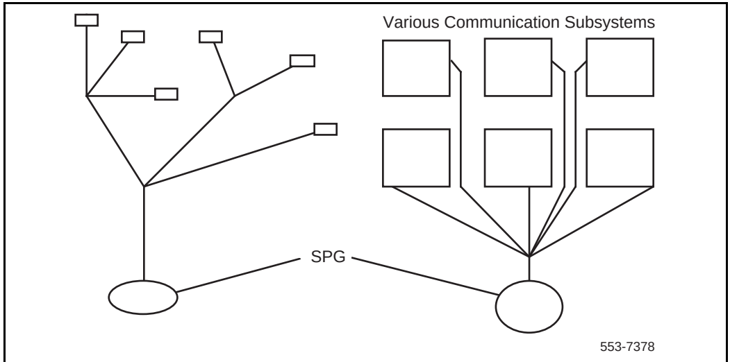
Figure 5 Single point ground
