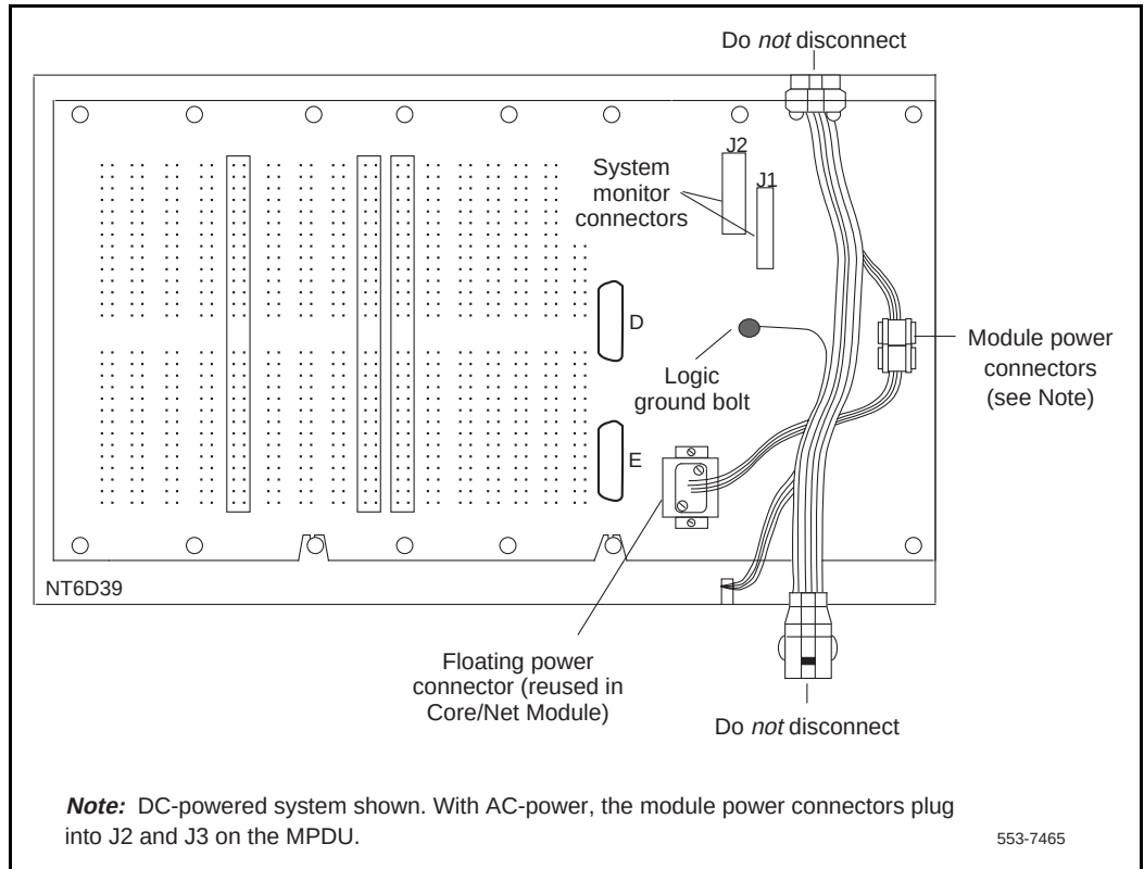
Figure 84 Power connectors on the rear of the NT6D39 CPU/Network module backplanes
