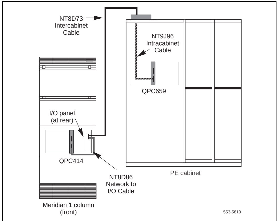
Figure 32 Cabling path for network-to-PE connections
