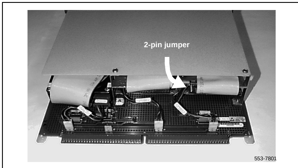
Figure 147 Option 51C 2-pin jumper location on MDU card
