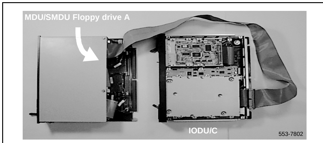
Figure 42 Cabling the MDU to the IODU/C card
