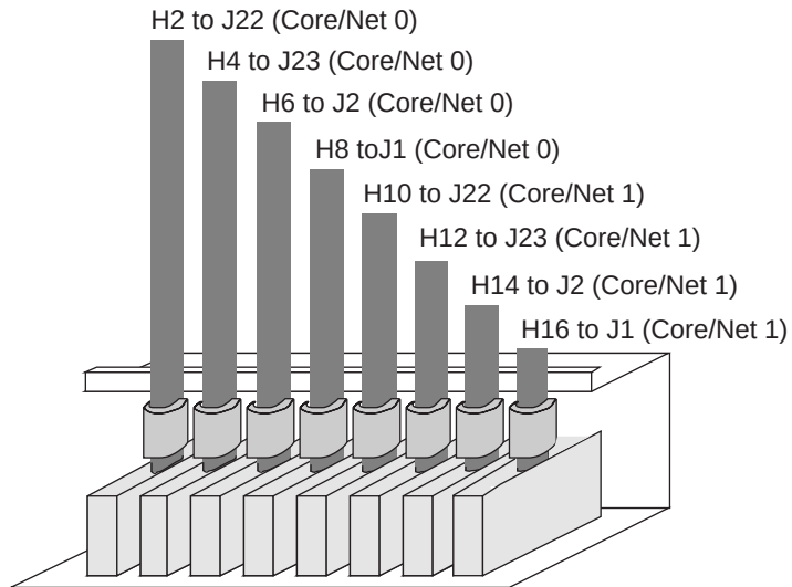
Figure 21 Group 1 and 2 cables connecting to the connector bracket
