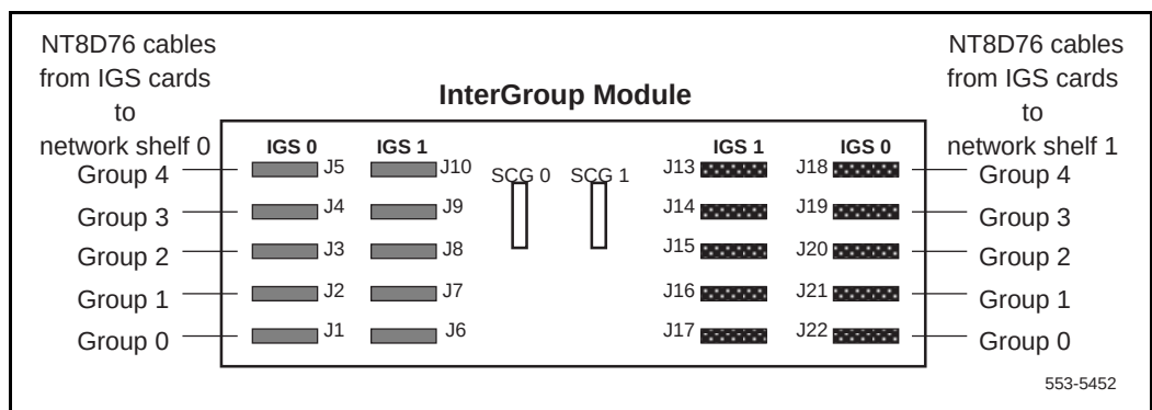
Figure 105 QPC412 IGS card cable assignments to the InterGroup module
