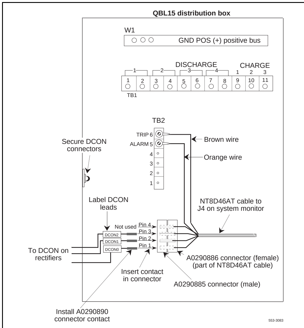
NT8D46AT cable field wiring connections
