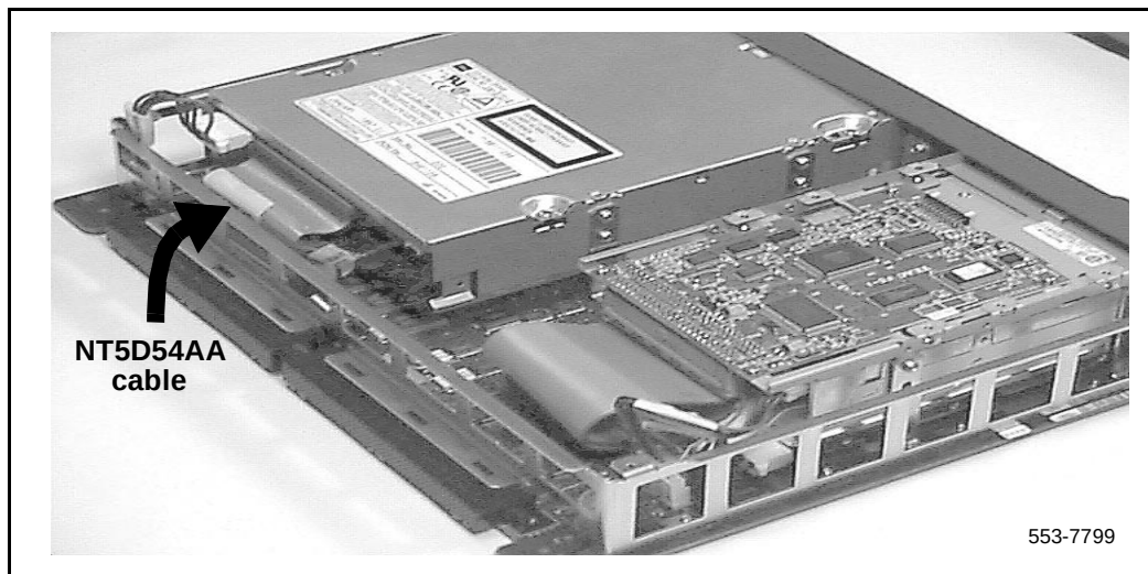
Figure 41 Location of NT5D54 cable on IODU/C card
