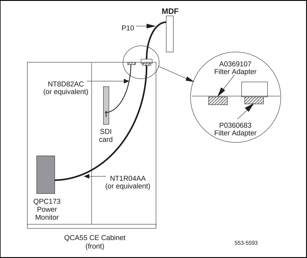
Figure 24 Power monitor and SDI connections in the QCA55 cabinet
