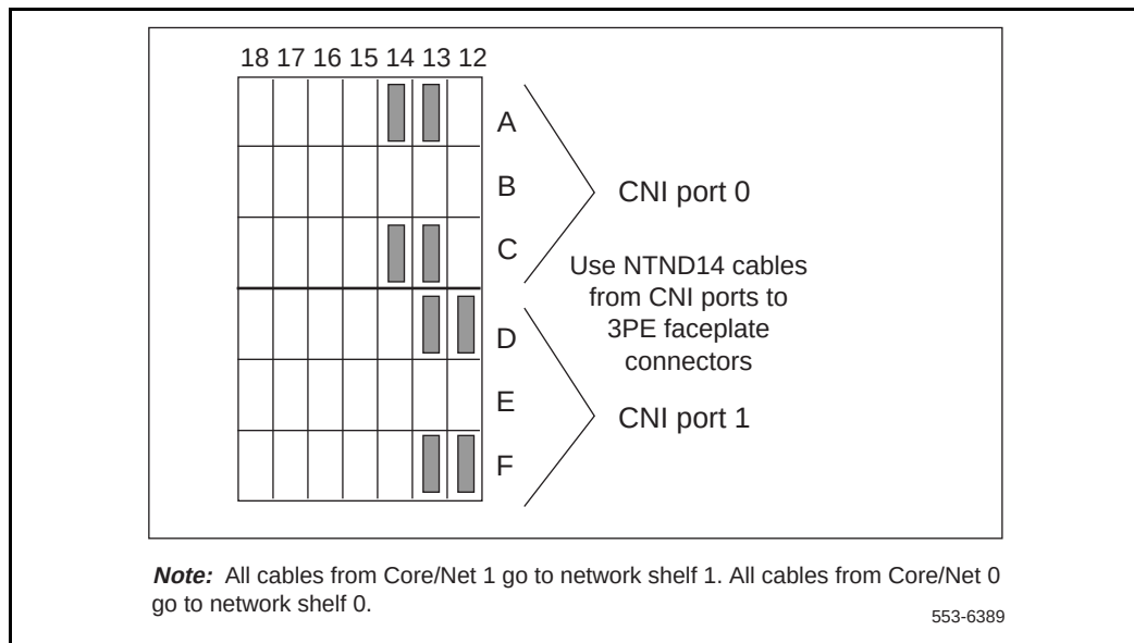
Figure 91 NT5D21 Core/Net module (rear)—backplane connections for CNI slots
