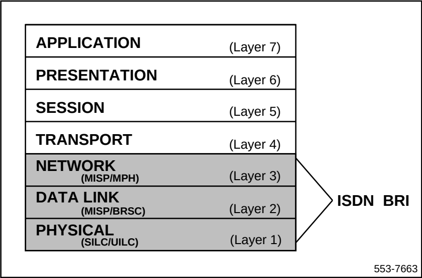
Figure 1 OSI model
