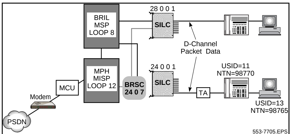
Figure 2 DSL terminal configuration with D-channel and B-channel packet data
