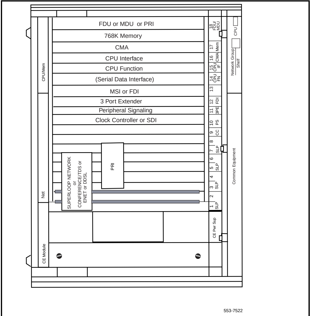
Figure 12 Meridian 1 system Options 51/61
