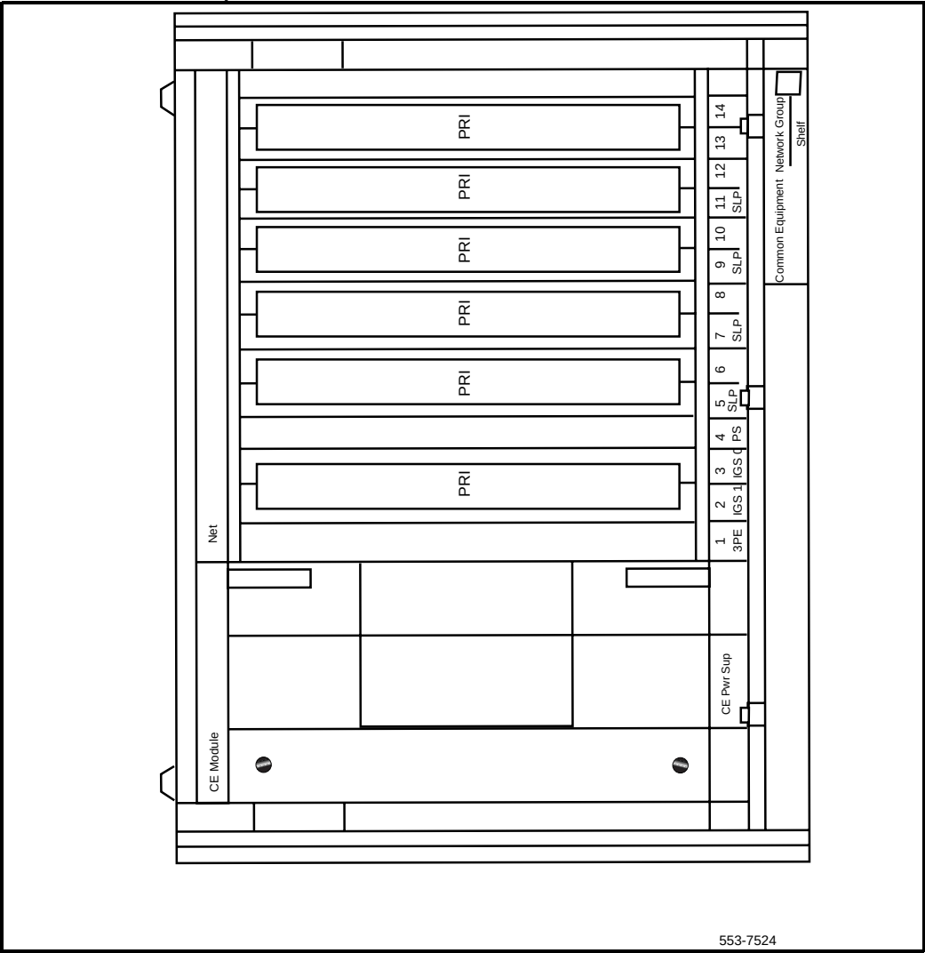
Figure 16 Meridian 1 network expansion module with six PRI cards
