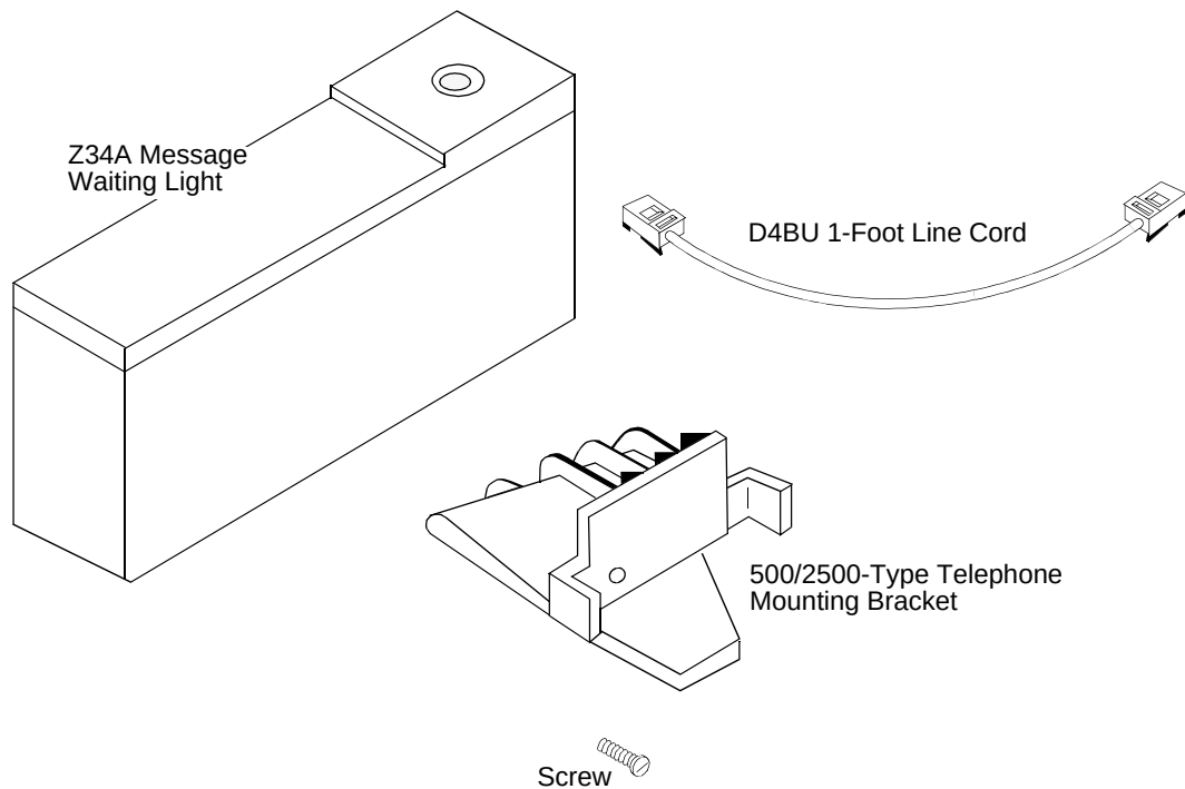
Figure 19-9. The Z34A Message Waiting Indicator
