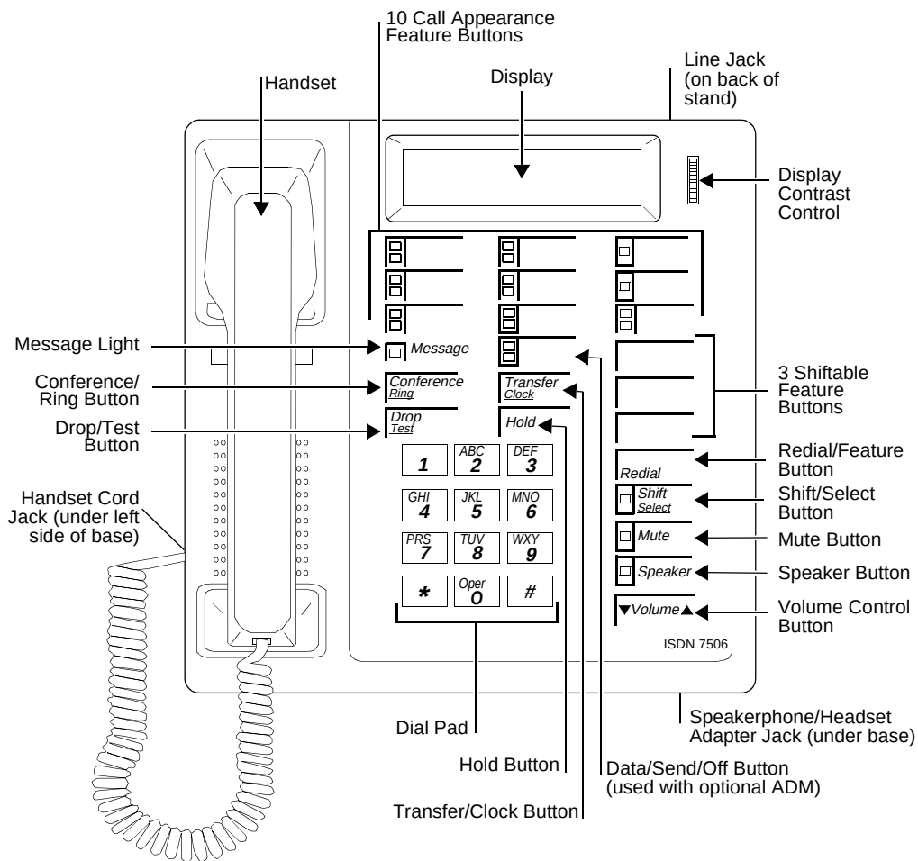
Figure 16-2. The 7506 Asynchronous Data Modular Display Terminal
