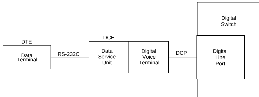
Figure 20-15. A Block Diagram of 703A Data Service Unit Interfaces
