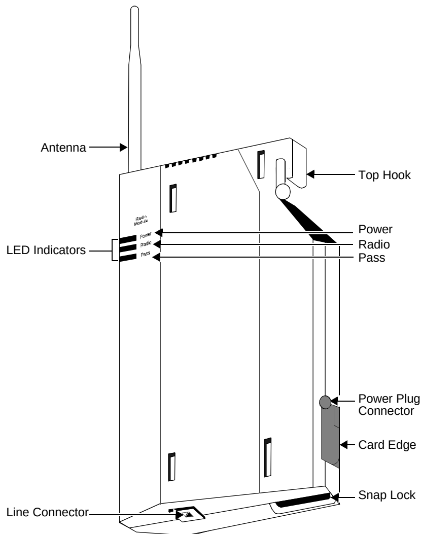
Figure 17-7. The MDW 9000 Telephone, Radio Module
