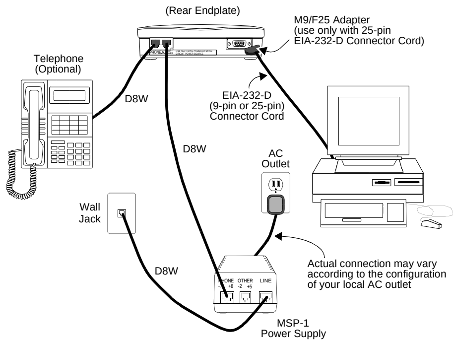
Figure 20-7. Typical Installation of the International Configuration, Including Telephone and Separate Power Supply
