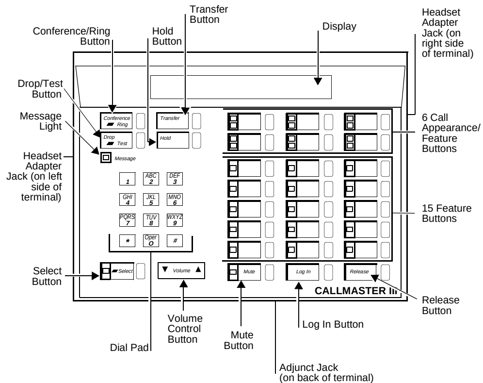
Figure 13-2. The CALLMASTER II and CALLMASTER III Voice Terminal
