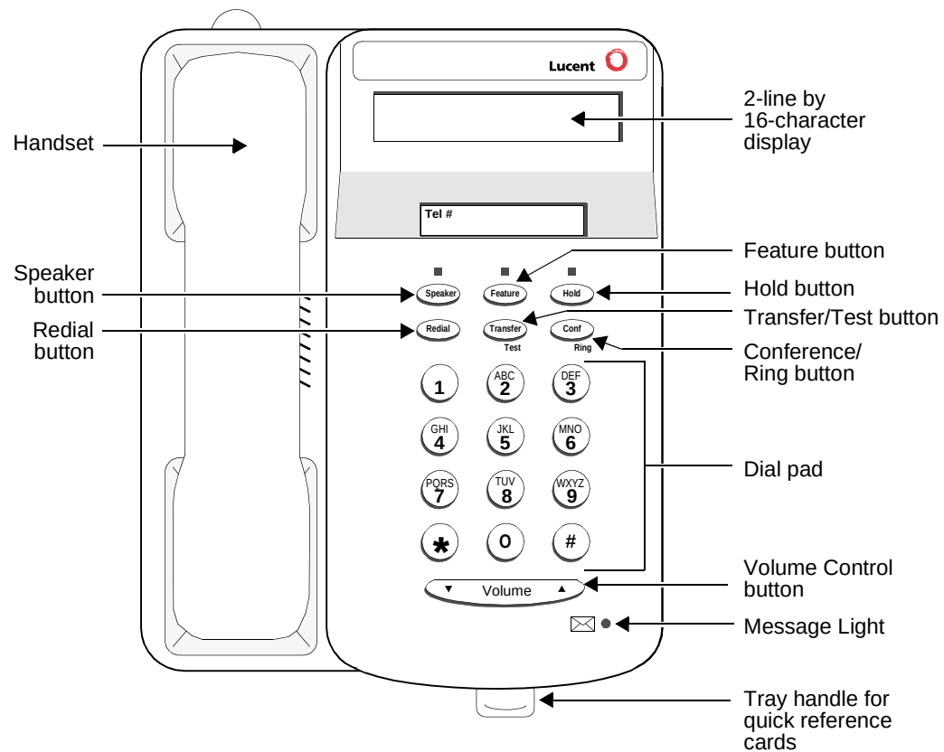
Figure 7-2. The 6402D Telephone
