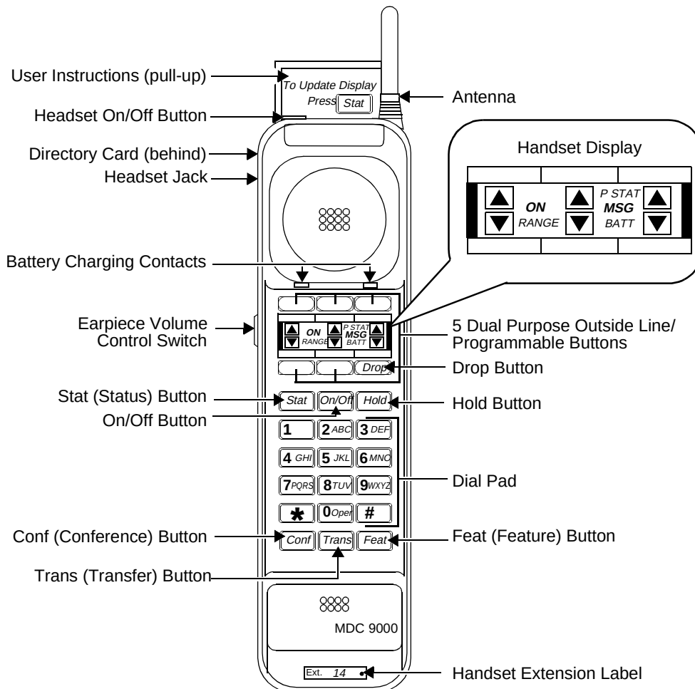
Figure 17-1. The MDC 9000 Telephone, Top View of Handset, Including Enlarged Display Area
