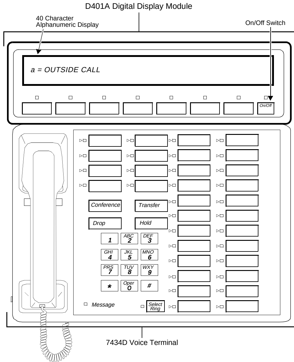
Figure 19-2. The D401A Digital Display Module Mounted on a 7434D Voice Terminal
