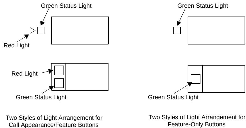
Figure 2-2. Button Lights
