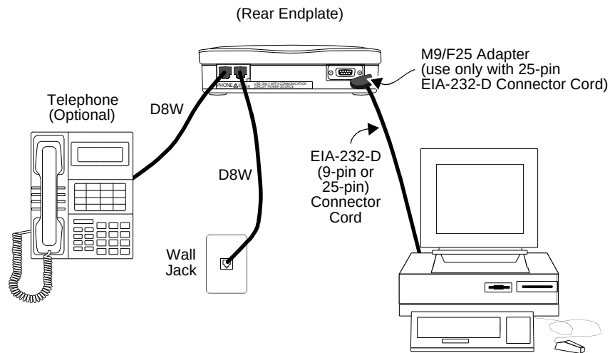
Figure 20-8. Typical Installation of the US and International Configuration, Including Telephone and Closet Power Supply
