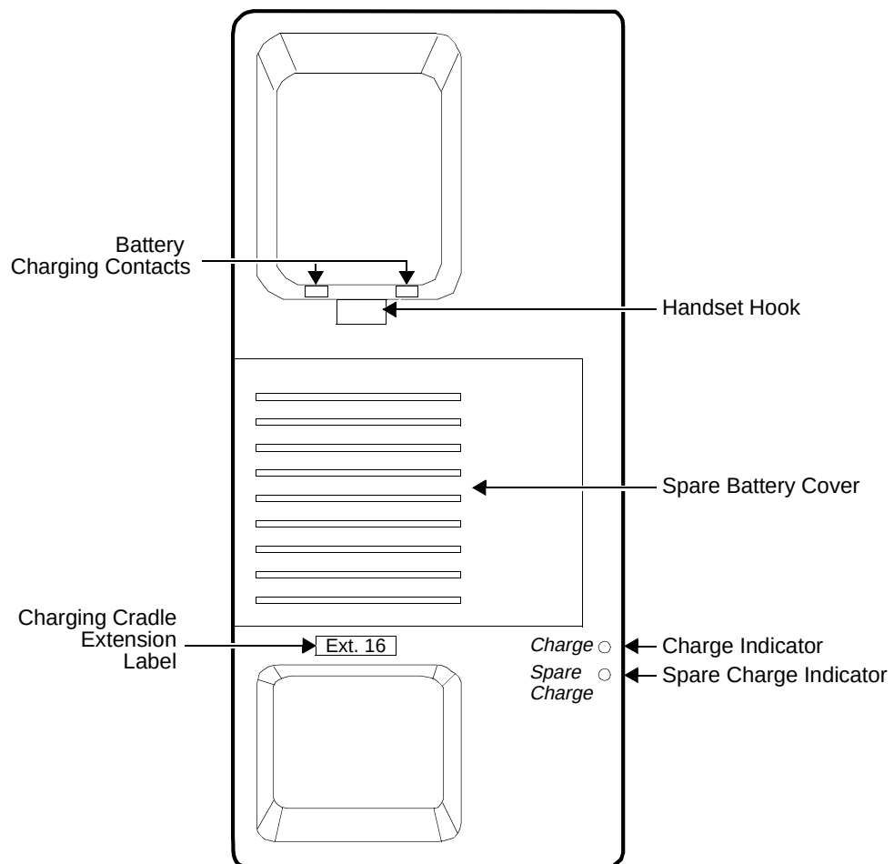
Figure 17-6. The MDW 9000 Telephone, Top View of Charging Cradle
