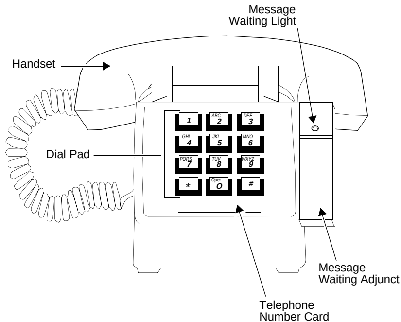
Figure 14-4. The 2500 Telephone with Message Waiting Adjunct
