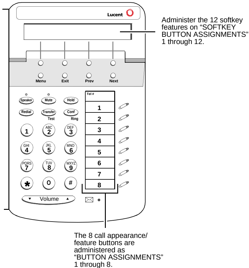
Figure 7-6. Button Numbering for Administering the 6408 Telephones Connected to a DEFINITY System Release 6.1 or Later
