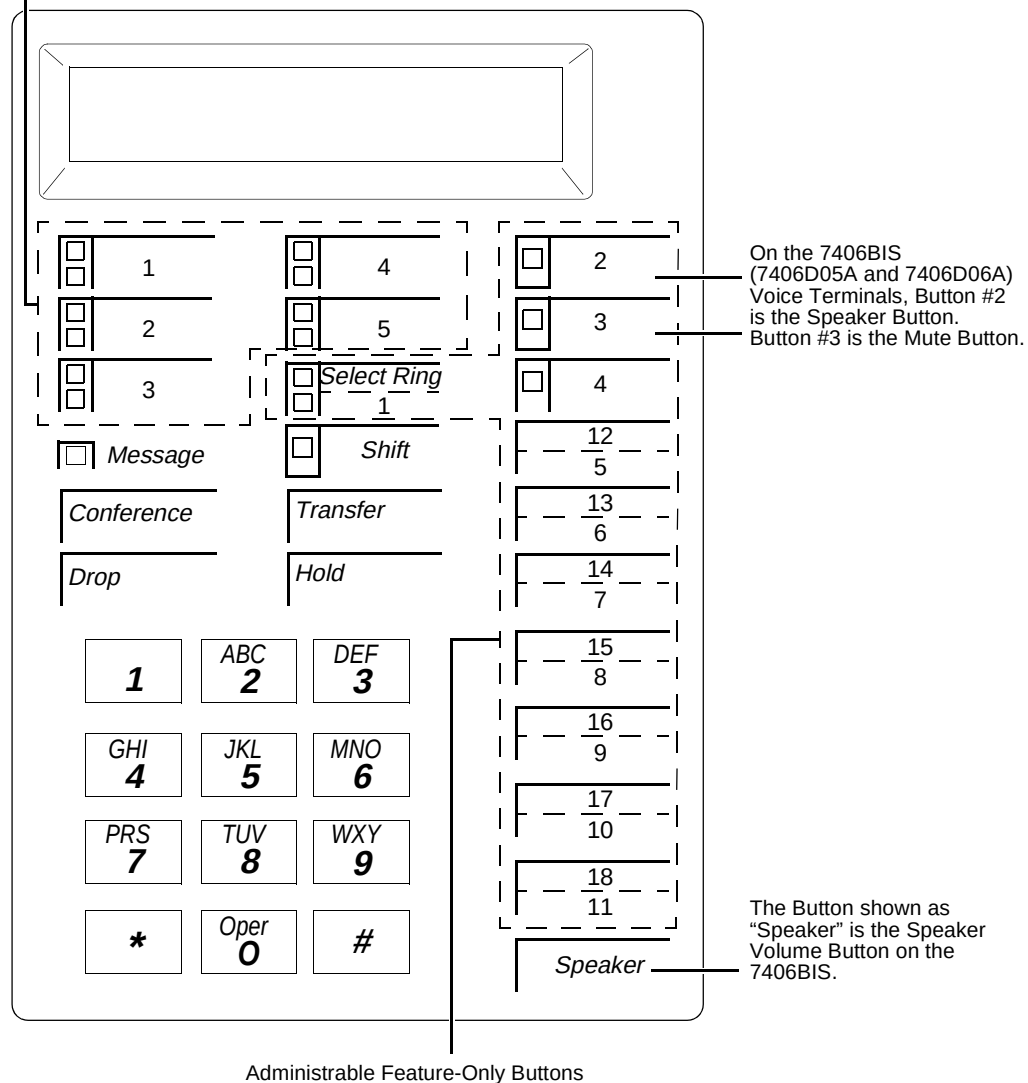
Figure 11-13. Button Numbering for Administering the 7406D and 7406BIS Voice Terminals Connected to a System 75, a DEFINITY G1 or G3, or a DEFINITY ECS
