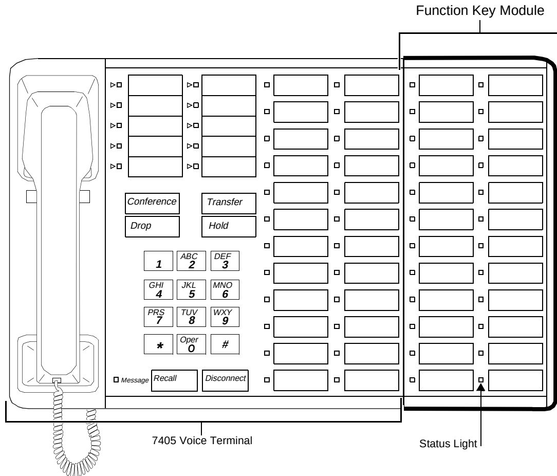
Figure 19-3. The F201 or F401A Function Key Module Mounted on a 7405D Voice Terminal
