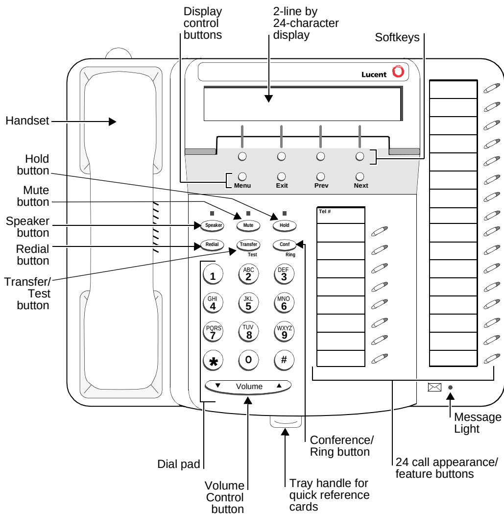
Figure 7-9. The 6424D Plus Telephone
