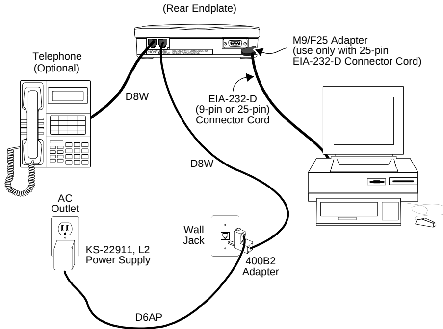
Figure 20-6. Typical Installation of the US Configuration, Including Telephone and Separate Power Supply
