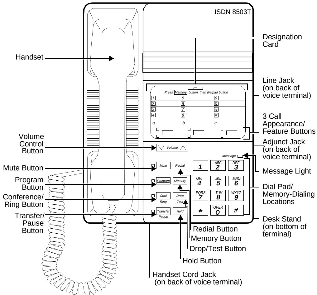
Figure 16-4. The Desk-mounted ISDN 8503T Voice Terminal
