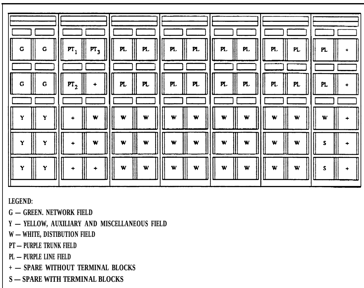
Figure 2-8. Separated Trunk and Line Ports
