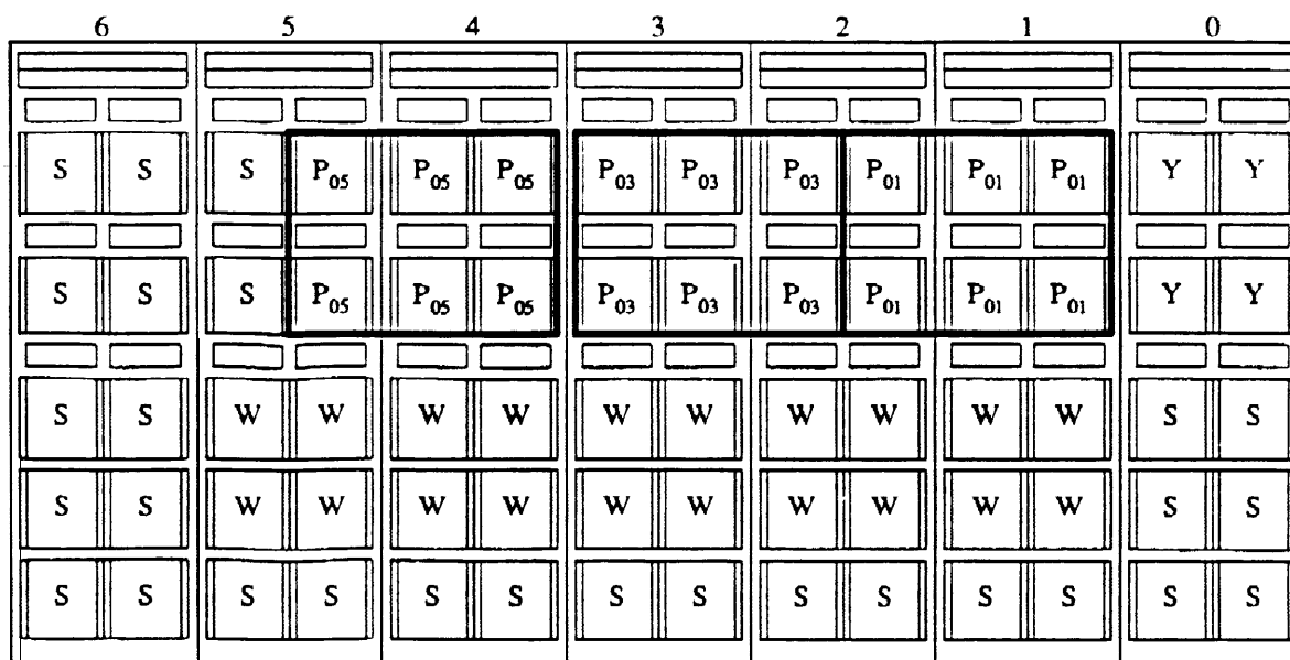
Figure 10-4. 7-Module System Mounted on Self-Supporting Type-1 Frame, Rear
