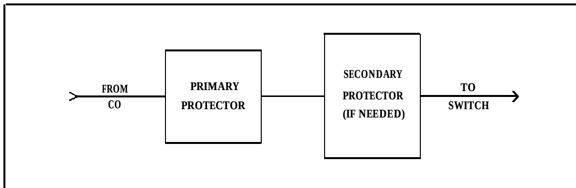
Figure 3-1. Placement of Electrical Protectors on CO Side of Switch
