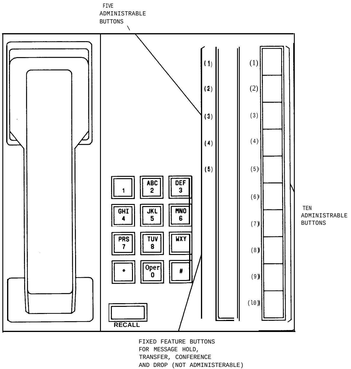
Figure 2-8. 20-Button MET Voice Terminal Administrable Button Number Assignments
