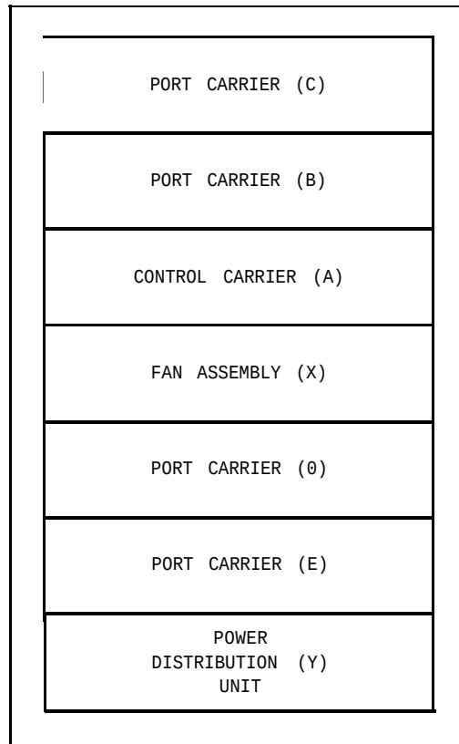
Figure 2-11. Model 3 Carrier Locations and Designations (Front View)
