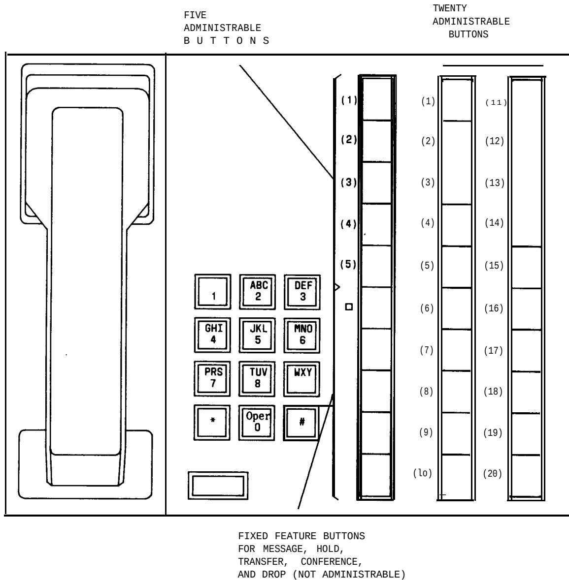
Figure 2-9. 30-Button MET Voice Terminal Administrable Button Number Assignments
