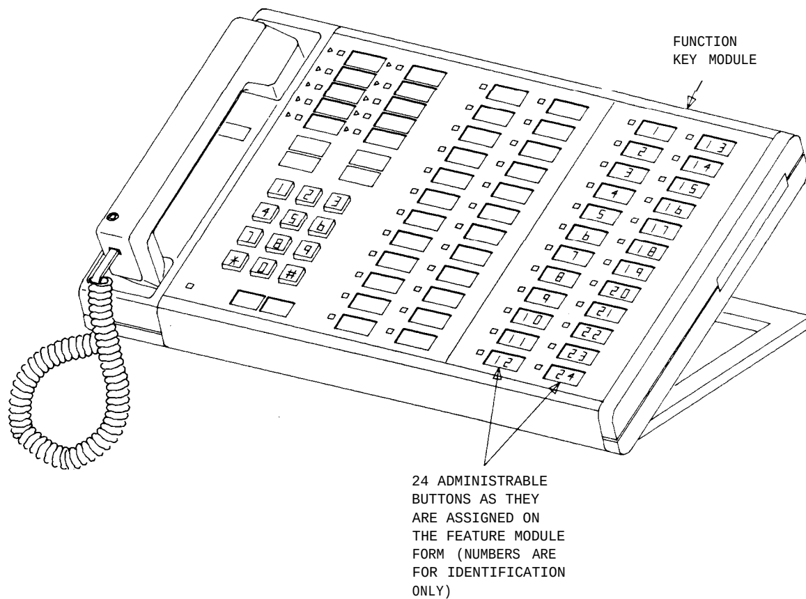
Figure 4-6. Model 7405D Voice Terminal With Optional Feature Module and Administrable Button Assignment
