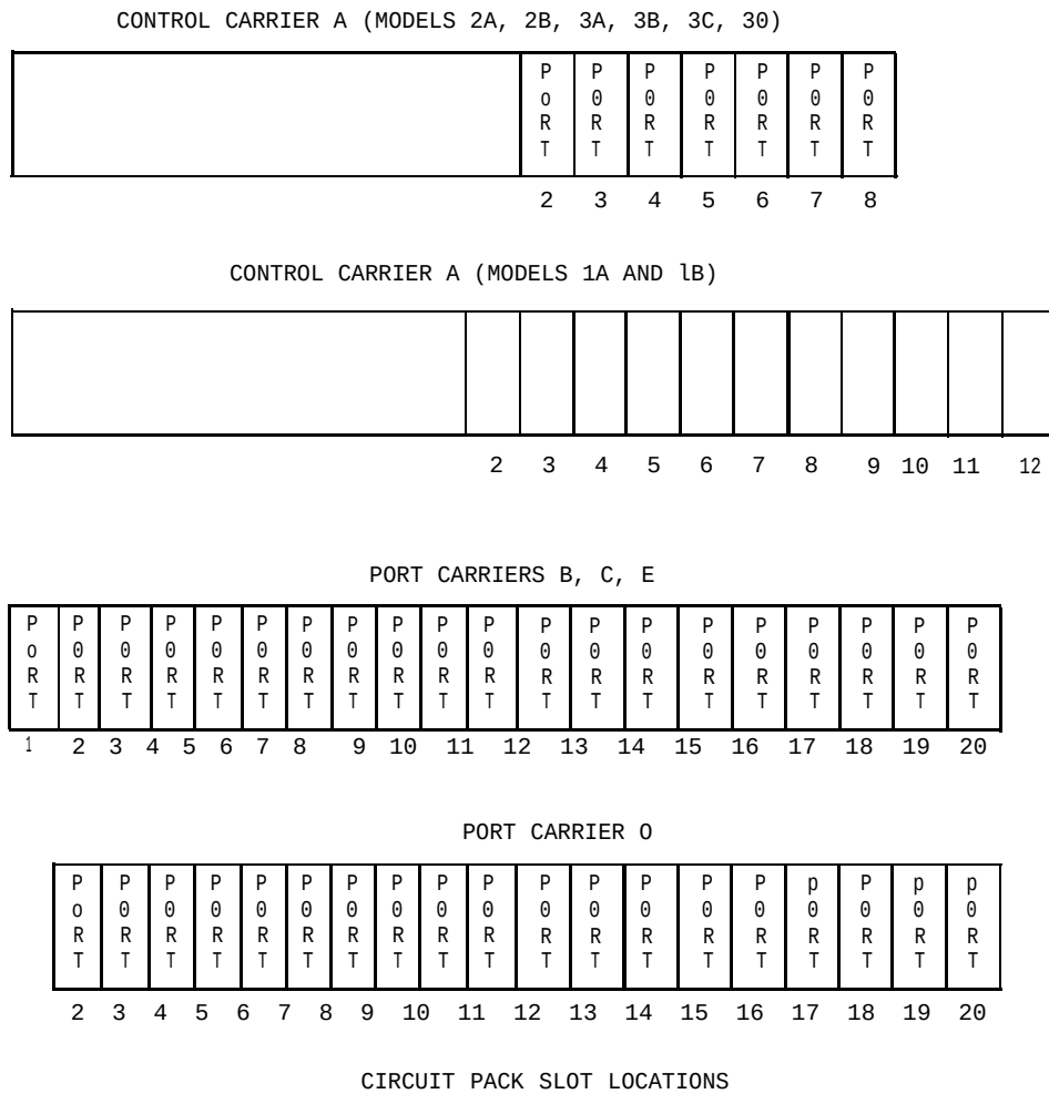
Figure 2-10. Control and Port Carrier Circuit Pack Slot Locations for Model 3 and Models 1 and 2 (Front View)
