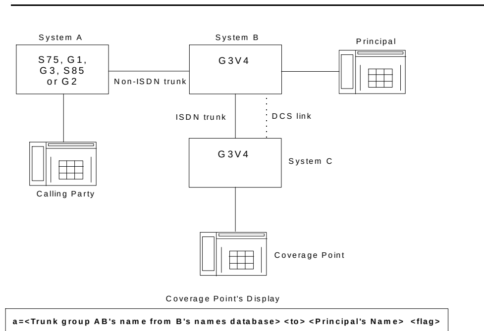
Figure 3-10. Display — Non-DCS, Non-ISDN Trunk to DCS Trunk over ISDN Trunk
