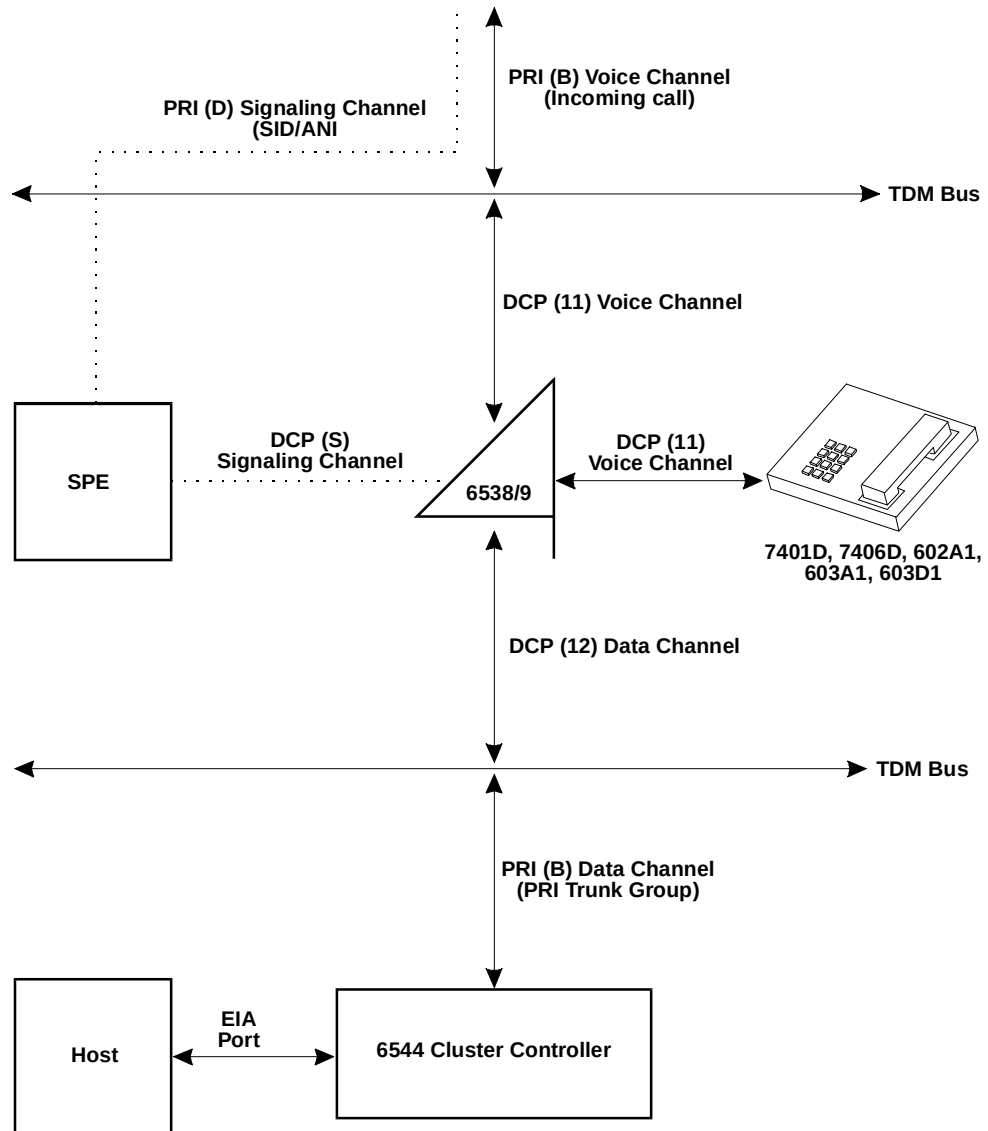
Figure 3-3. Constellation Hardware/Signaling Arrangement
