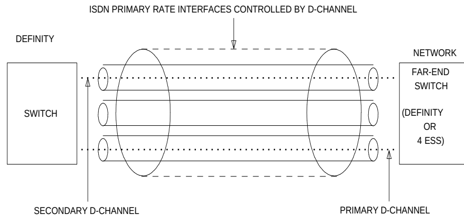
Figure 3-16. Example D-Channel Backup With Three ISDN-PRIs
