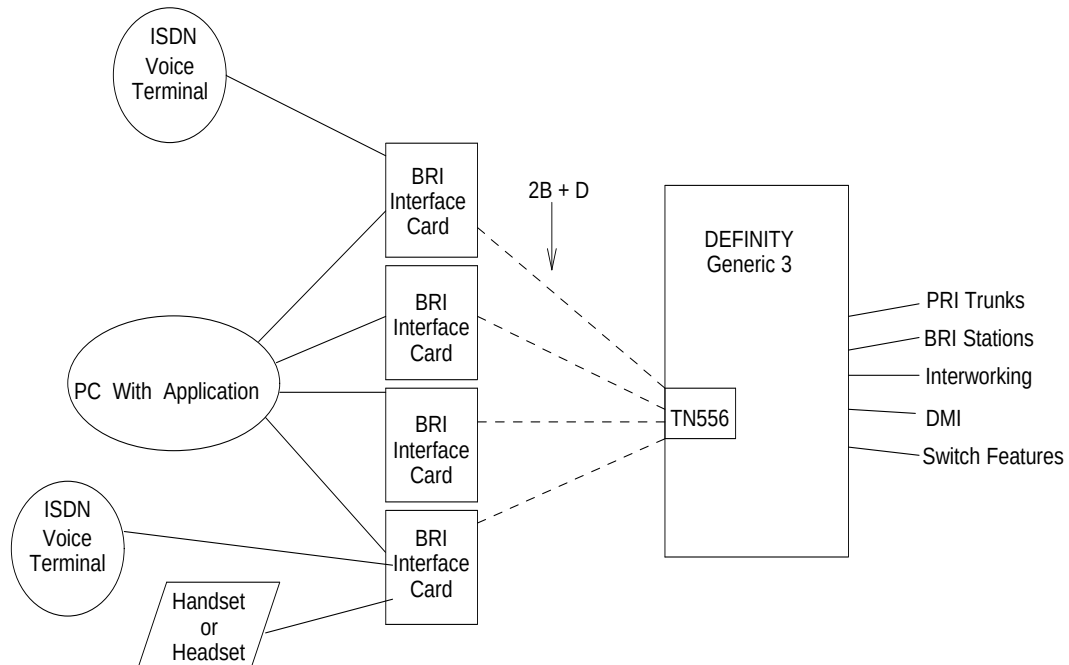
Figure 3-28. ISDN—BRI PC Interface Configuration (Group 3)
