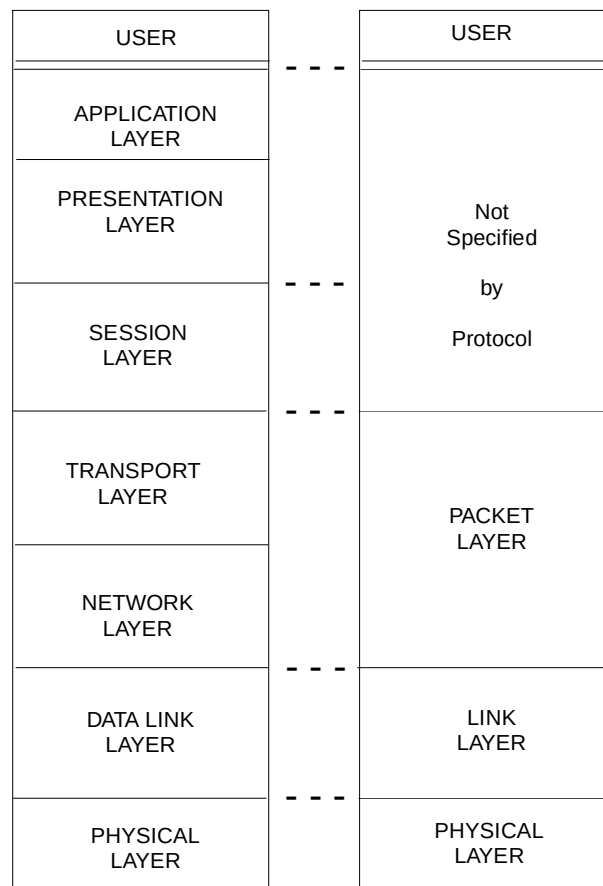
X.25 Protocol Layers
