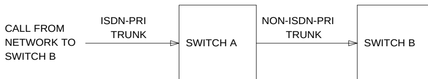
Figure 3-23. Interworking Example
