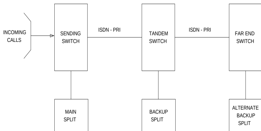
Figure 3-25. Look Ahead Interflow Using a Tandem Switch
