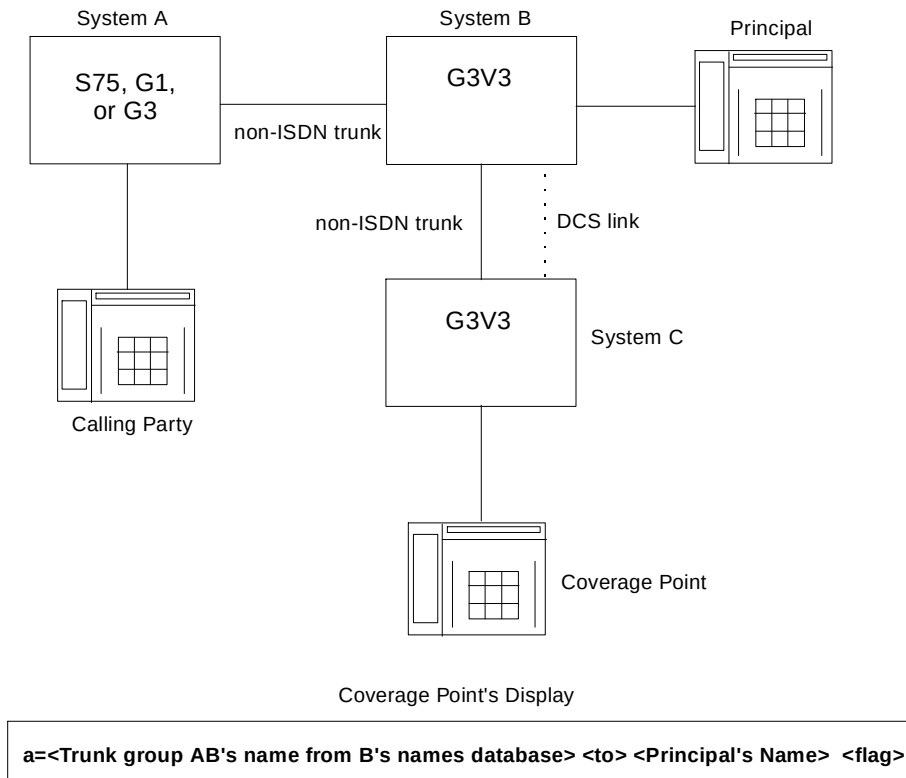
Figure 3-9. Display — Non-DCS, Non-ISDN Trunk to DCS Trunk over Non-ISDN Trunk
