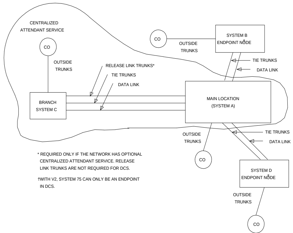
Figure 2-6. Typical Distributed Communications System
