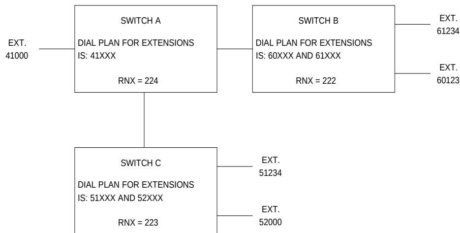
Figure 3-30. UDP Example
