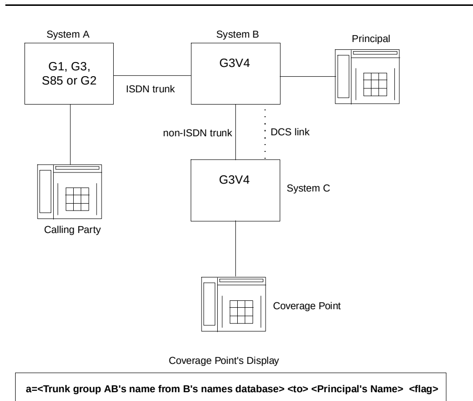
Figure 3-12. Non-DCS ISDN Trunk to Non-ISDN DCS Trunk
