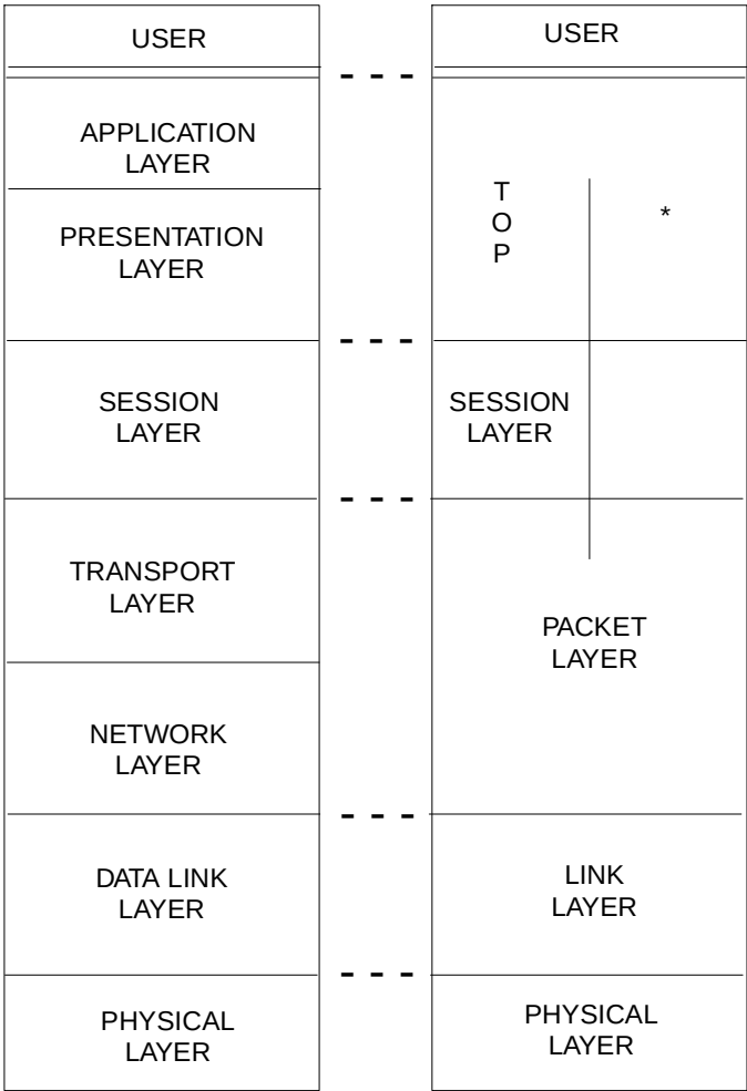
BX.25 Protocol Layers
