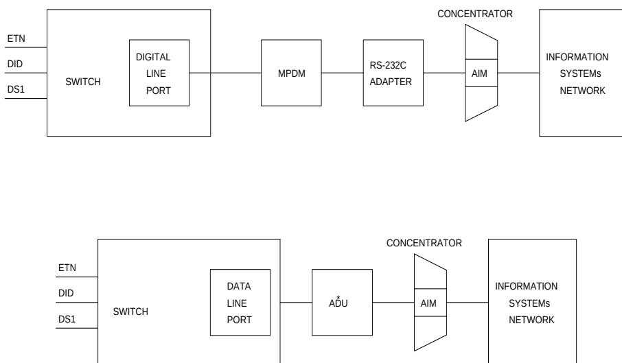
Figure 3-19. System-to-ISN Connectivity
