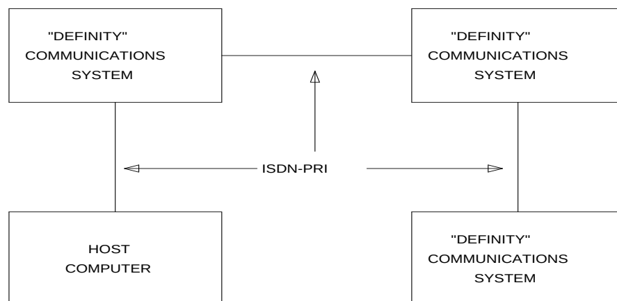
Figure 3-20. ISDN-PRI Private Network Configuration
