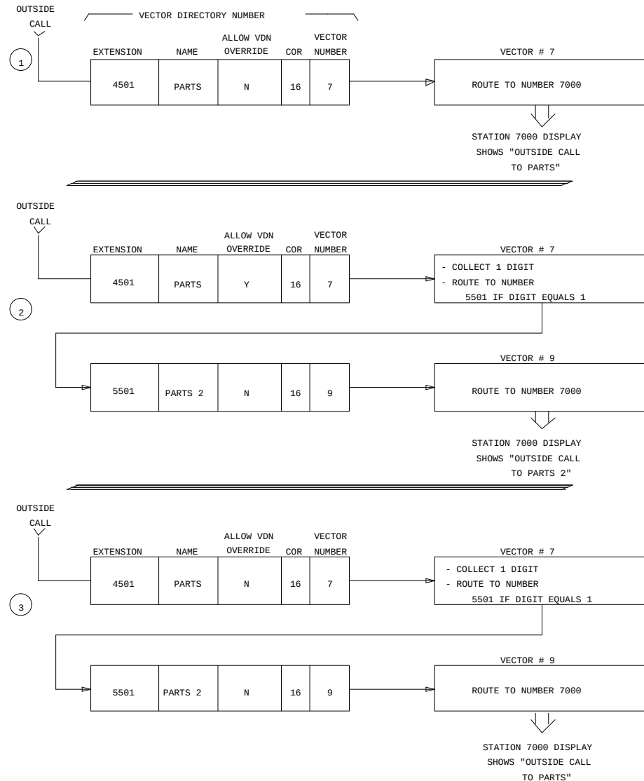
Figure 3-1. Typical VDN Call Processing Examples
