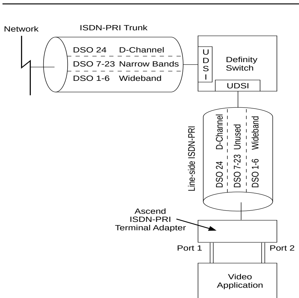
Figure 3-39. Wideband Switching Video Application
