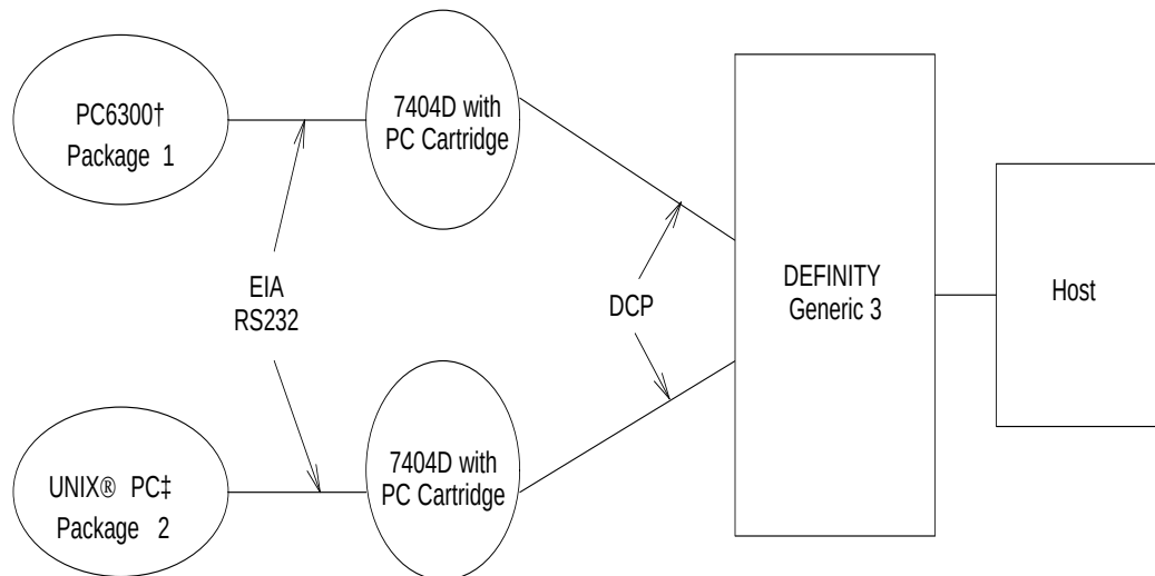
Figure 3-26. DCP PC Interface Configuration (Group 1)
