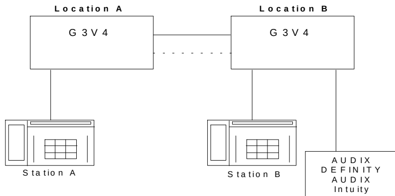
Figure 3-4. Applications for DCS Call Coverage
