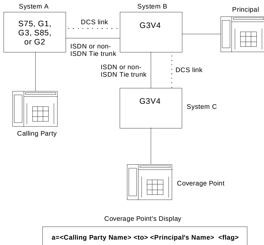
Figure 3-8. Display — DCS Trunks End-to-End
