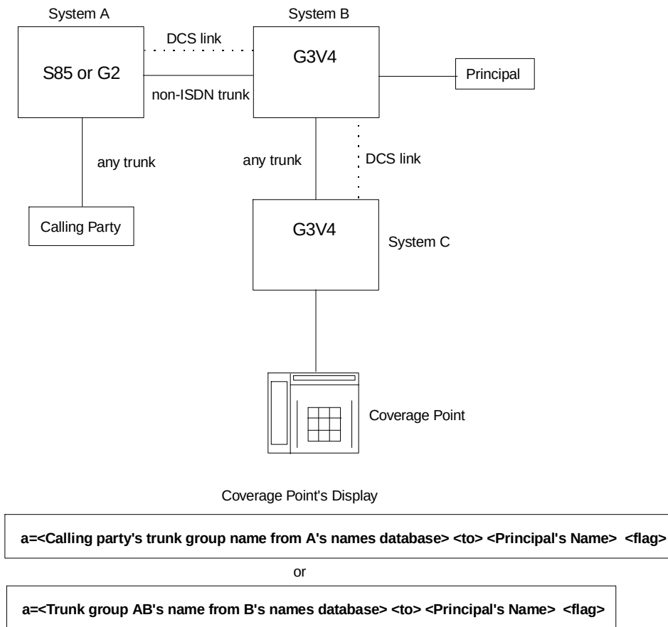
Figure 3-13. Display — Call Initiated by a Trunk on System 85 or G2
