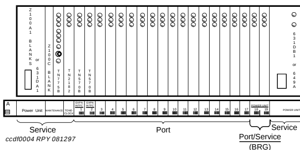
Figure 35. Expansion Control Carrier (J58890AF) (Front)
