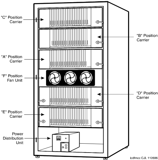
Figure 10. Typical Multicarrier Cabinet
