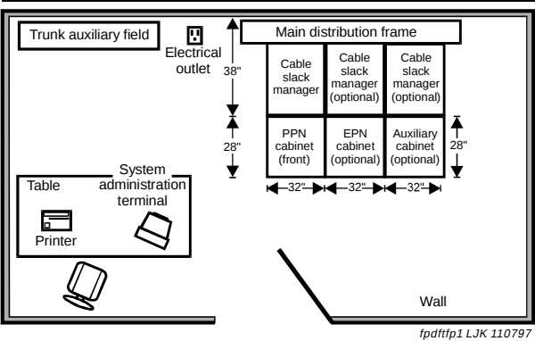
Figure 15. Typical Floor Plan with EPN and Auxiliary Cabinet
