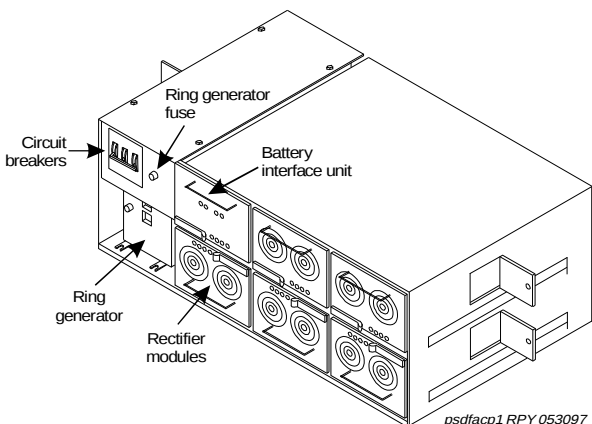
Figure 25. AC Power Distribution Unit (J58890CH-1) (Front)
