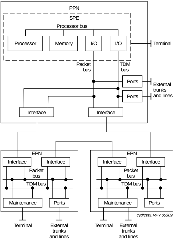
Figure 3. Components of a Directly-Connected System
