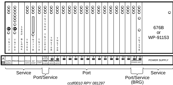
Figure 39. Basic Control Cabinet (J58890L) (Front)
