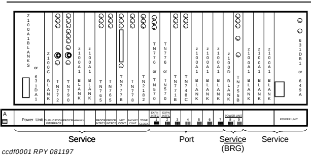
Figure 31. Control Carrier (J58890AH) (Front)
