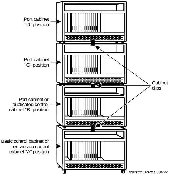
Figure 38. Typical SCC Stack
