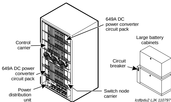
Figure 30. DC Power Distribution in Multicarrier Cabinets
