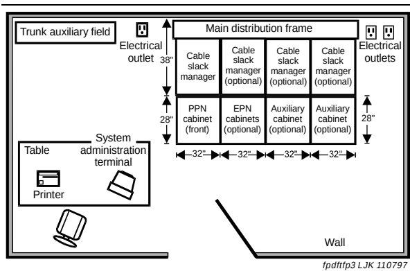
Figure 16. Typical Floor Plan with an additional EPN and Auxiliary Cabinets
