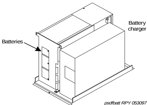
Figure 23. Battery Charger (Optional Part of J58890CE-2) (Front)
