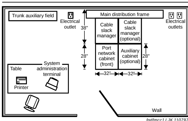
Figure 14. Typical Multicarrier Cabinet Floorplan
