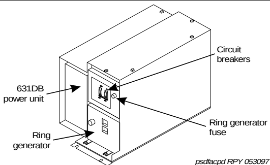
Figure 22. AC Power Distribution Unit (J58890CE-2) (Front)
