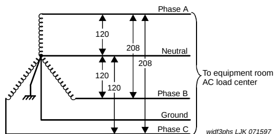
Figure 19. Three Phase, 4-Wire, 120/208 VAC, 60 -Source
