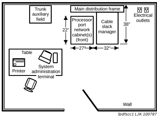
Figure 13. Typical Single-Carrier Cabinet Floor Plan
