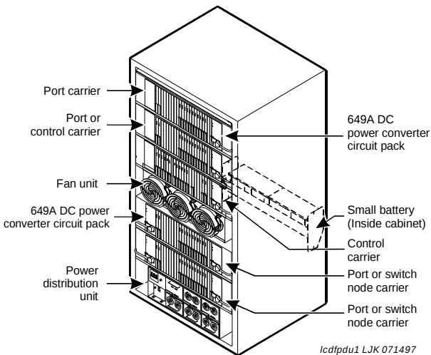
Figure 29. Power Distribution in Multicarrier Cabinets
