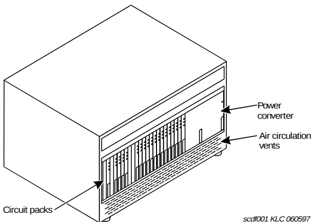
Figure 9. Typical Single-Carrier Cabinet
