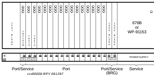
Figure 42. Port Cabinet (J58890H) (Front)
