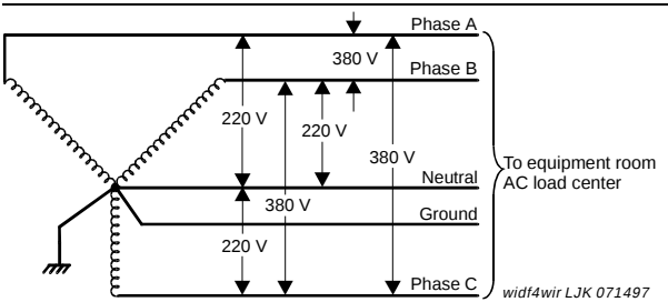
Figure 20. International 4-Wire, 220/380 VAC, 50-Hz Source
