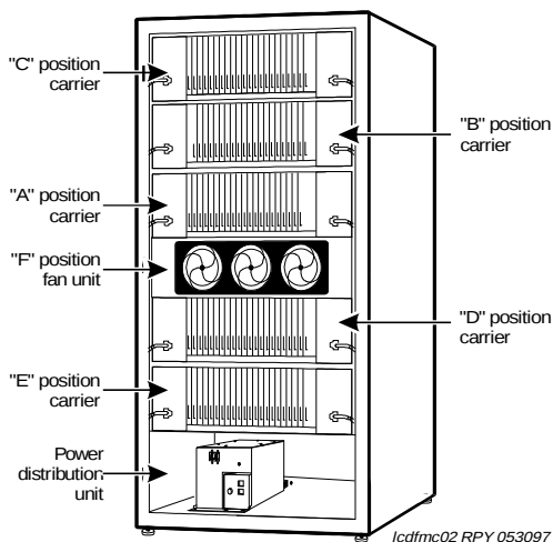
Figure 28. Typical DC-Powered MCC Layout
