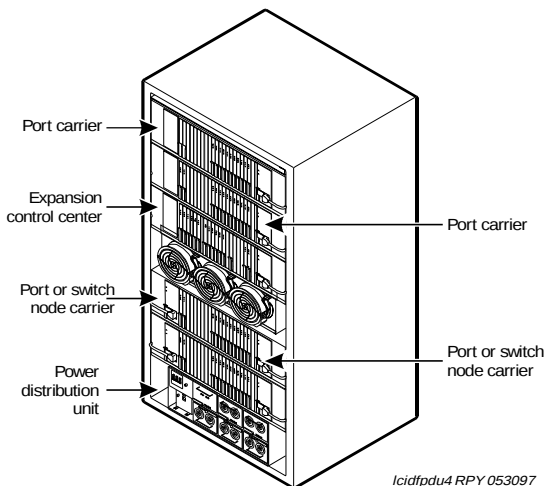
Figure 30. Typical Multicarrier EPN Cabinet (J58890A)
