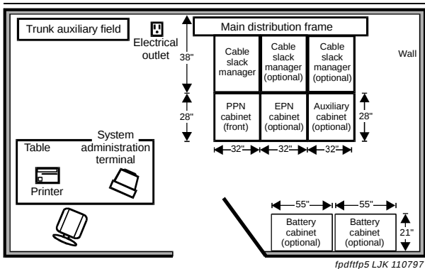
Figure 17. Typical Floor Plan with Battery Cabinets
