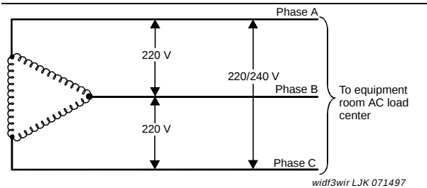
Figure 21. International Delta, 3-Wire, 220 or 240 VAC, 50-Hz Source
