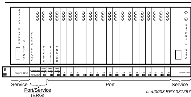
Figure 34. Port Carrier (J58890BB) (Front)
