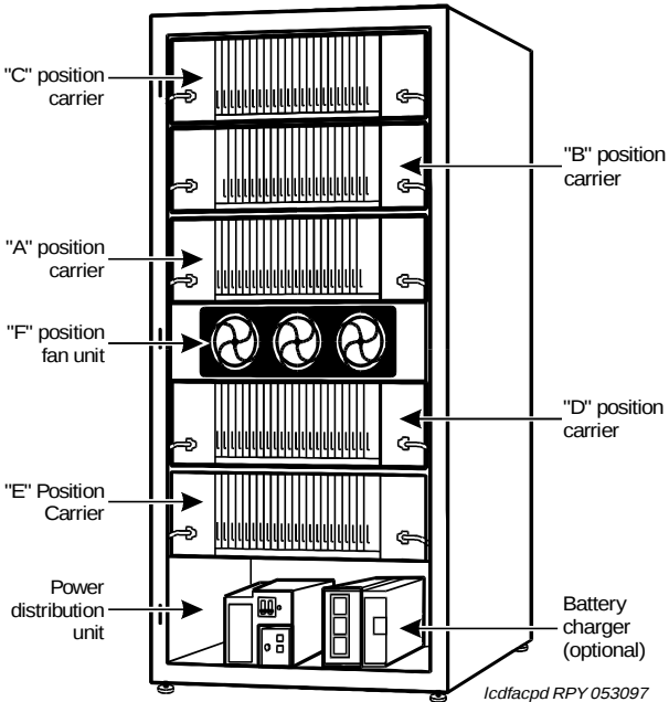
Figure 24. AC Power Distribution in Multicarrier Cabinets
