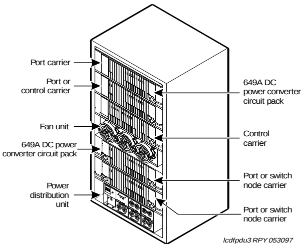
Figure 29. Typical Multicarrier PPN Cabinet (J58890A)
