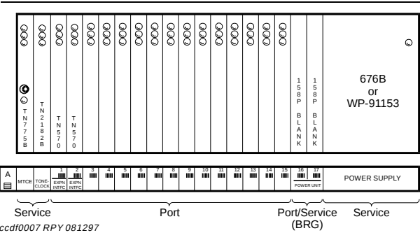
Figure 41. Expansion Control Cabinet (J58890N) (Front)
