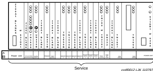
Figure 33. Processor Carrier (J58890AP) (Front)
