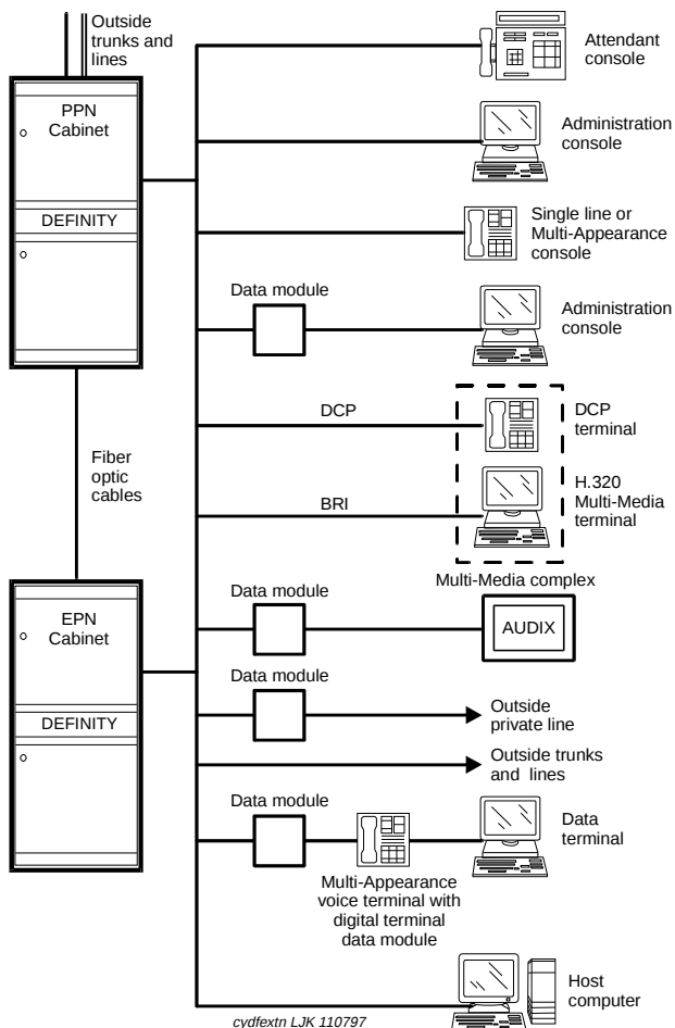
Figure 11. Typical Connections to the External Environment
