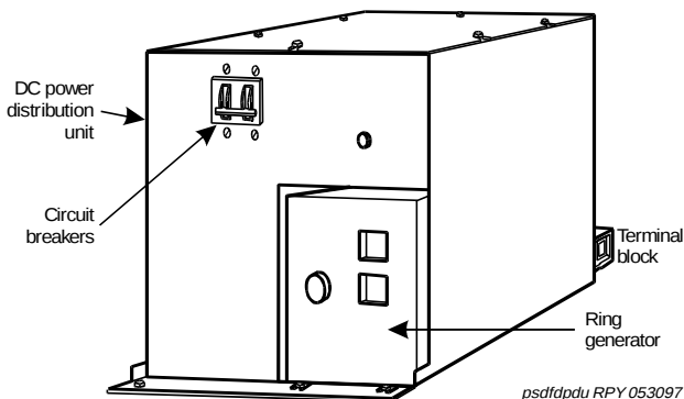
Figure 28. DC Power Distribution Unit (J58890CF-2) (Front)
