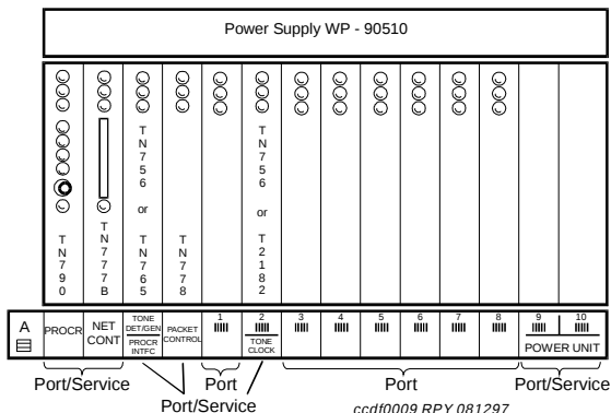
Figure 43. CSCC (J58890S L8) (Front)
