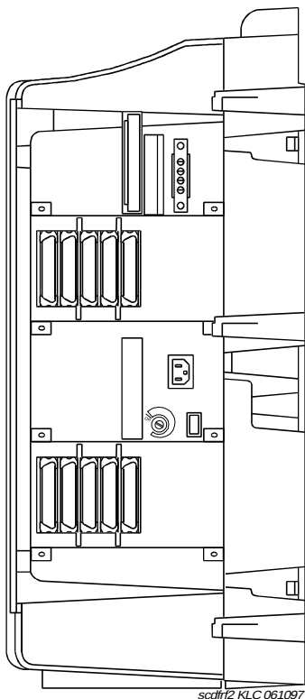
Figure 46. CMC (J58890T) (Right Side)
