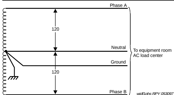
Figure 18. Single-Phase, 120/240 VAC, 60 Hz Source
