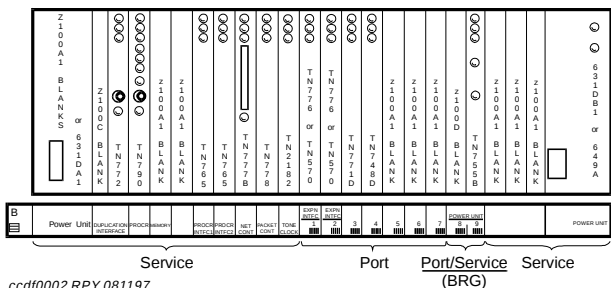
Figure 32. Duplicated Control Carrier (J58890AJ) (Front)
