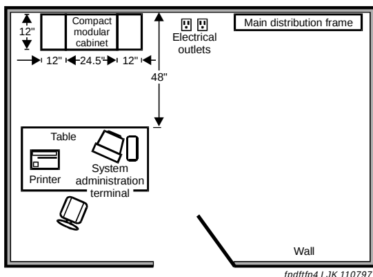
Figure 12. Typical Compact Modular Cabinet Floor Plan
