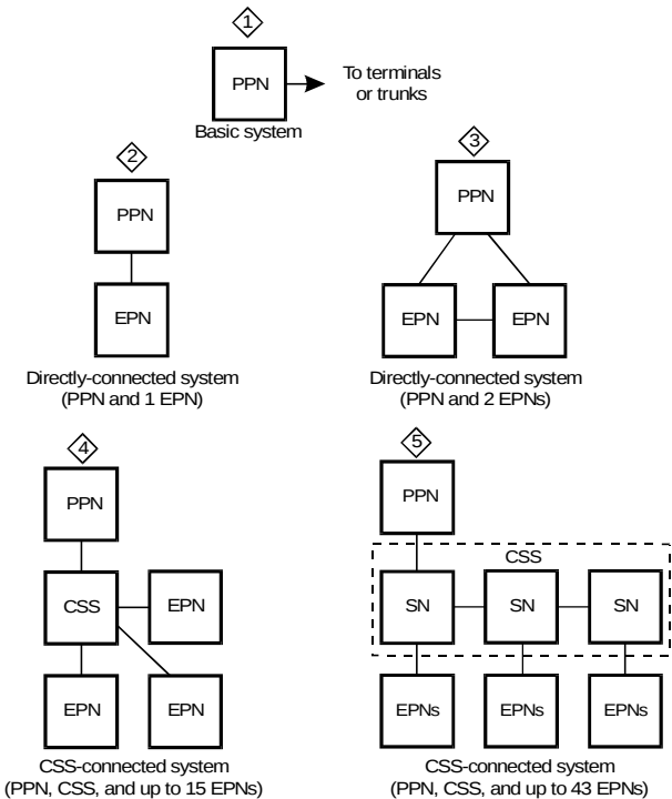
Figure 2. Main System Configurations
