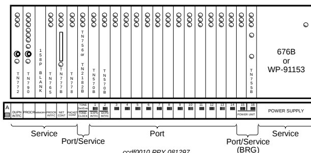
Figure 40. Duplicated Control Cabinet (J58890M) (Front)
