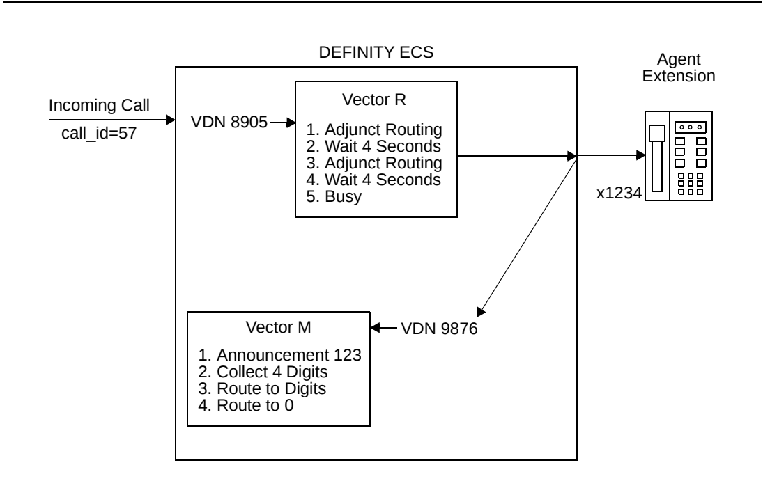
Figure A-13. Call Flow for a Direct Agent Call where RONA Timer Expires
