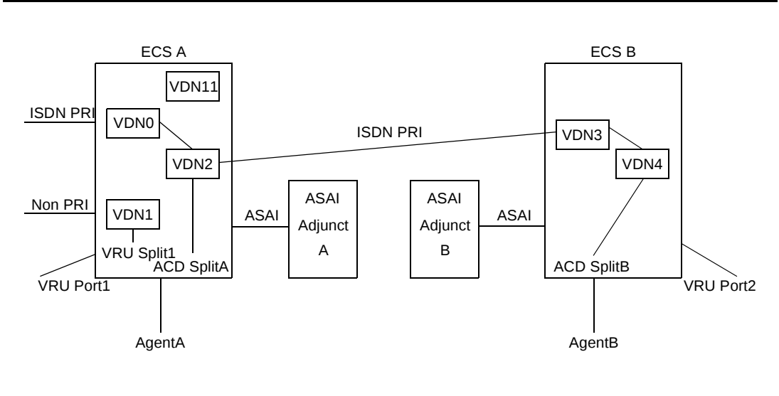
Figure A-18. Distributed ACD Configuration
