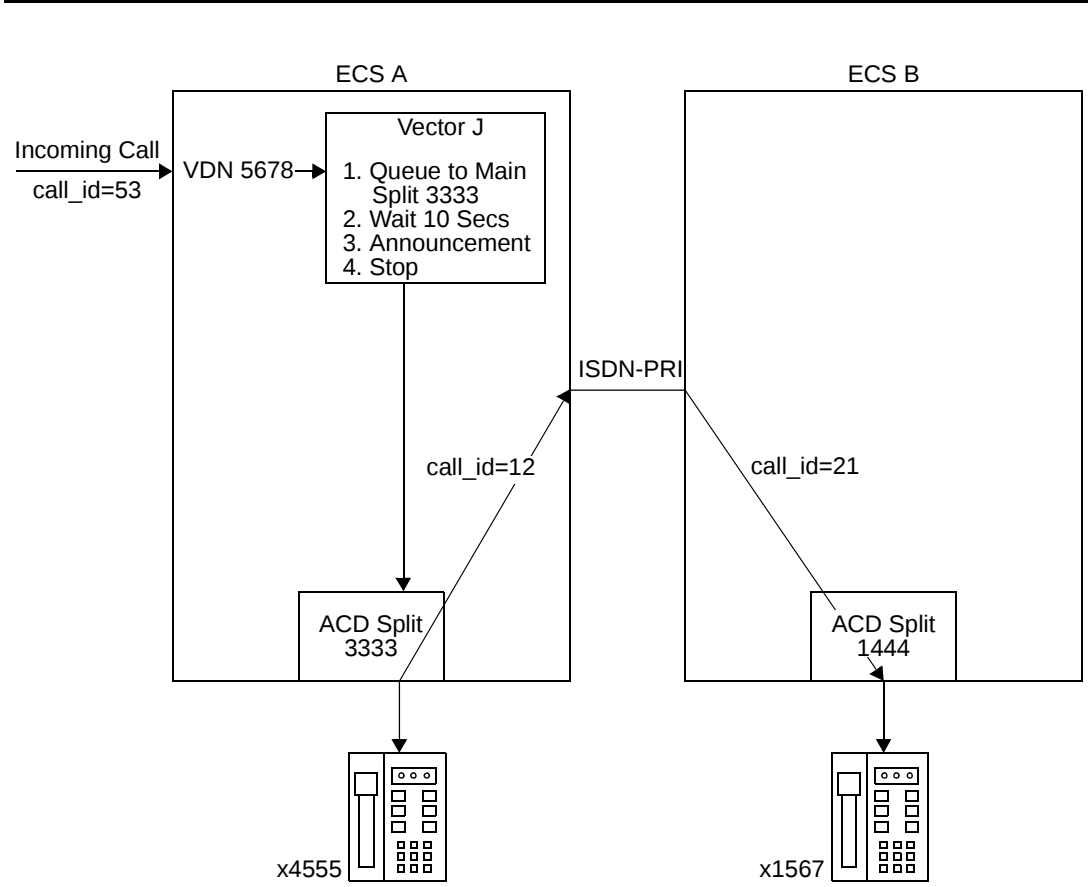
Figure A-3. Call Flow for Consultation Transfer to Another ECS
