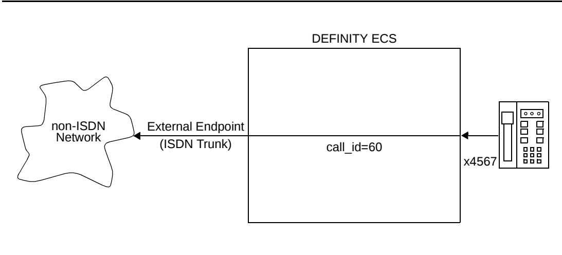
Figure A-17. Call Flow for Outgoing ISDN Call that Traverses a non-ISDN Network
