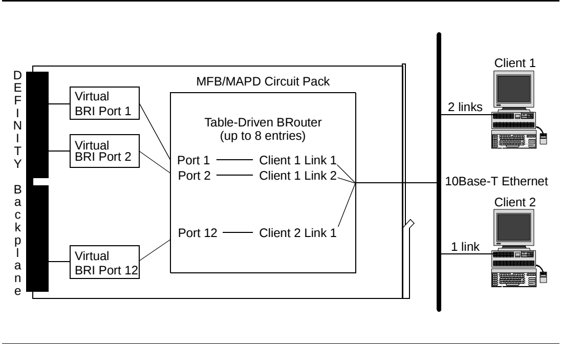
Figure 13-6. Relationship of Virtual BRI Ports, Brouter, and DEFINITY LAN Gateway Clients
