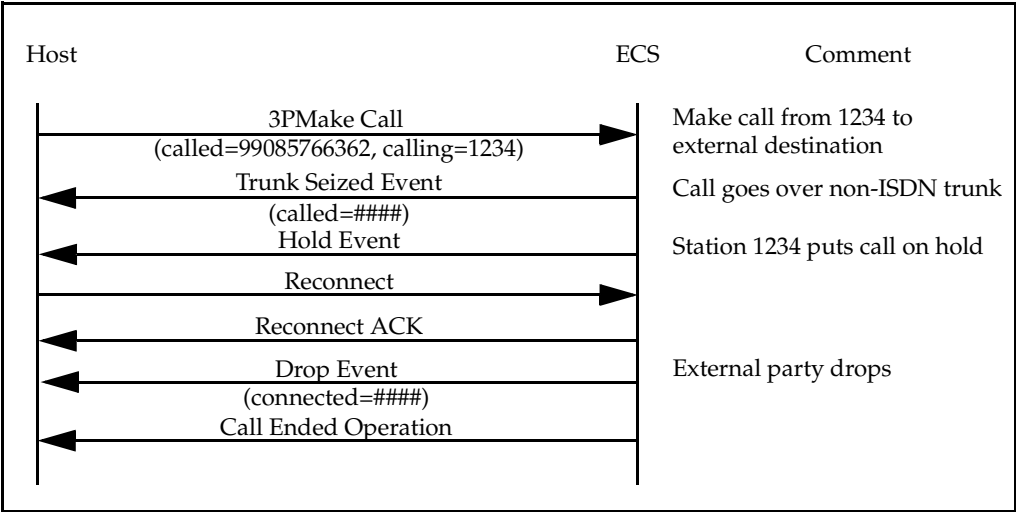
Figure A-16. Outgoing Call over Non-ISDN Trunk
